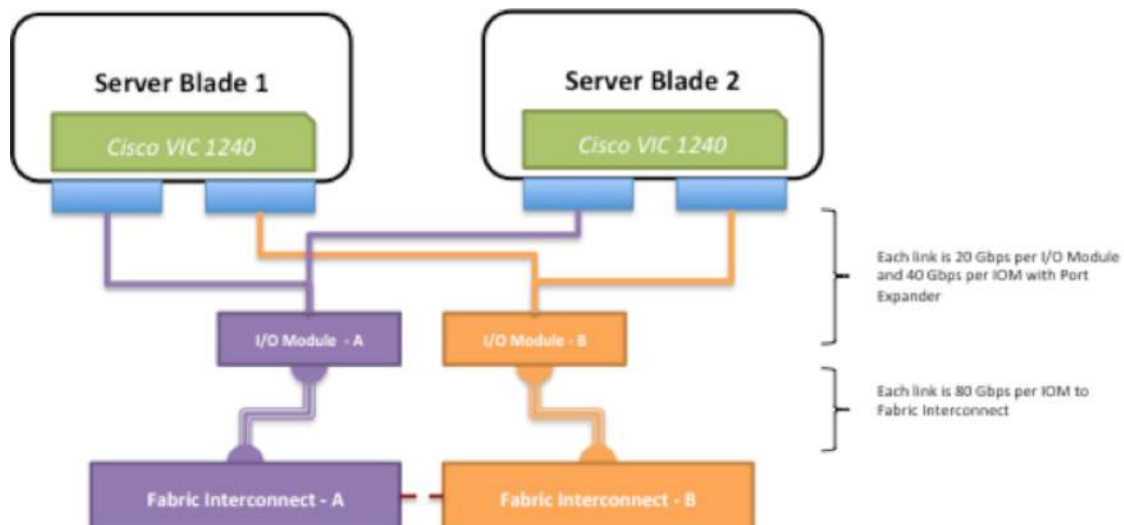
Figure 4. Network Topology
