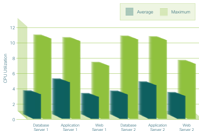
Figure 5. A Two-Node Cisco UCS Configuration Easily Handled Oracle PeopleSoft North American Payroll Processing for 240,000 Employees, with Low CPU Utilization
