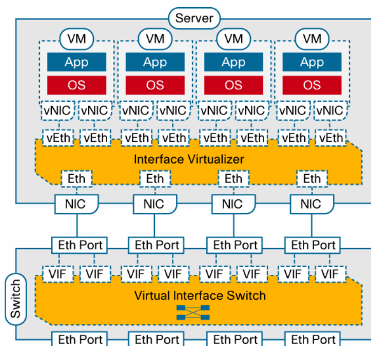
Figure 4. Architectural Elements of the NIV Model
