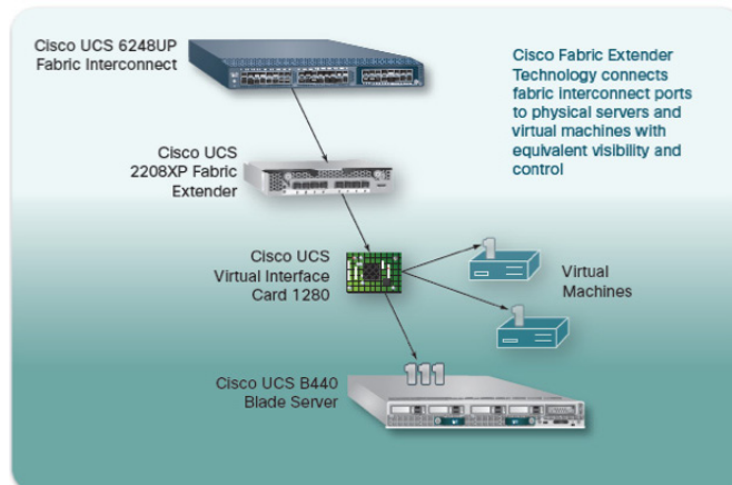
Figure 5: Cisco Fabric Extender Technology
