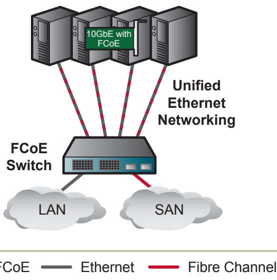
Figure 4. FCoE enables unified Ethernet networking, passing SAN and LAN traffic over a single 10 gigabit ethernet NIC.
