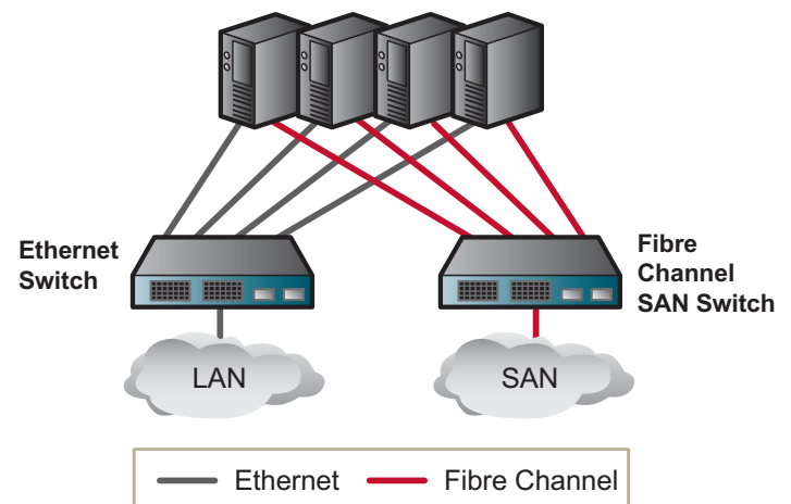
Figure 2. Today, most data centers use separate LAN and SAN networks with separate switches and network adapters in the server; for Fibre Channel SANs. This topology requires a dedicated Fibre Channel infrastructure.
