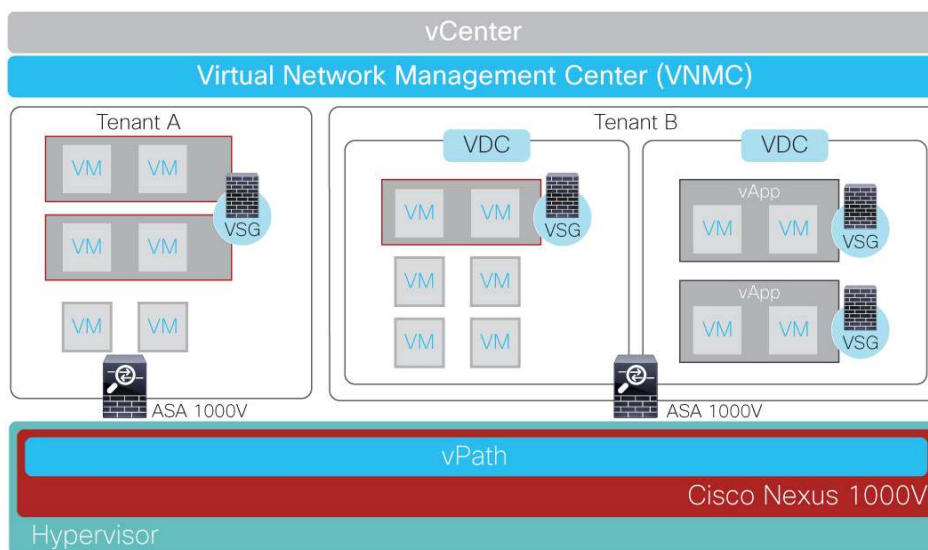
Figure 2. Illustrates how the Cisco ASA 1000V integrates with the Nexus 1000V virtual switch and Cisco VSG.
