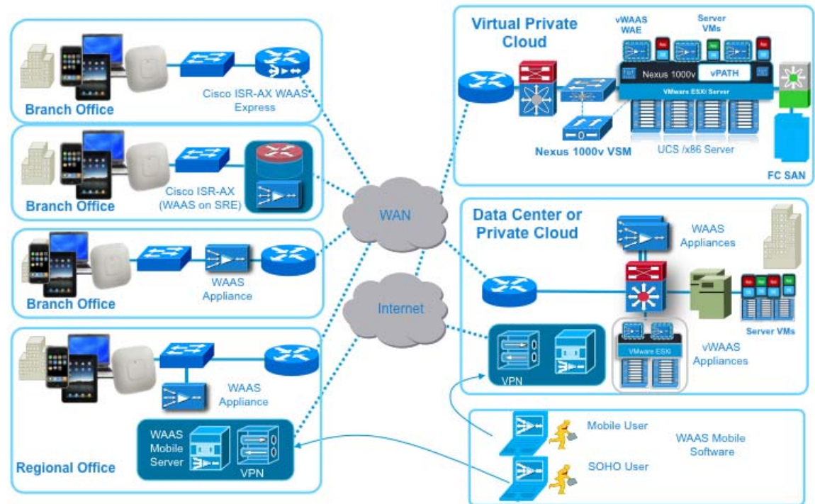
Figure 2 Branch Office BYOD Planning Architecture
