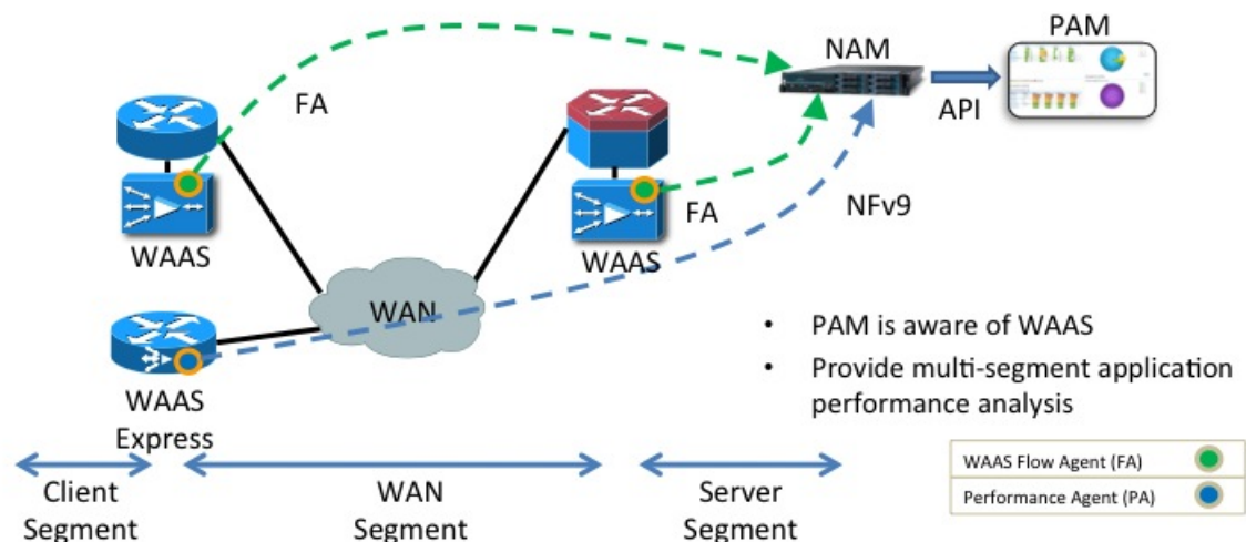
Figure 5 Cisco Flow Agent and Performance Agent
