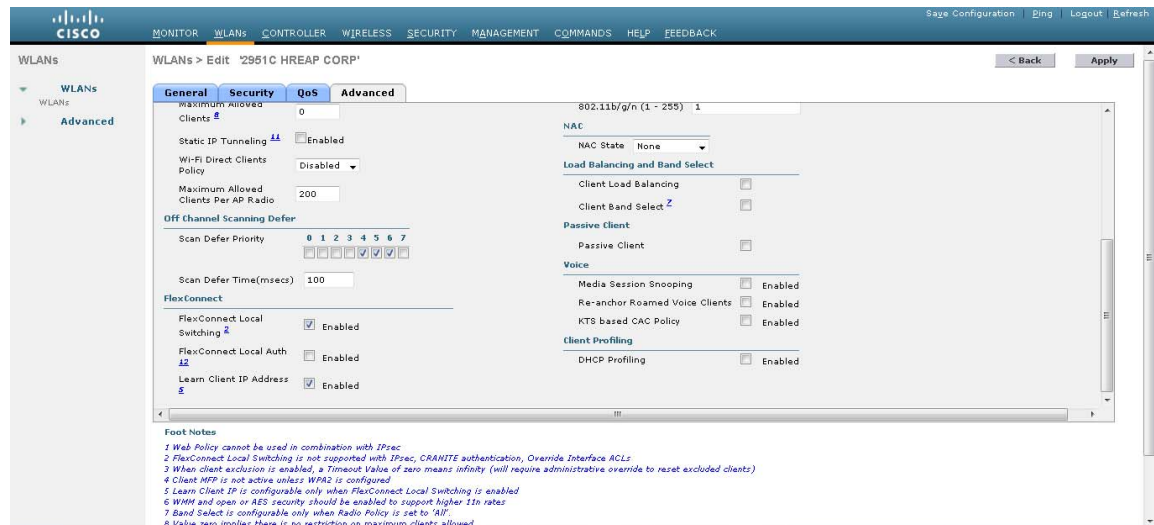
Figure 3 Cisco FlexConnect to Enable Local Switching
