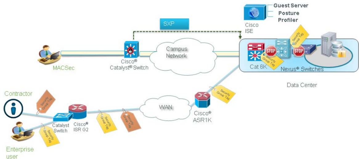
Figure 4 Identity and Security with TrustSec
