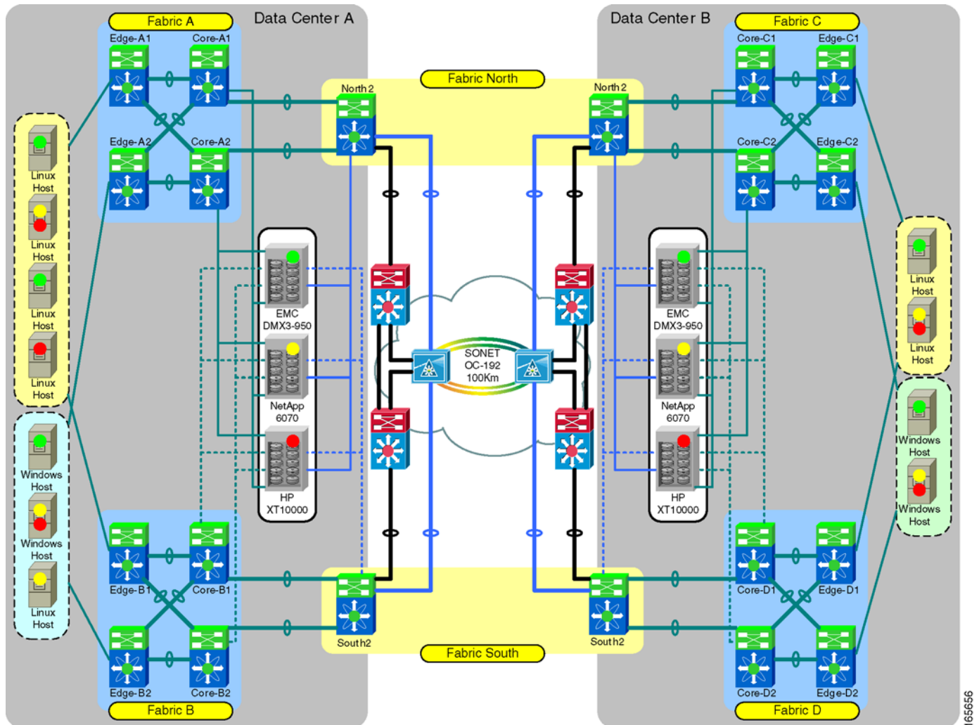
Figure 4-1 DCAP SAN Test Topology Overview
