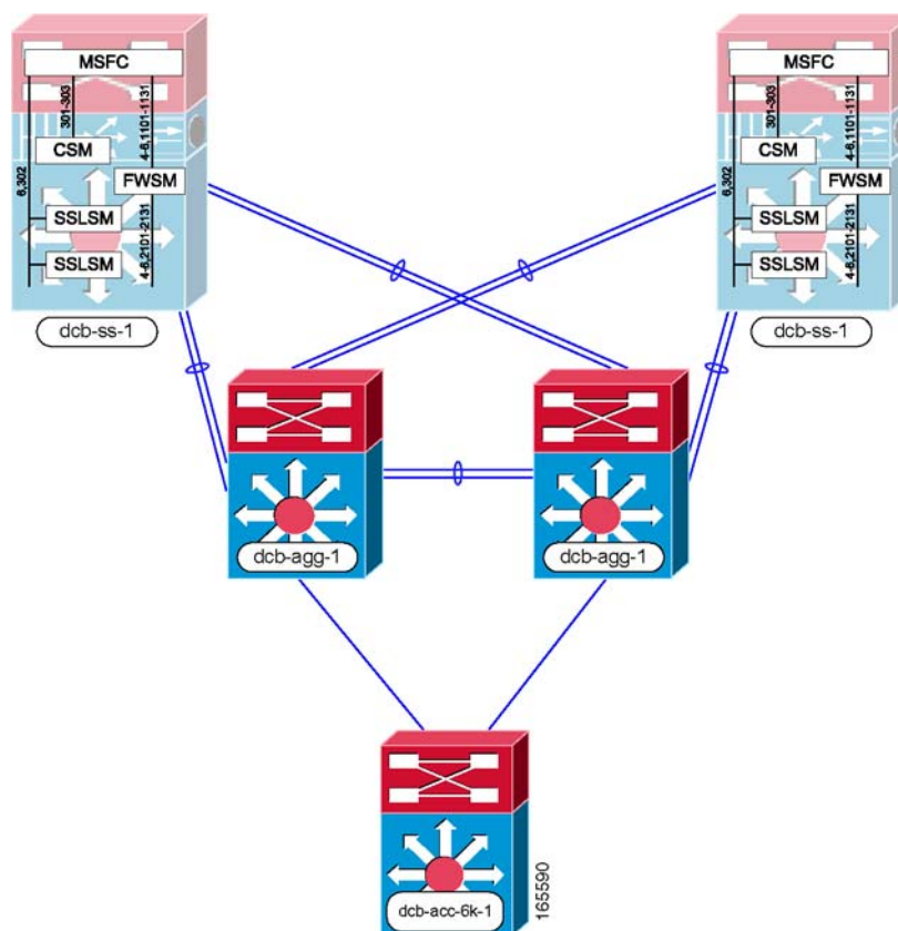
Figure 3-6 Logical and Physical Configuration of the Service Switch Deployment in DC-B
