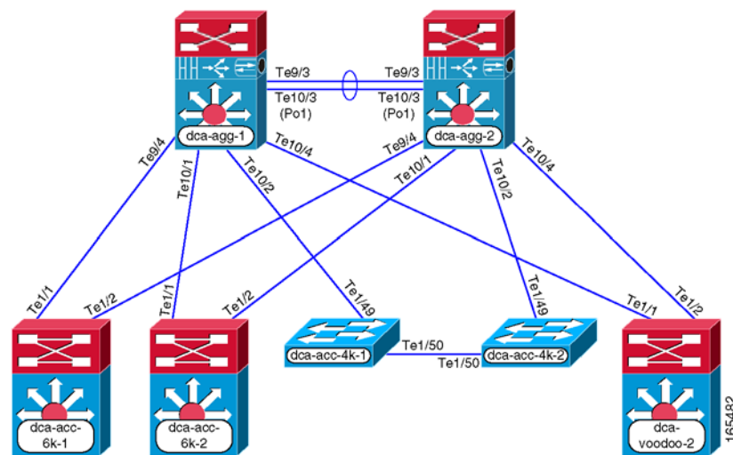
Figure 2-2 Layer 2 Topology
