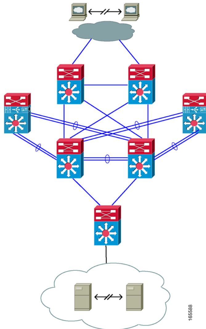
Figure 3-1 Service Switch Overview Topology in DC-B
