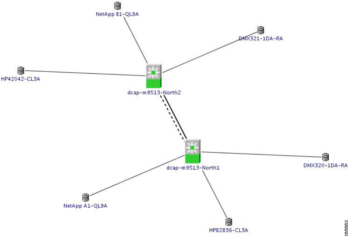
Figure 4-8 Fabric Manager Topology Map for North Transit Fabric
