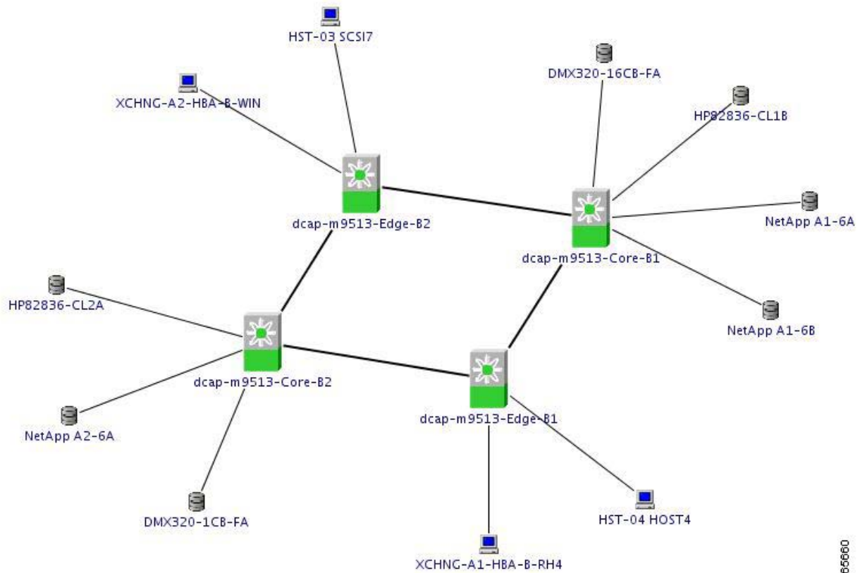
Figure 4-5 Fabric Manager Topology Map for Fabric B
