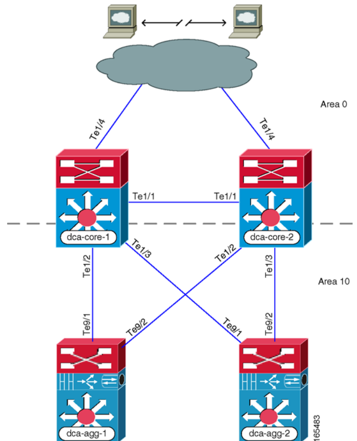
Figure 2-3 Layer 3 Topology
