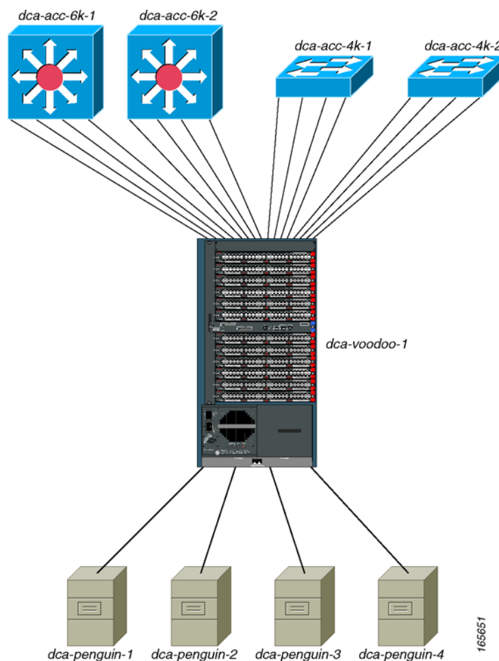
Figure D-1 Catalyst 6513 Used in Voodoo Solution
