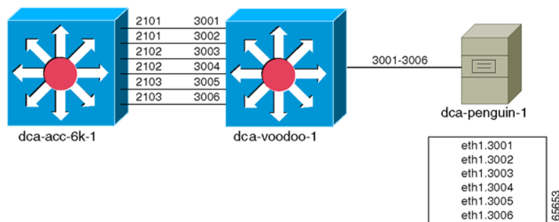
Figure D-3 Voodoo Solution Using a Dedicated 802.1q Subinterface for Each Emulated Server
