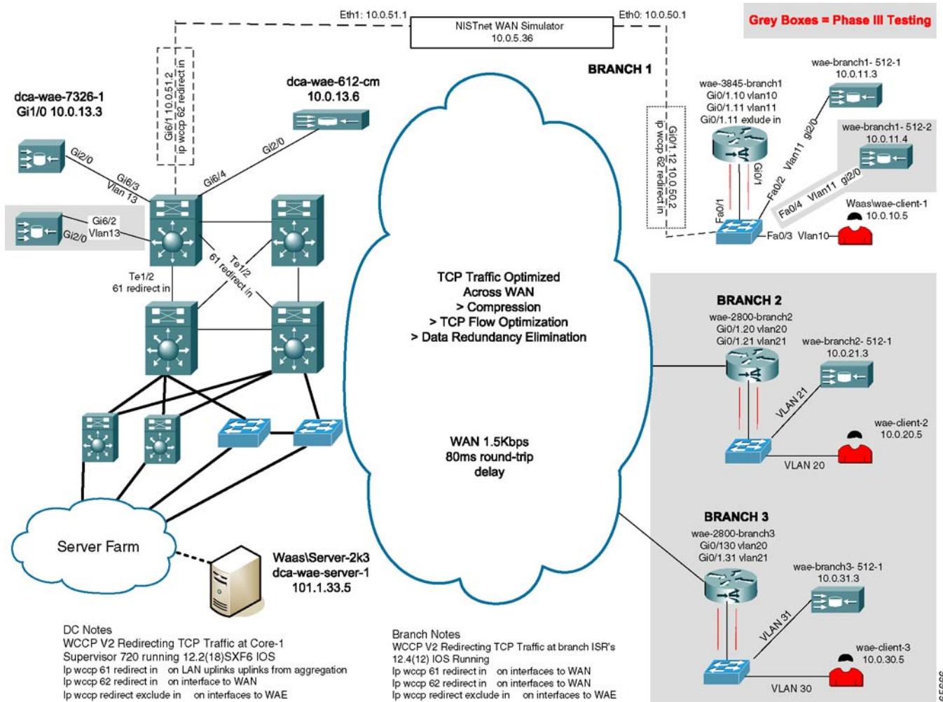
Figure 6-1 DCAP WAAS Test Topology
