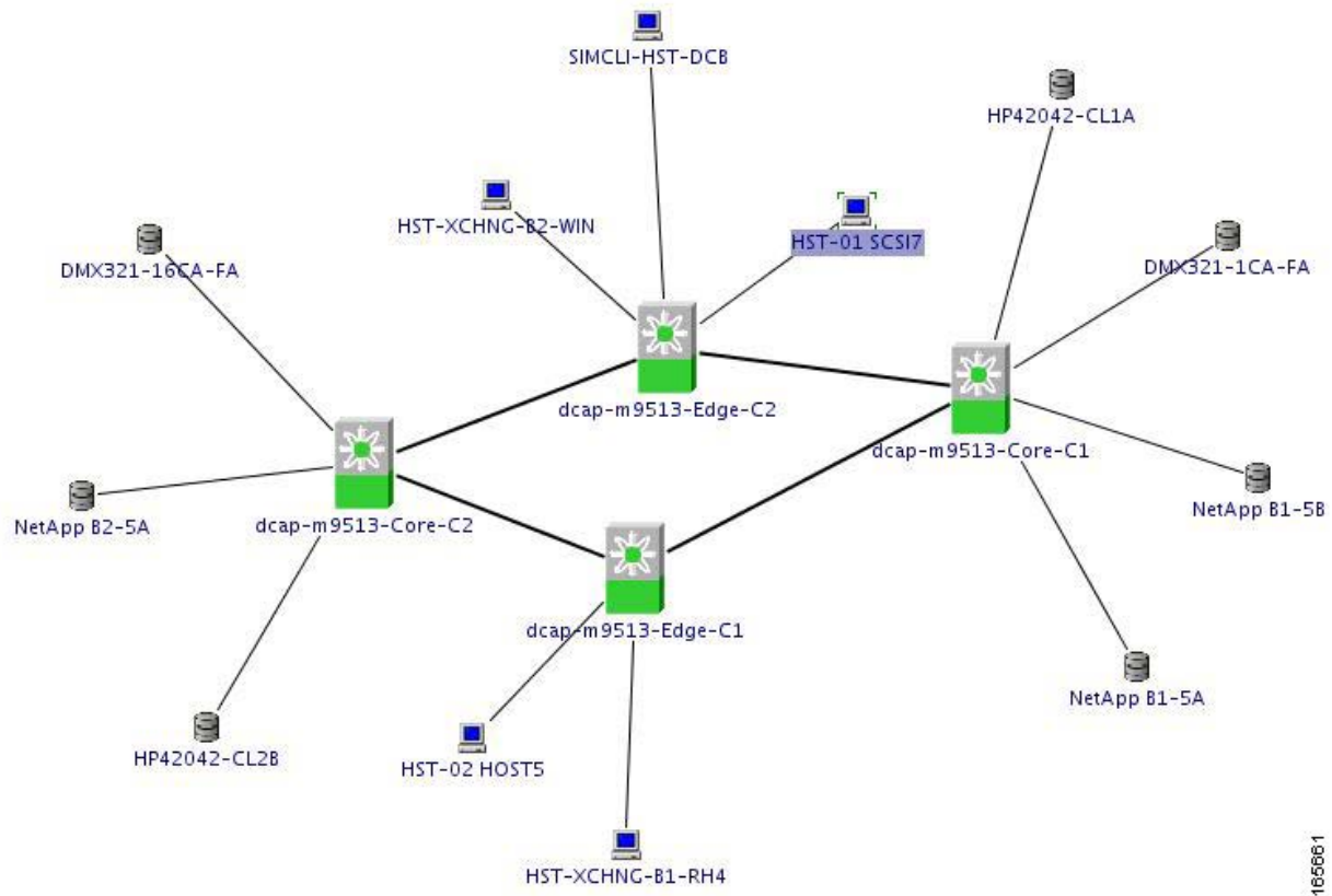
Figure 4-6 Fabric Manager Topology Map for Fabric C
