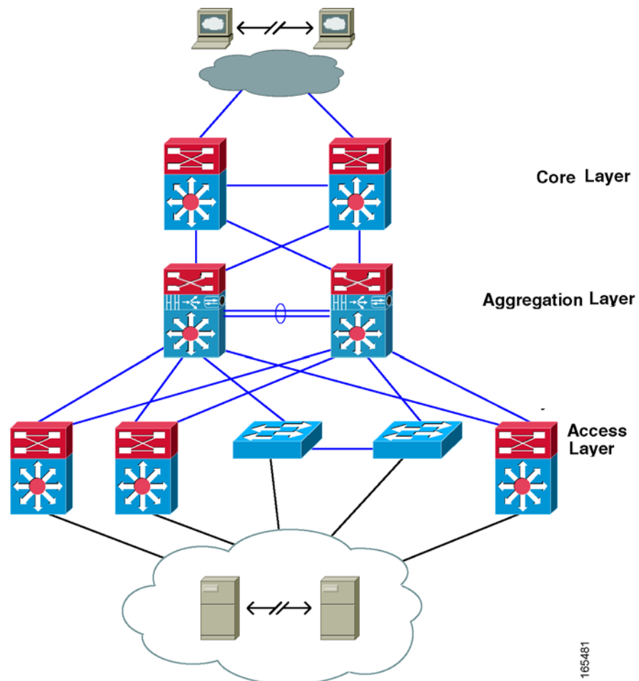
Figure 2-1 DCAP Logical Topology
