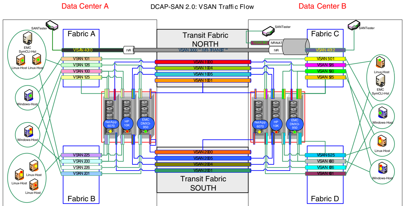
Figure 4-3 DCAP SAN VSAN Traffic Flow
