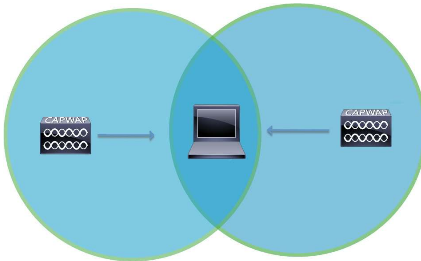
Figure 8. Co-Channel Interference
