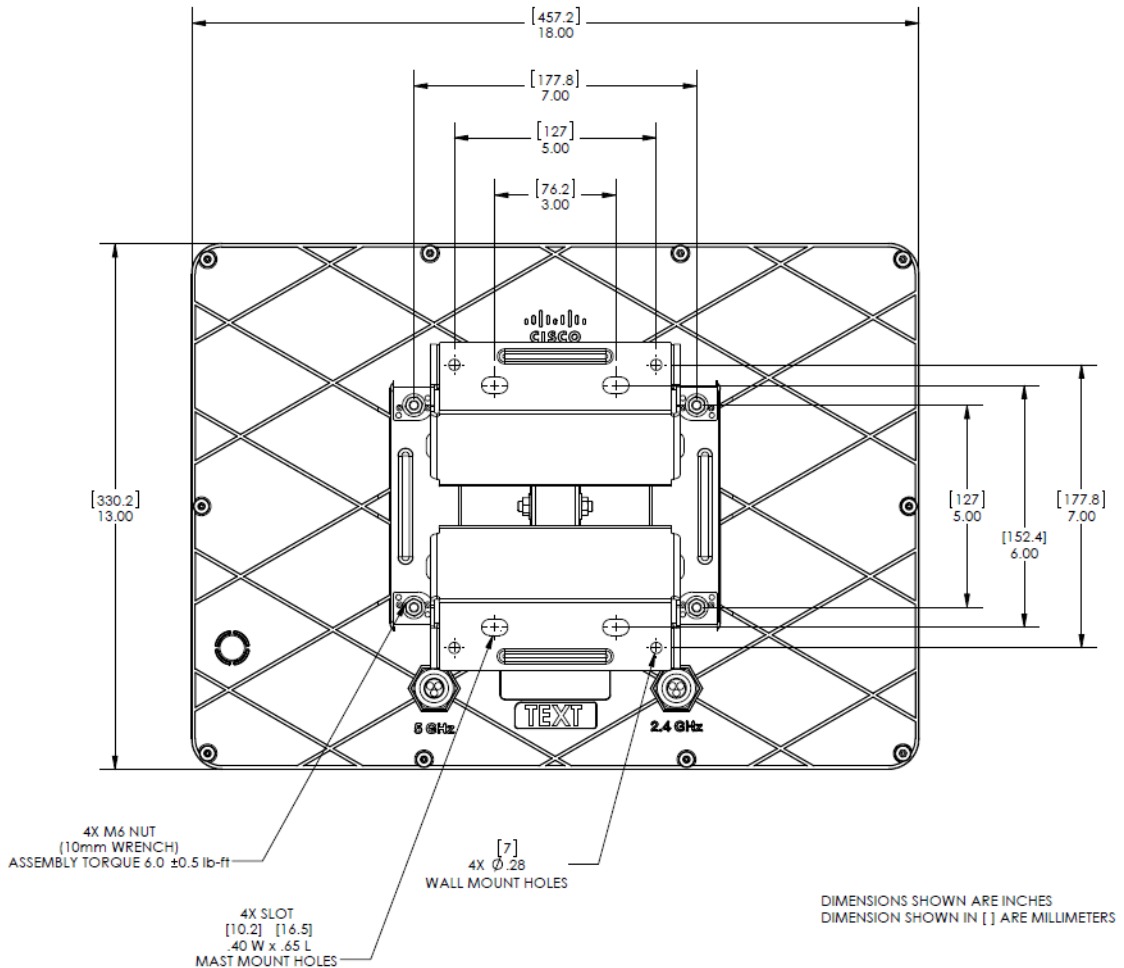
Figure 1 Bear View of Antenna and Bracket
