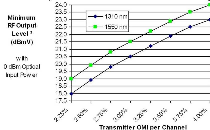
Receiver RF Output Level Vs Transmitter OMI – Rx switch in -6 dB setting
