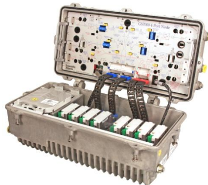
Figure 1. GS7000 4-Way Segmentable Node with 55/70 MHz Split
