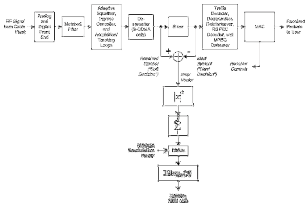
Figure 11. Block Diagram of Generalized Digital QAM Receiver, Showing Computation of Receive MER
