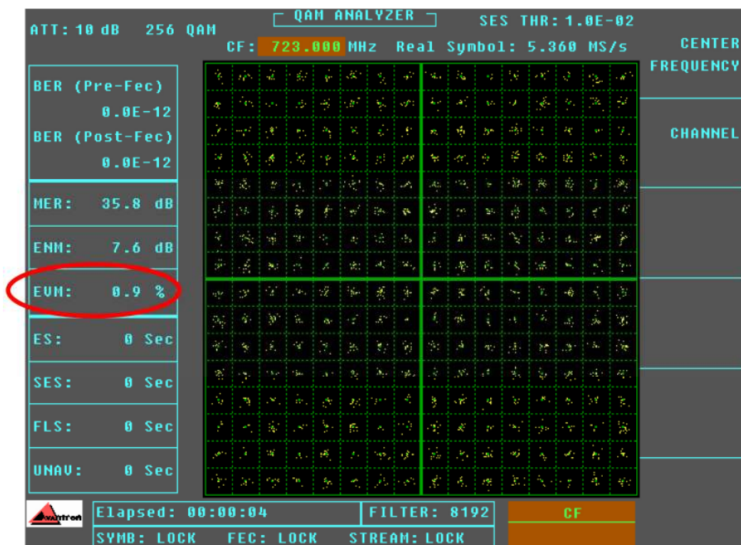
Figure 16. The EVM of This Downstream 256-QAM Digitally Modulated Signal Is 0.9 Percent. (Courtesy of Sunrise Telecom)
