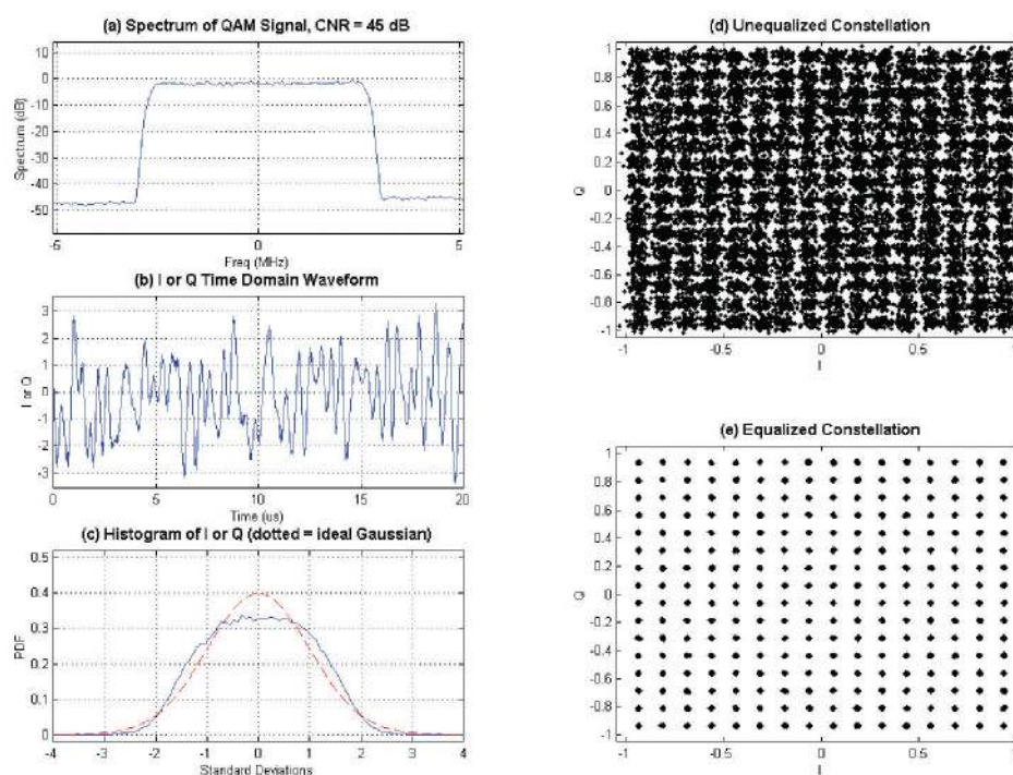
Figure 9. Views of a QAM Waveform (256 QAM, E_s/N_0 = 45 dB, with slight channel amplitude tilt and ripple)
