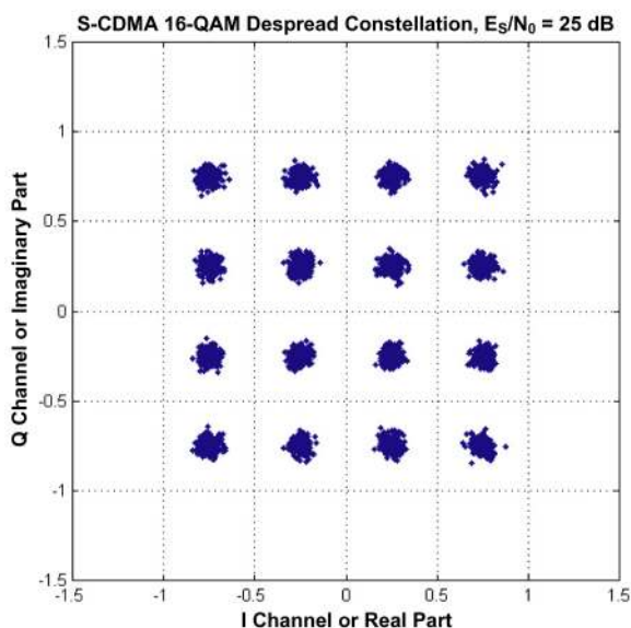
Figure 23. S-CDMA 16-QAM Constellation with 25-dB RxMER
