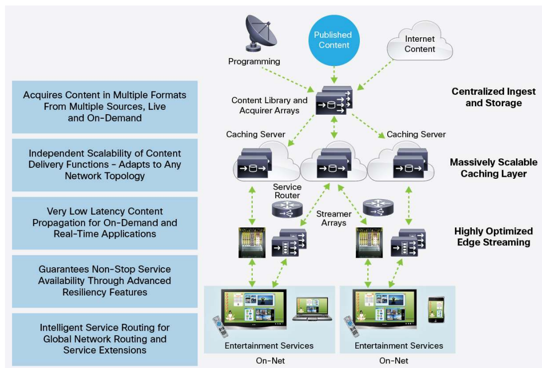
Figure 1. Cisco VDS Internet Streaming Solution
