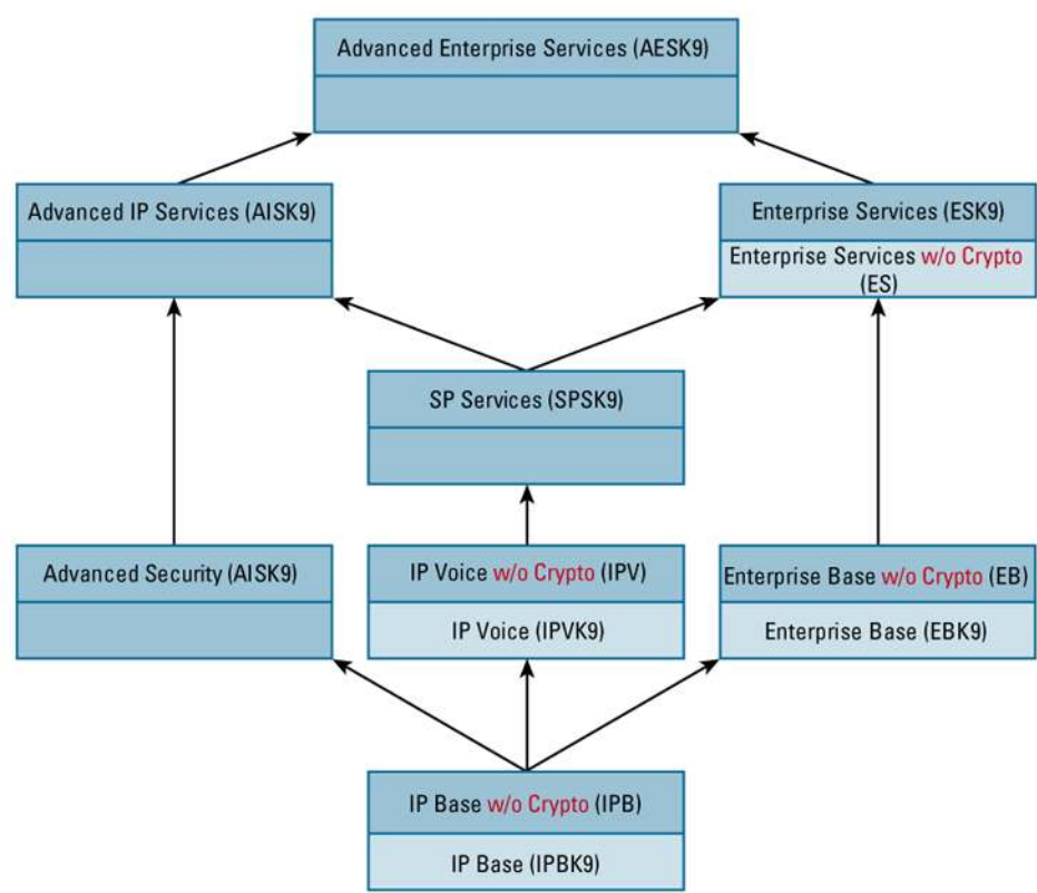
Figure 1. Reformation Feature Map
