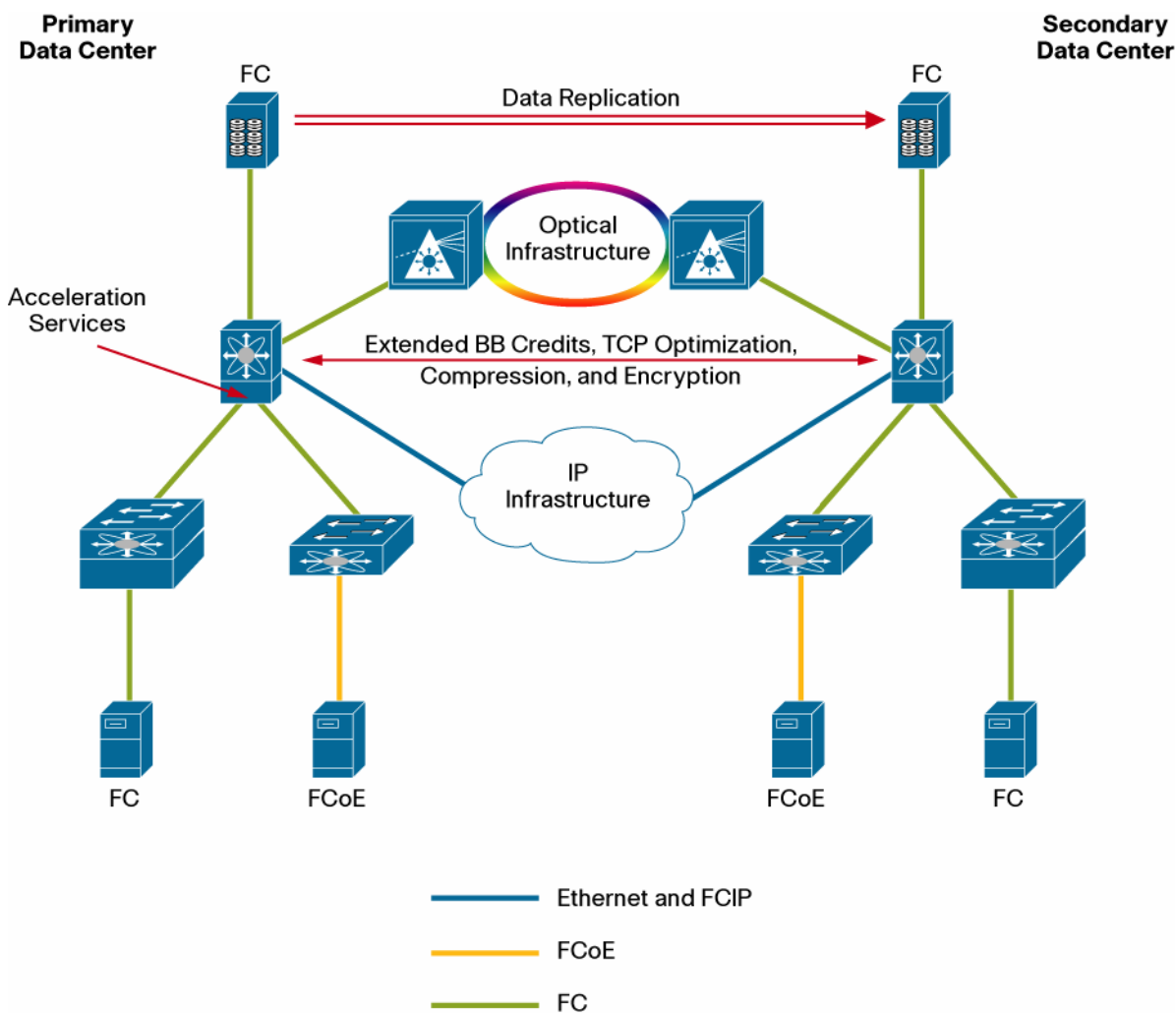
Figure 12. Flexible SAN Extension Solutions
