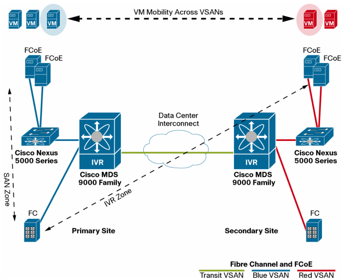
Figure 7. IVR: Enables Long-Distance Virtual Machine Mobility
