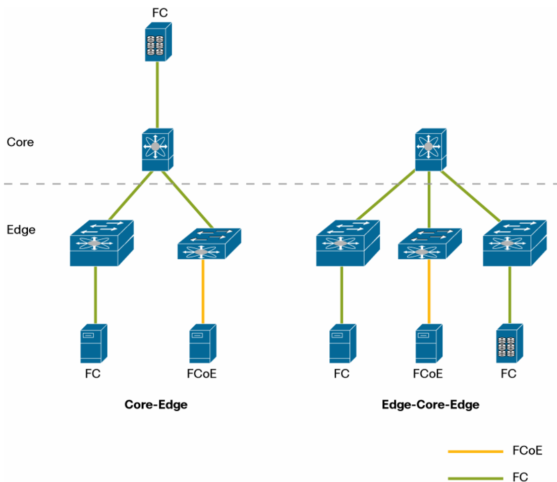
Figure 2. Core-Edge and Edge-Core-Edge Topologies
