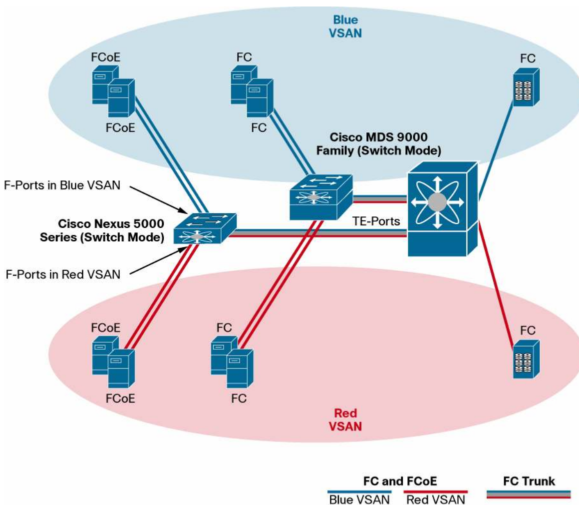
Figure 3. Trunking Expansion Port in Switch Mode
