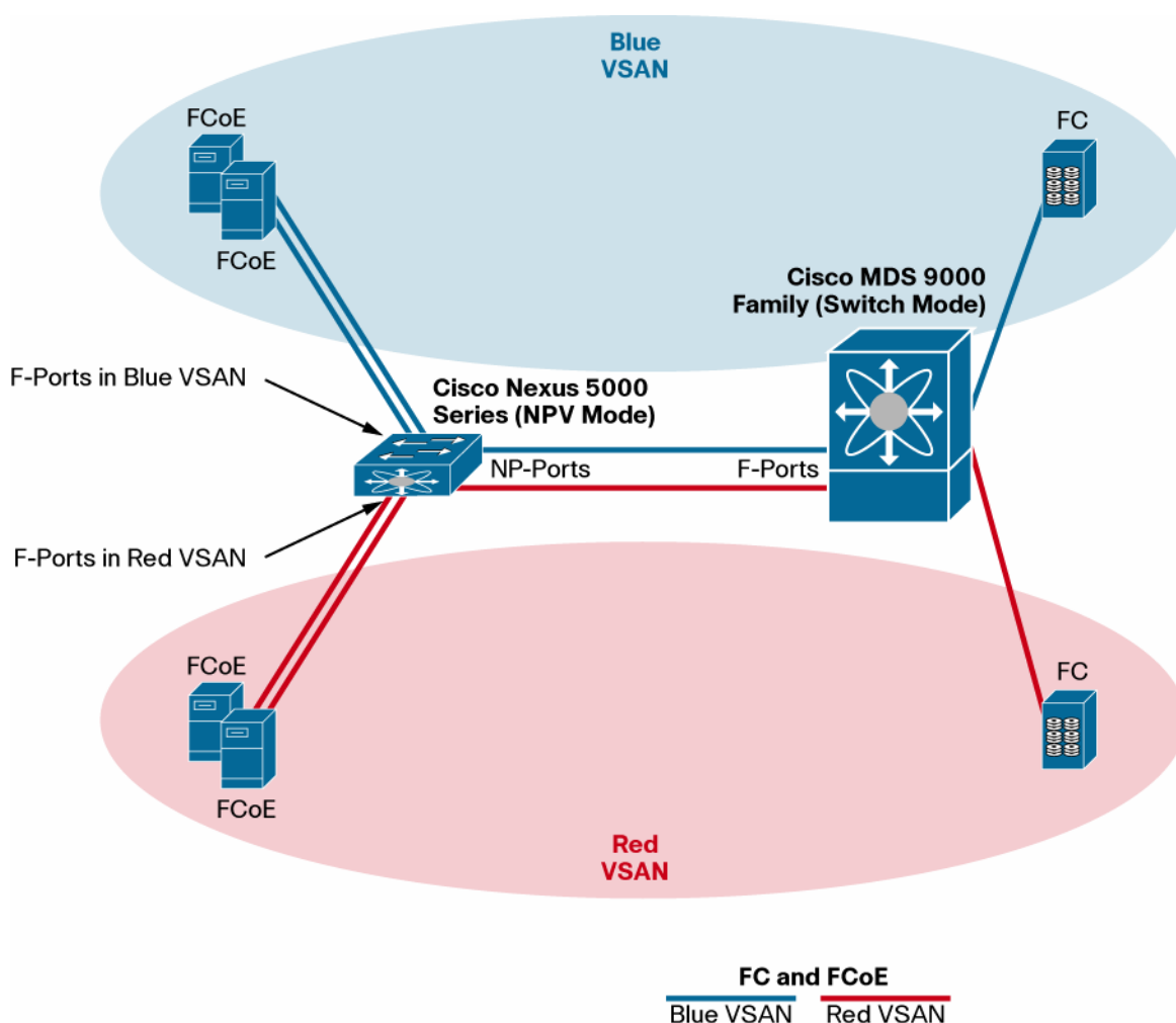
Figure 5. Automatic VSAN Selection on the Uplink
