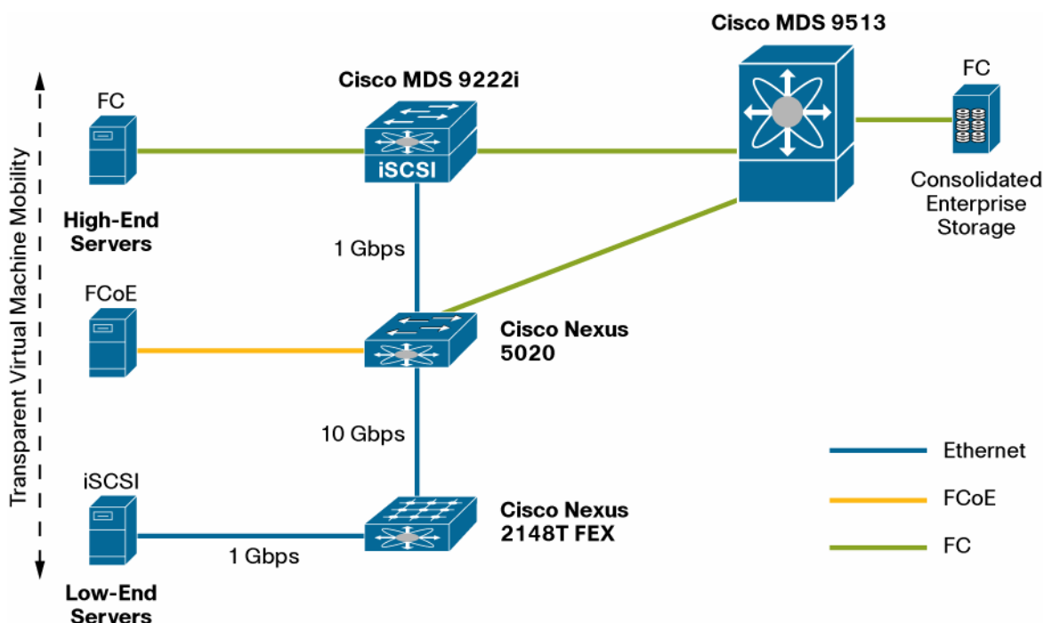
Figure 11. Transparent Integration of Fibre Channel, FCoE, and iSCSI
