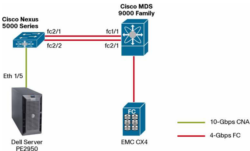
Figure 13. Topology
