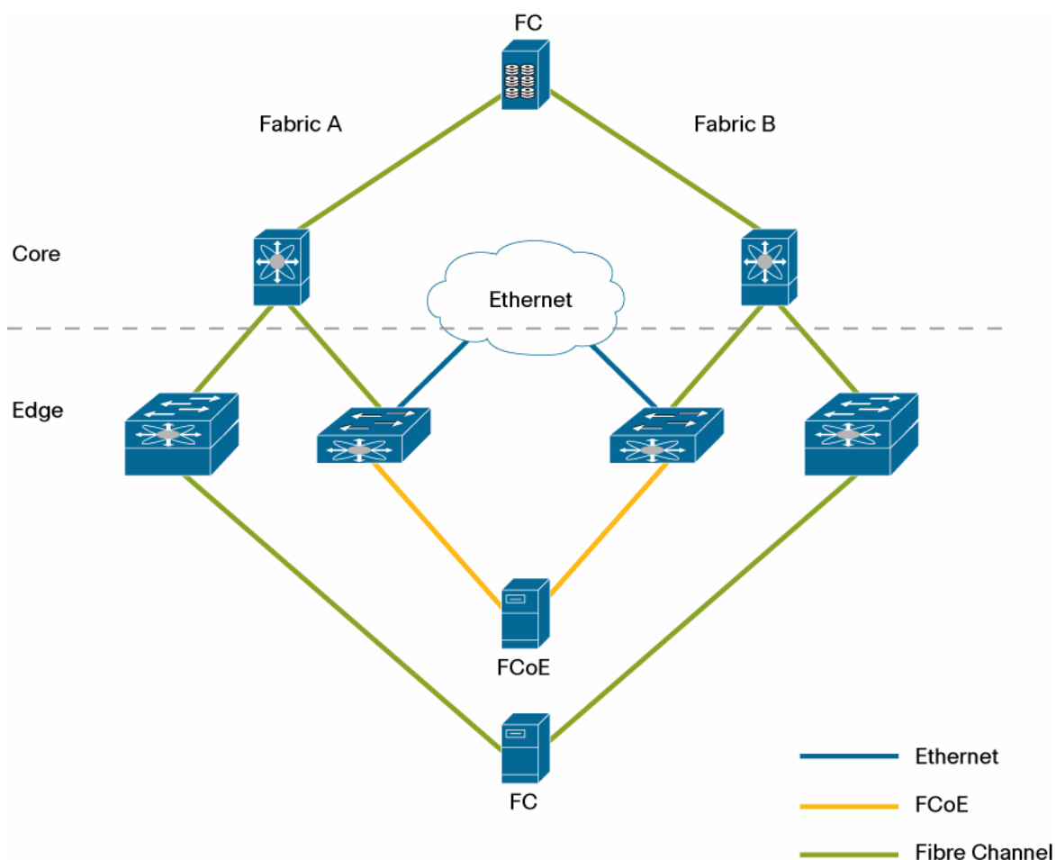
Figure 1. Dual Fabric in a Unified I/O Deployment
