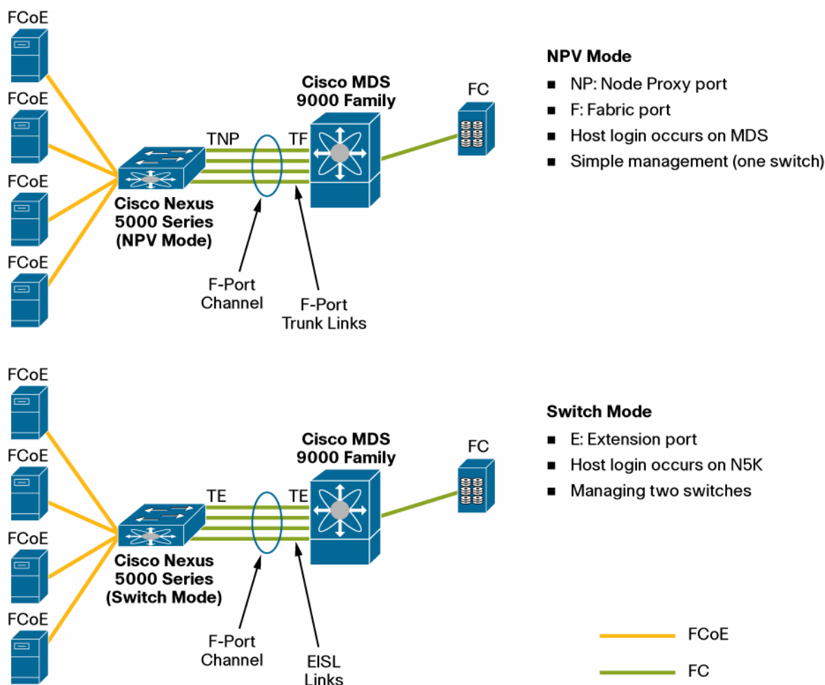
Figure 8. SAN Port Channel and Trunking
