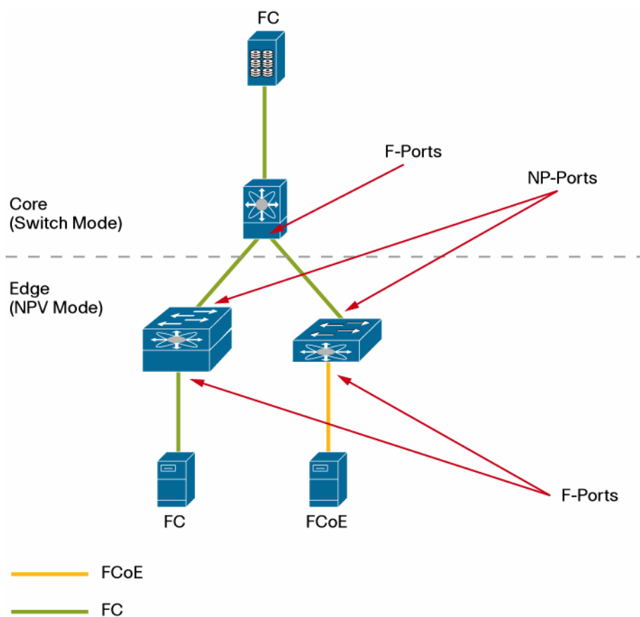
Figure 4. Edge Switch in NPV Mode with, Node Proxy Port (NP-Port)
