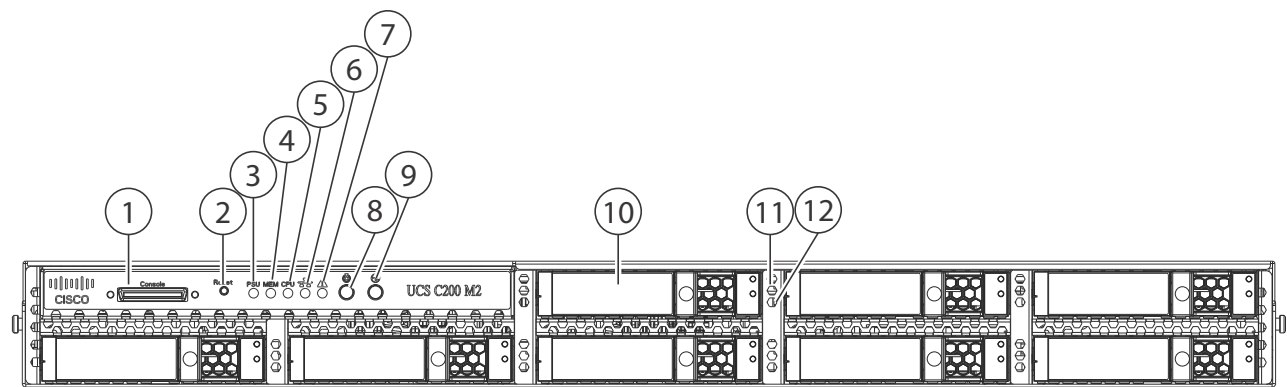
Figure 2 Chassis Front View (Control Panel Installed)
