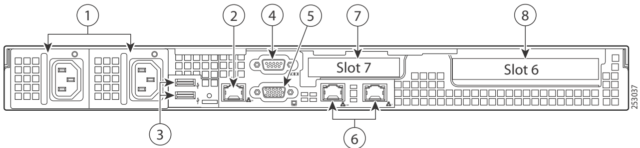
Figure 4 Chassis Rear View
