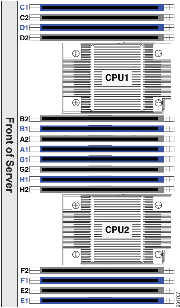
Figure 7 Physical Layout of CPU DIMM Channels and Banks
