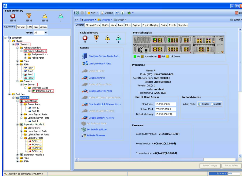
Figure 3. Cisco UCS Manager Discovers Resources When They Are Plugged into the System, Adding Them to Inventory or Provisioning Them Automatically
