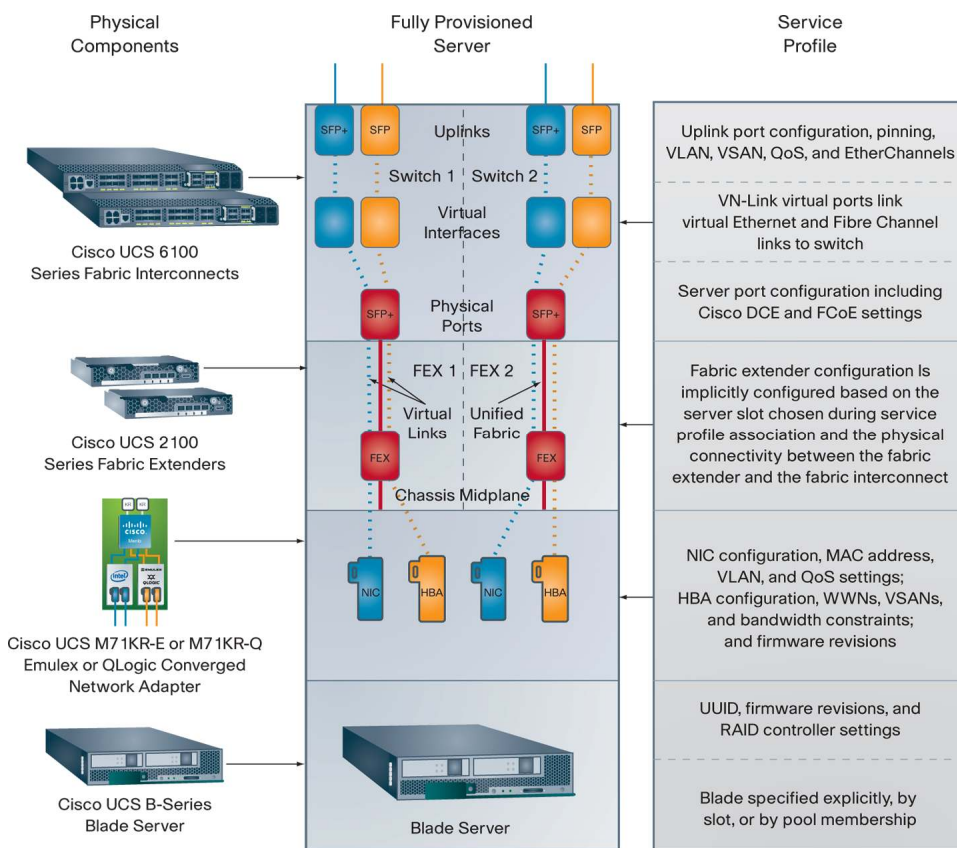
Figure 4. Service Profiles Specify How Physical Components Are Used to Provision Servers and Their Interconnects
