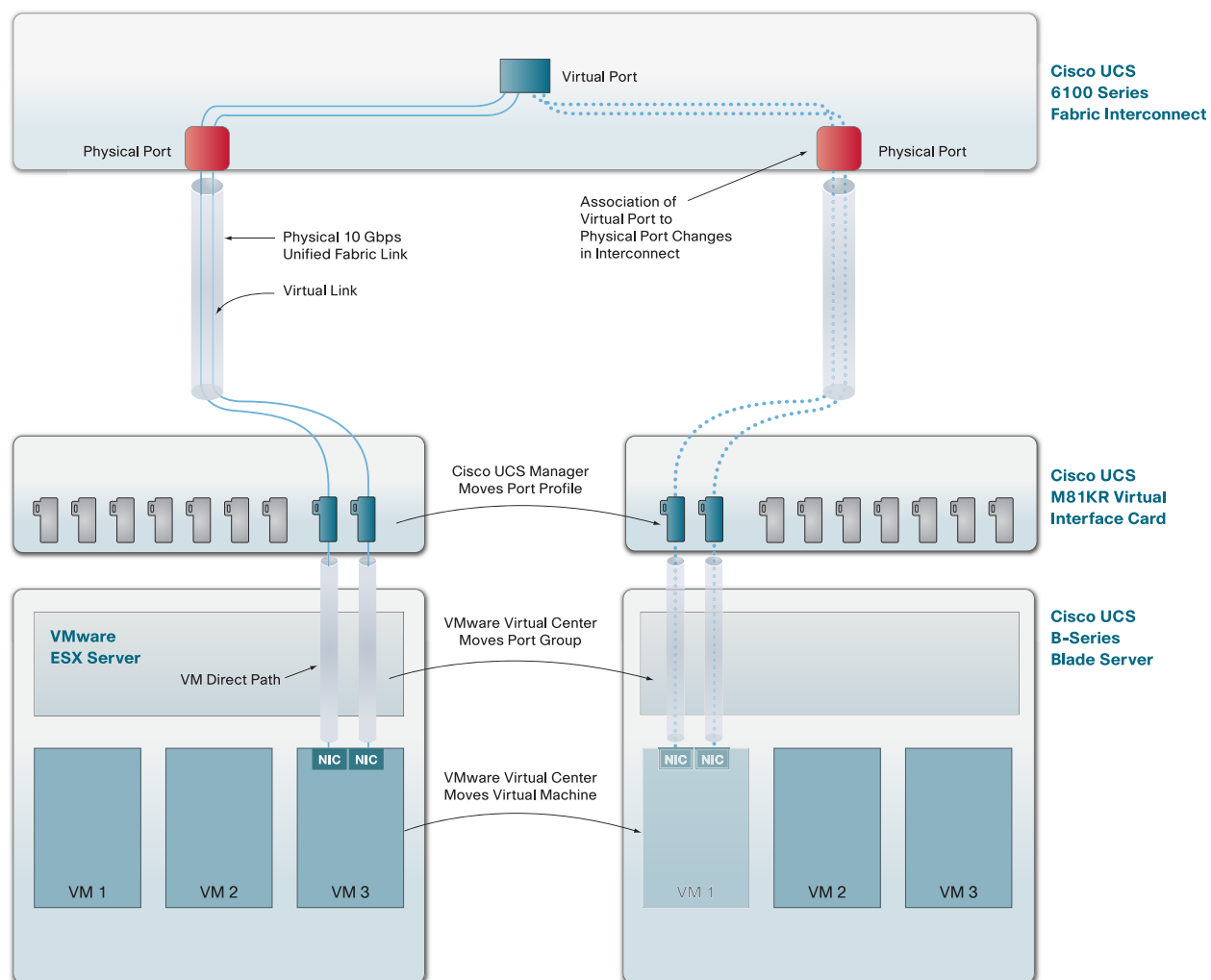
Figure 5. Cisco VN-Link Technology Enables Per-Virtual-Machine Links That Are Managed and Moved Independently of Physical Links
