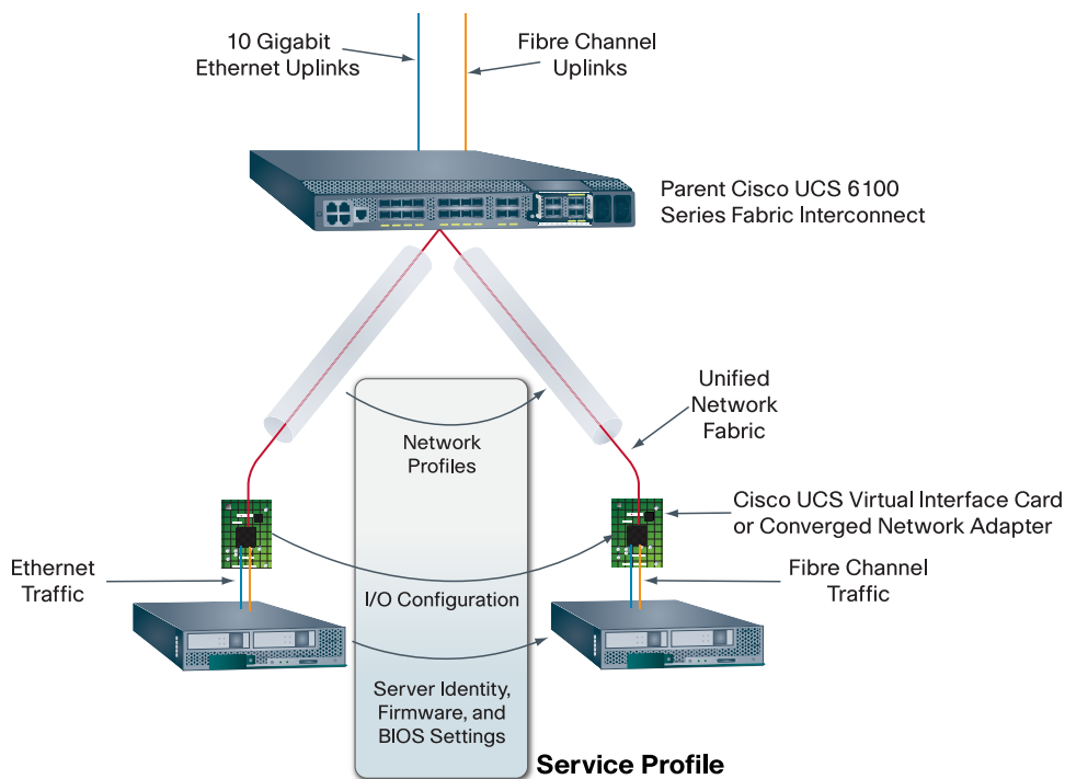
Figure 2. Service Profiles Provision Server and Network Resources and Can Move Server Configurations Between Physical Servers
