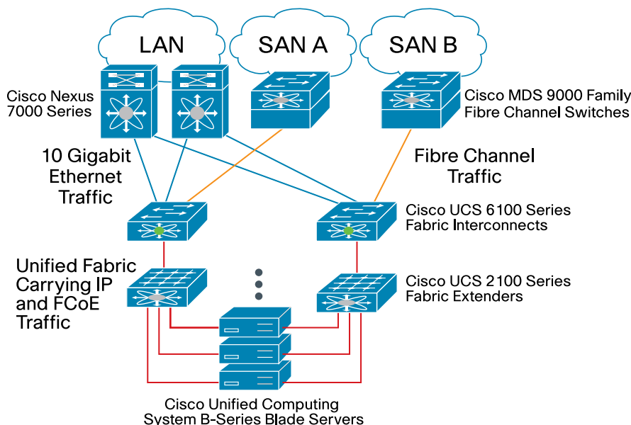
Figure 1. A Unified Fabric Carries Multiple Traffic Streams to Cisco UCS 6100 Series Fabric Interconnects, Where Ethernet and Fibre Channel Traffic Splits onto Separate Networks
