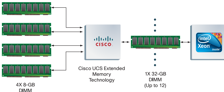
Figure 3. Cisco Extended Memory Technology Makes Four Physical DIMMs Appear to the CPU as a Single, Large, Logical DIMM
