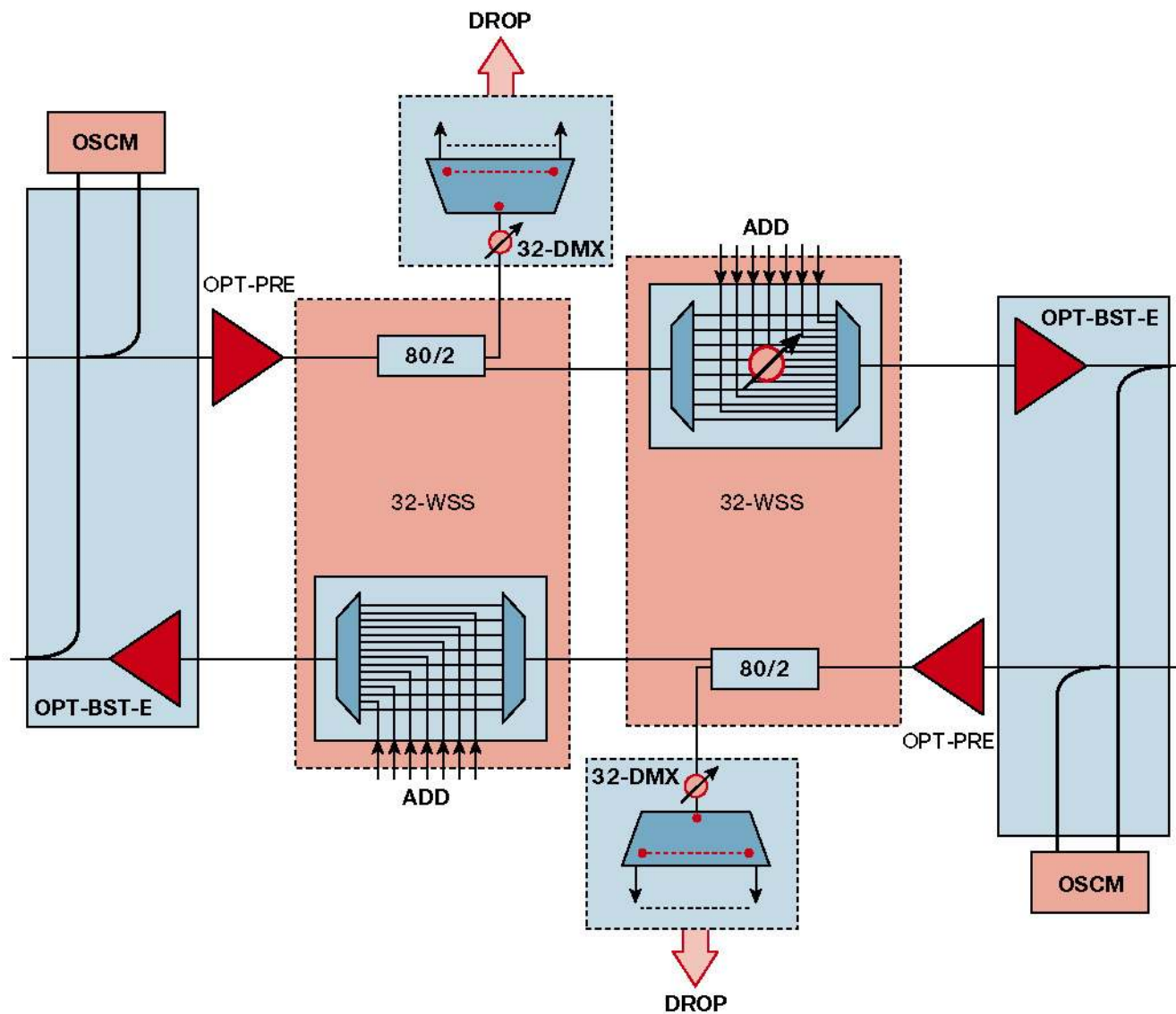
Figure 2 32 Channel ROADM Node
