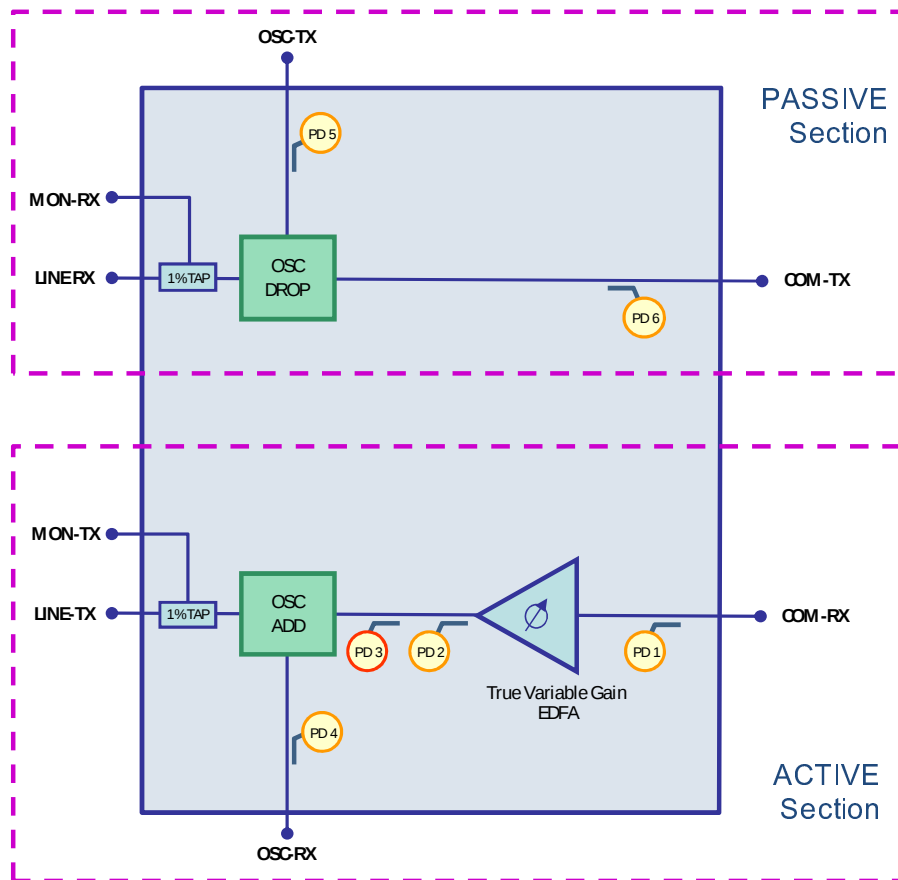
Figure 2. Functional Block Diagram (OPT-EDFA-17 and OPT-EDFA-24)
