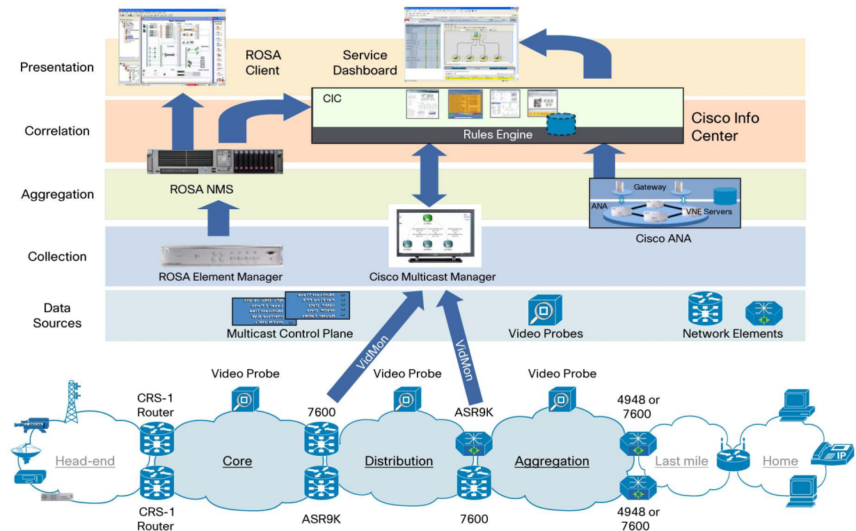
Figure 1. Cisco VAMS 3.0 Reference Architecture
