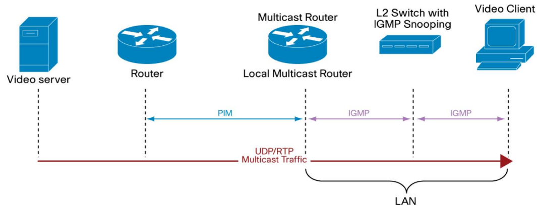
Figure 2. A Typical IP Multicast Network Configuration
