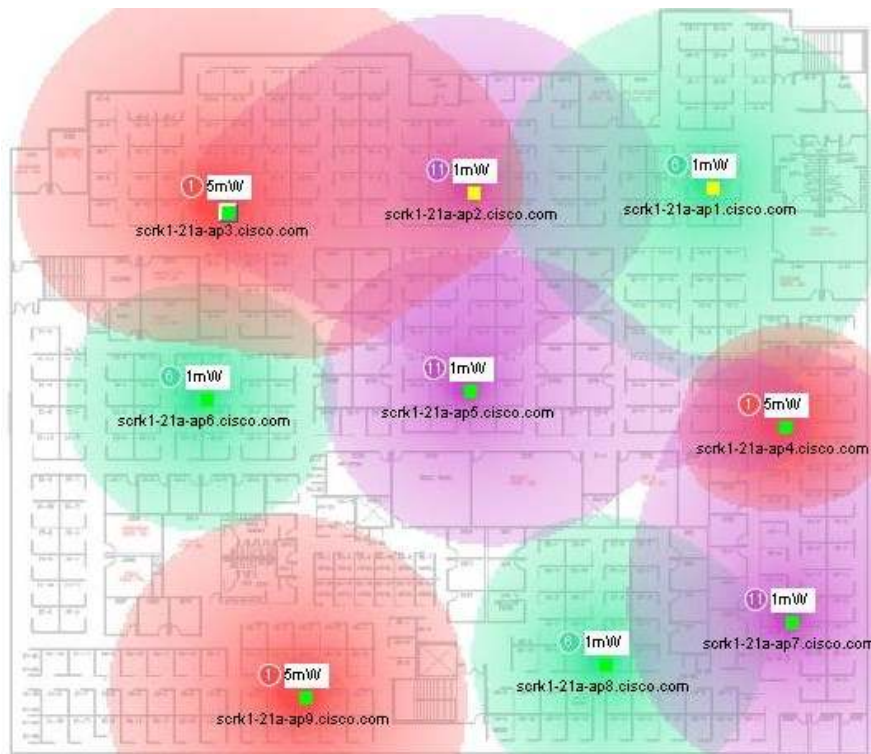
Figure 2. CiscoWorks WLSE Express: RF Coverage
