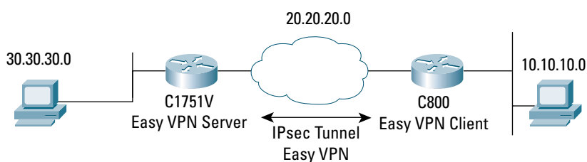
Figure 1 Network Diagram
