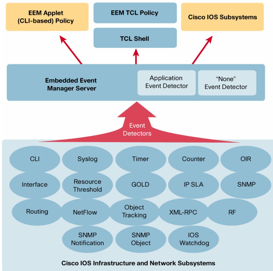
Figure 1. EEM Architecture
