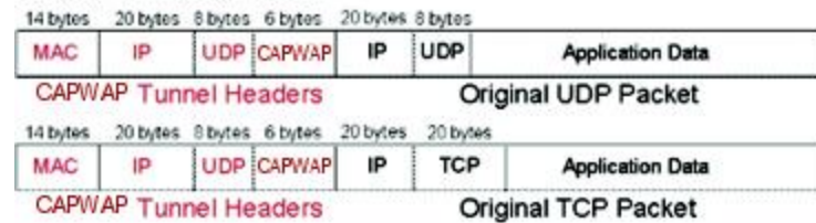
Figure 8: CAPWAP Tunneled Packets
