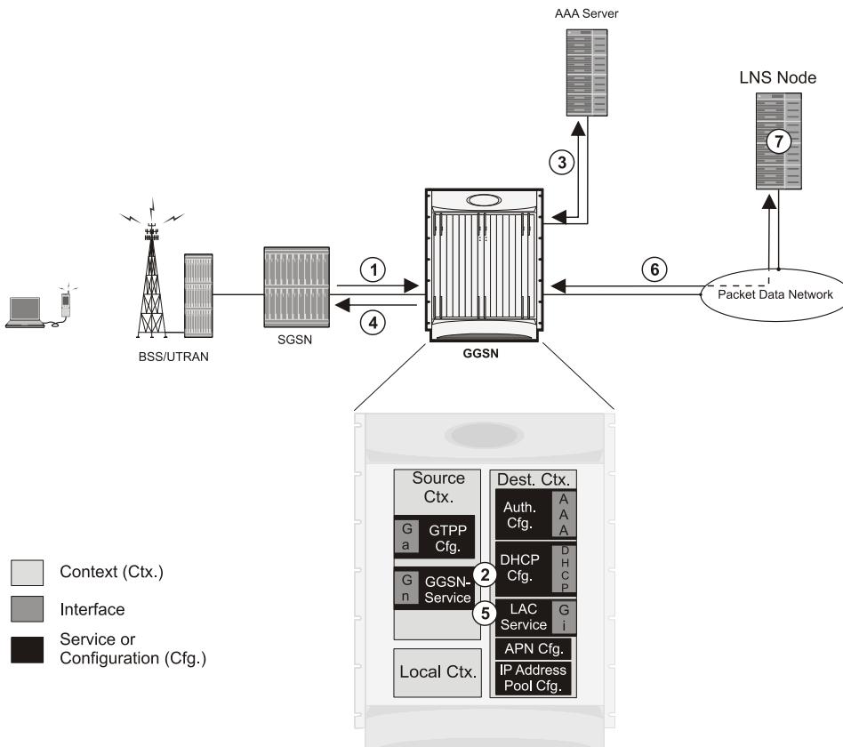
Figure 31. Non-transparent IP PDP Context Call Processing with L2TP Tunneling
