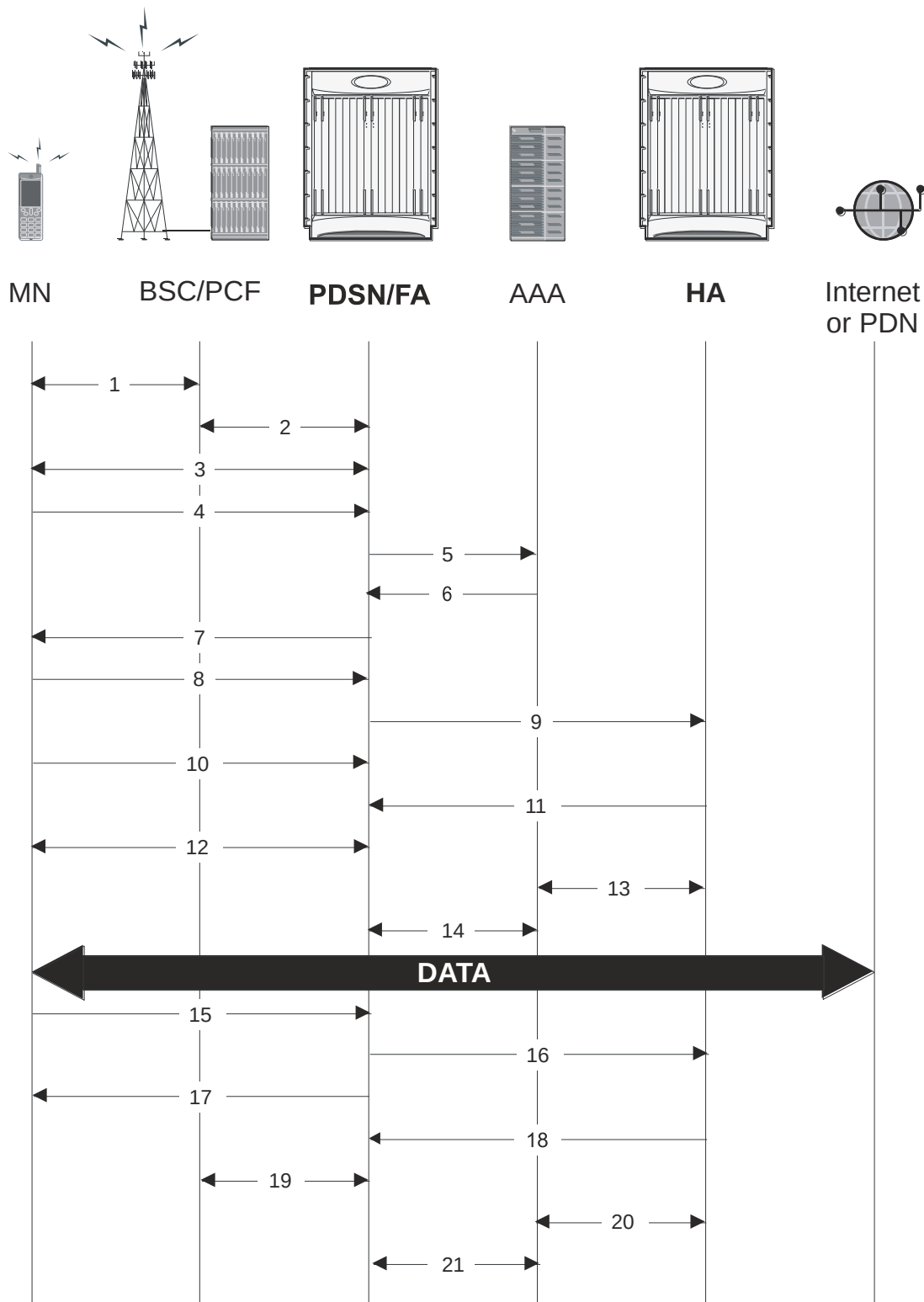
Figure 49. HA Assigned IP Address Proxy Mobile IP Call Flow
