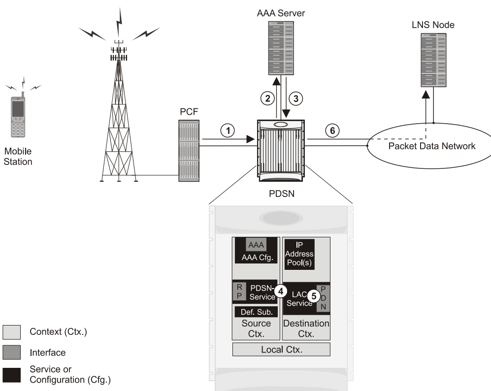
Figure 27. Attribute-based L2TP Session Processing for SIP
