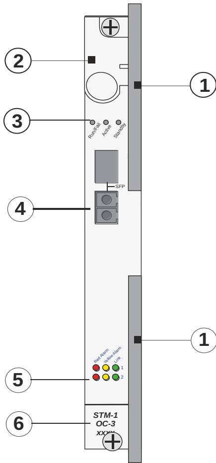
Figure 47. CLC Channelized Line Card
