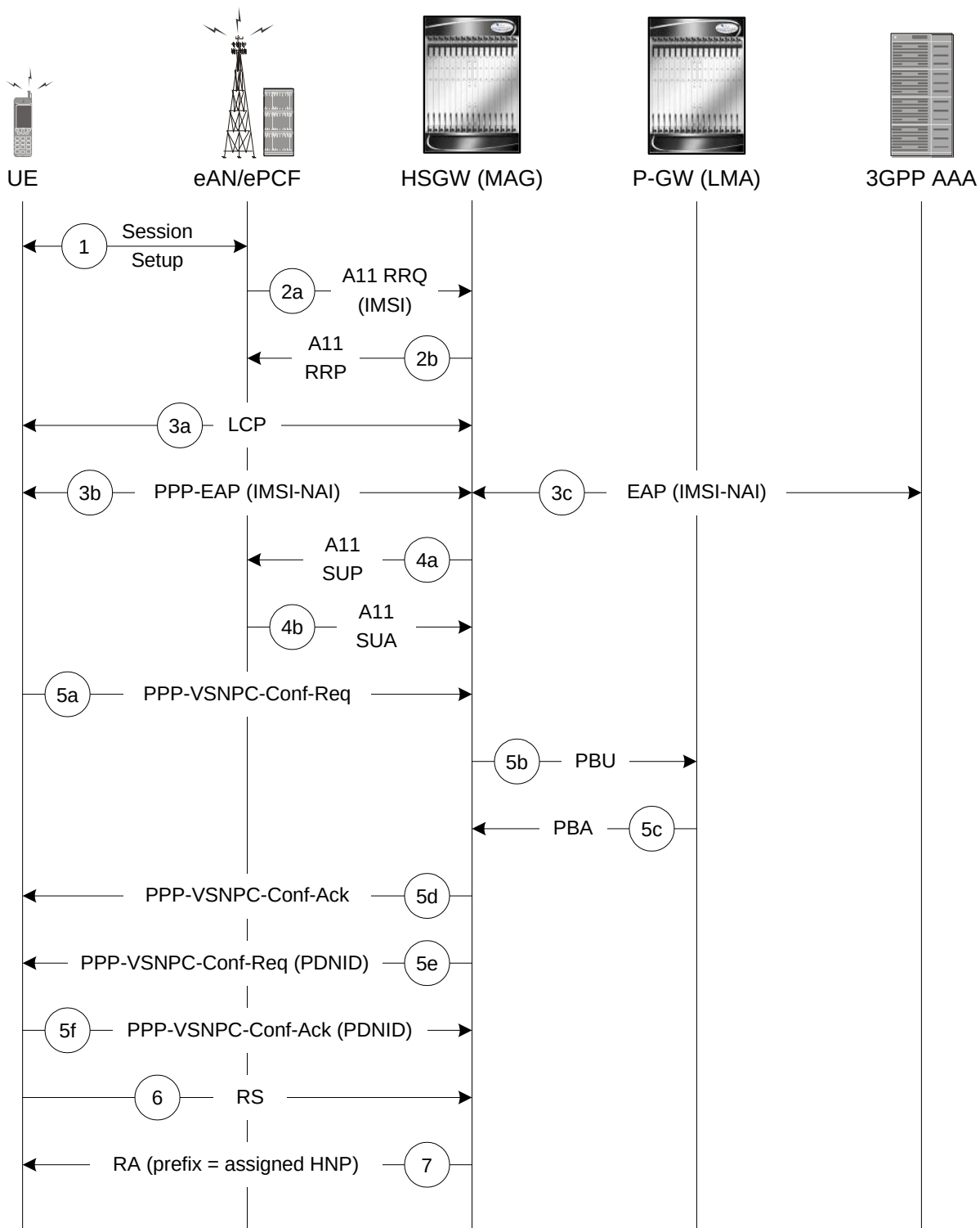
Figure 128. Initial Attach with IPv6/IPv4 Access Call Flow
