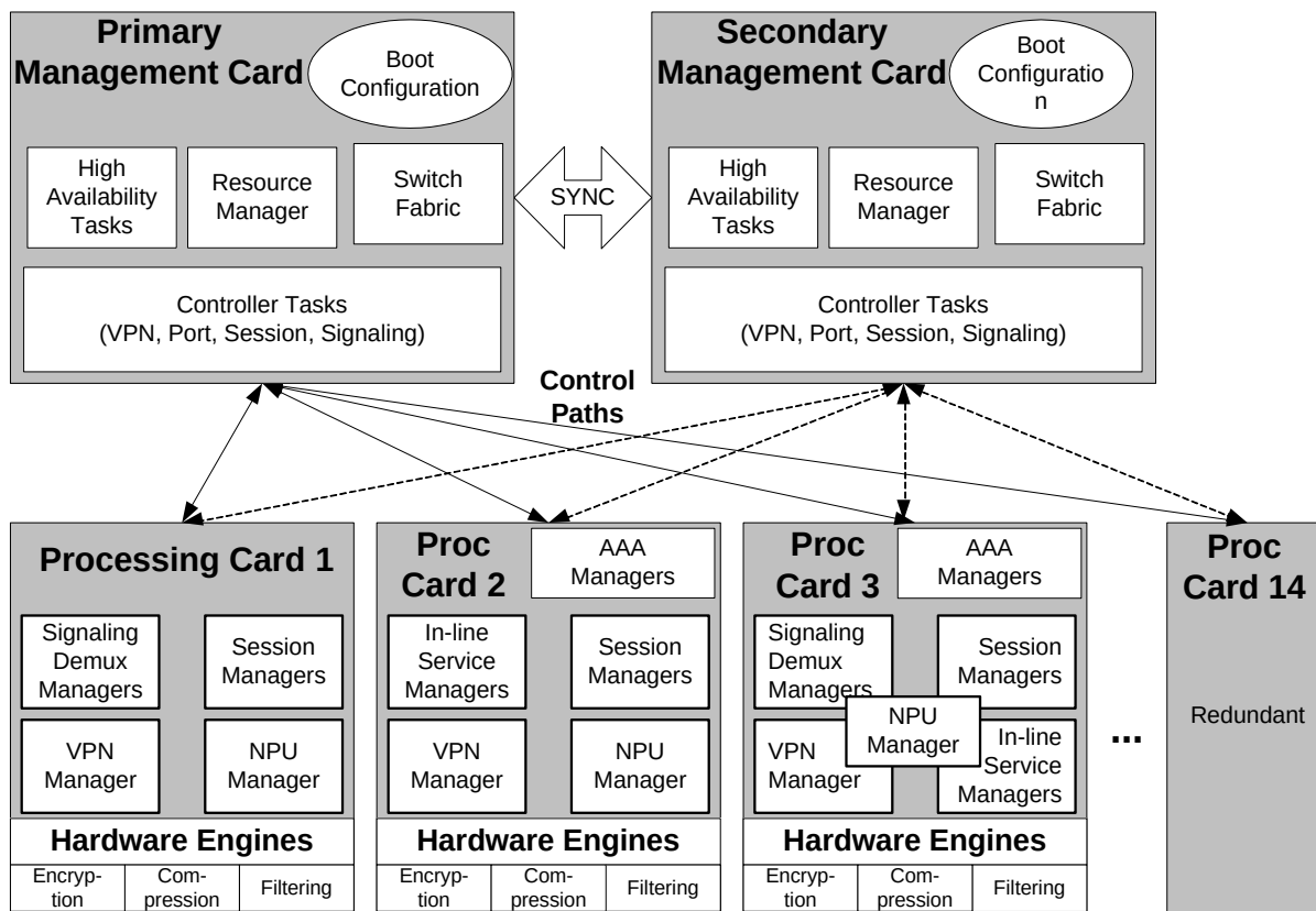
Figure 50. Software Architecture Block Diagram
