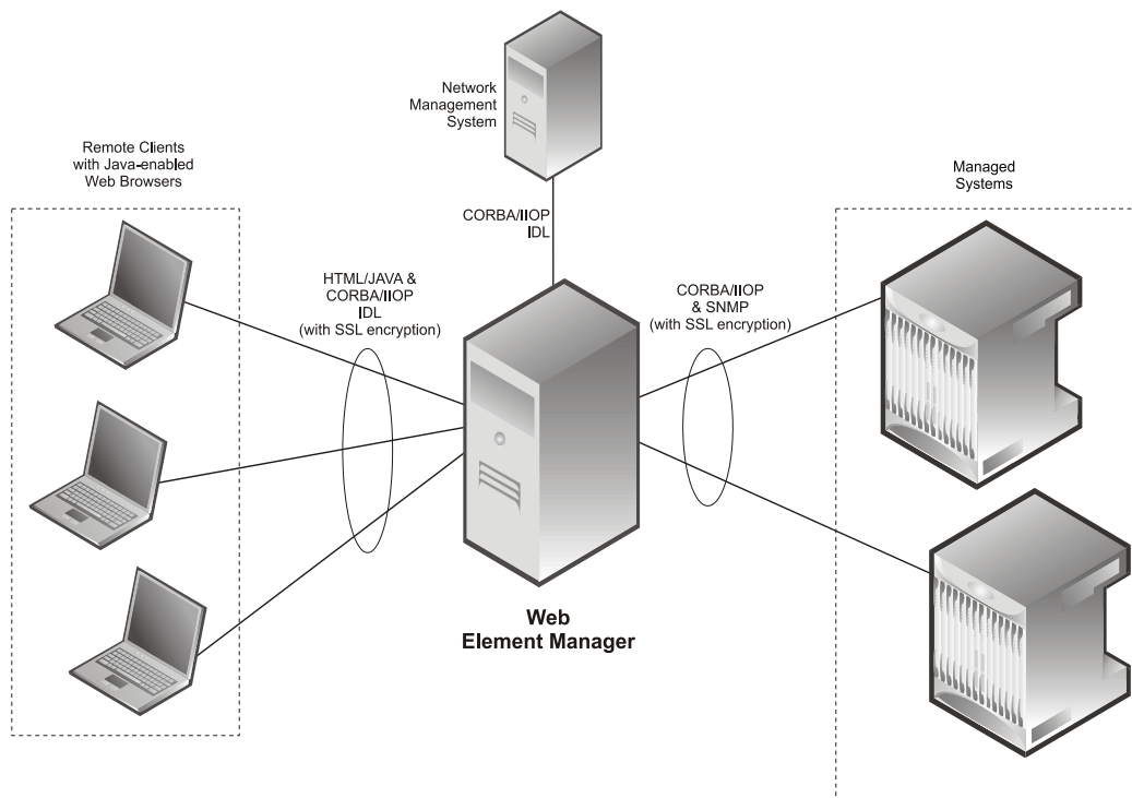
Figure 154. Web Element Manager Network Interfaces
