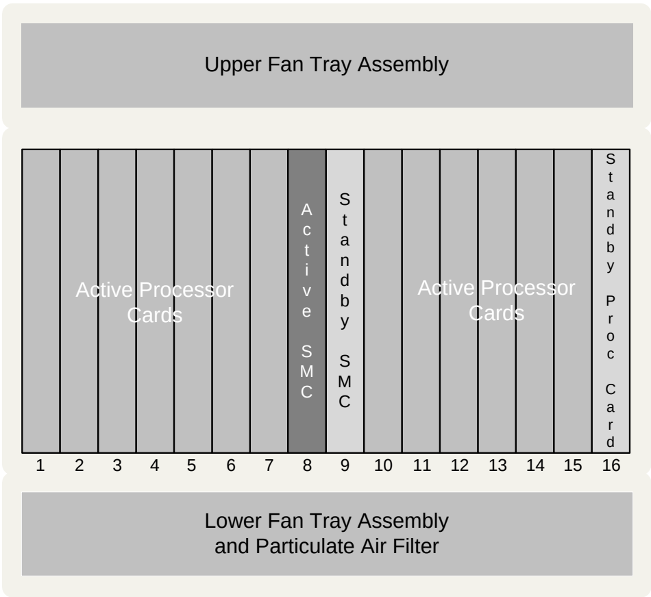
Figure 51. Recommended Redundant Configuration for Data Services - Front View
