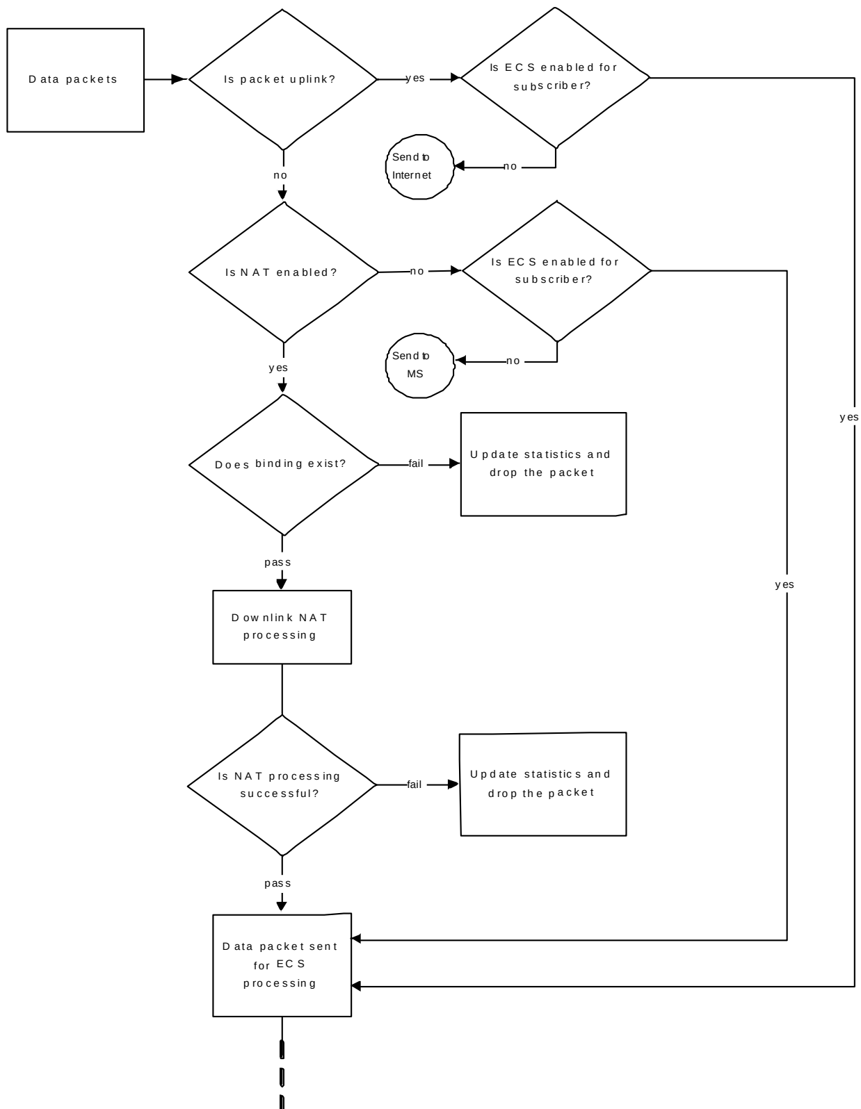
Figure 229. NAT Processing Flow
