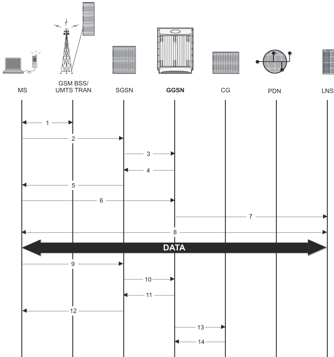
Figure 113. Virtual Dialup Access Call Flow
