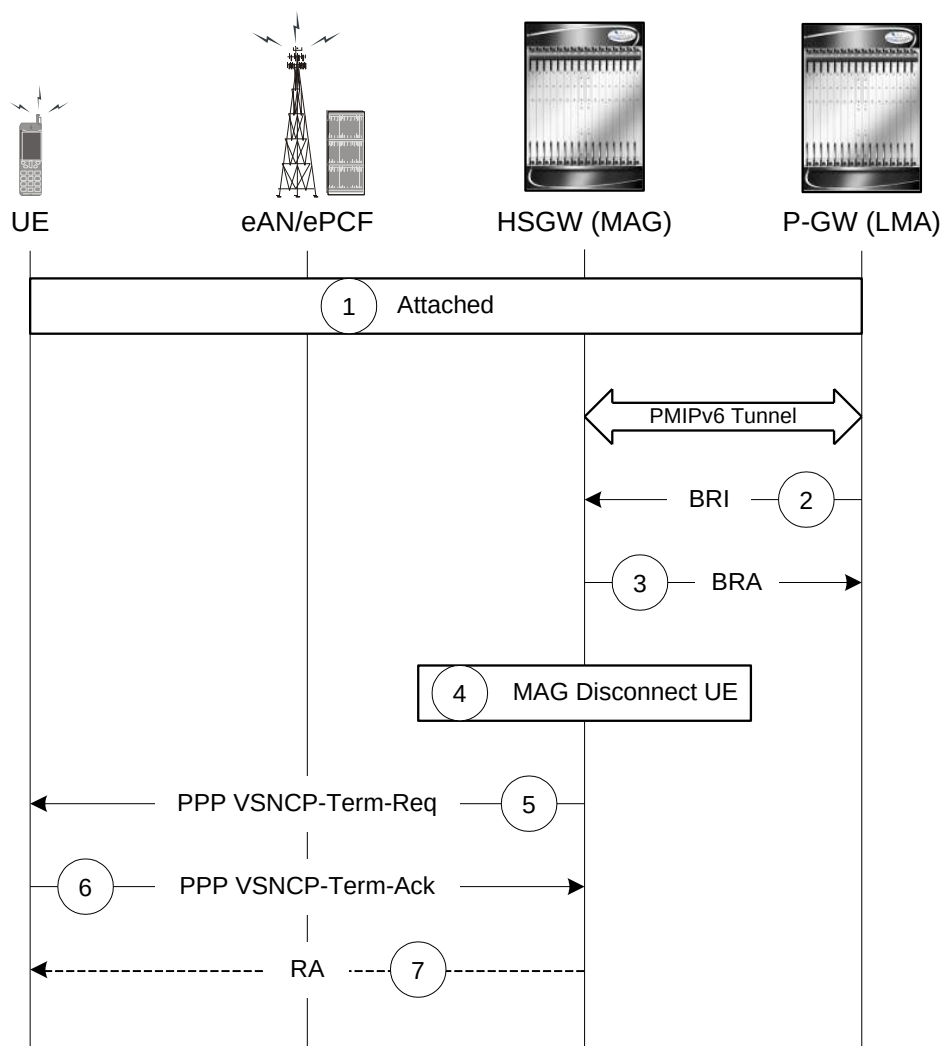
Figure 159. PDN Connection Release by the HSGW Call Flow
