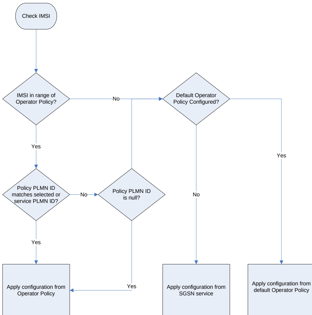
Figure 183. Logic Diagram for Policy Selection
