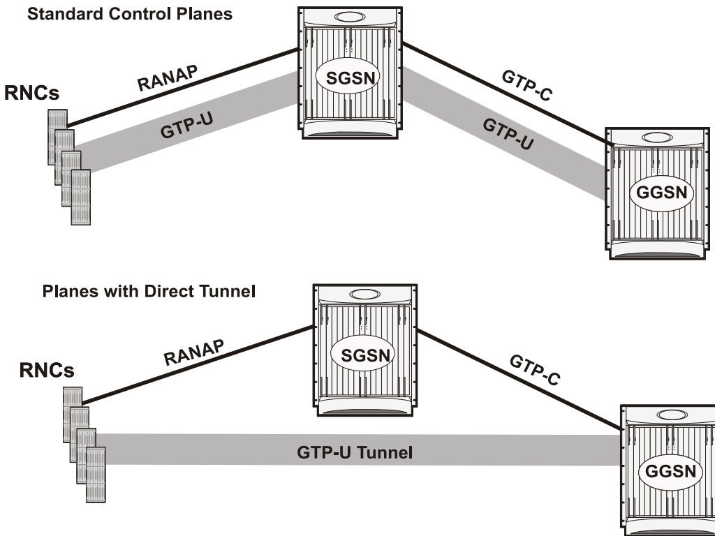
Figure 184. GTP-U with Direct Tunnel
