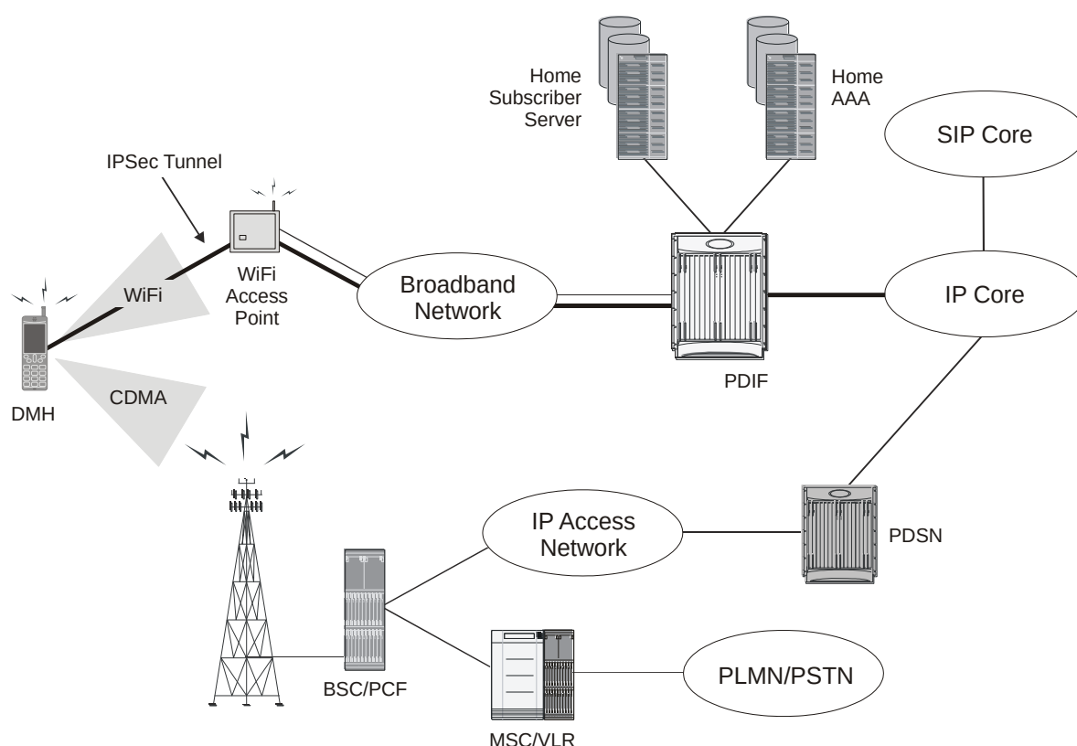
Figure 137. PDIF/FA Mobile IP Interfaces
