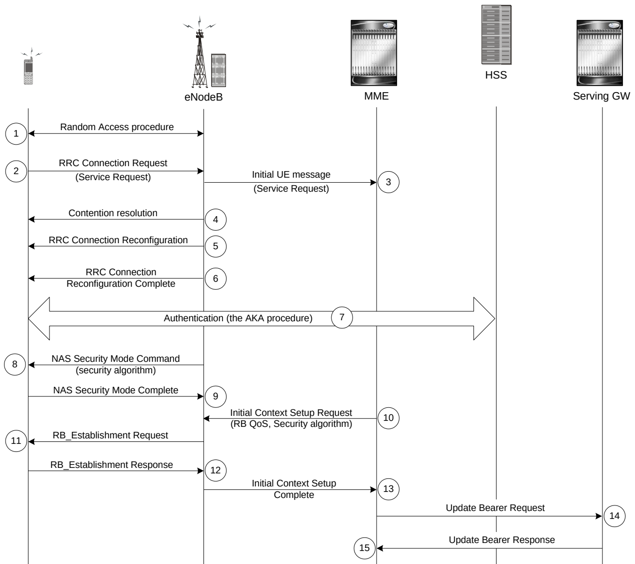
Figure 214. User-initiated Service Request Message Flow
