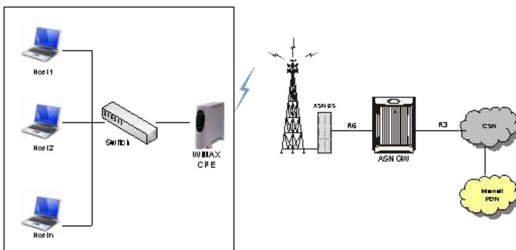
Figure 59. Multi Host Support in WiMAX Network
