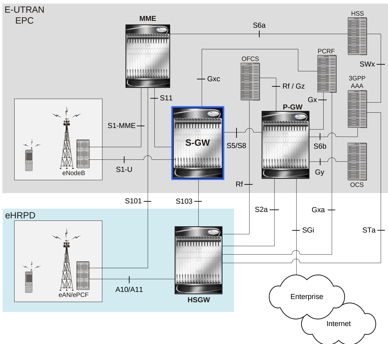
Figure 171. Basic E-UTRAN/EPC and eHRPD Network Topology
