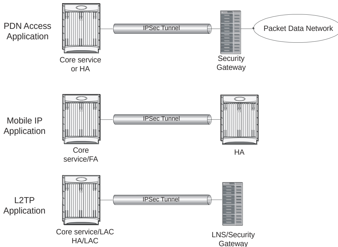
Figure 210. IPSec Applications
