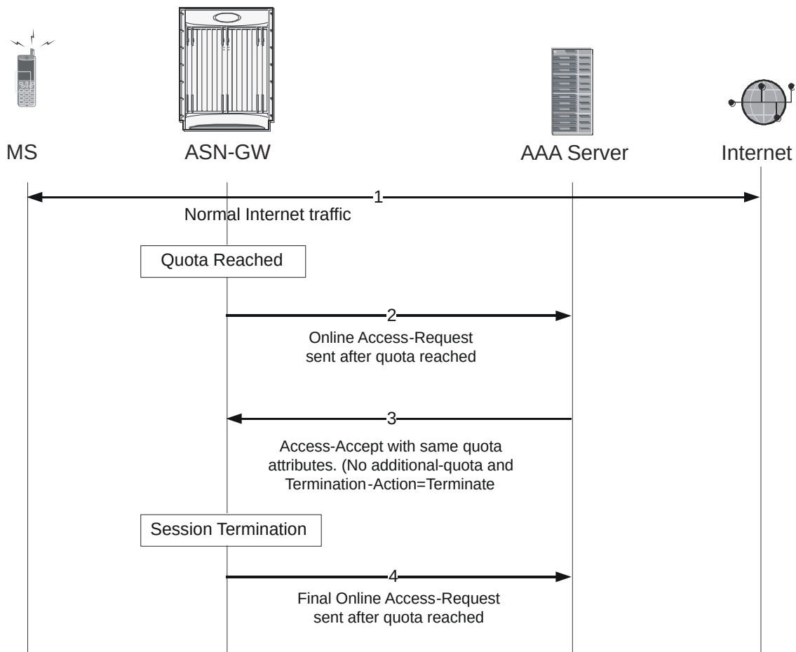
Figure 81. Call Flow for Terminating the Call on Quota-Reach
