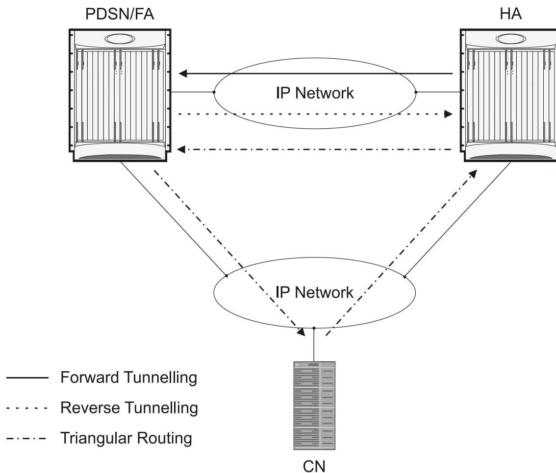
Figure 120. Mobile IP, FA and HA Tunneling/Transport Methods.
