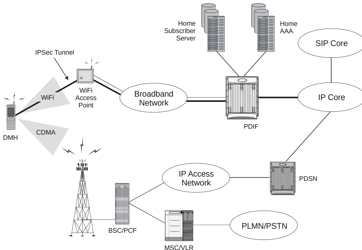
Figure 140. PDIF Simple IP Implementation
