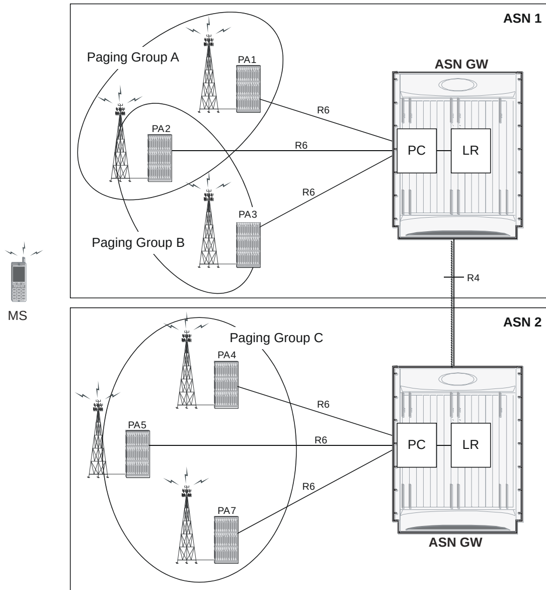
Figure 86. ASN Paging Controller and Location Registry in WiMAX Networks
