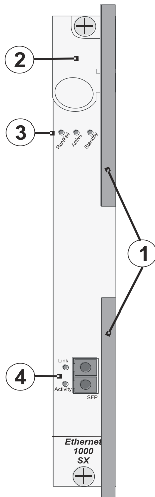
Figure 42. Ethernet 1000 Line Card
