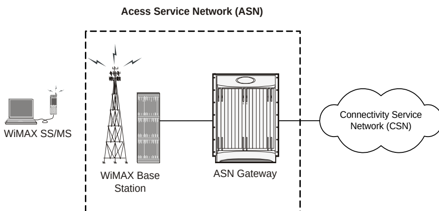
Figure 56. Basic ASN Gateway Network
