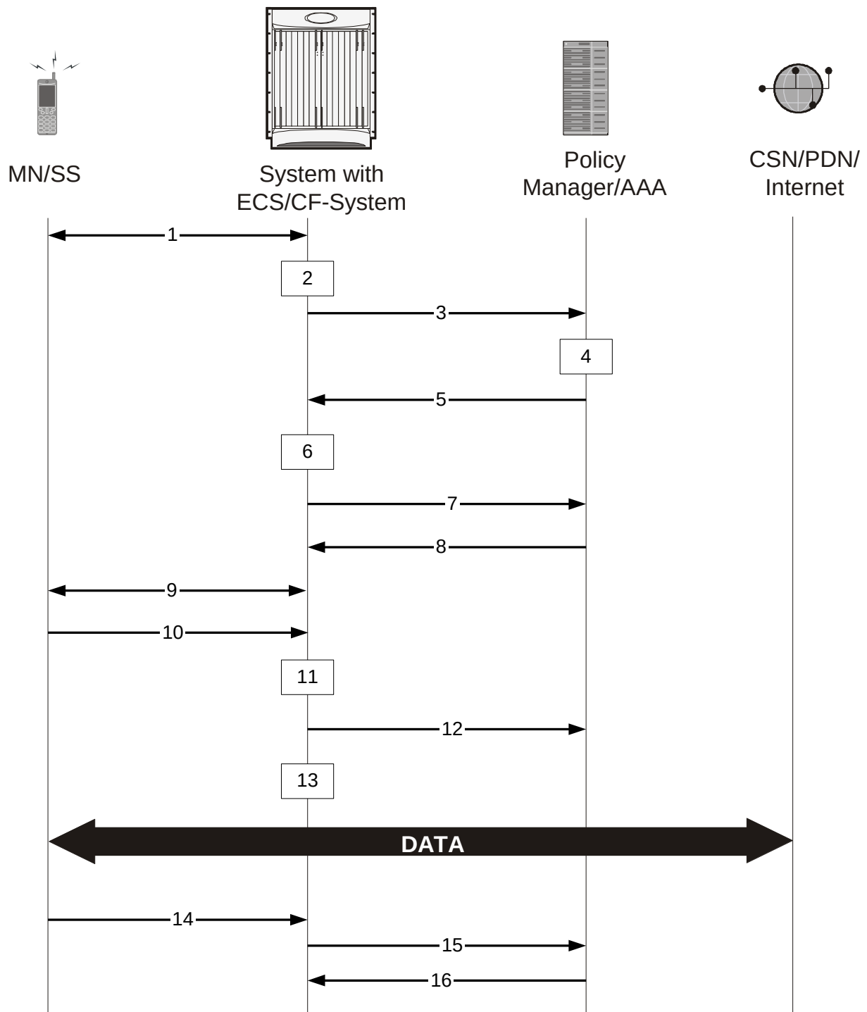
Figure 192. Content Filtering Call Flow
