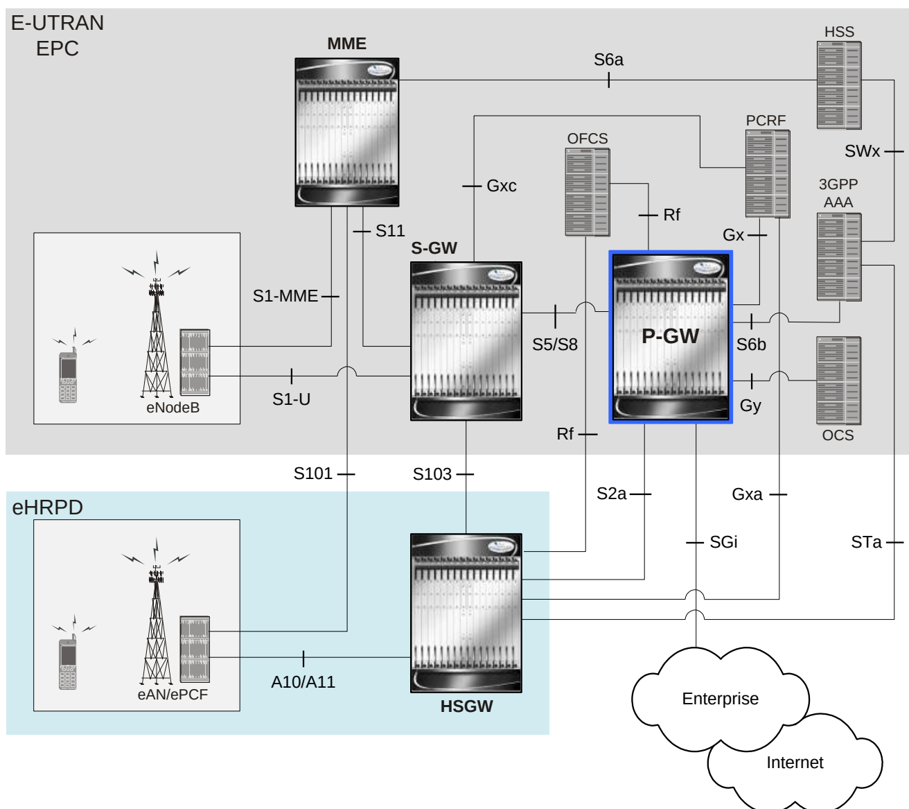
Figure 148. Basic E-UTRAN/EPC and eHRPD Network Topology
