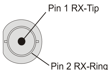
Figure 242. SPIO BITS BNC Timing Interface Pin-out
