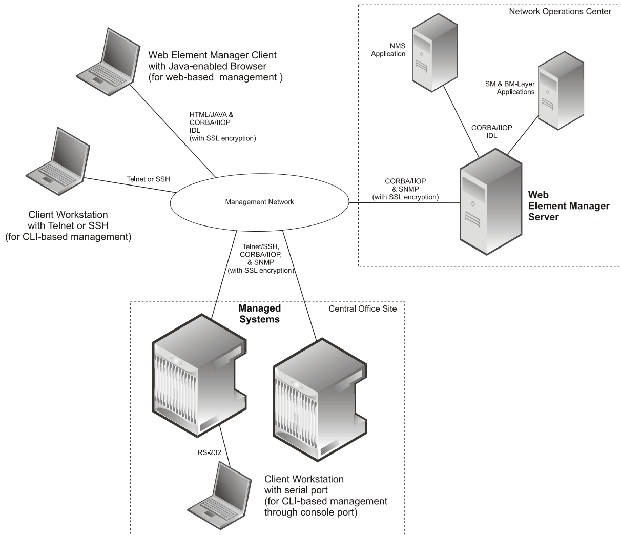
Figure 153. Element Management Methods
