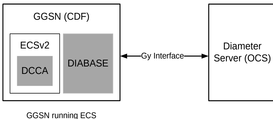
Figure 200. Logical Online Charging with Gy Interface
