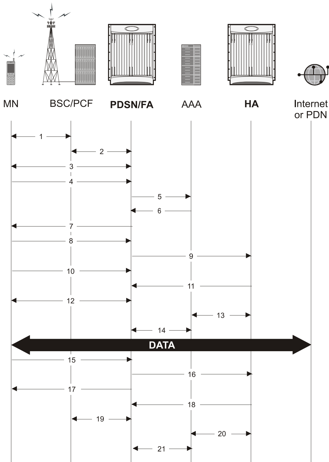
Figure 98. AAA/PDSN Assigned IP Address Proxy Mobile IP Call Flow
