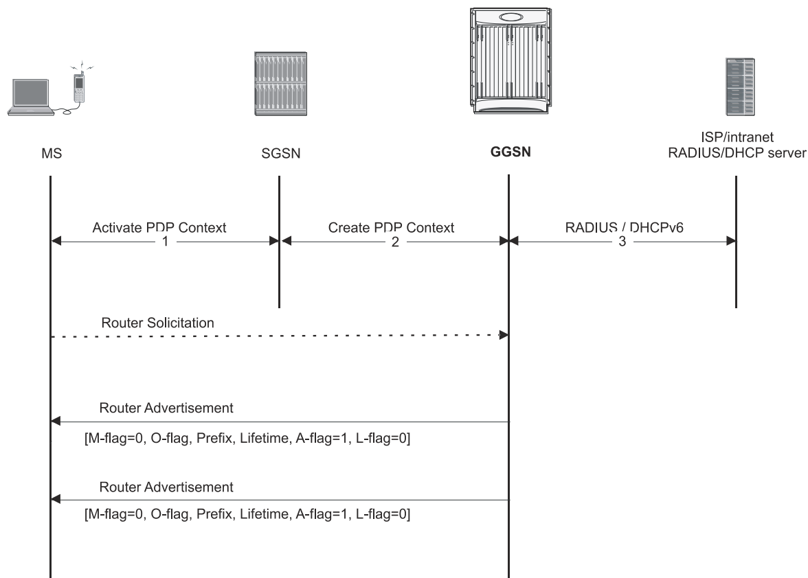
Figure 117. IPv6 Stateless Address Autoconfiguration Flow
