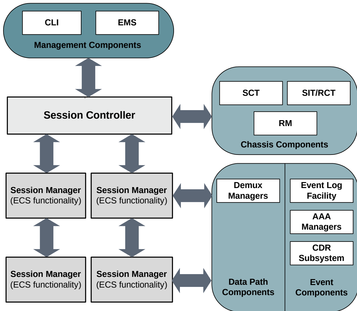
Figure 194. ECS Architecture
