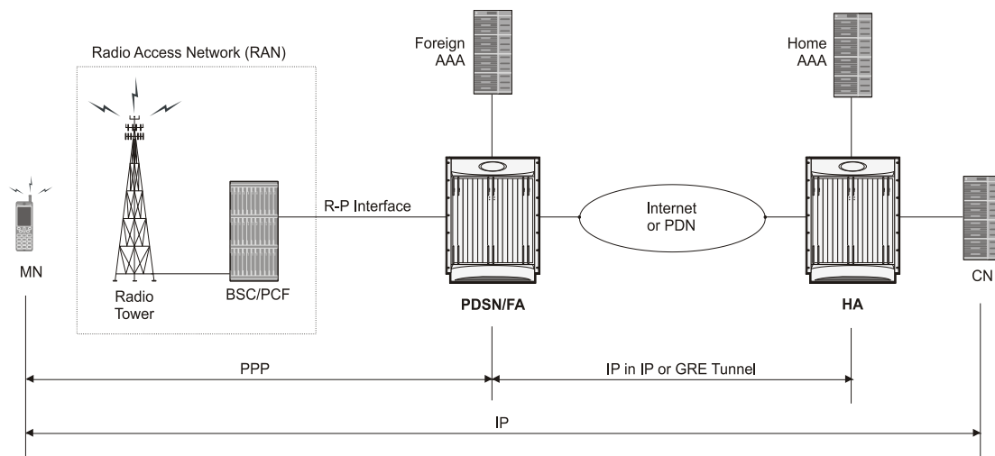
Figure 121. Mobile IP Protocol Usage.
