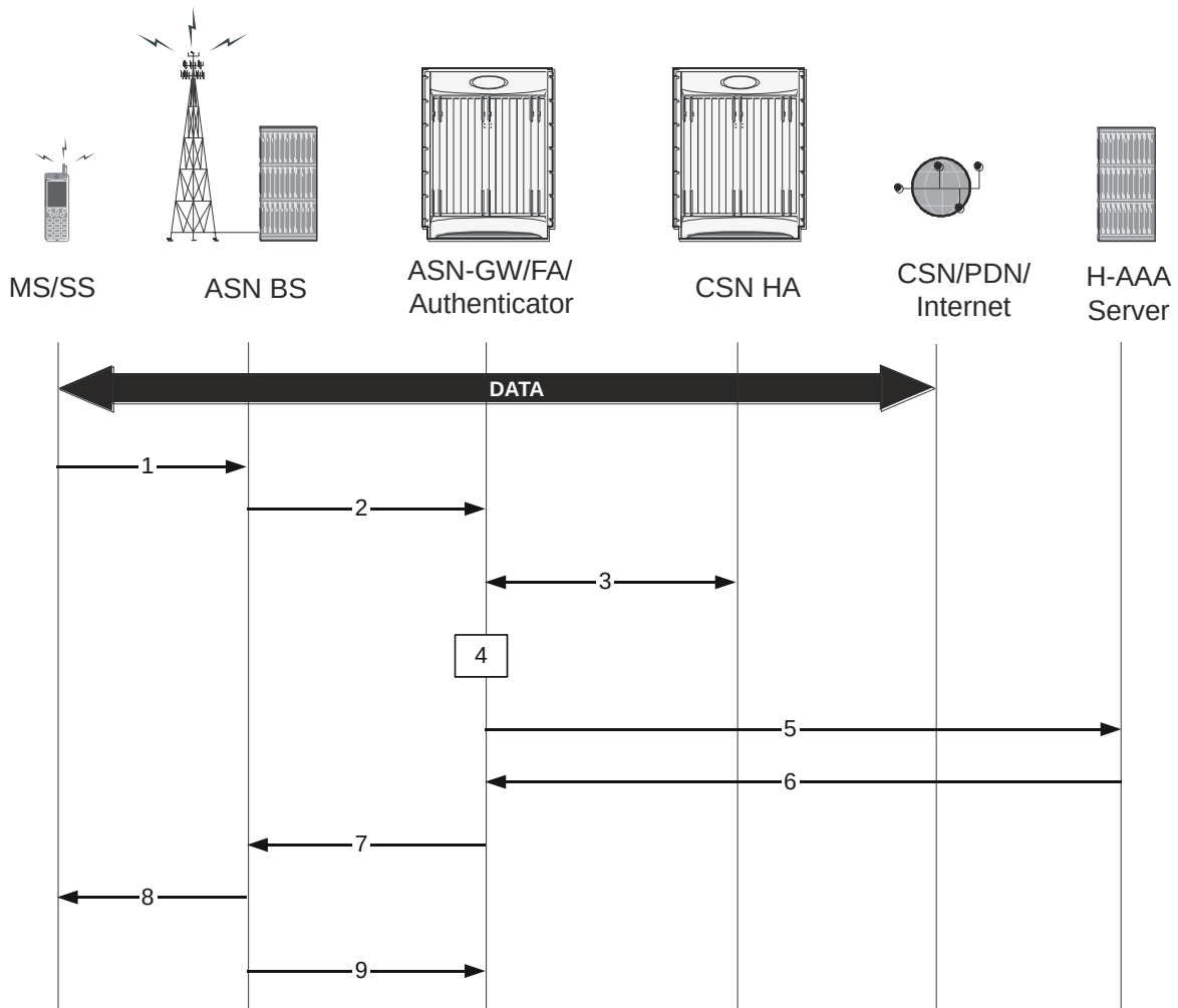
Figure 67. MS Triggered Network Exit Call Flow
