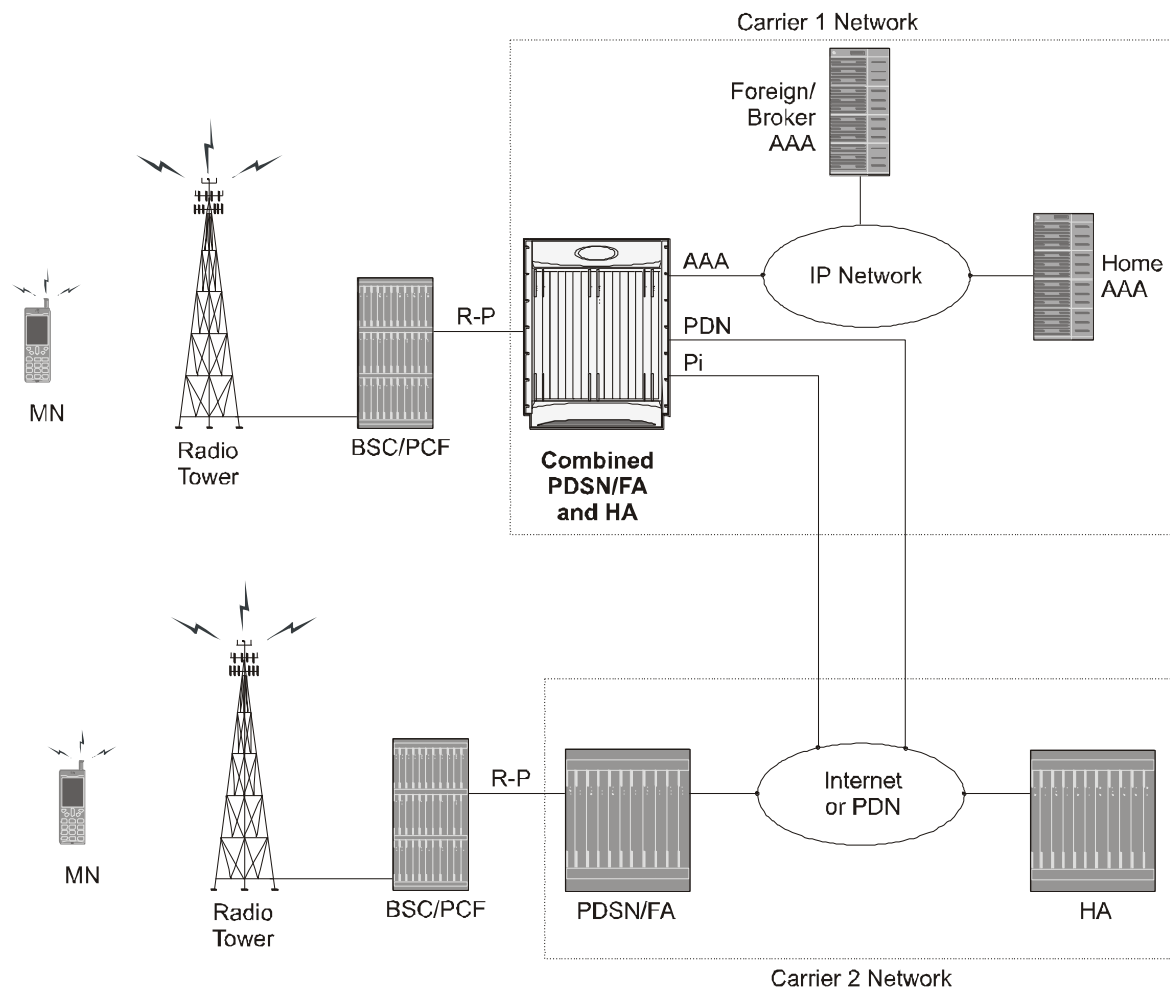
Figure 92. Co-located PDSN/FA and HA Configuration Example
