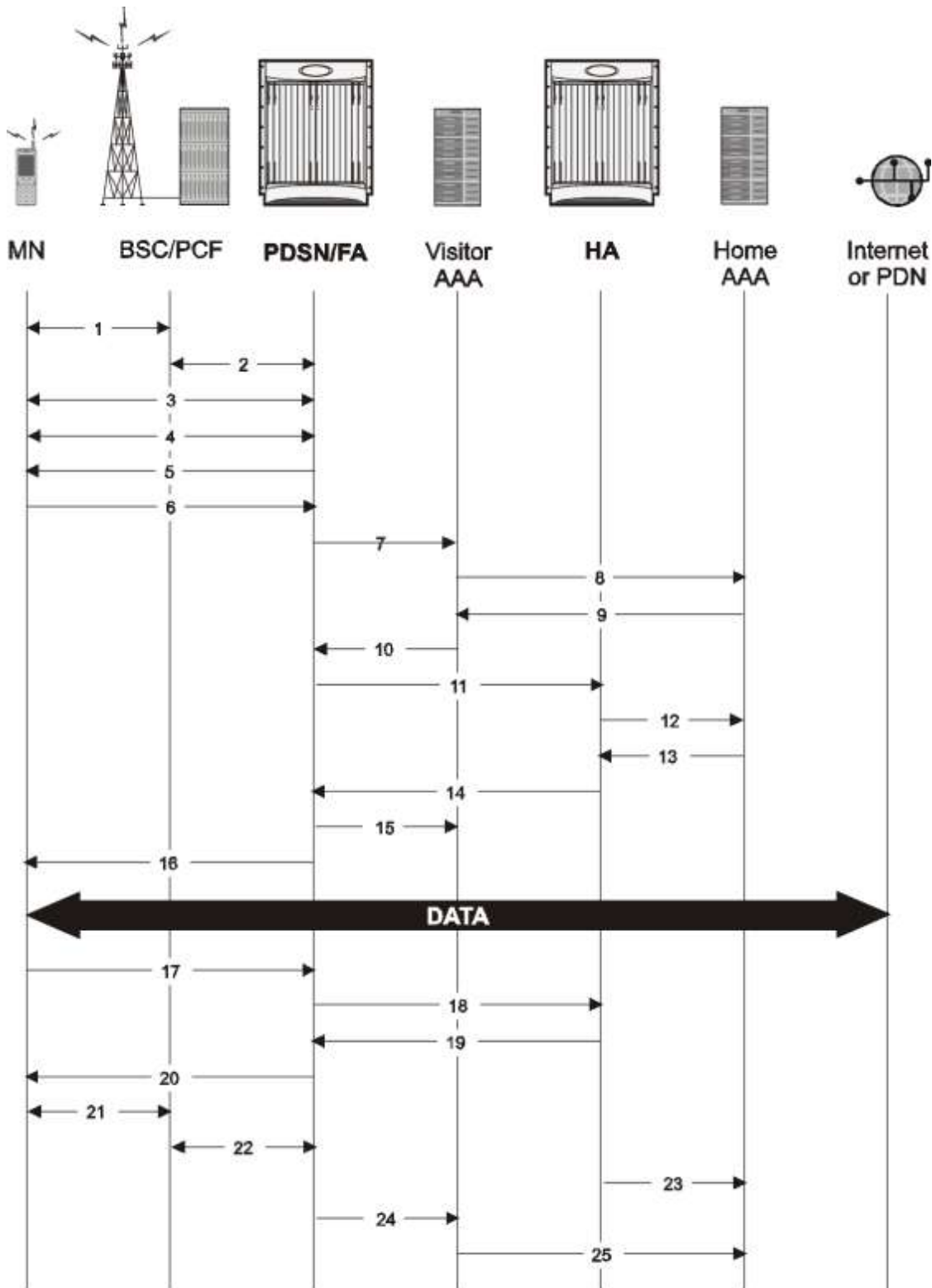
Figure 97. Mobile IP Call Flow
