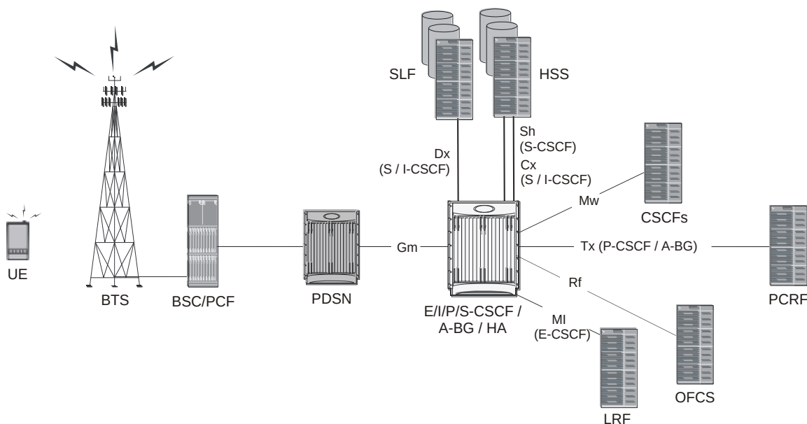
Figure 165. CDMA2000 CSCF/A-BG/HA SCM Deployment Example
