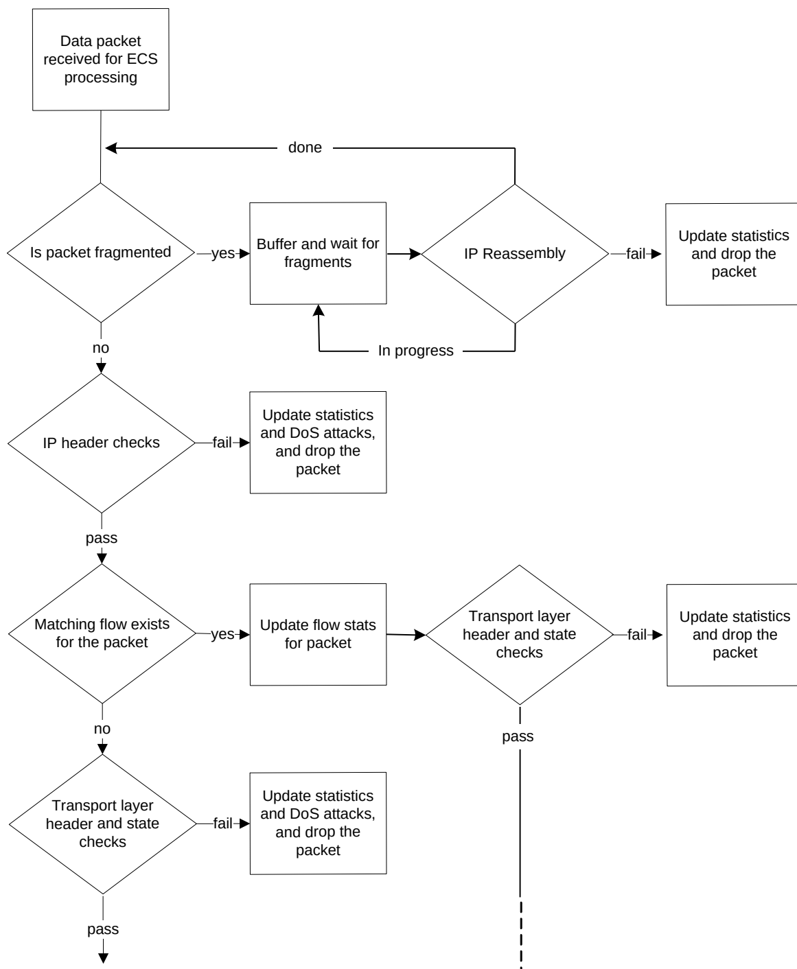
Figure 217. Stateful Firewall Processing
