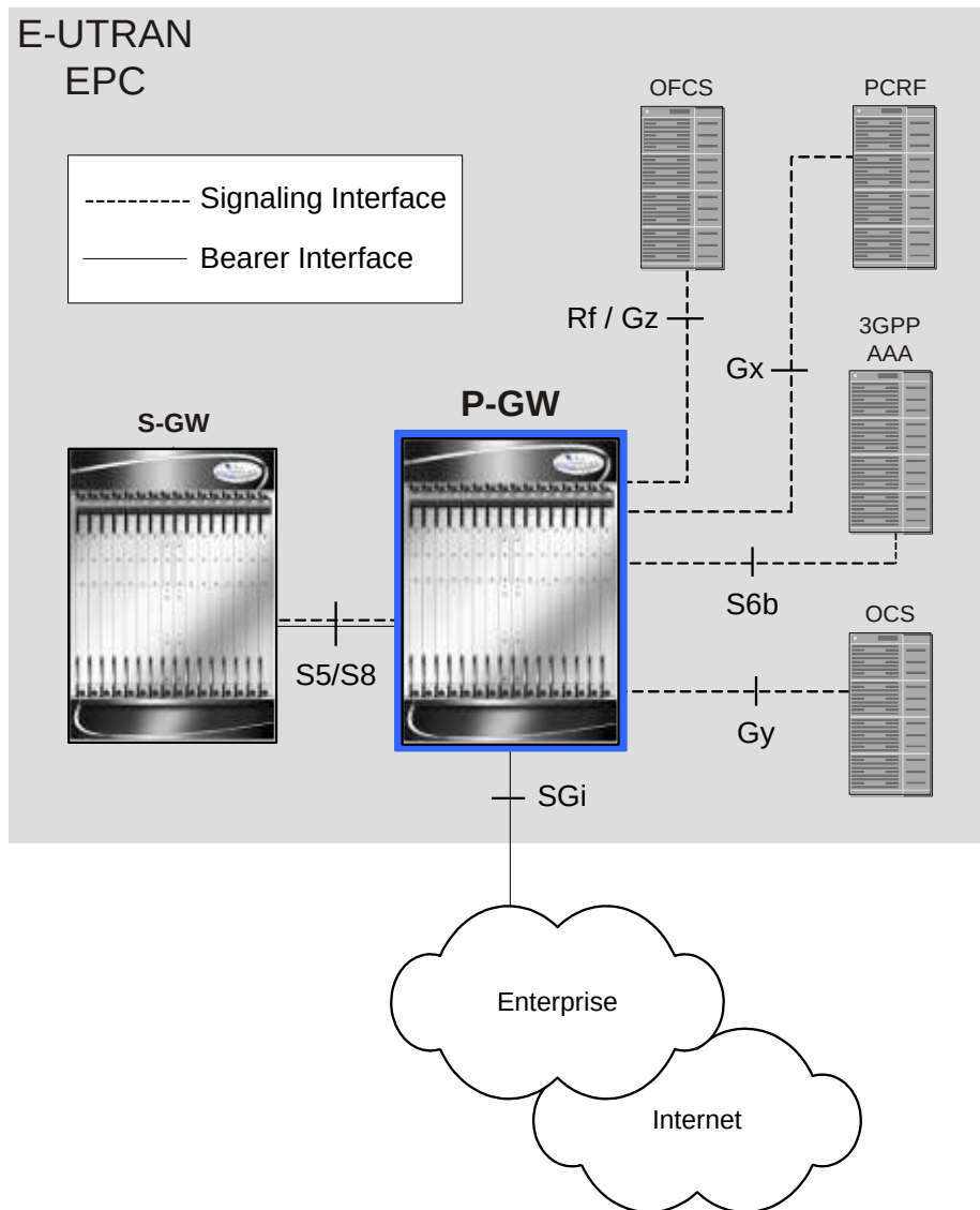
Figure 152. P-GW Interfaces in the E-UTRAN/EPC Network
