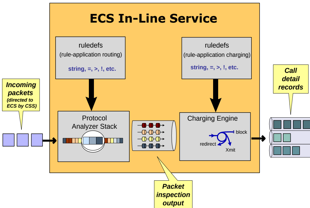
Figure 196. ECS In-line Service Processing
