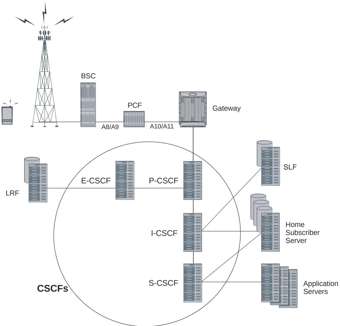
Figure 163. IMS CSCF Components
