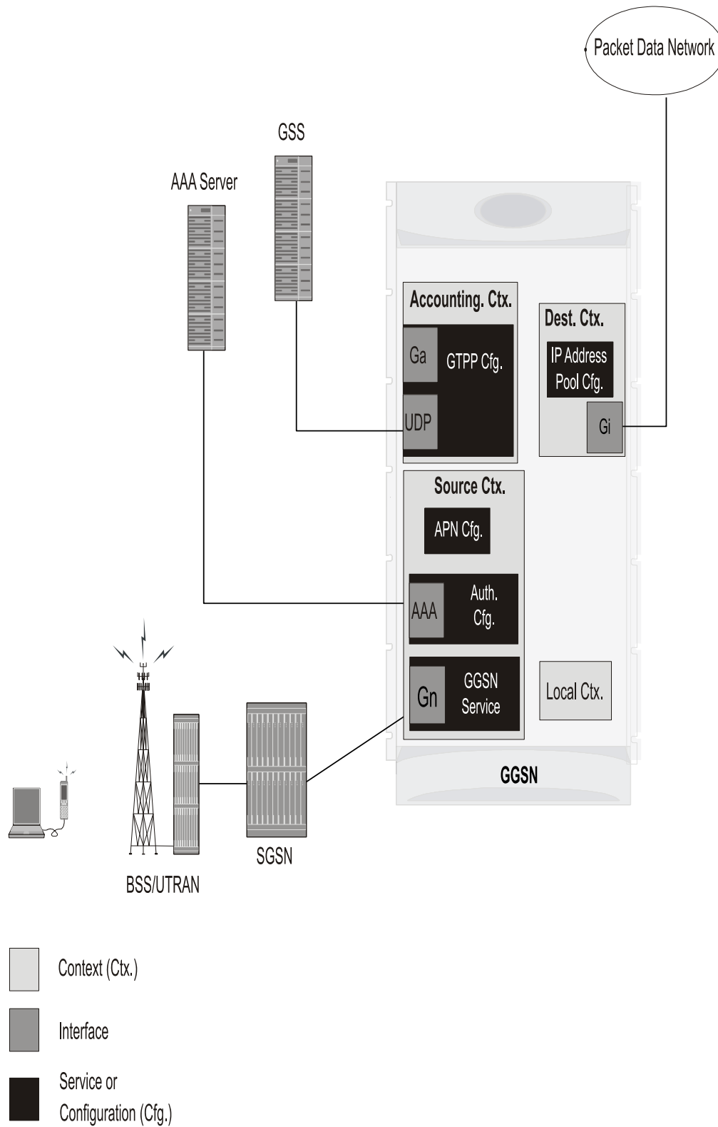
Figure 222. GGSN Contexts and Interfaces
