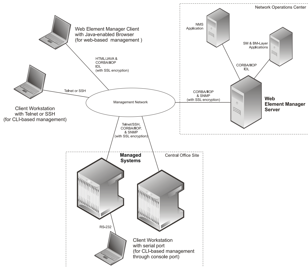
Figure 53. Element Management Methods
