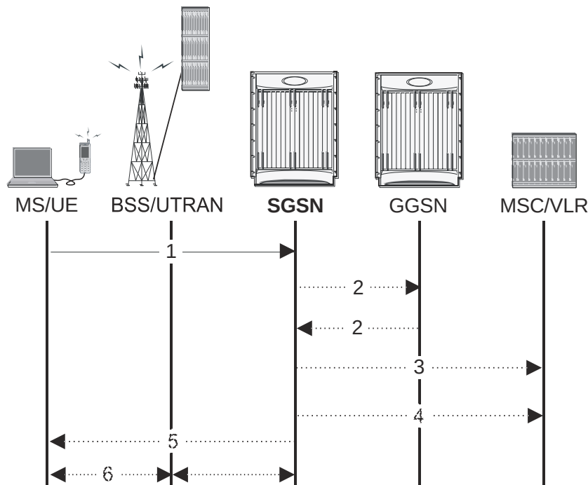
Figure 189. MS-Initiated Combined GPRS/IMS Detach
