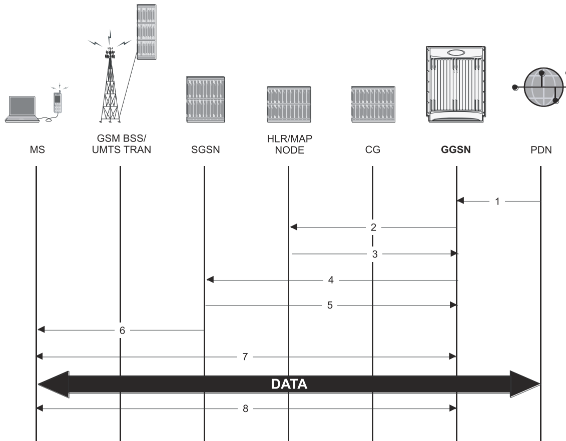
Figure 111. Network-initiated Session Call Flow
