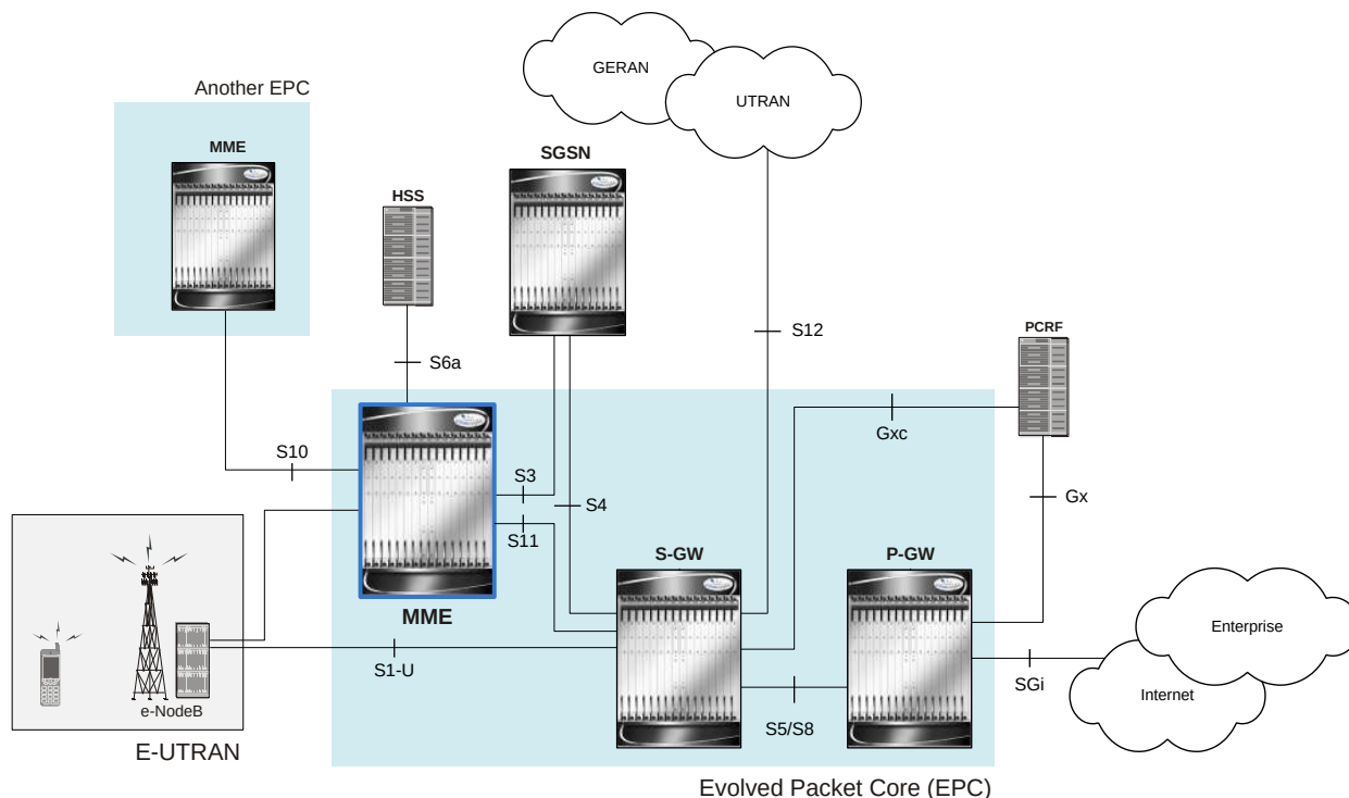
Figure 206. Architecture of LTE/SAE Network
