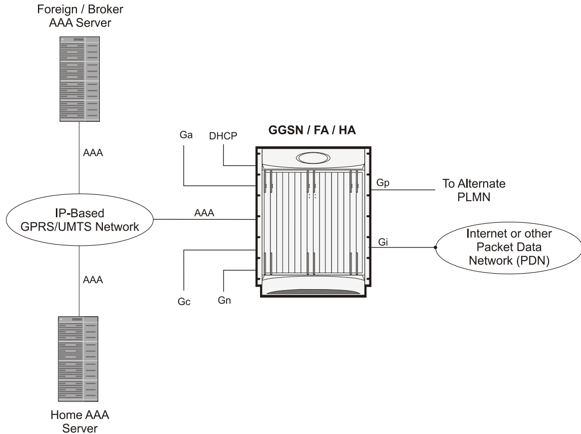
Figure 103. Combined GGSN/FA/HA Deployment for Mobile IP and/or Proxy Mobile IP Support
