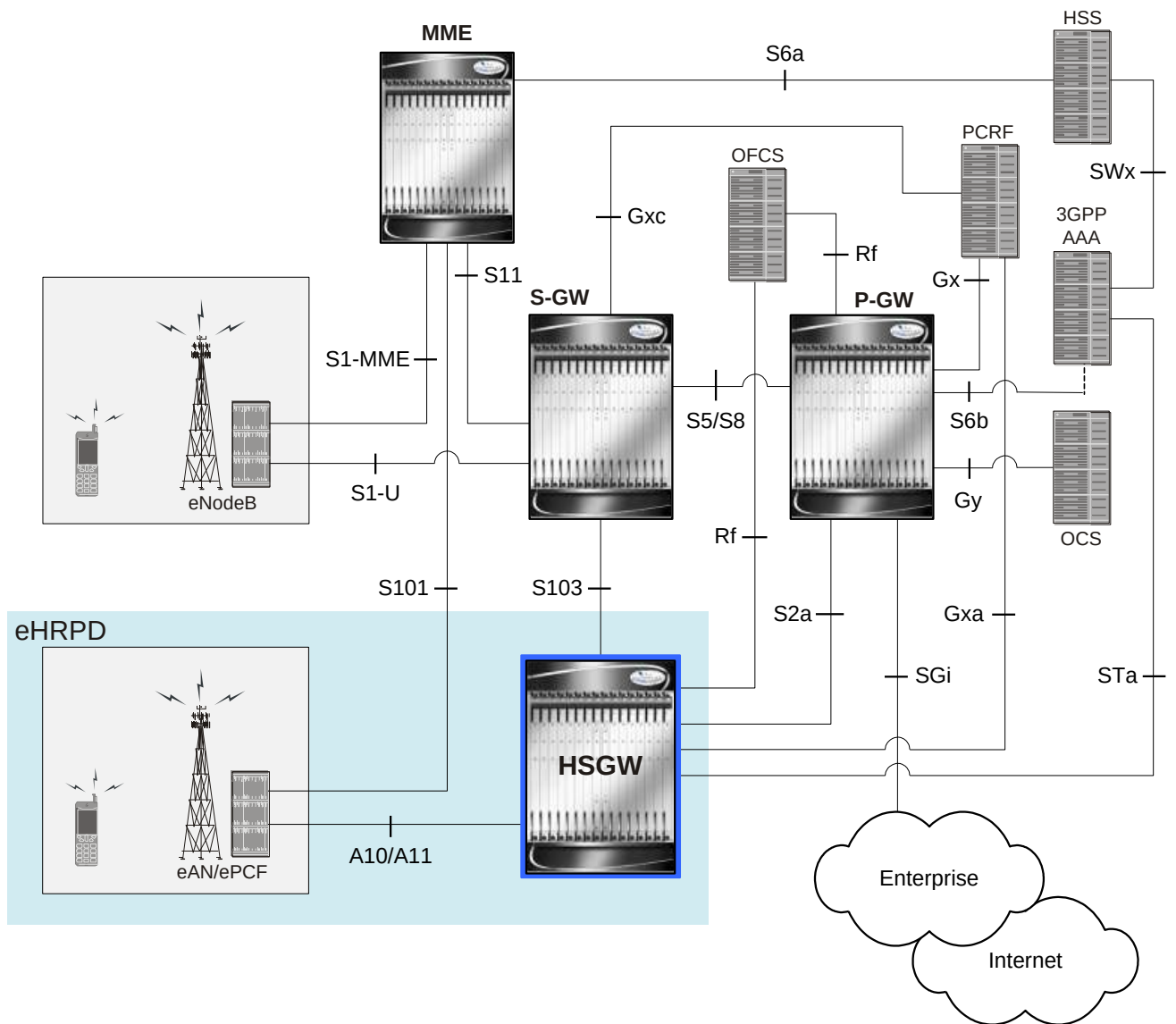
Figure 123. eHRPD Basic Network Topology
