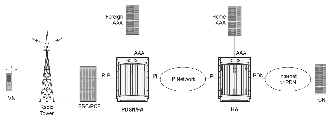
Figure 118. PDSN/FA and HA Network Deployment Configuration Example
