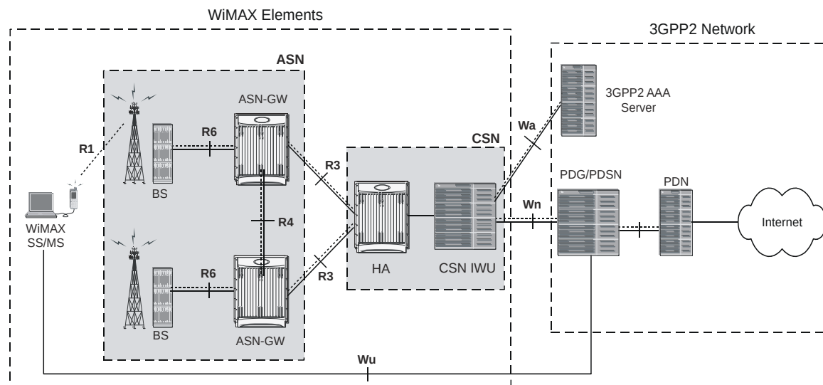
Figure 85. ASN Gateway with 3GPP2 Overlay
