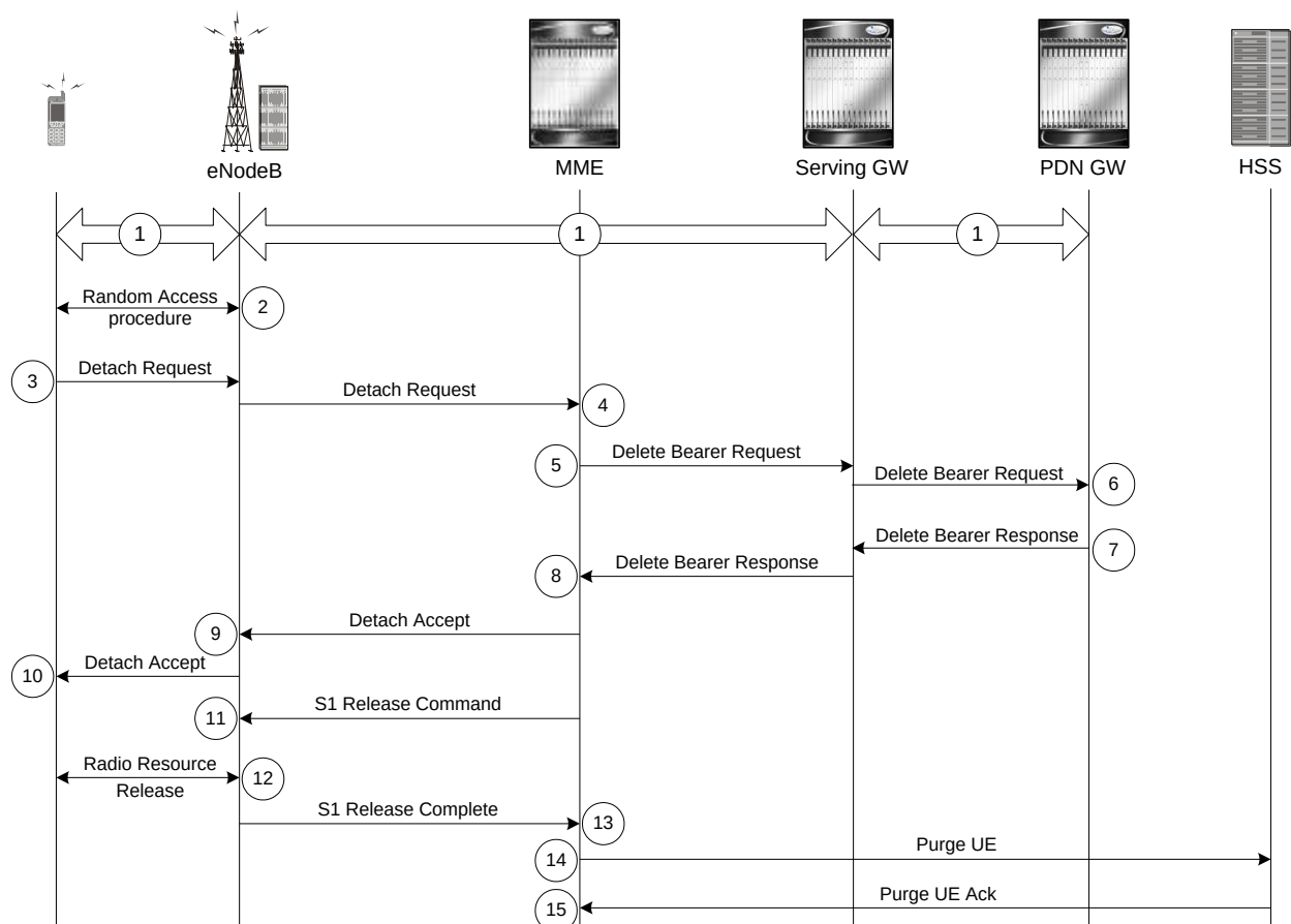
Figure 213. Subscriber De-registration Setup Message Flow
