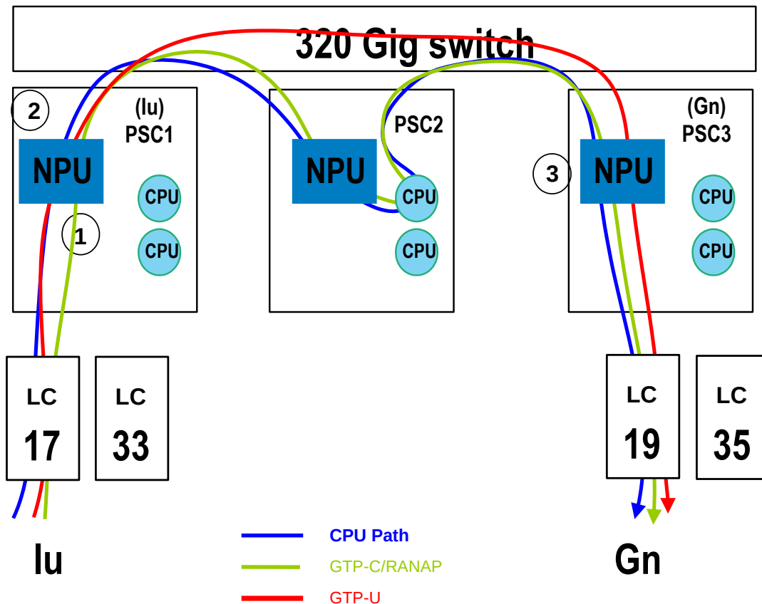
Figure 182. SGSN NPU FastPath
