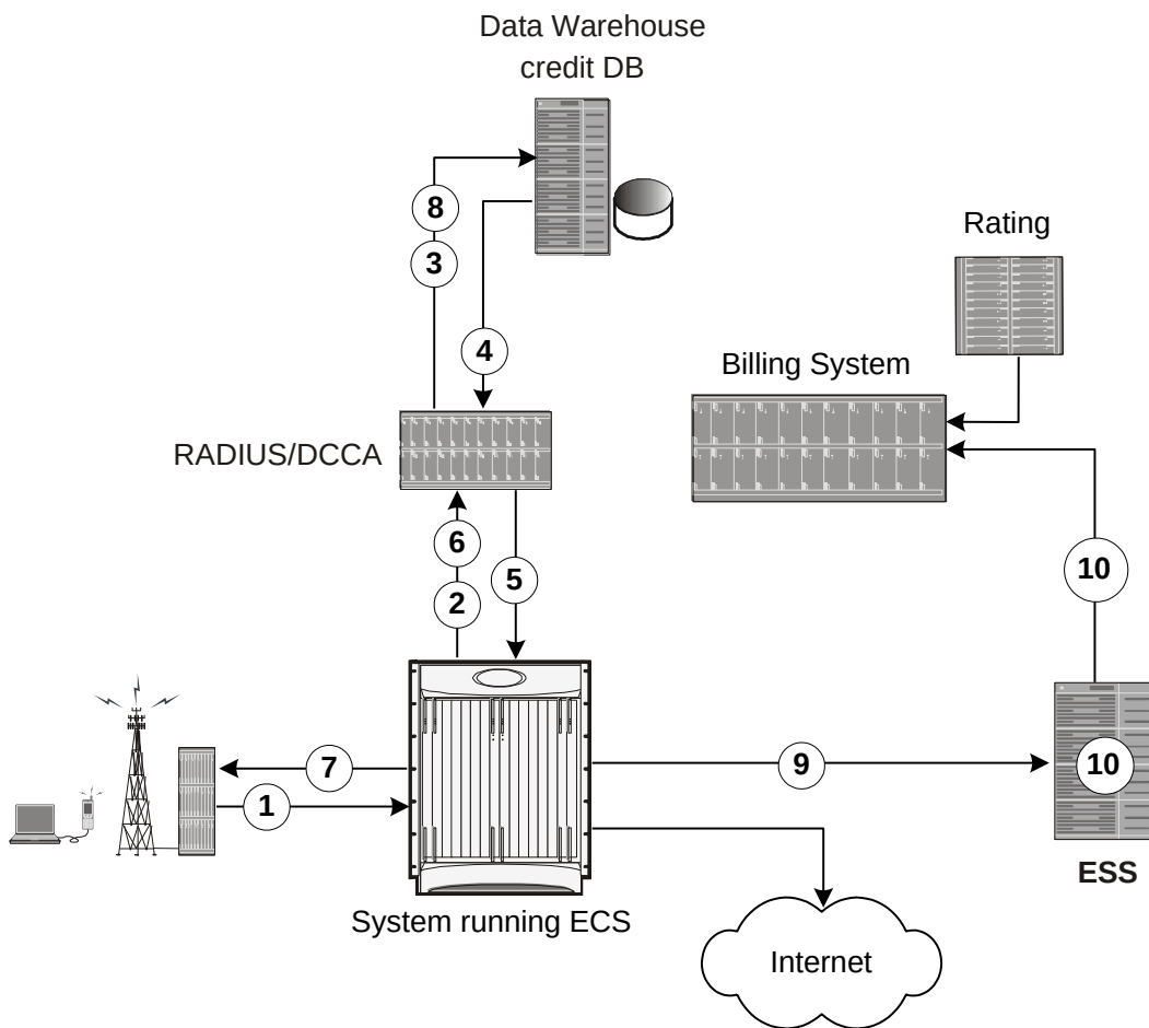
Figure 202. Prepaid Charging in GPRS/UMTS/CDMA-2000 Networks
