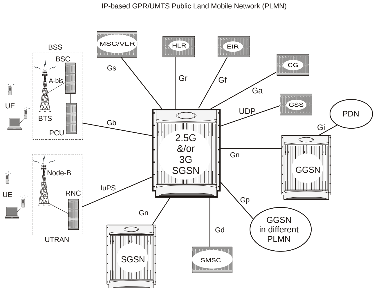
Figure 178. Dual Access 2.5G/3G SGSNs
