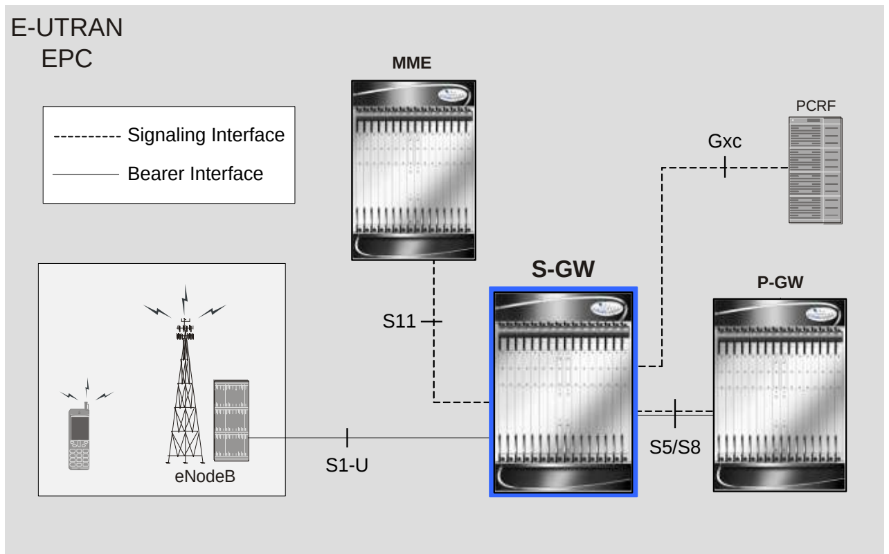
Figure 173. S-GW Interfaces in the E-UTRAN/EPC Network
