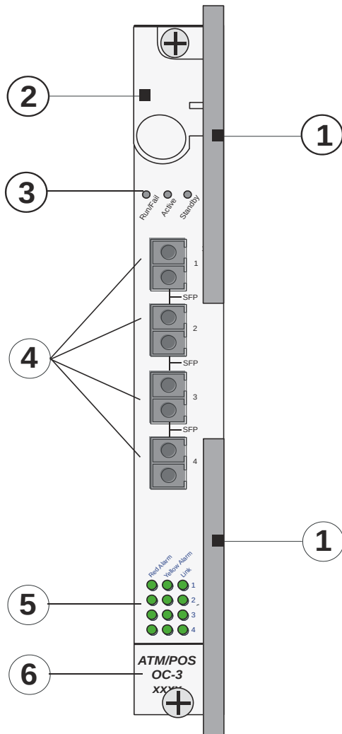
Figure 45. OLC Optical (ATM) Line Card
