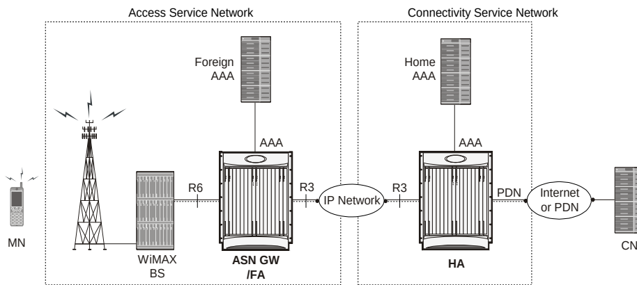
Figure 63. ASN Gateway/FA and HA Network Deployment Configuration Example
