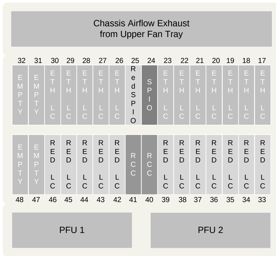
Figure 52. Recommended Redundant Configuration for Data Services - Rear View
