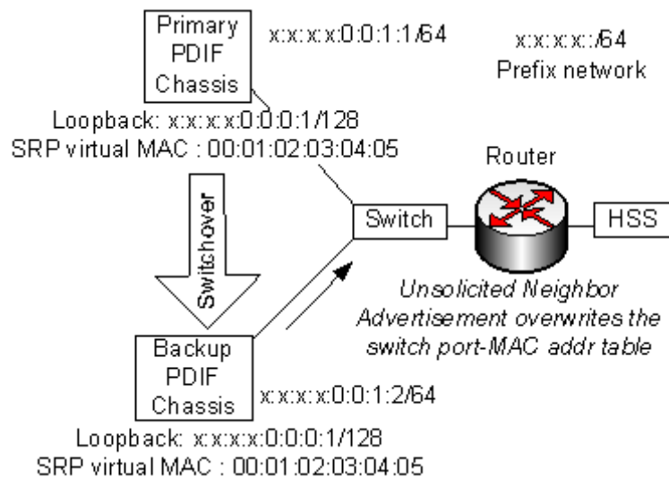
Figure 146. Switchover Example for a Common IPv6 Subnet
