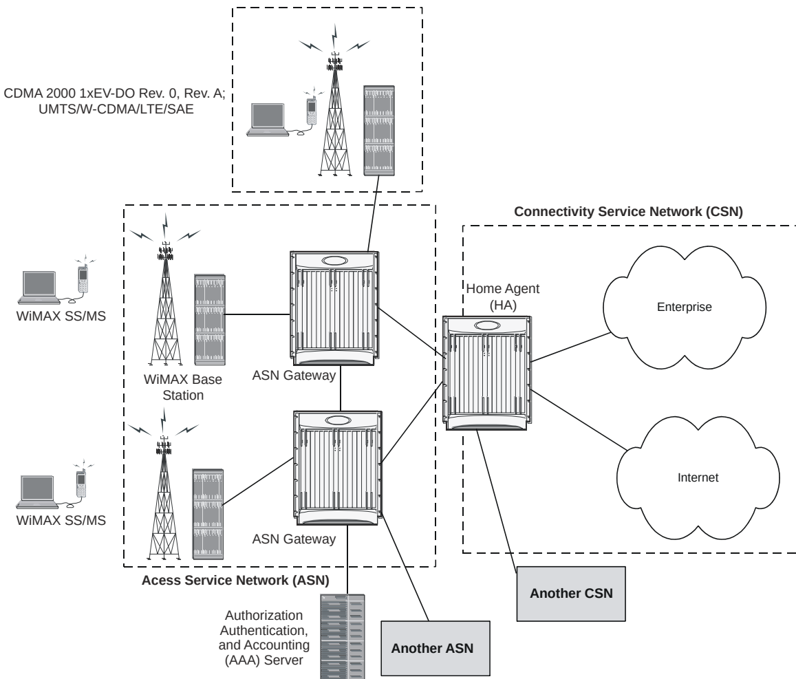
Figure 60. WiMAX Network Architecture
