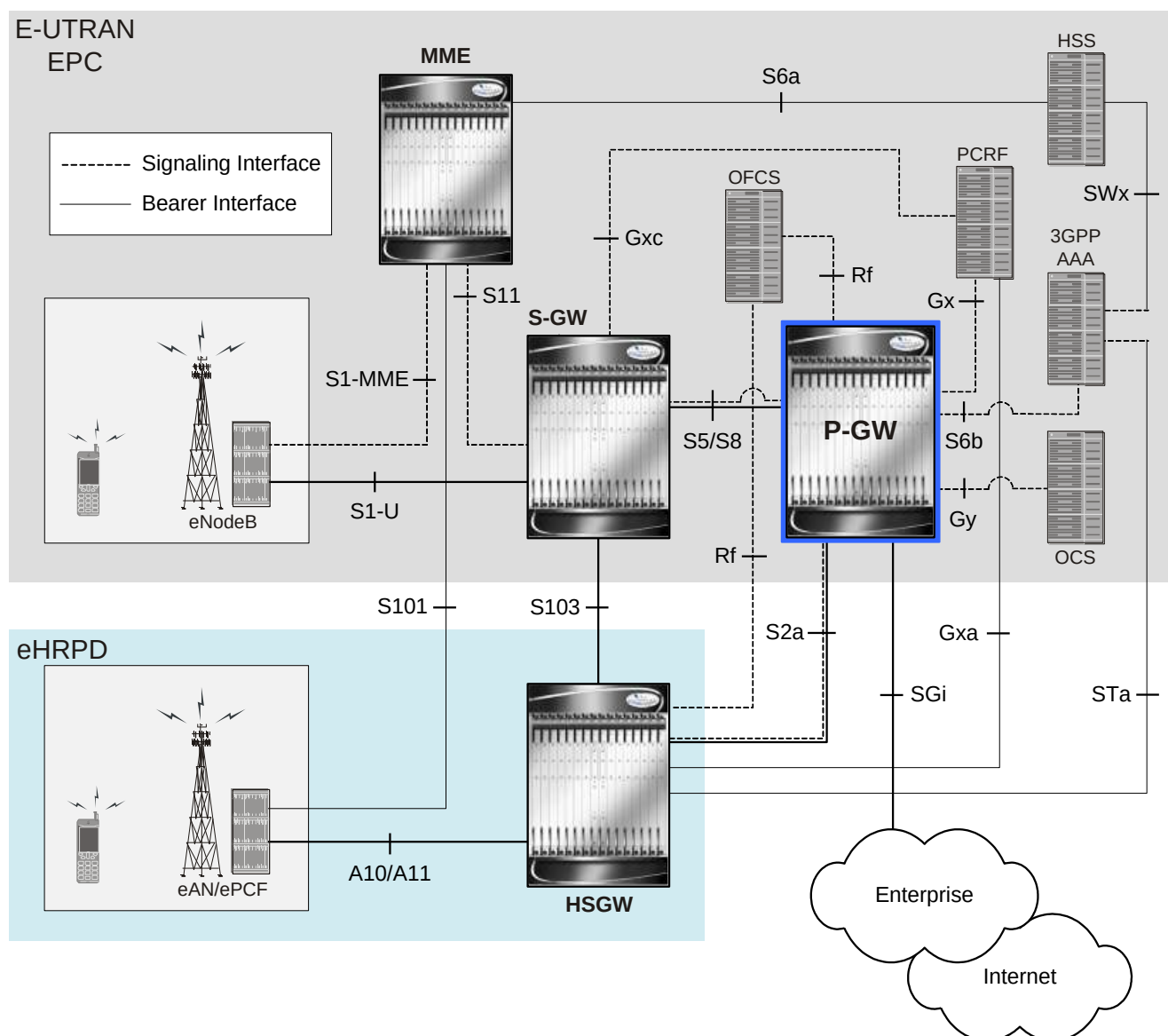
Figure 149. P-GW in the E-UTRAN/EPC Network Supporting the eHRPD Network
