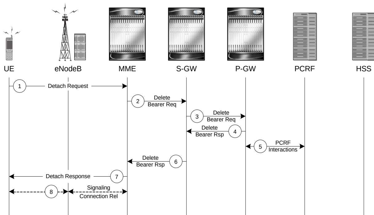
Figure 177. Subscriber-initiated Detach Call Flow
