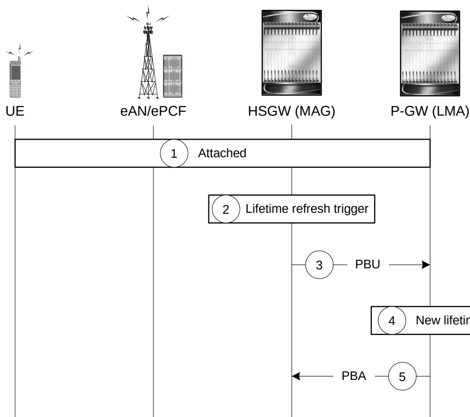
Figure 156. PMIPv6 Lifetime Extension (without handover) Call Flow
