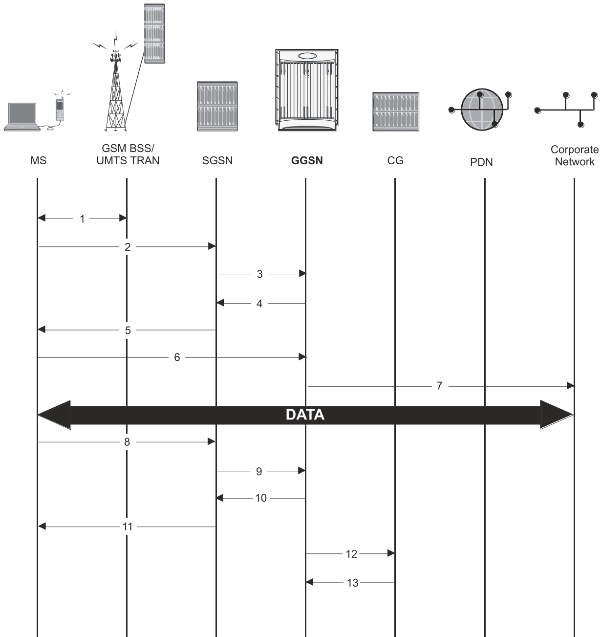
Figure 114. Corporate IP VPN Connectivity Call Flow
