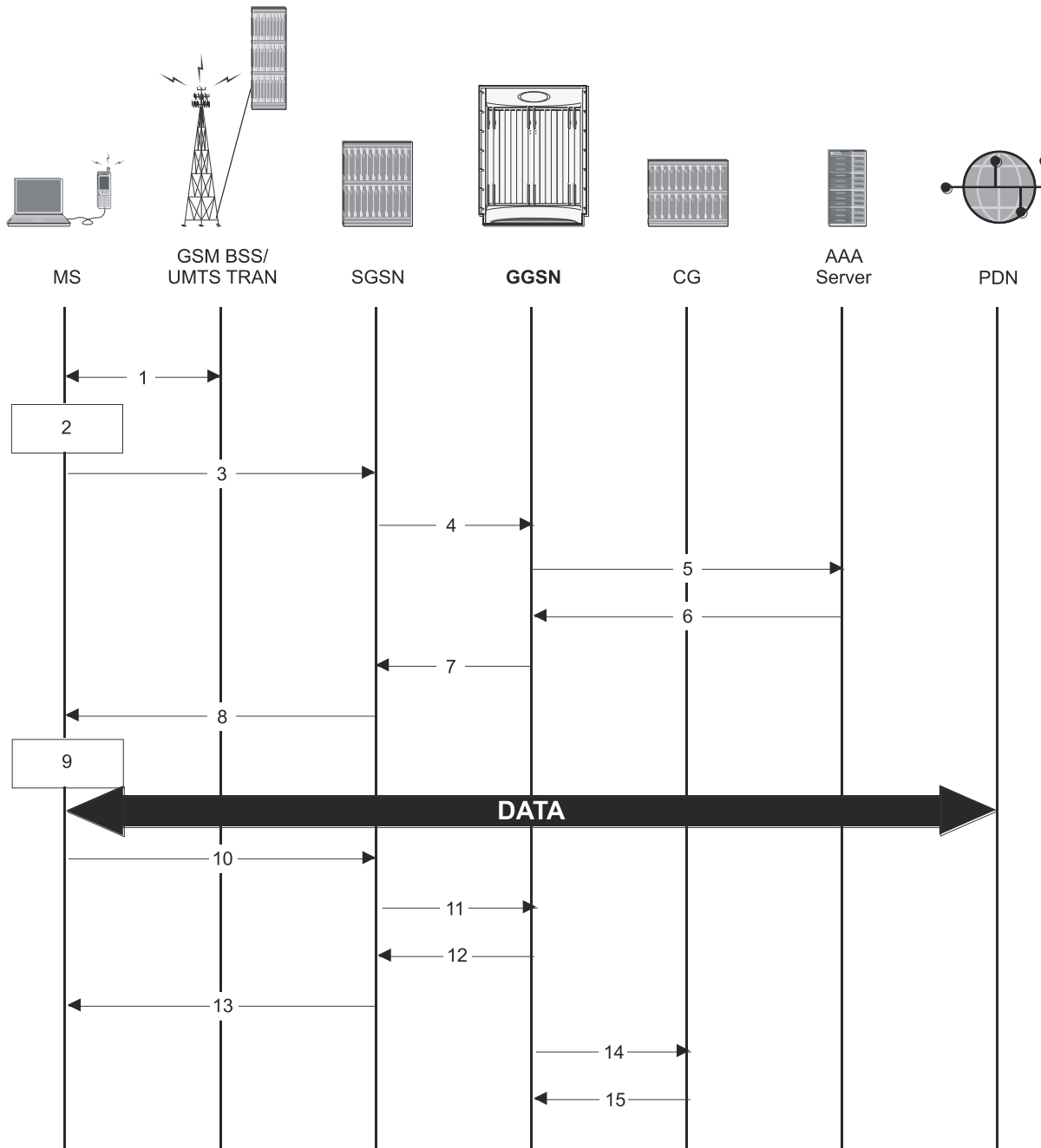
Figure 110. Non-Transparent IP Session Call Flow
