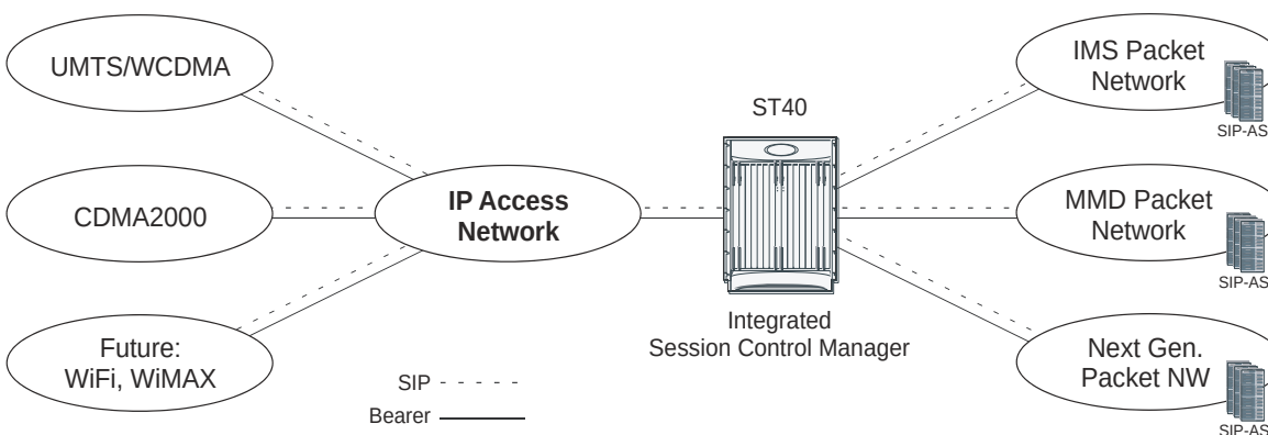
Figure 167. Cisco Integrated Session Control Manager
