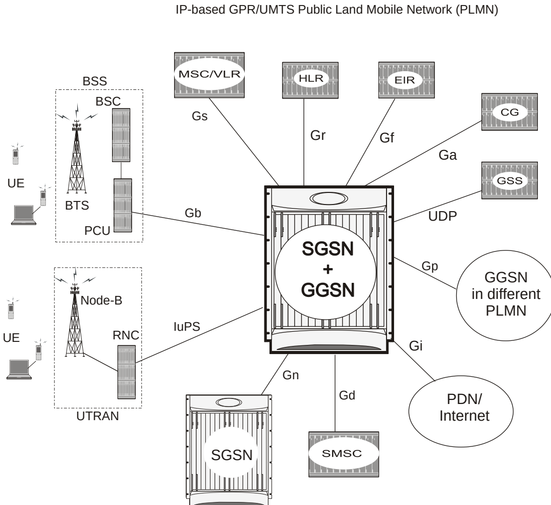
Figure 179. Co-located SGSN and GGSN
