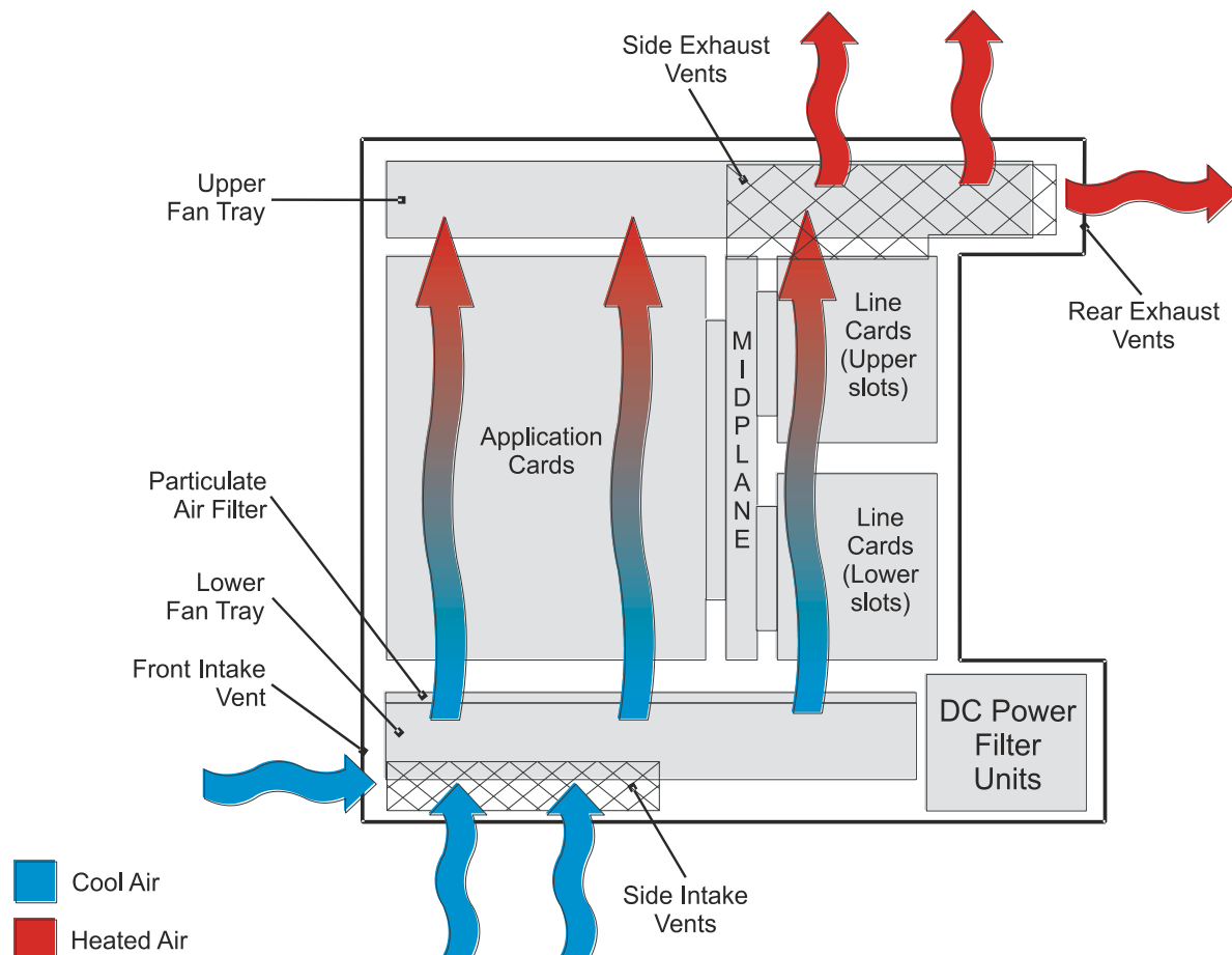
Figure 254. System Airflow and Ventilation
