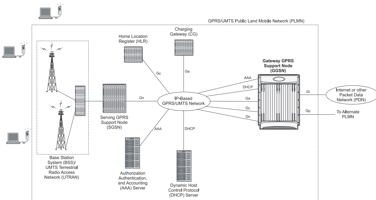
Figure 100. Basic GPRS/UMTS Network Topology
