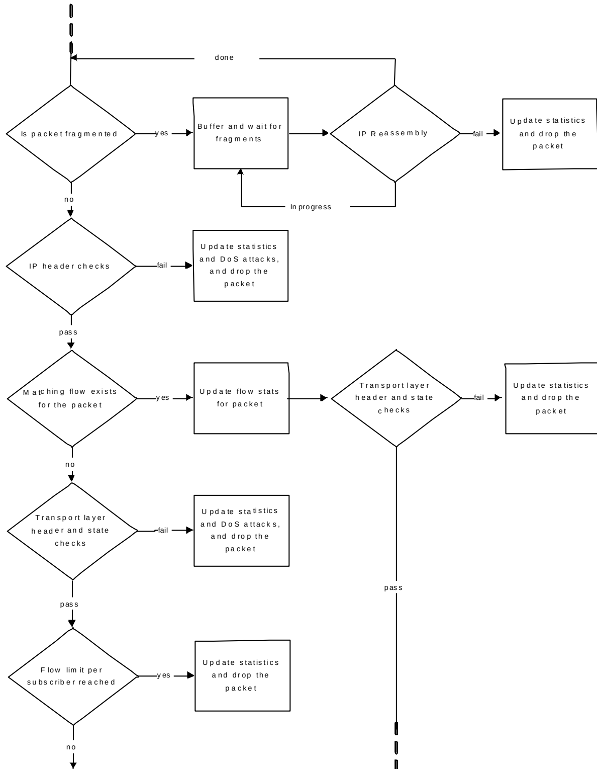
Figure 230. ... NAT Processing Flow
