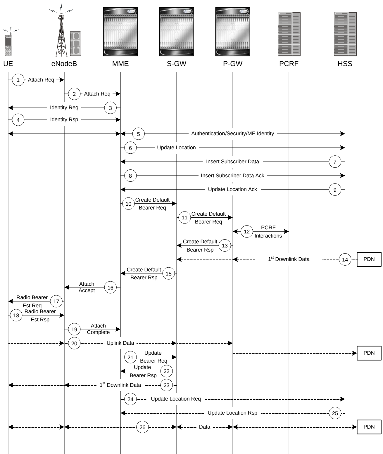
Figure 176. Subscriber-initiated Attach (initial) Call Flow
