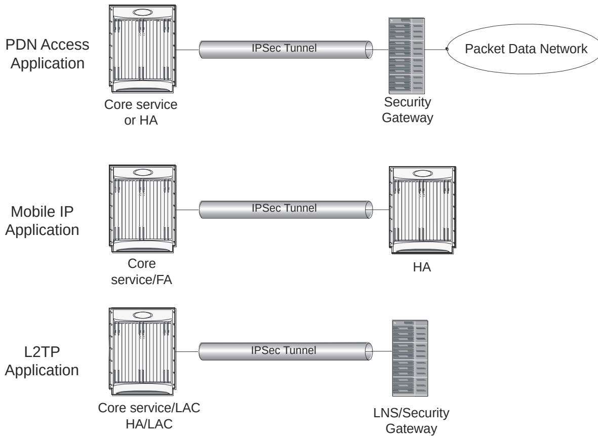
Figure 107. IPSec Application
