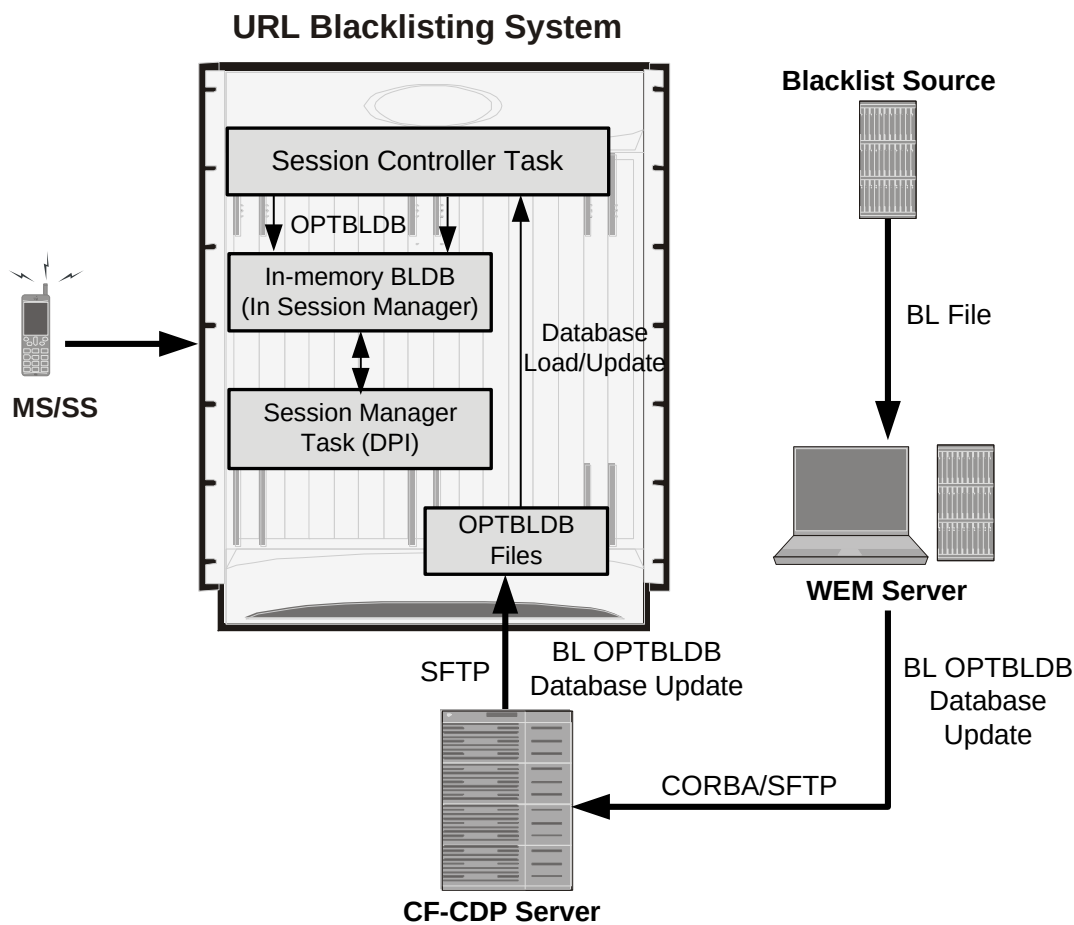
Figure 190. High-Level Architecture of URL Blacklisting with ACS
