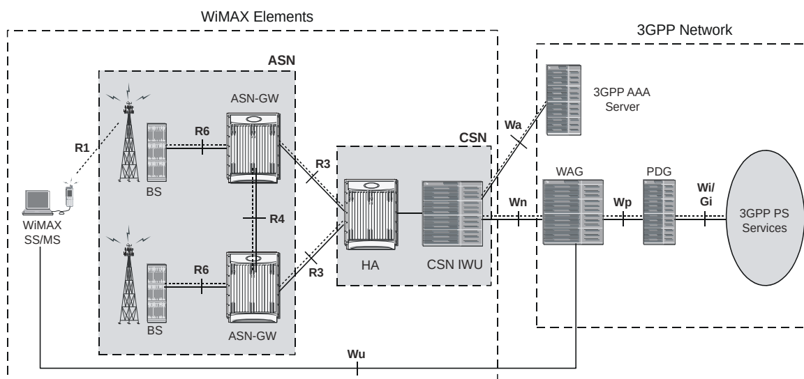
Figure 84. ASN Gateway with 3GPP Overlay
