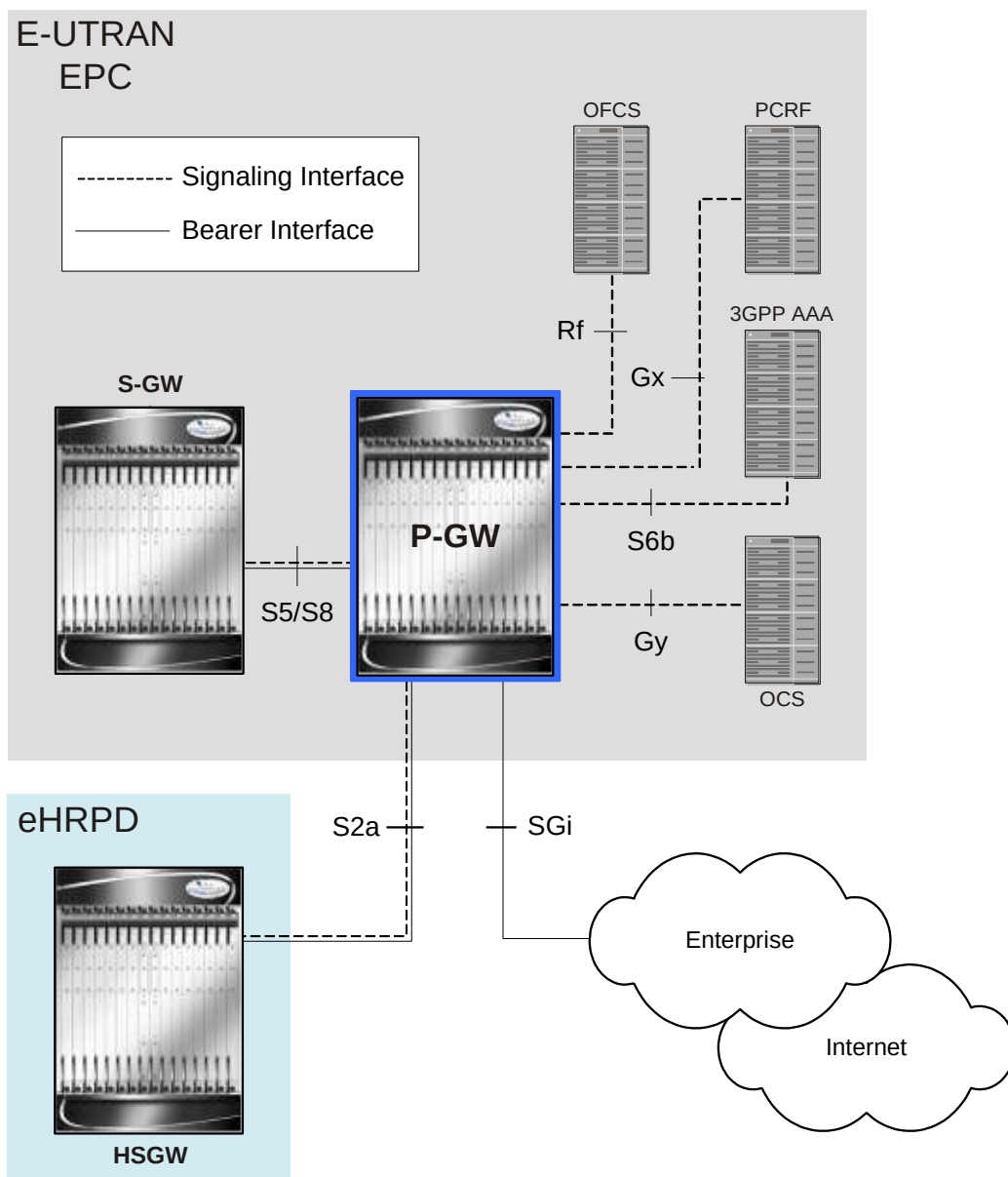
Figure 150. P-GW Interfaces Supporting eHRPD to E-UTRAN/EPC Connectivity
