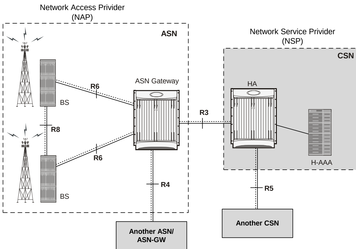
Figure 61. ASN Network Reference Model with ASN Gateway
