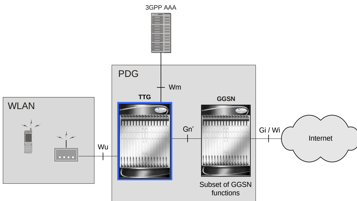
Figure 147. The TTG in a PDG Implementation
