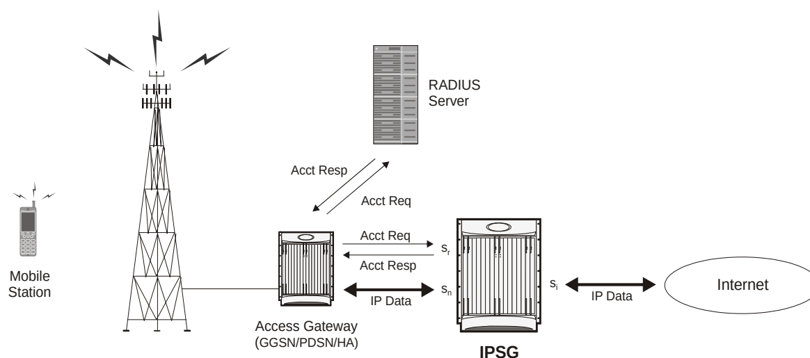
Figure 133. IPSG Message/Data Flow (RADIUS Server Mode)
