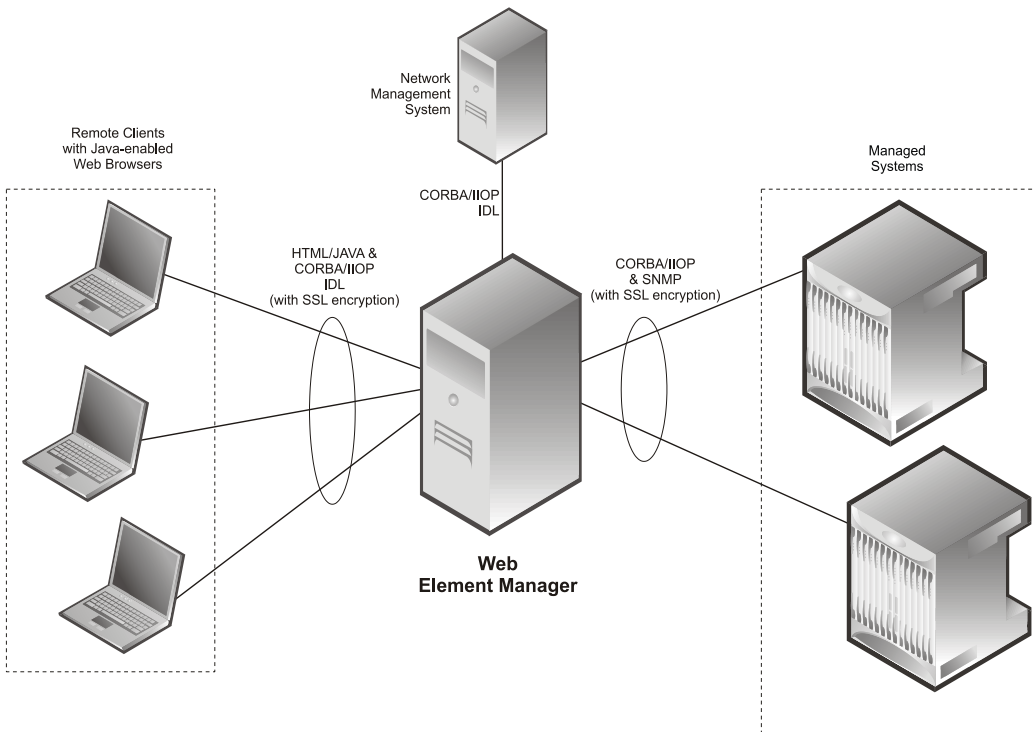
Figure 127. Web Element Manager Network Interfaces
