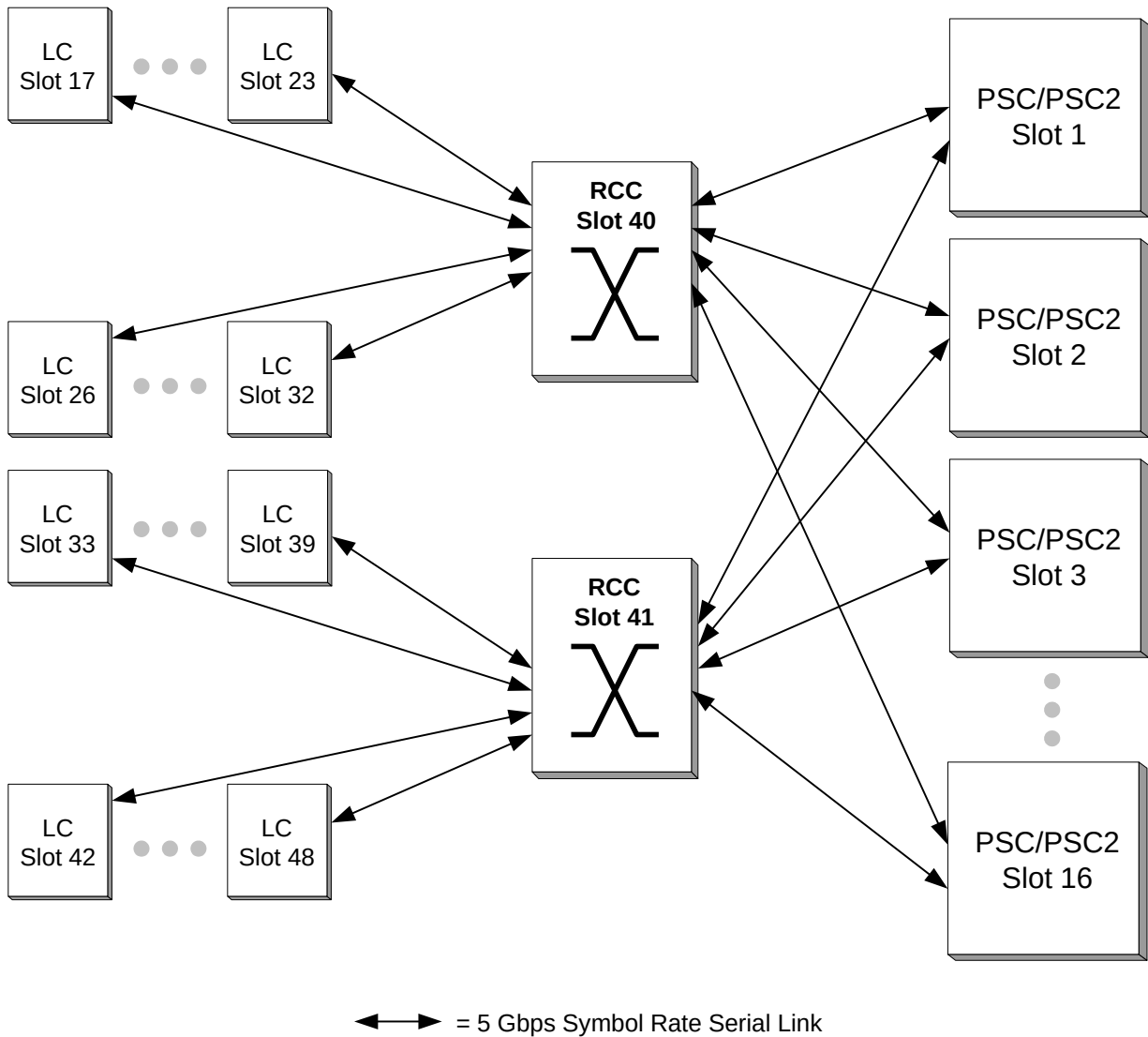
Figure 31. Logical View of RCC Links for Failover
