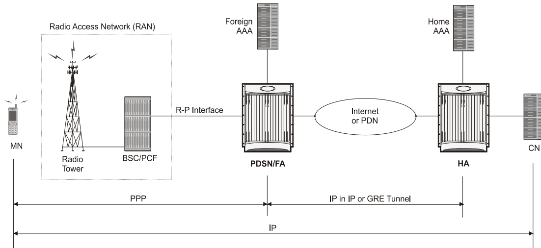
Figure 96. Mobile IP Protocol Usage
