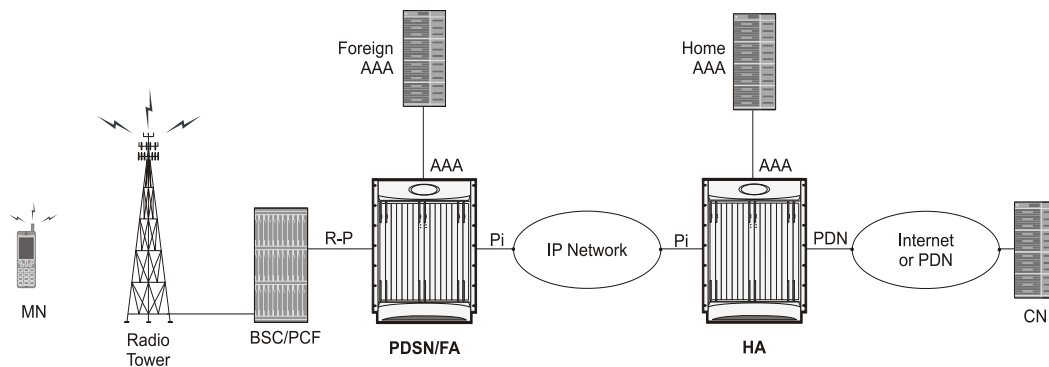
Figure 91. PDSN/FA and HA Network Deployment Configuration Example
