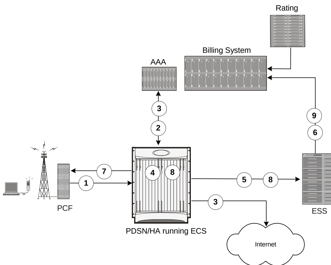
Figure 205. Postpaid Billing with ECS in CDMA-2000 Network
