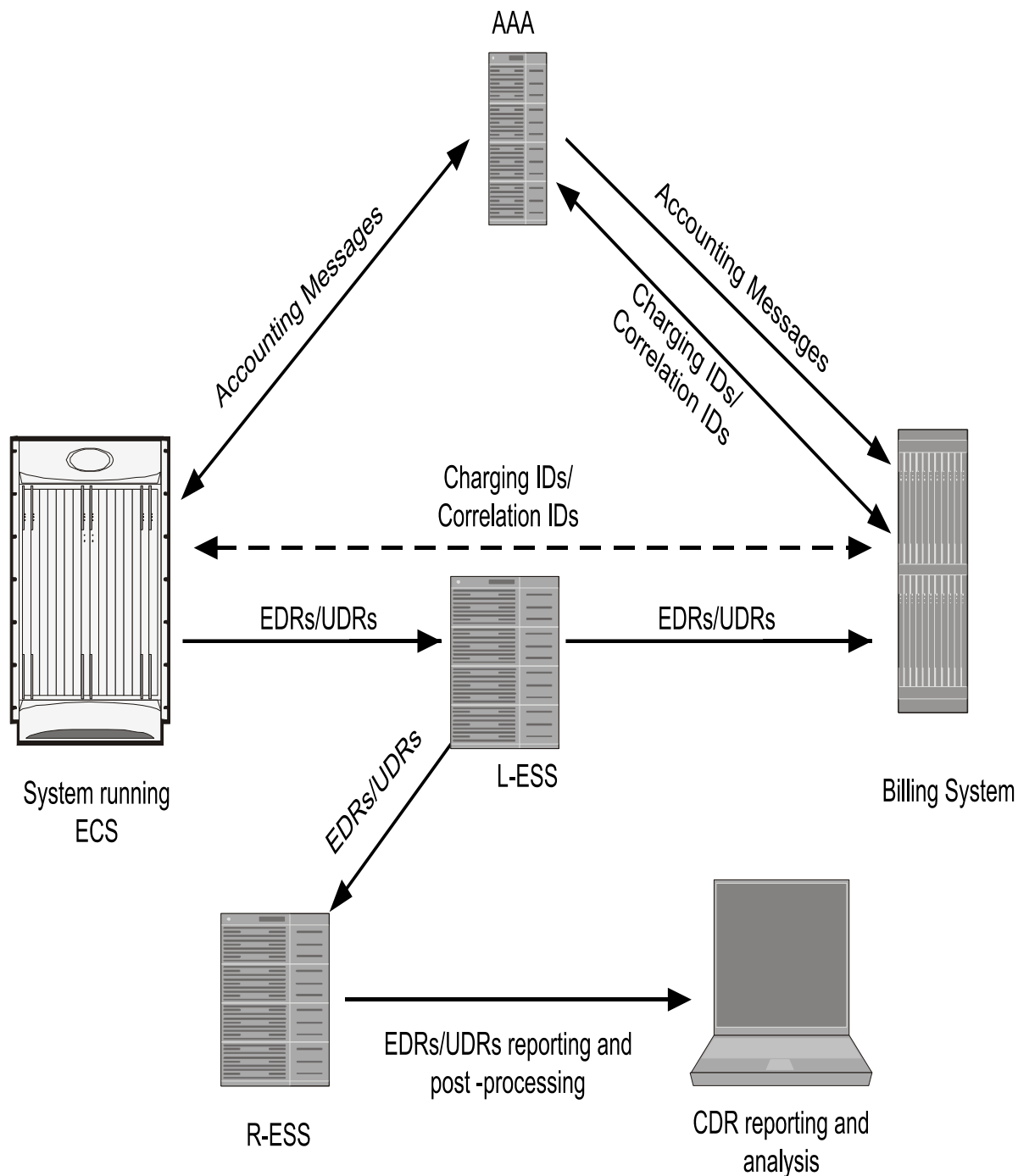
Figure 224. ESS architecture with ECS
