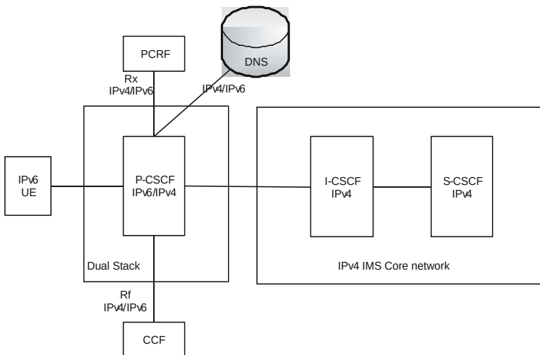
Figure 168. Interworking Between IPv6 UE and IPv4 IMS Core Network
