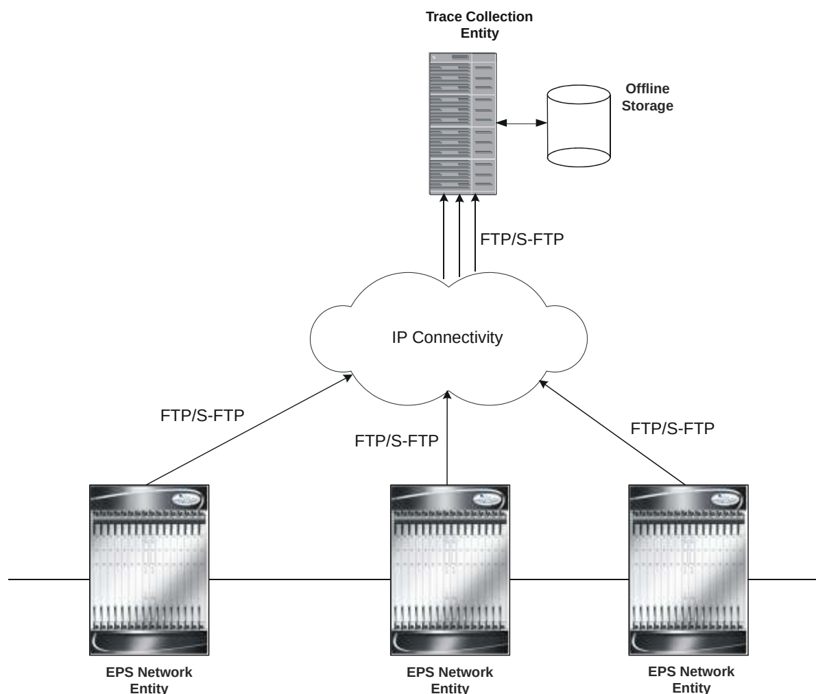
Figure 208. Session Trace Function and Interfaces
