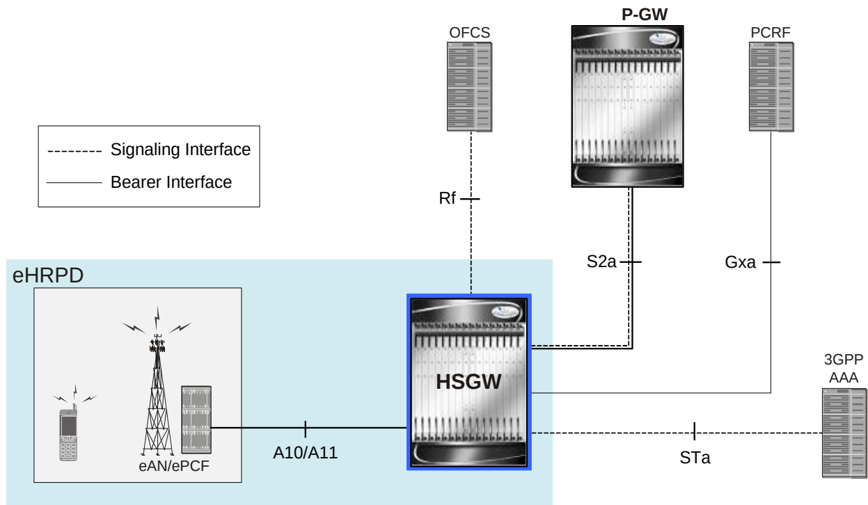
Figure 125. HSGW Supported Network Interfaces
