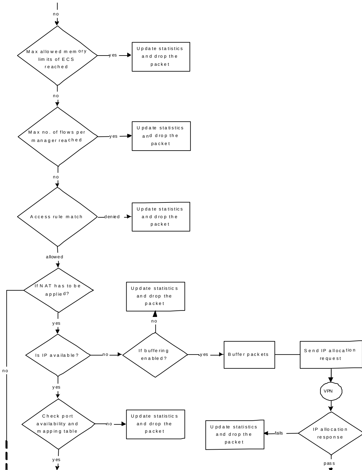
Figure 231. ... NAT Processing Flow
