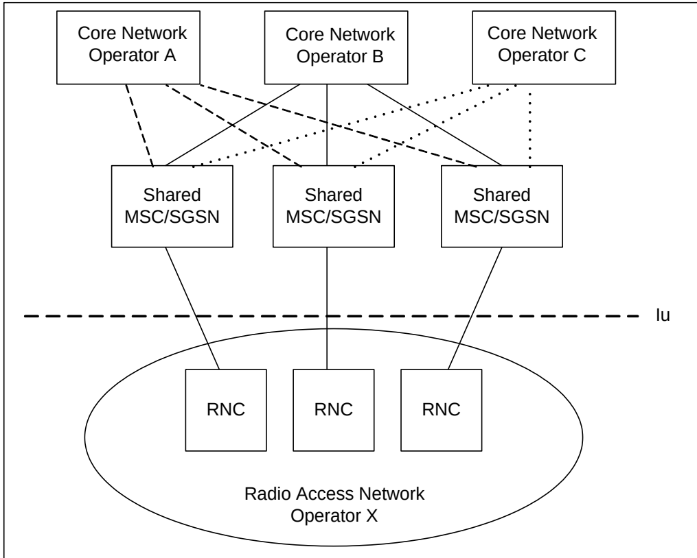
Figure 180. GWCN-type Network Sharing
