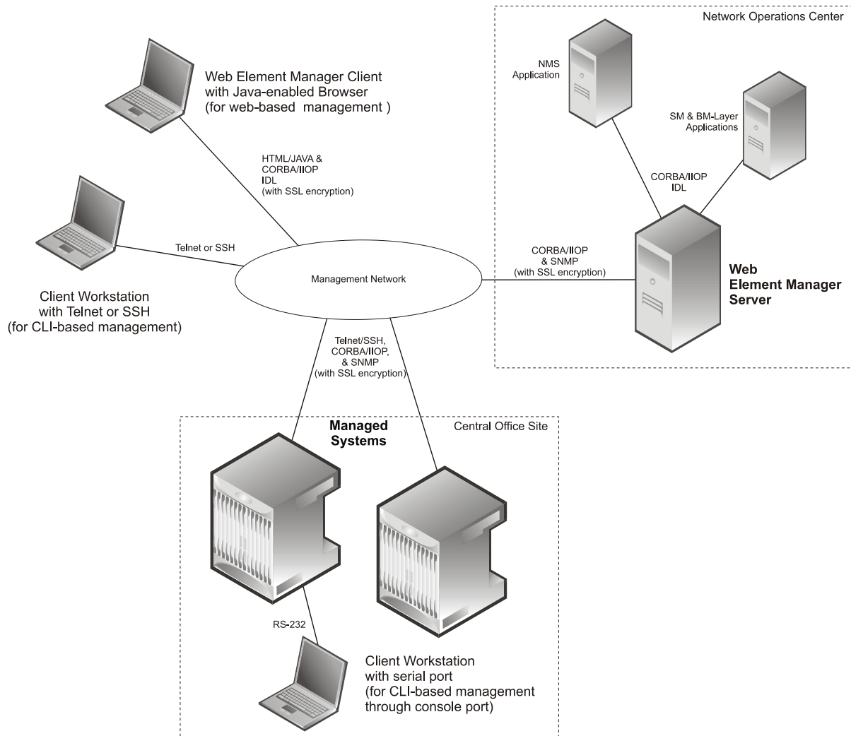
Figure 211. Element Management Methods
