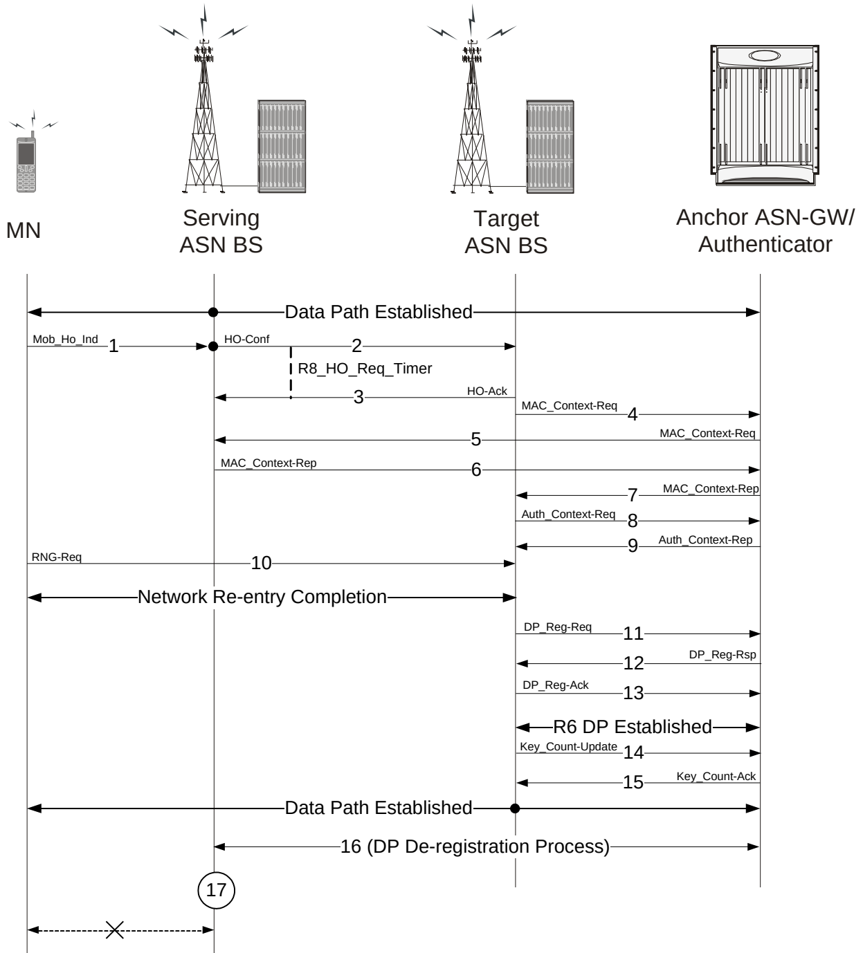
Figure 71. MS initiated Uncontrolled Intra-ASN Gateway Handover Action Phase
