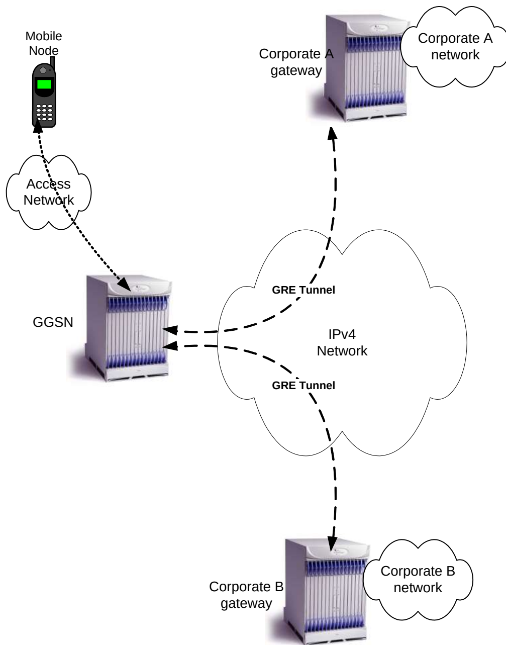
Figure 106. GRE Deployment Scenario
