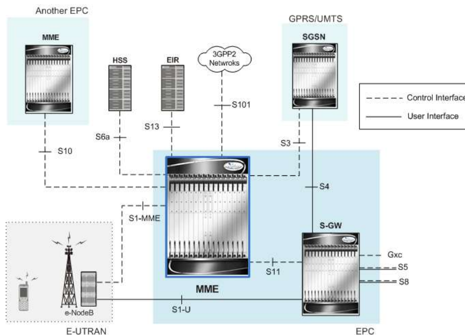
Figure 207. The MME in LTE/SAE Networks and Interfaces
