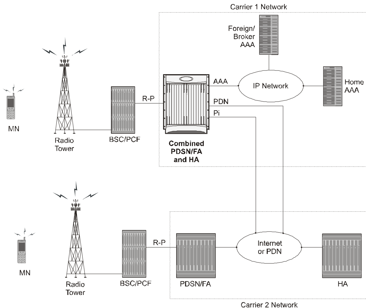
Figure 119. Co-located PDSN/FA and HA Configuration Example.
