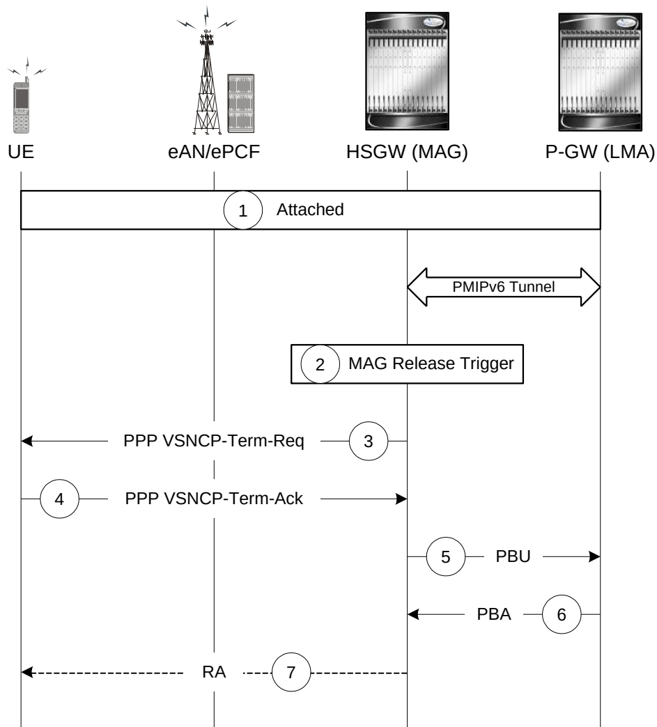
Figure 158. PDN Connection Release by the HSGW Call Flow
