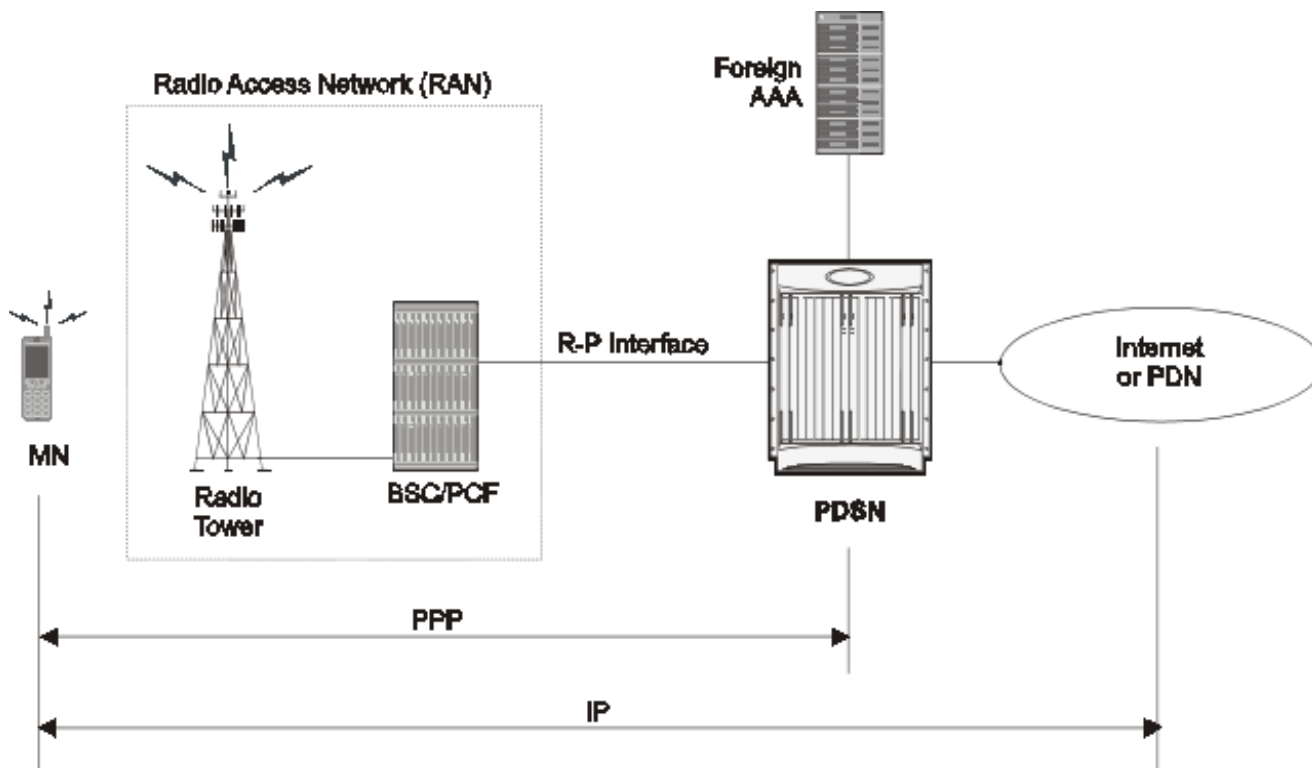
Figure 93. Simple IP Protocol Usage
