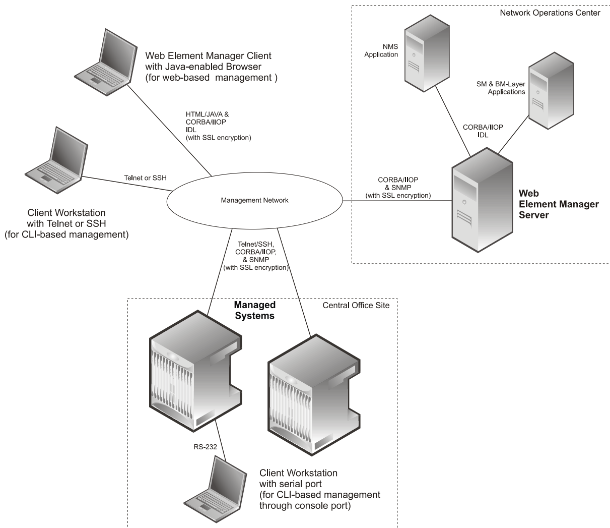
Figure 105. Element Management Methods
