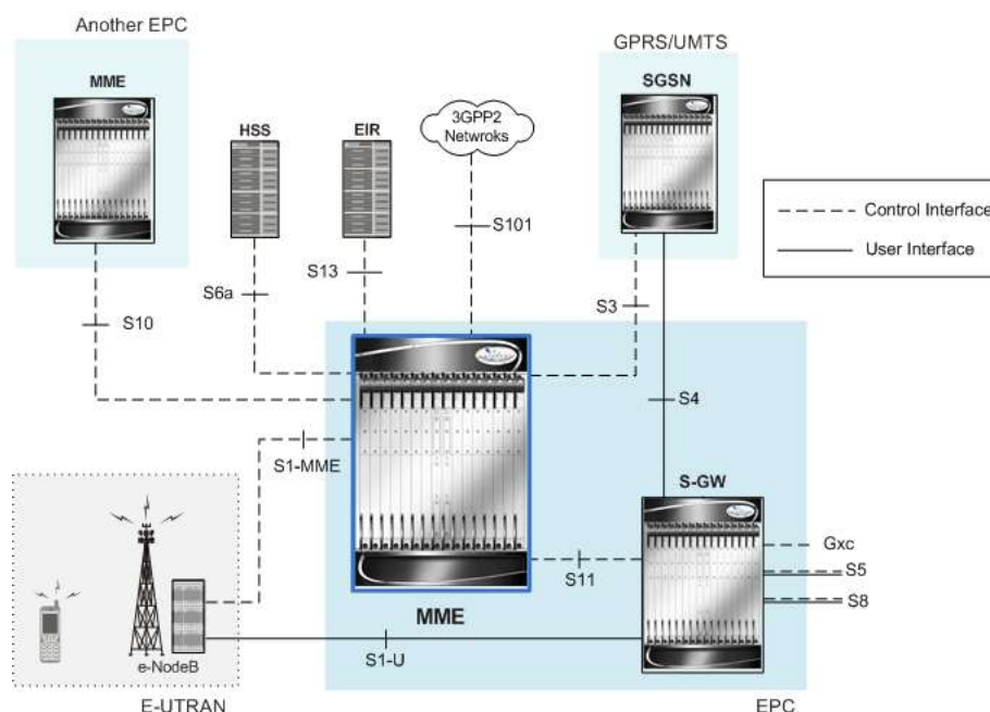
Figure 9. MME in LTE/SAE Networks and Interfaces
