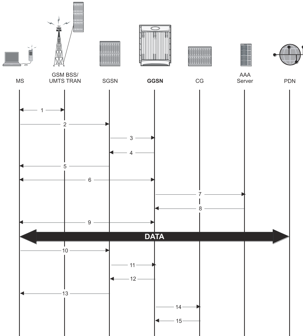
Figure 112. PPP Direct Access Call Flow
