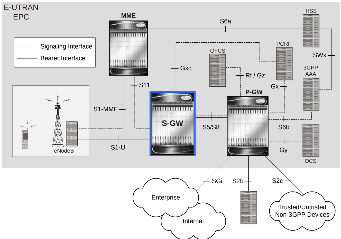
Figure 172. S-GW in the E-UTRAN/EPC Network
