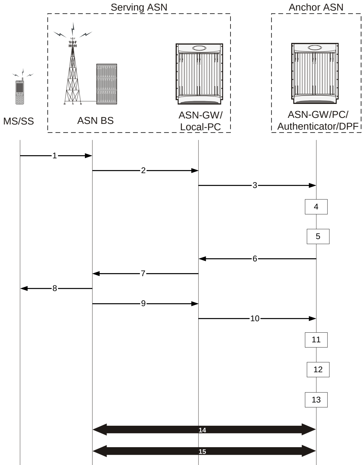
Figure 89. MS Initiated Idle Mode Entry Procedure Flow
