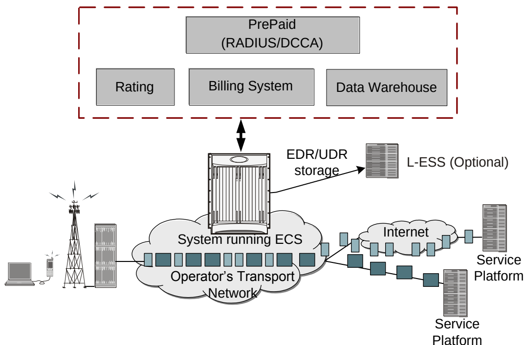
Figure 201. Prepaid Billing Scenario with ECS
