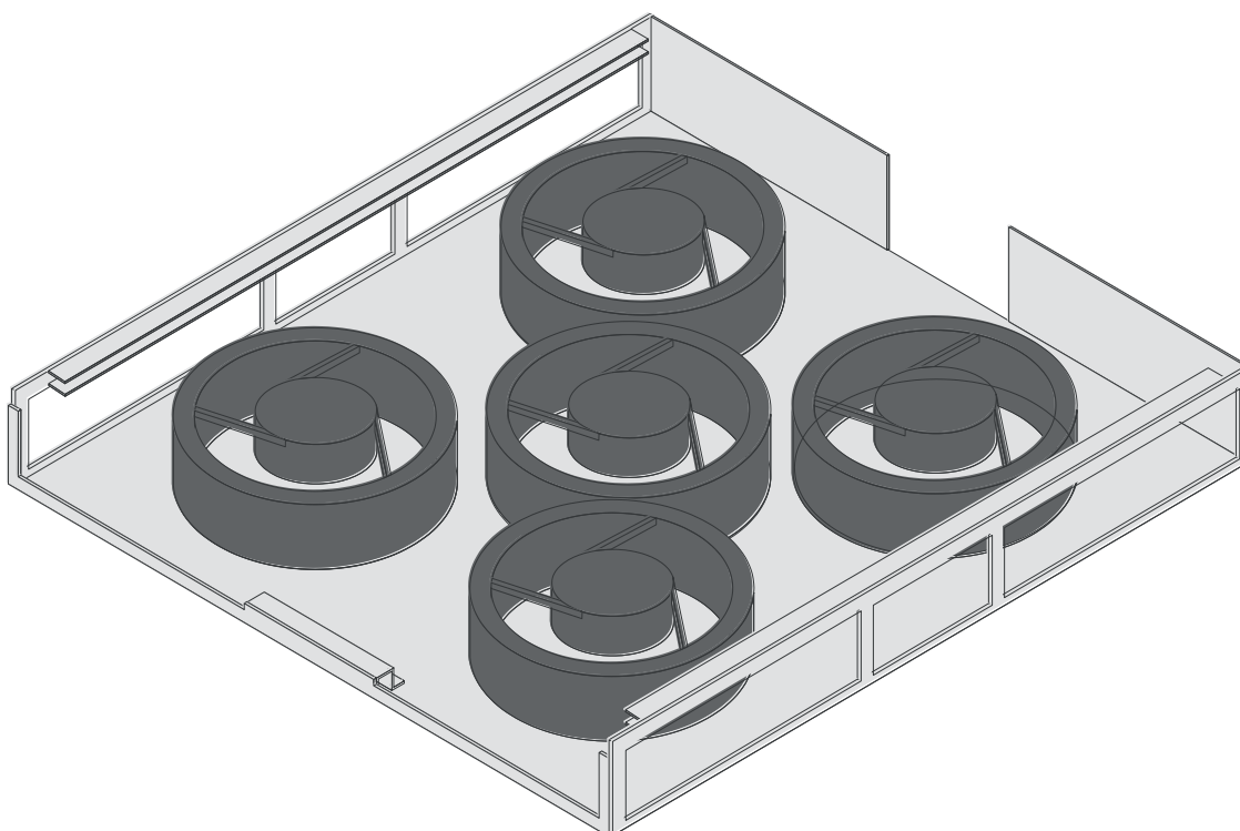
Figure 33. Lower Fan Tray Assembly
