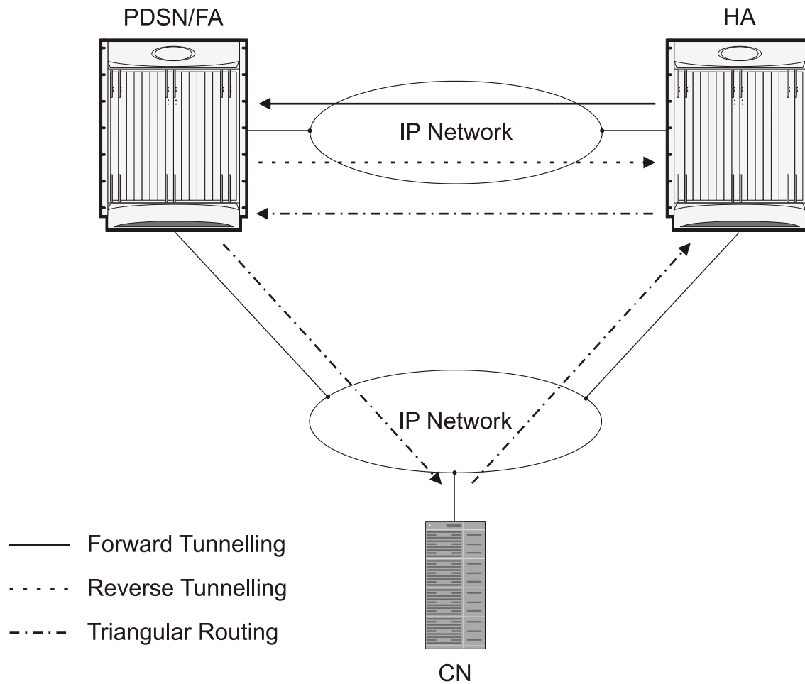
Figure 95. Mobile IP, FA and HA Tunneling/Transport Methods
