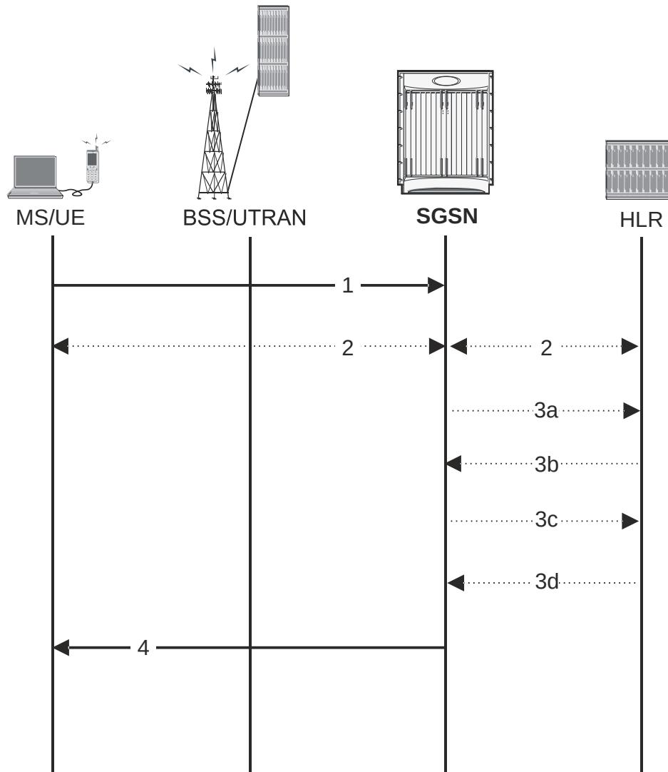
Figure 186. imple First-Time GPRS Attach
