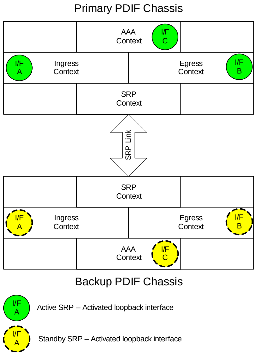
Figure 144. Loopback Interface Configuration
