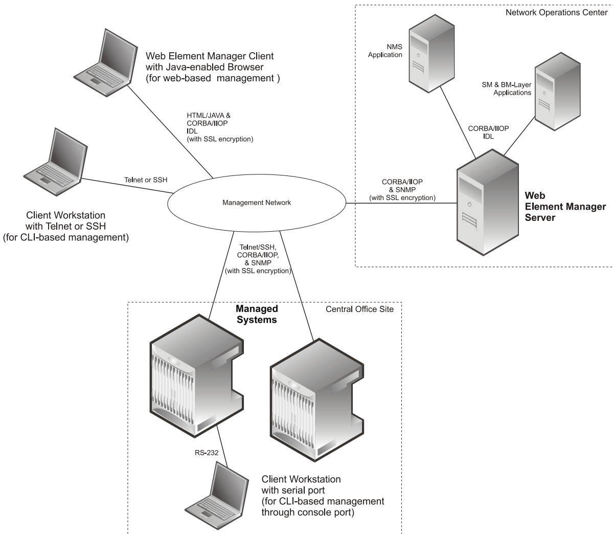
Figure 126. Element Management Methods
