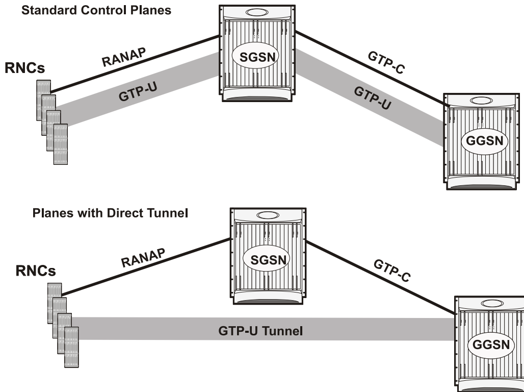
Figure 104. Direct Tunnel Support in GGSN
