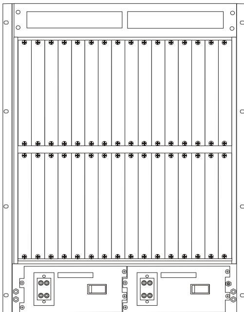
Figure 29. Rear Slot Numbering Scheme for Line Cards
