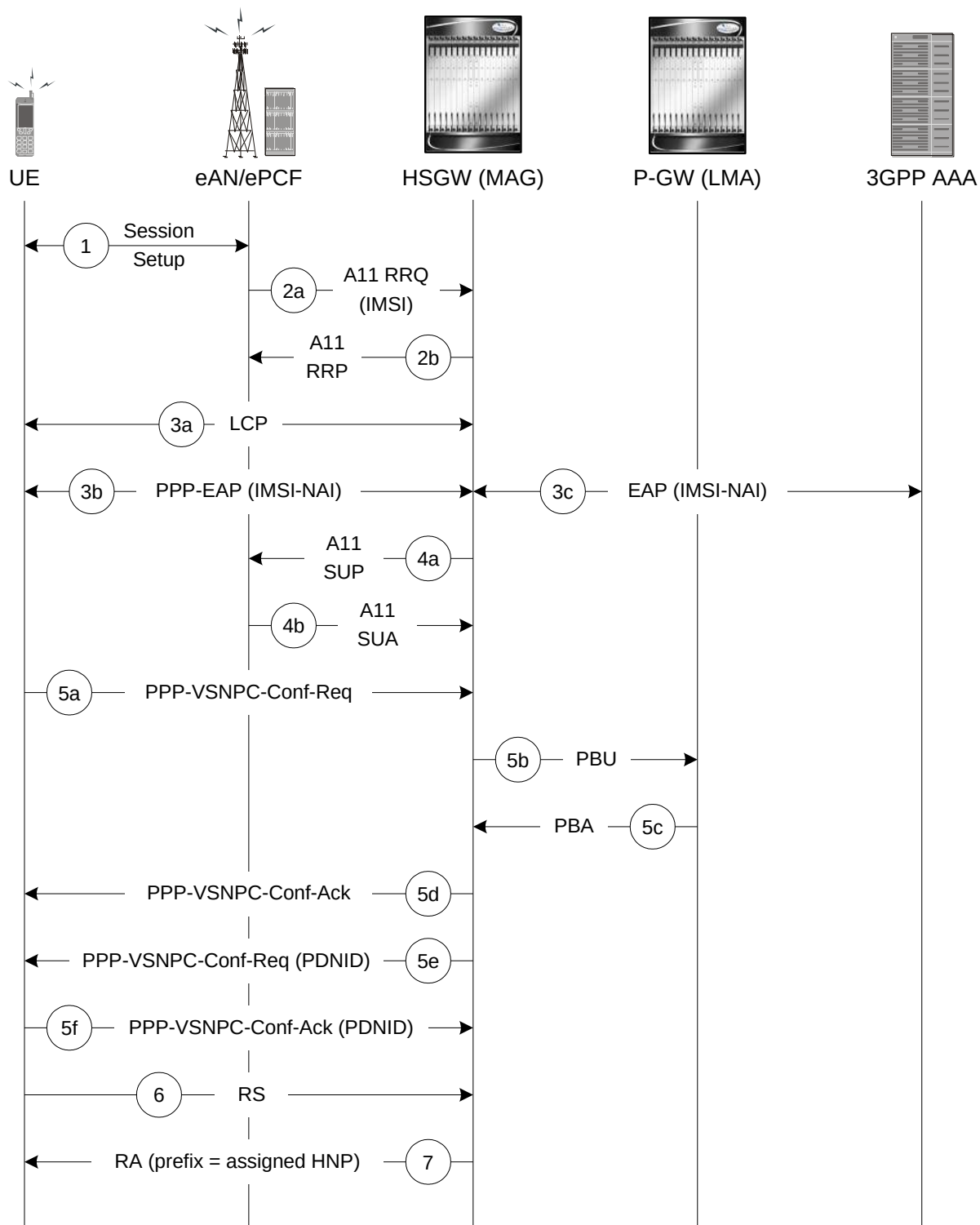
Figure 155. Initial Attach with IPv6/IPv4 Access Call Flow
