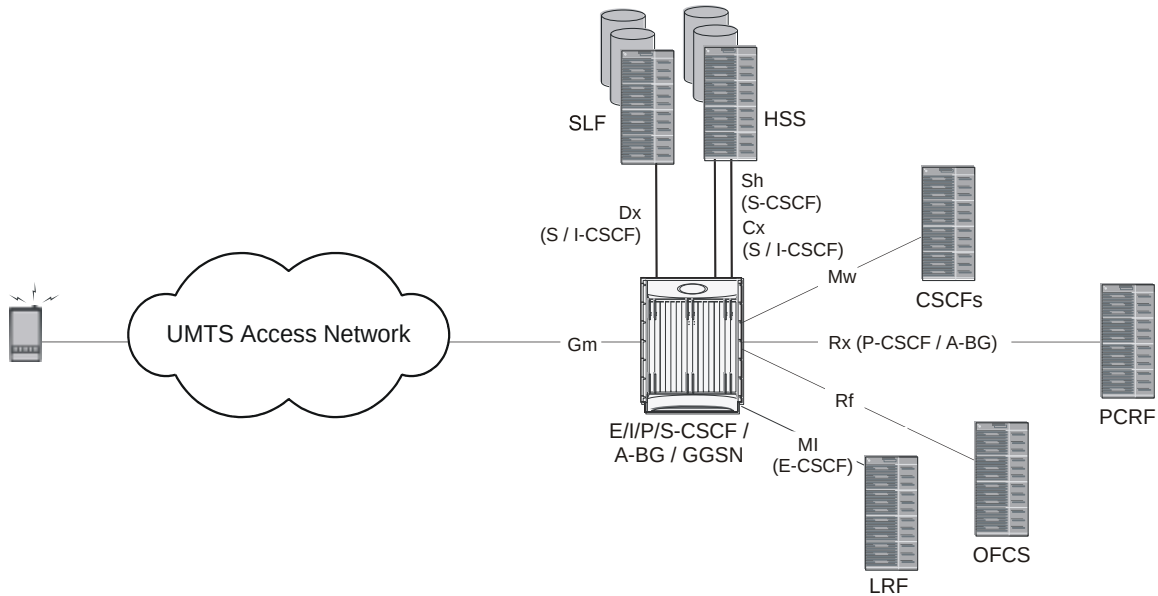
Figure 166. GSM/UMTS CSCF/A-BG/GGSN SCM Deployment Example
