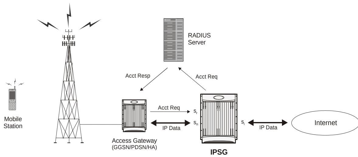
Figure 135. IPSG Message/Data Flow (RADIUS Snoop Mode)
