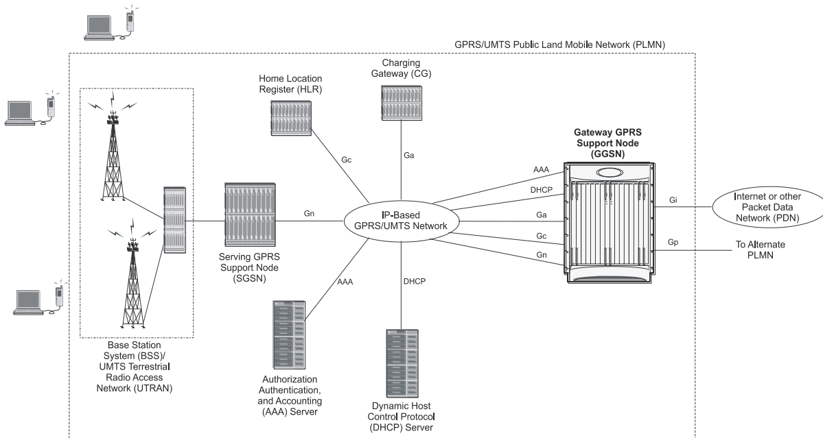
Figure 101. Basic GPRS/UMTS Network Topology
