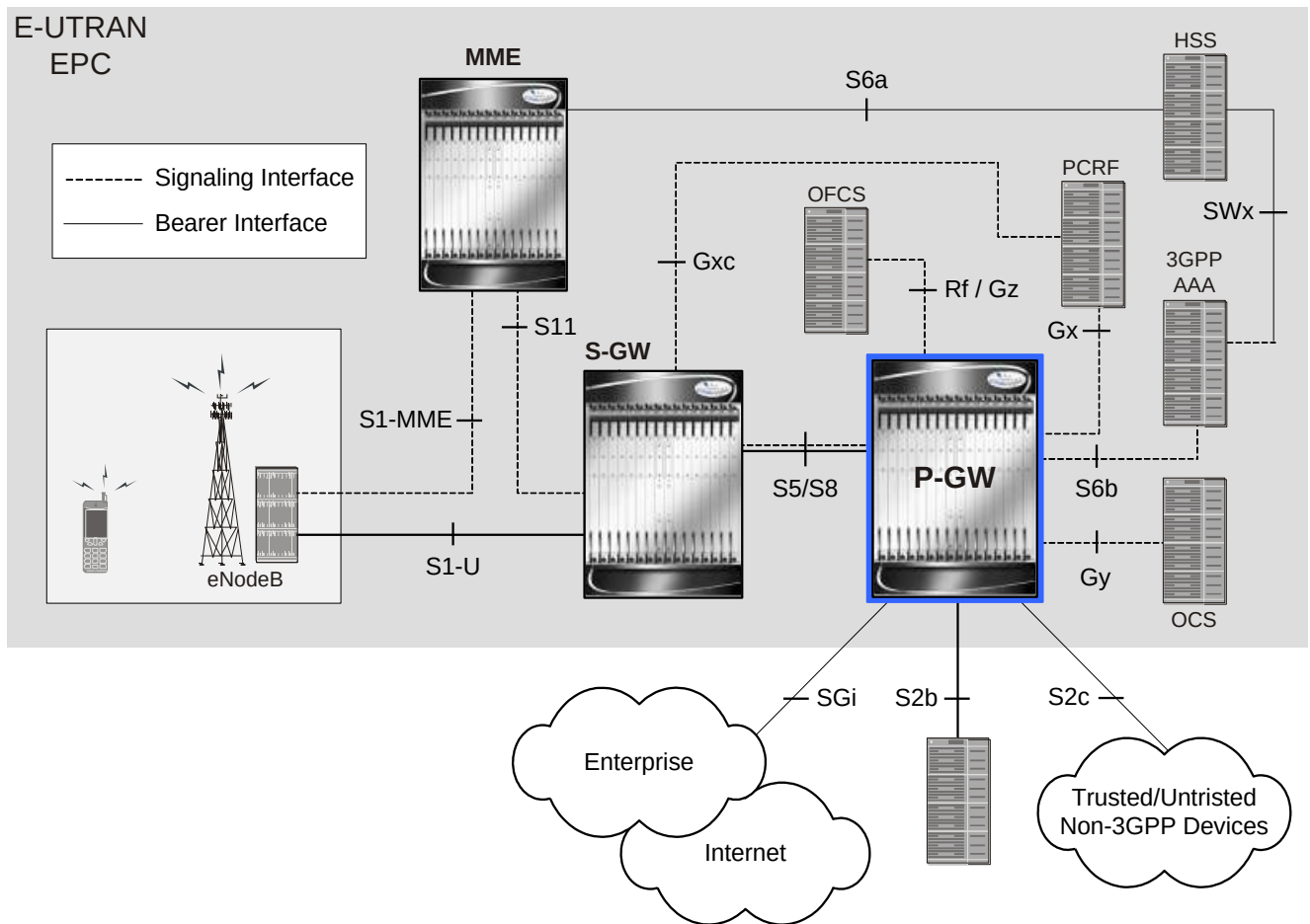
Figure 151. P-GW in the E-UTRAN/EPC Network
