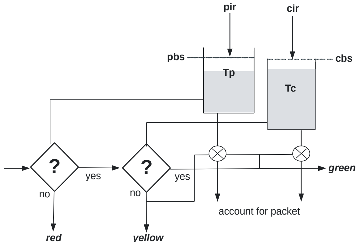
Figure 185. trTCM Algorithm Logic for Traffic Policing
