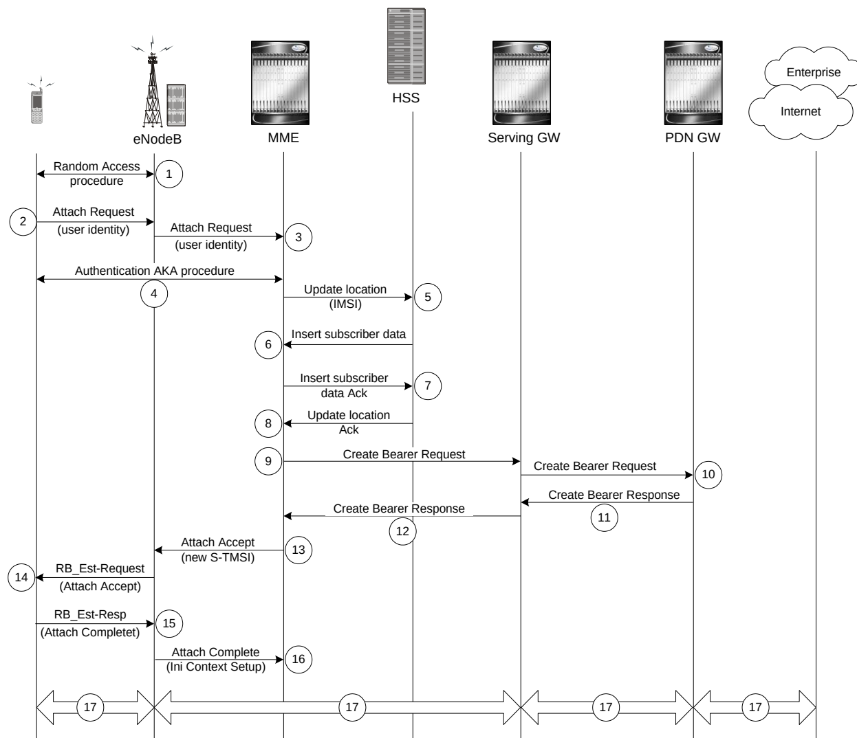
Figure 212. Subscriber Registration Setup Message Flow
