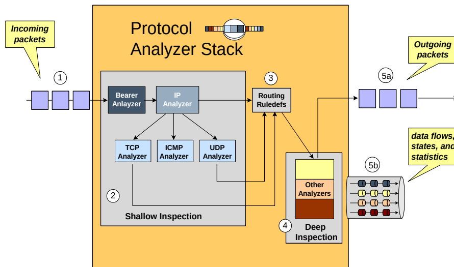
Figure 197. Routing Ruledefs and Packet Inspection
