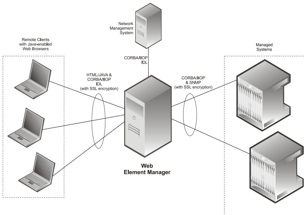
Figure 233. Web Element Manager Network Interfaces
