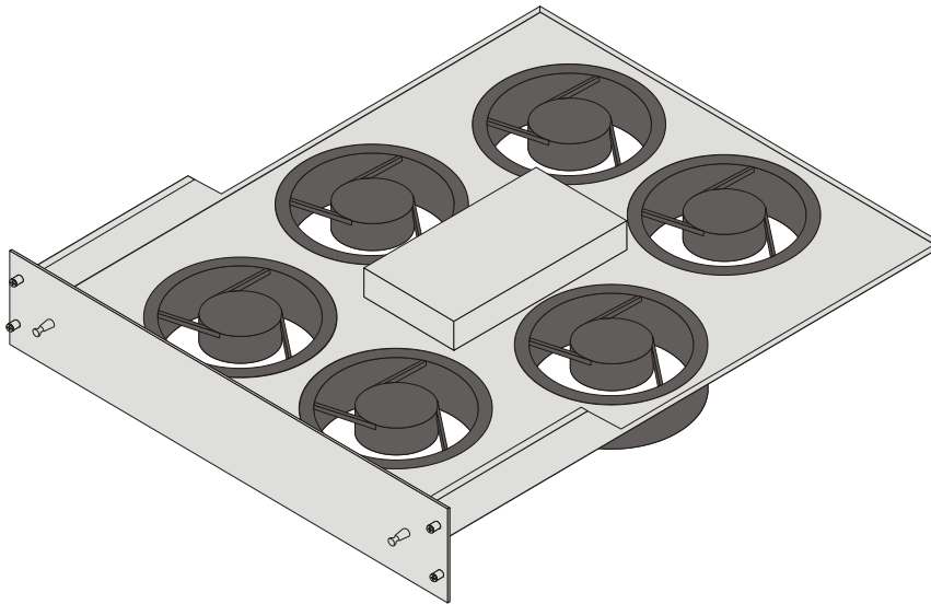
Figure 35. Upper Fan Tray Assembly
