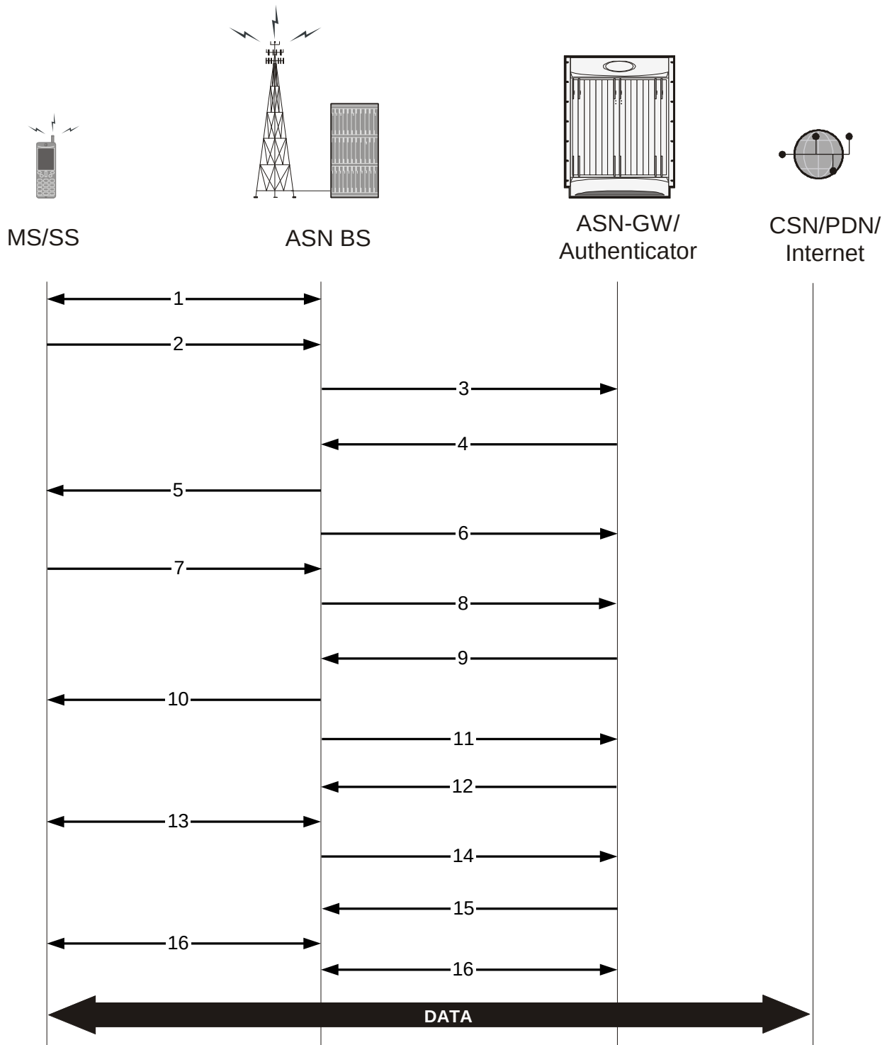
Figure 65. Initial Network Entry and Data Session Establishment without Authentication Call Flow
