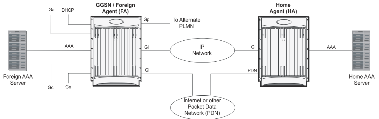
Figure 103. Combined GGSN/FA/HA Deployment for Mobile IP and/or Proxy Mobile IP Support
