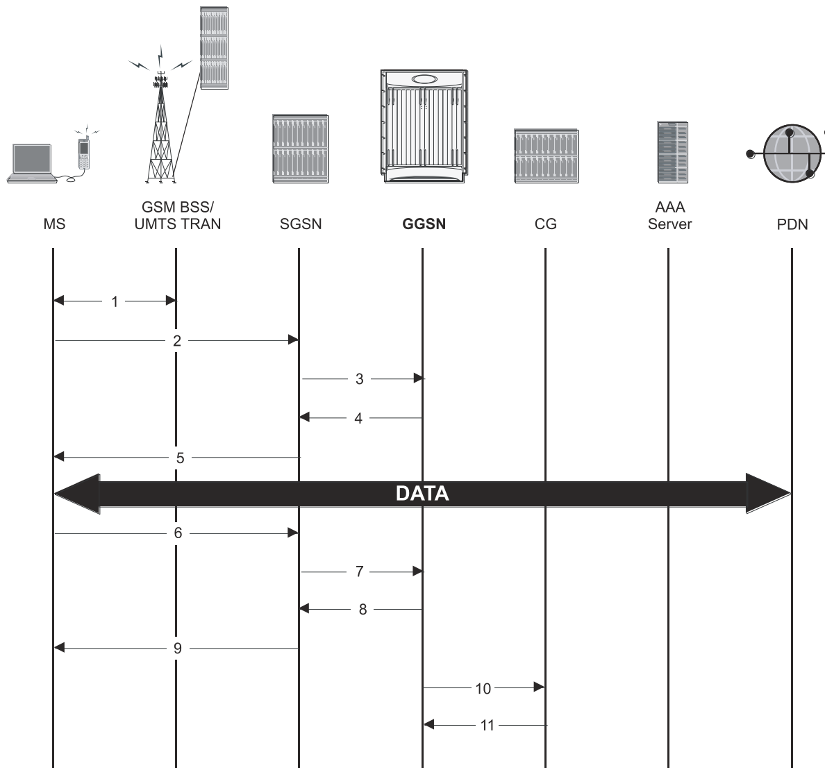
Figure 109. Transparent IP Session Call Flow
