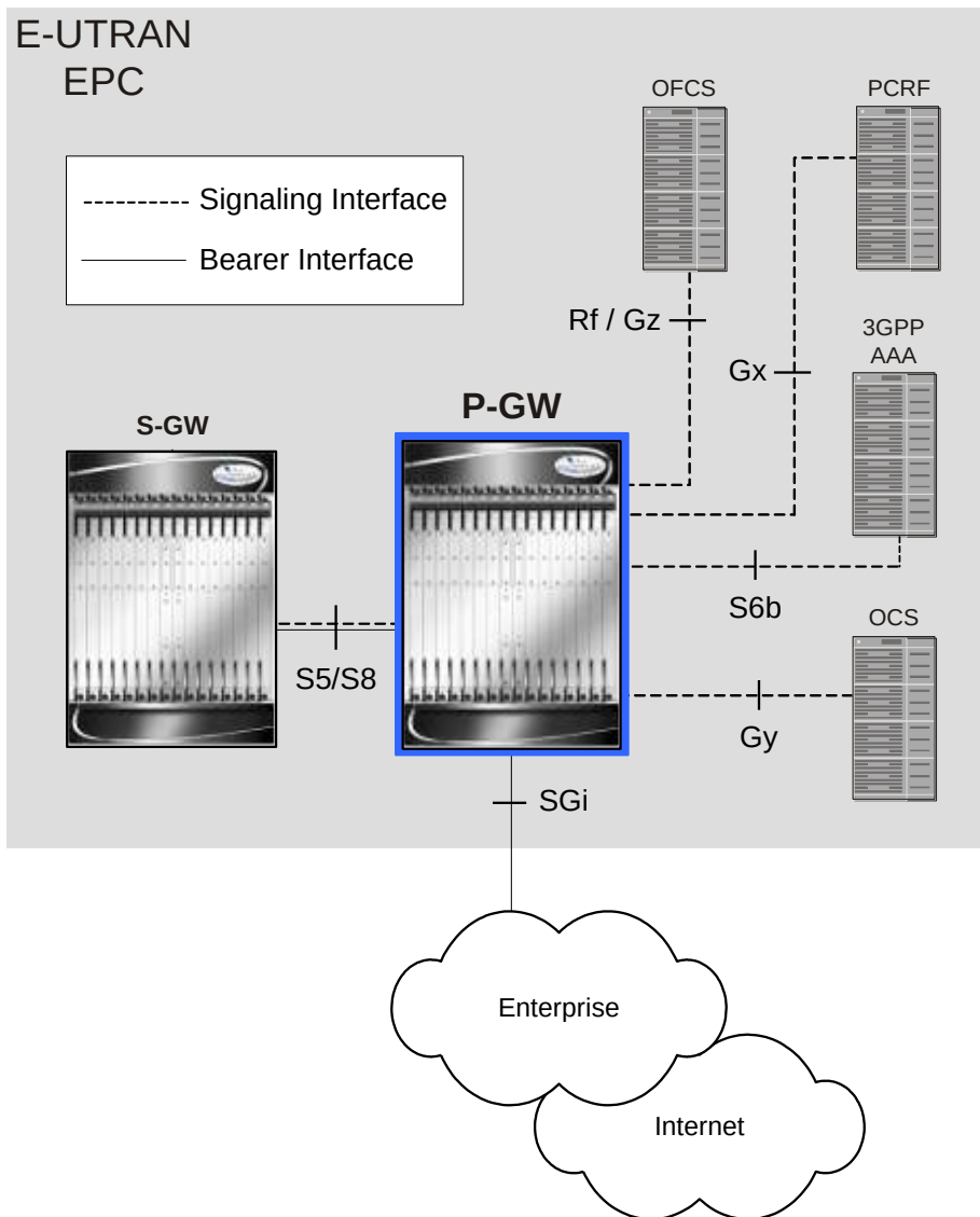
Figure 132. P-GW Interfaces in the E-UTRAN/EPC Network
