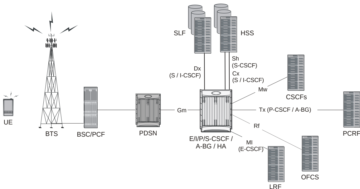
Figure 145. CDMA2000 CSCF/A-BG/HA SCM Deployment Example
