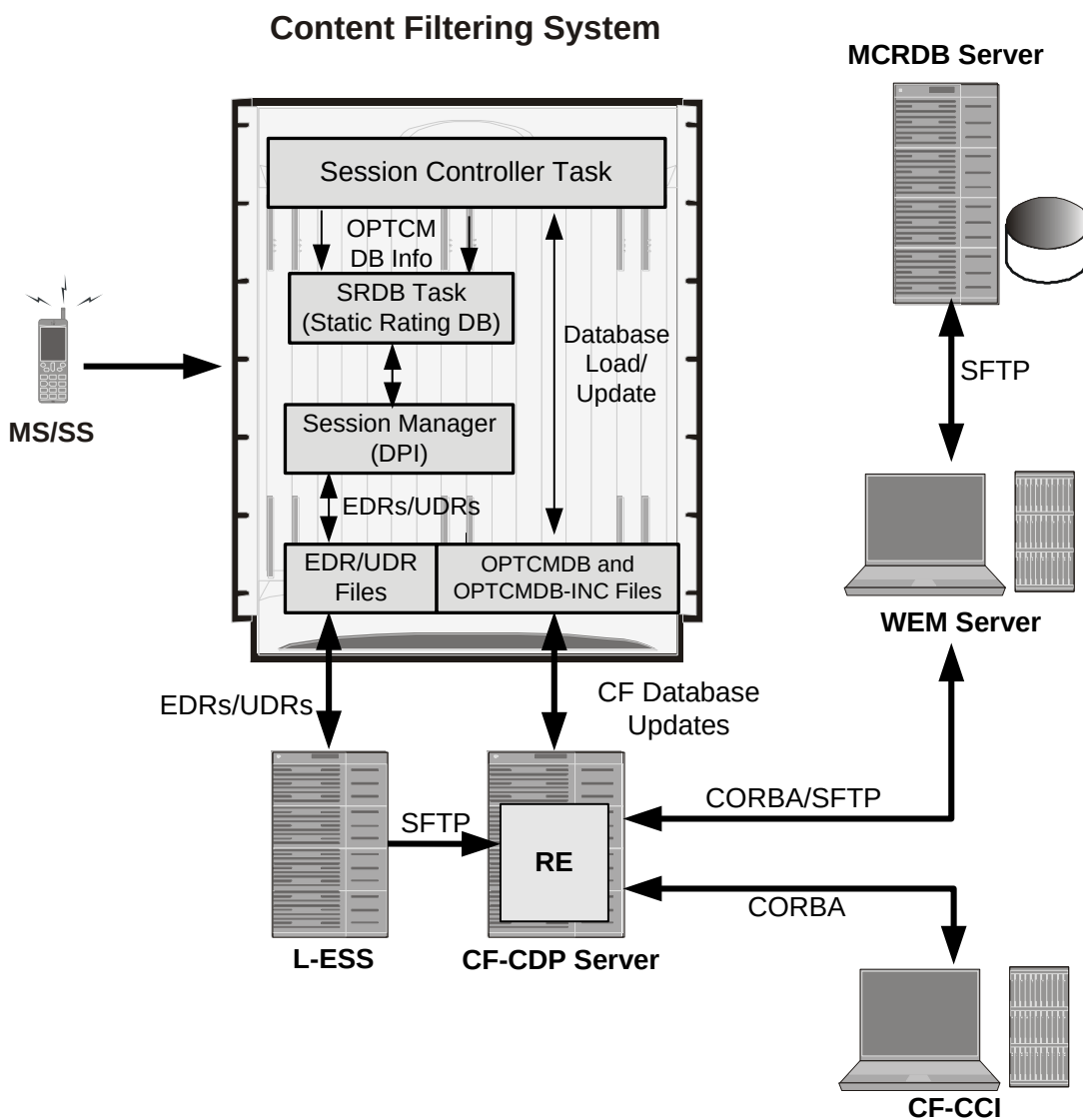
Figure 173. High-Level Architecture of Category-based Content Filtering
