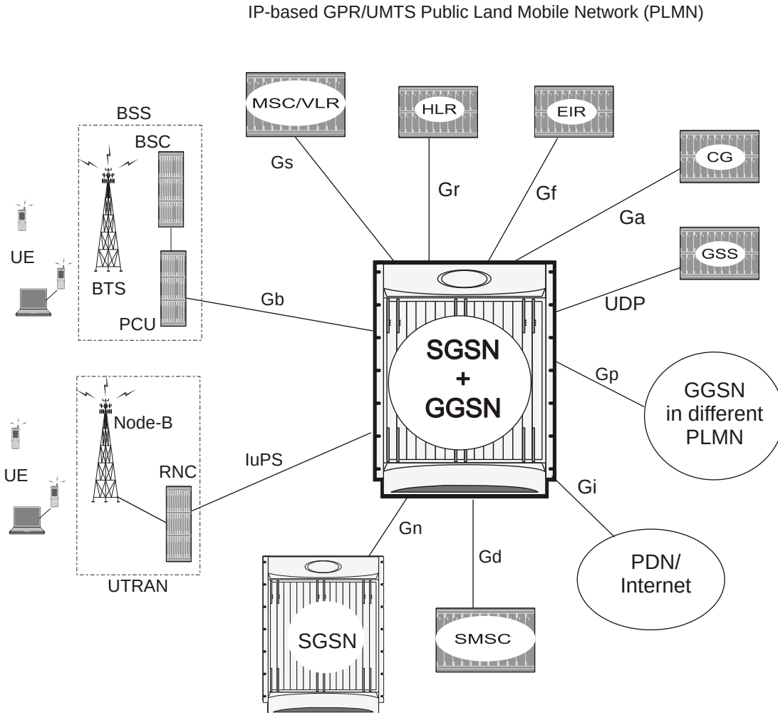
Figure 161. Co-located SGSN and GGSN
