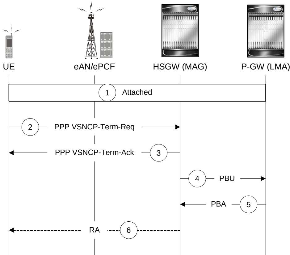
Figure 137. PDN Connection Release by the UE Call Flow
