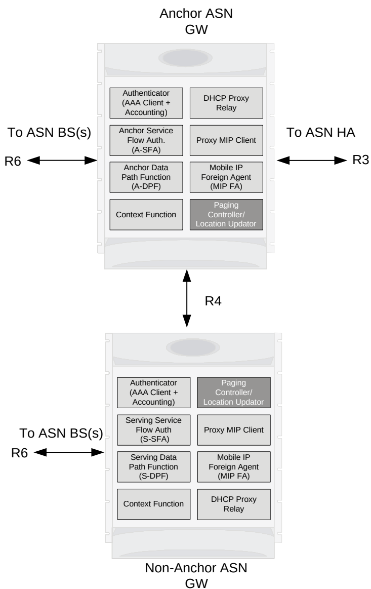
Figure 53. Distribution of Components and Function in ASN Gateway for Handover
