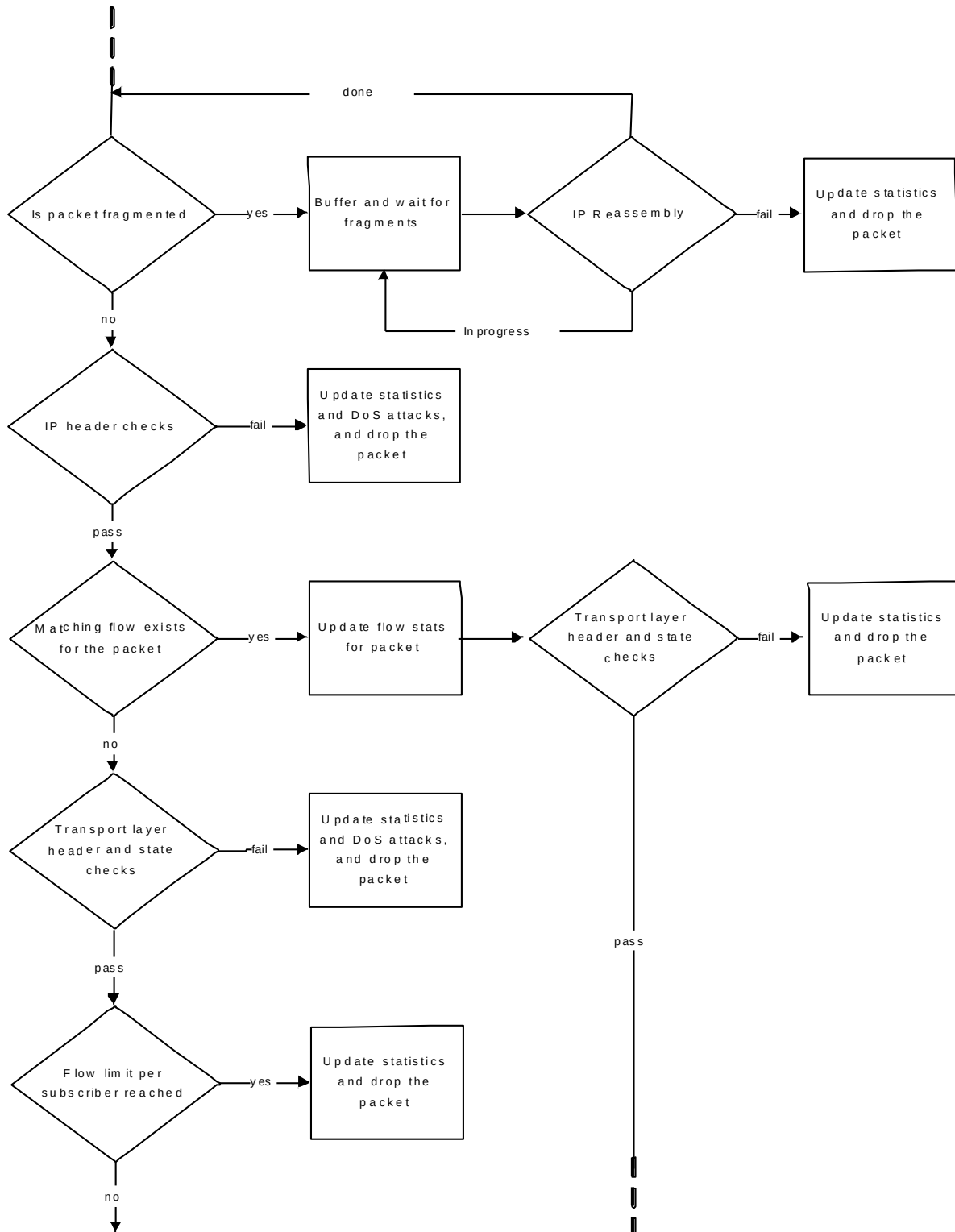
Figure 212. ... NAT Processing Flow
