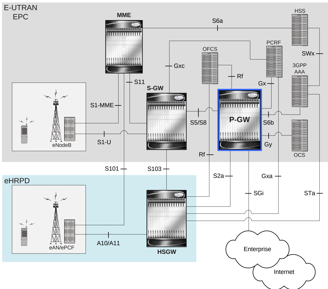
Figure 128. Basic E-UTRAN/EPC and eHRPD Network Topology
