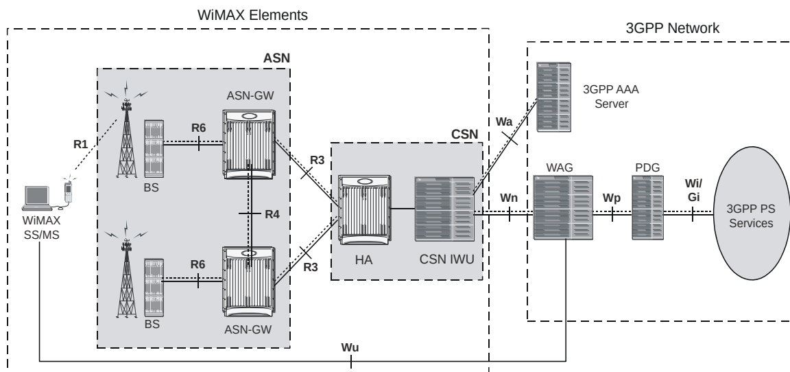
Figure 63. ASN Gateway with 3GPP Overlay
