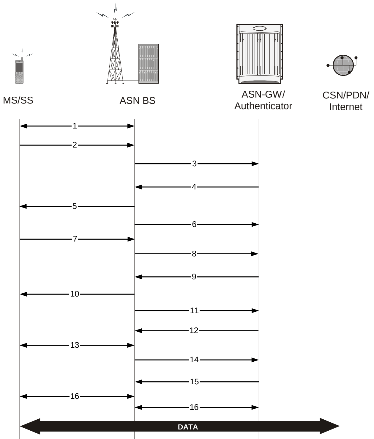
Figure 44. Initial Network Entry and Data Session Establishment without Authentication Call Flow
