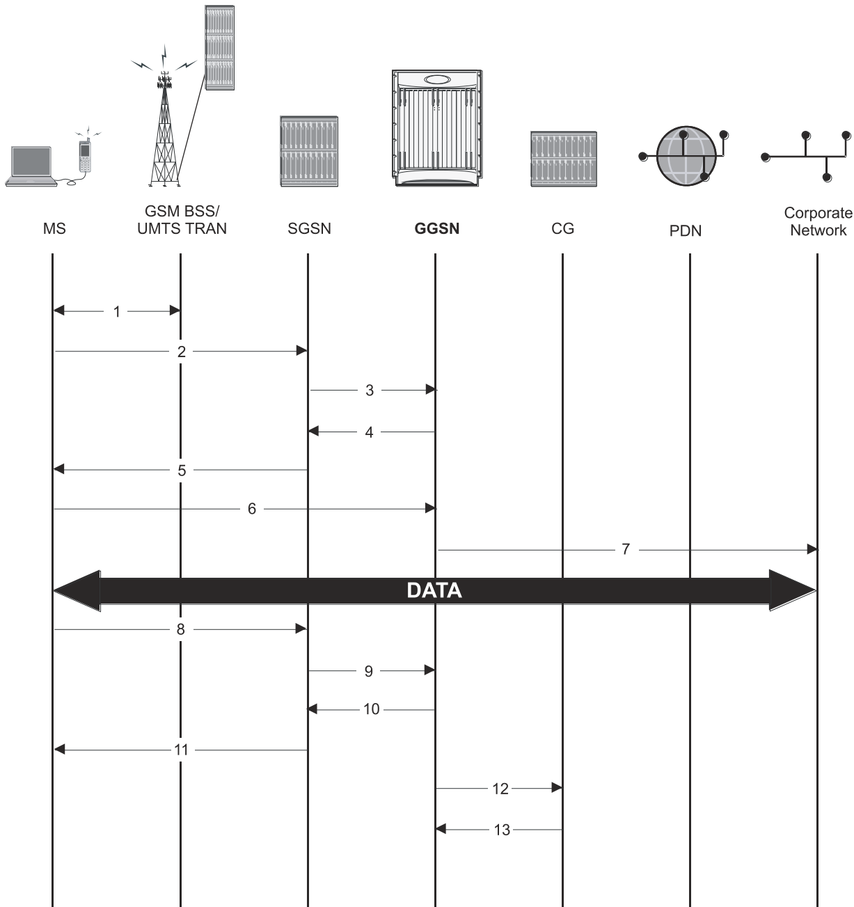
Figure 94. Corporate IP VPN Connectivity Call Flow
