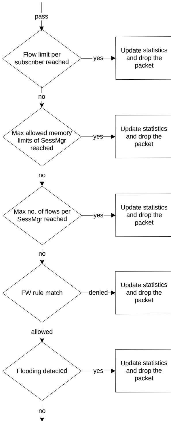
Figure 200. Continued... Stateful Firewall Processing
