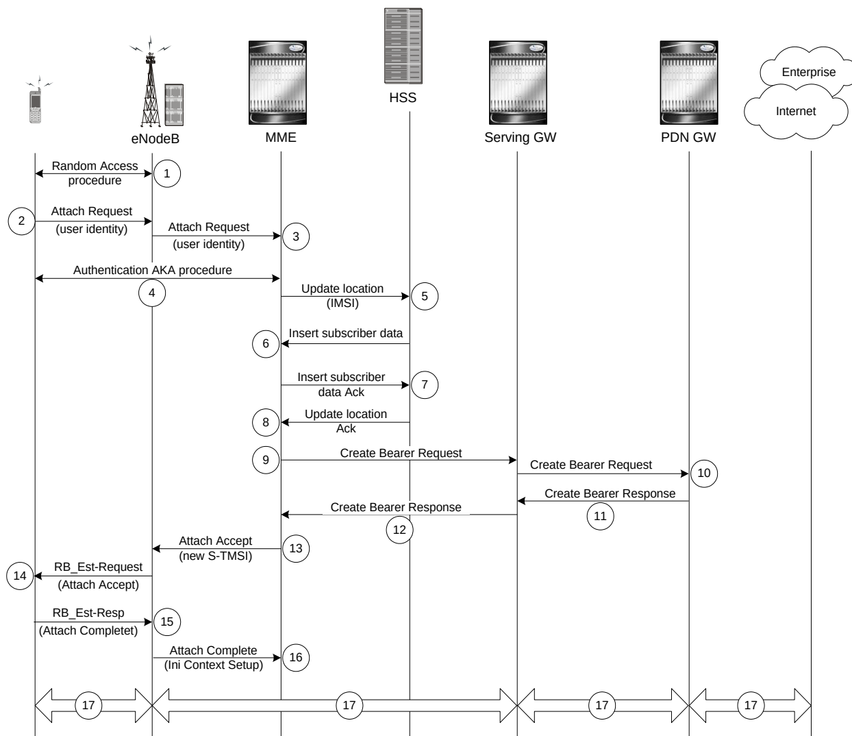
Figure 194. Subscriber Registration Setup Message Flow
