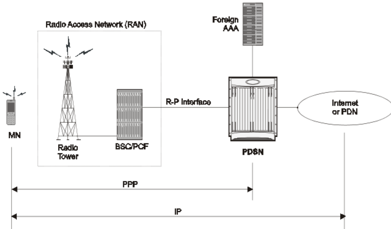
Figure 73. Simple IP Protocol Usage
