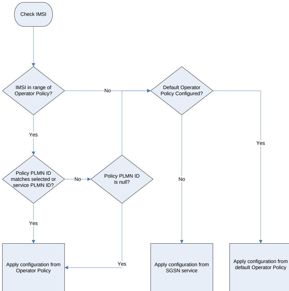
Figure 165. Logic Diagram for Policy Selection
