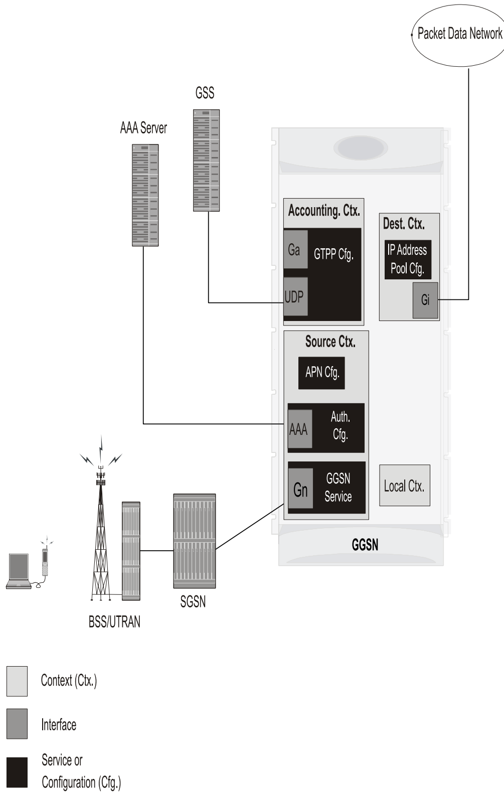
Figure 204. GGSN Contexts and Interfaces
