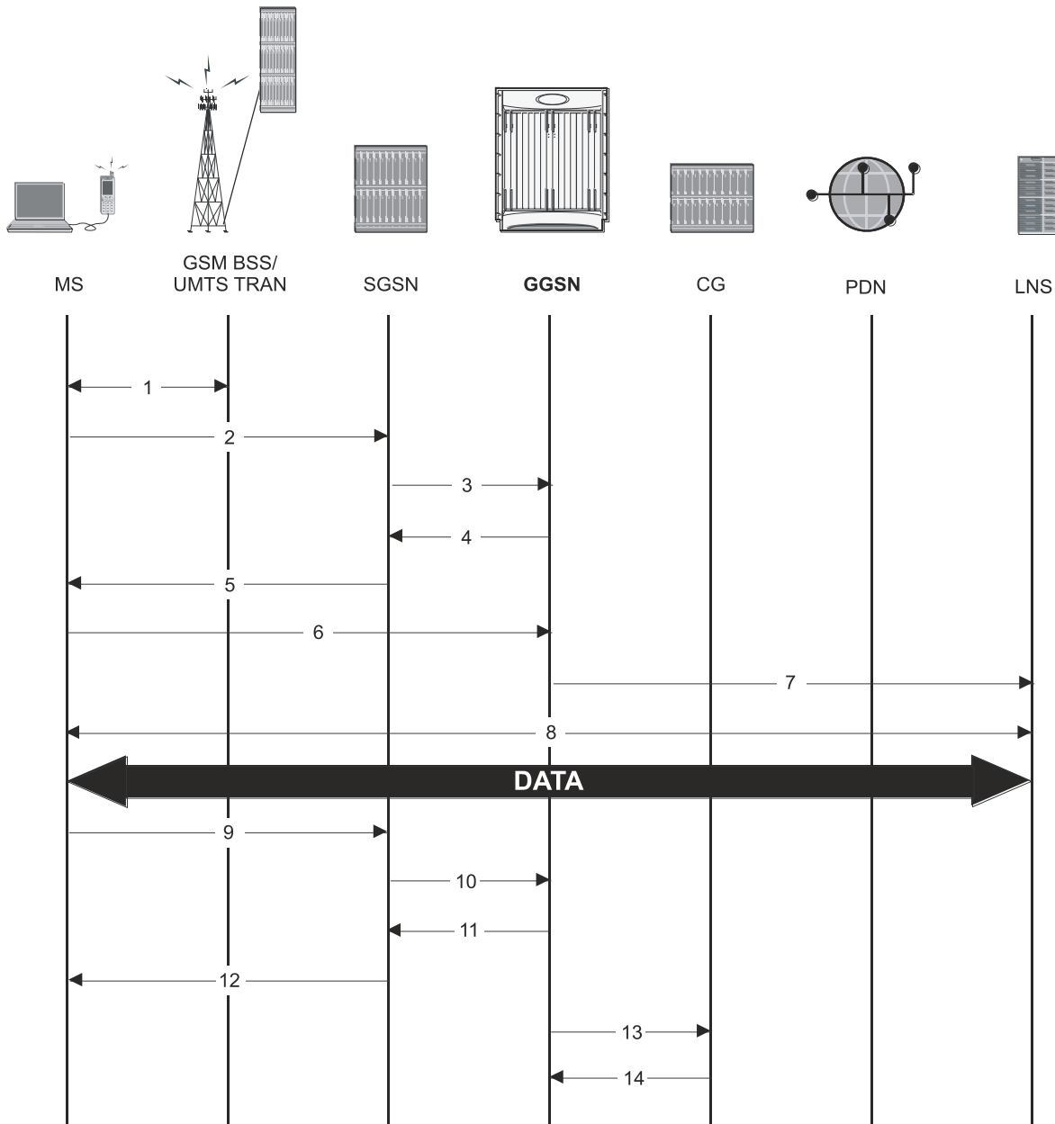
Figure 93. Virtual Dialup Access Call Flow
