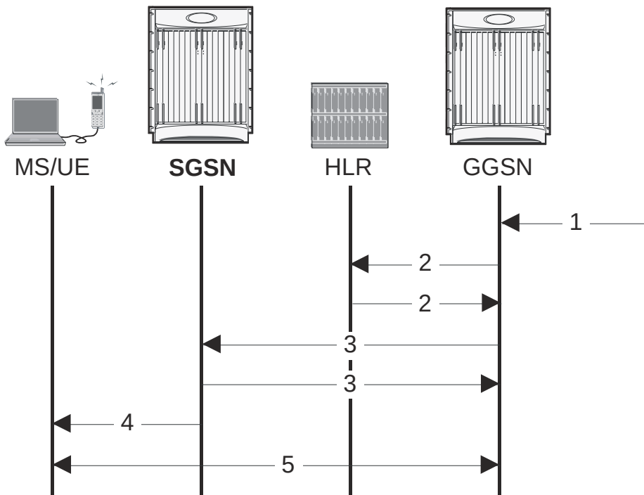
Figure 170. Network-Initiated PDP Context Activation
