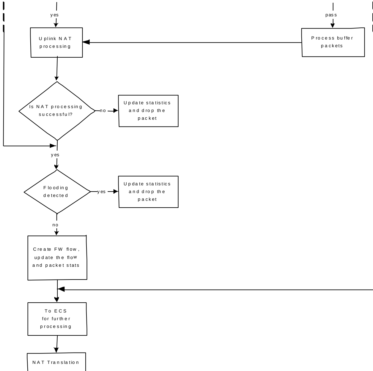
Figure 214. ... NAT Processing Flow
