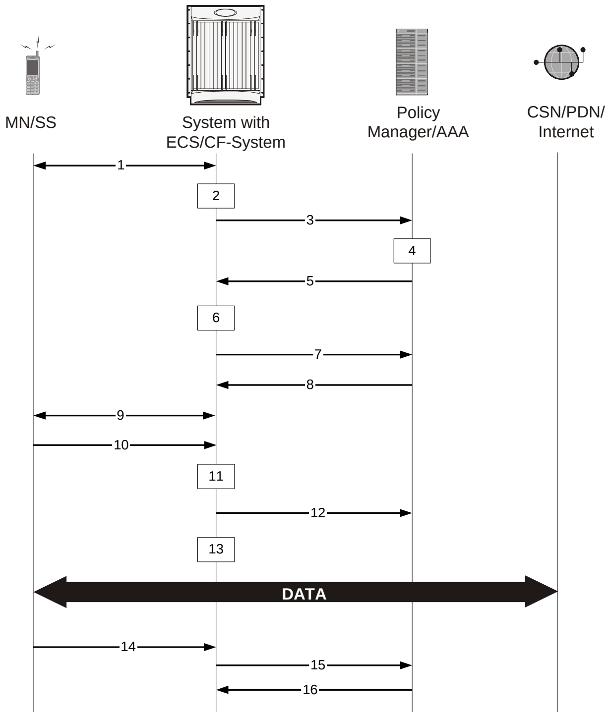
Figure 174. Content Filtering Call Flow
