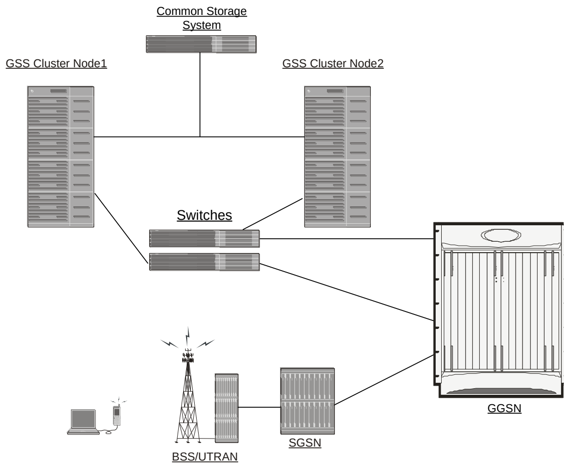
Figure 205. GSS Cluster Nodes in a GPRS/UMTS Network
