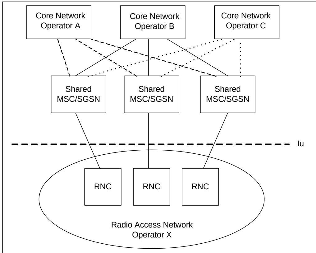
Figure 162. GWCN-type Network Sharing
