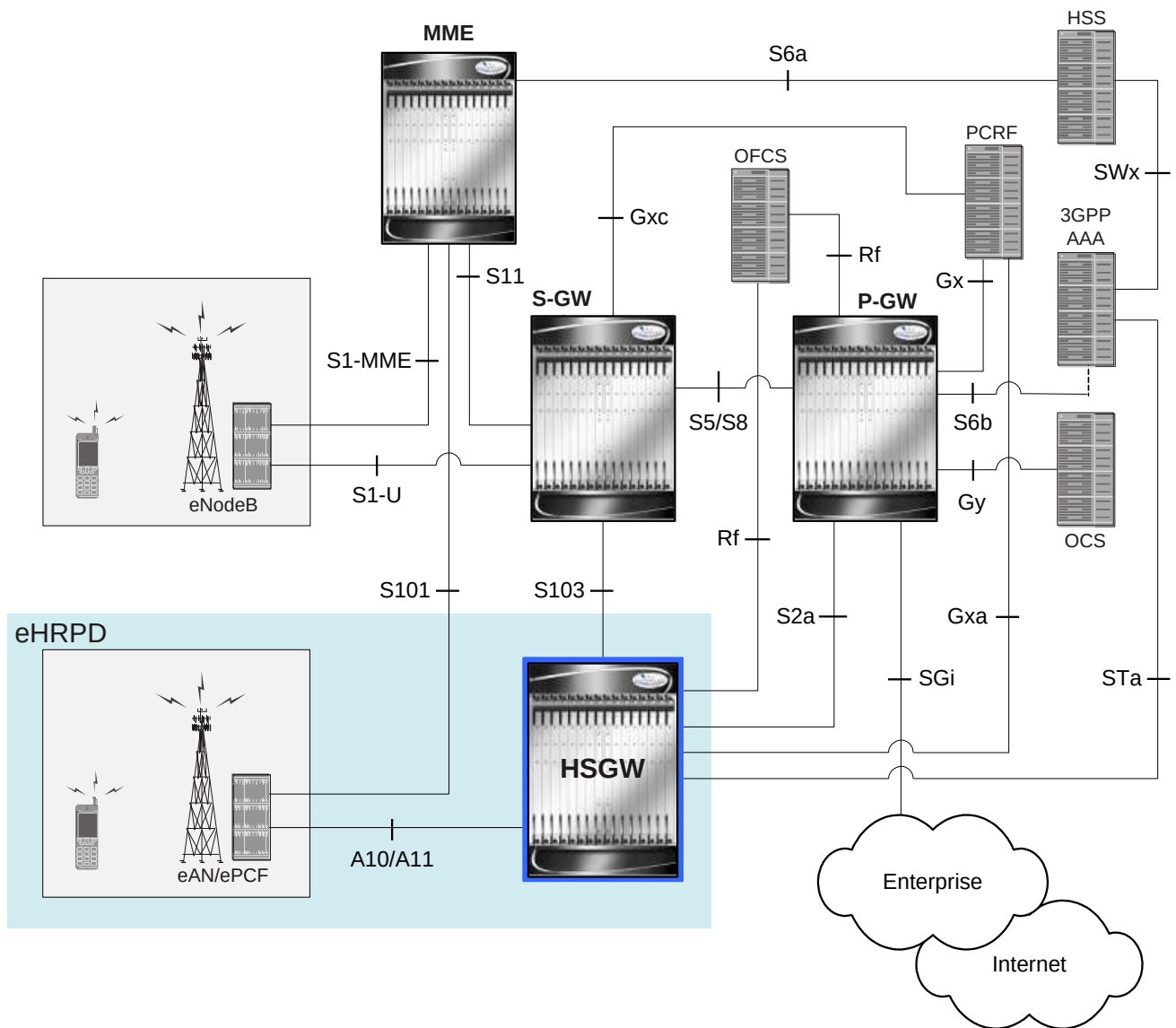
Figure 103. eHRPD Basic Network Topology
