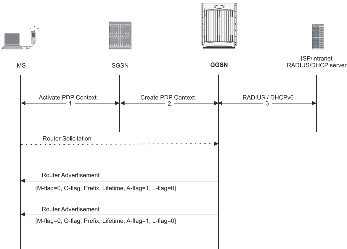
Figure 97. IPv6 Stateless Address Autoconfiguration Flow
