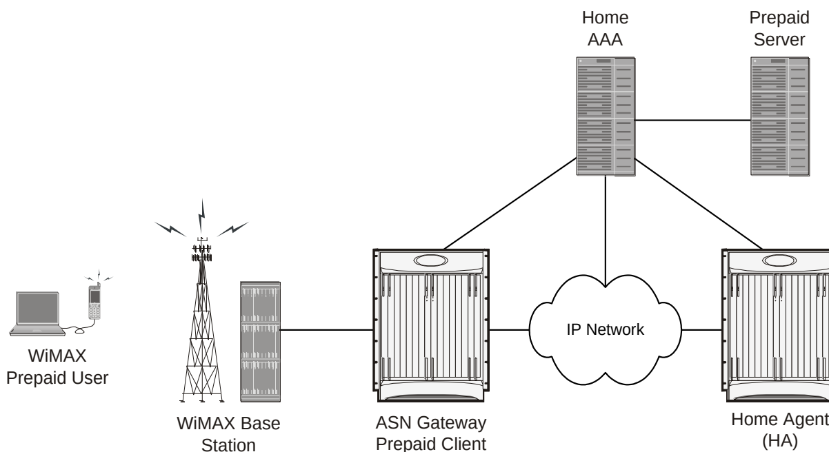
Figure 37. Prepaid Network Topology
