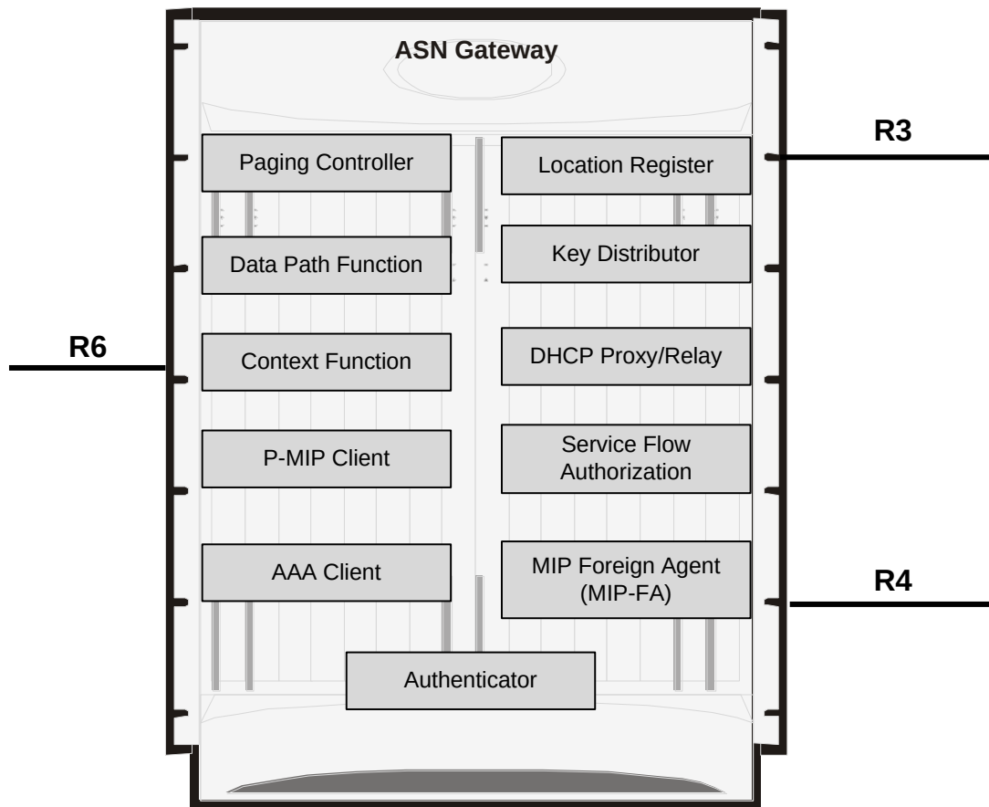
Figure 41. Functional view of ASN Gateway Profile-C
