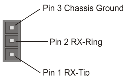
Figure 225. SPIO T1 BITS Timing Wire-Wrap Pin-out
