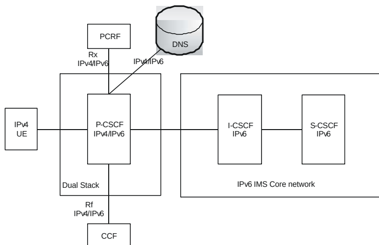
Figure 149. Interworking Between IPv4 UE and IPv6 IMS Core Network
