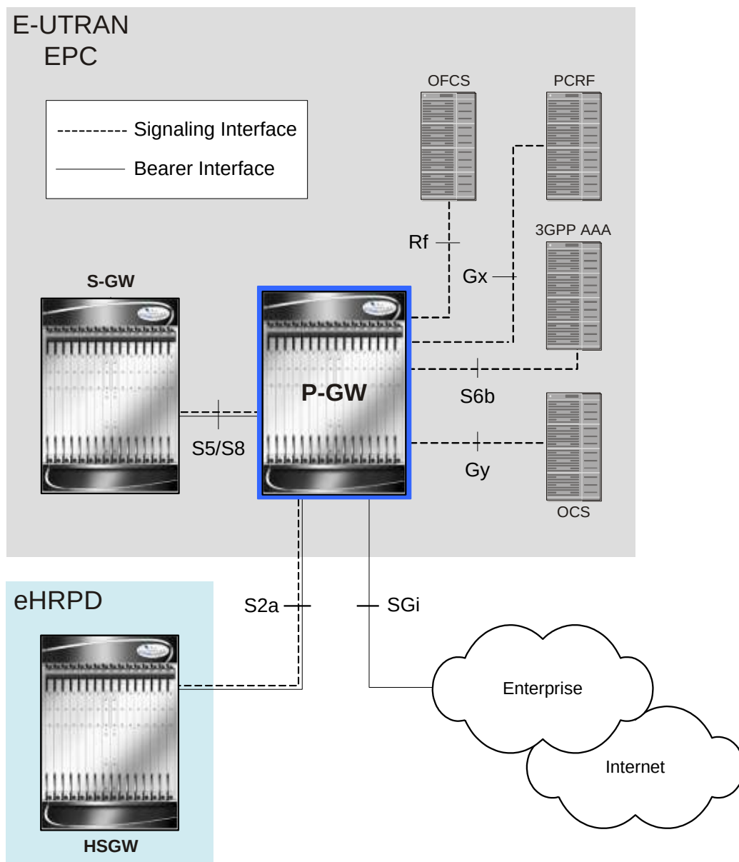
Figure 130. P-GW Interfaces Supporting eHRPD to E-UTRAN/EPC Connectivity
