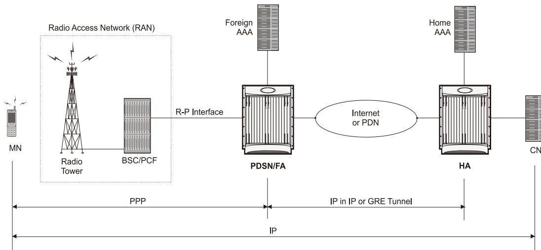
Figure 76. Mobile IP Protocol Usage
