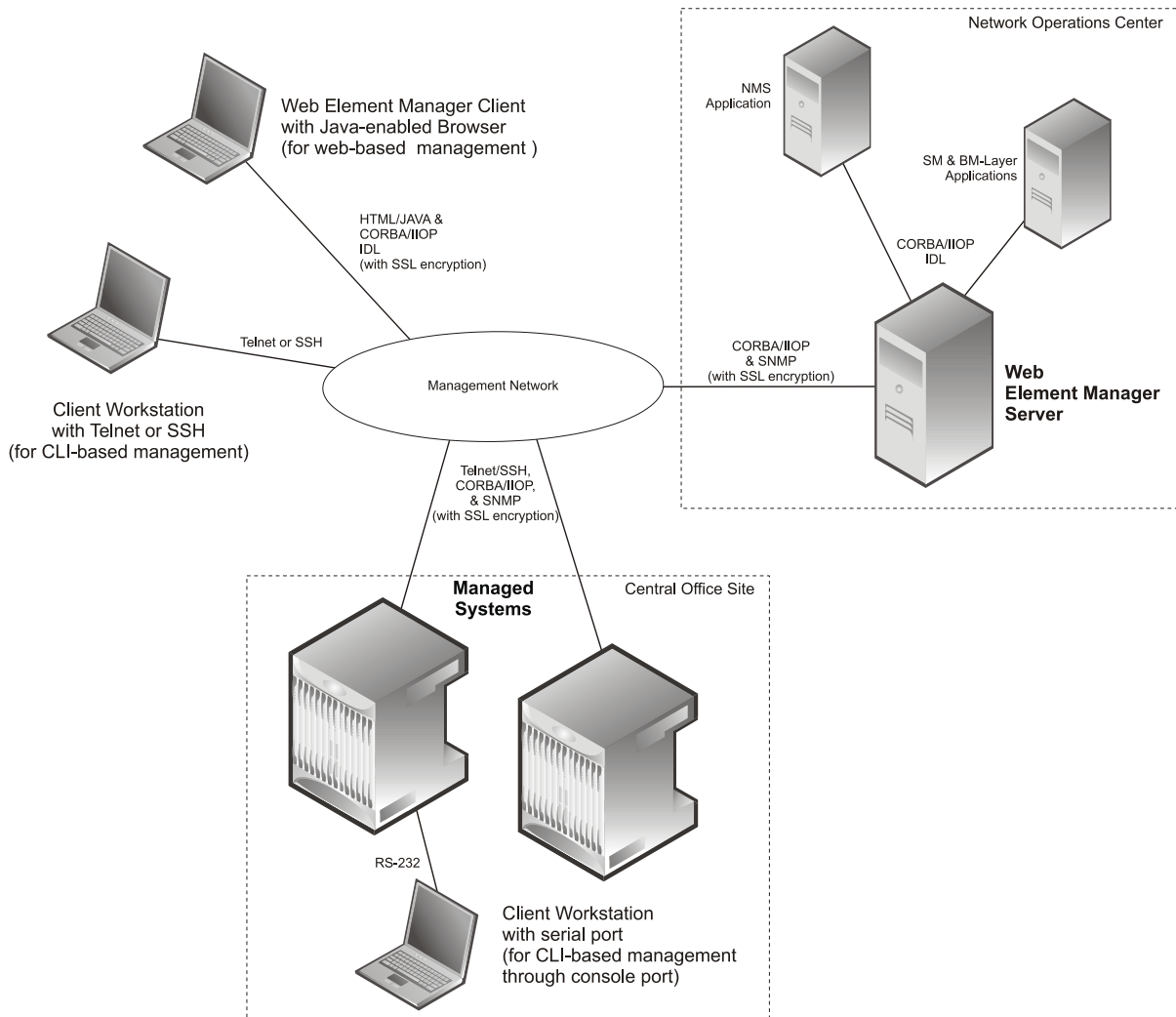
Figure 193. Element Management Methods
