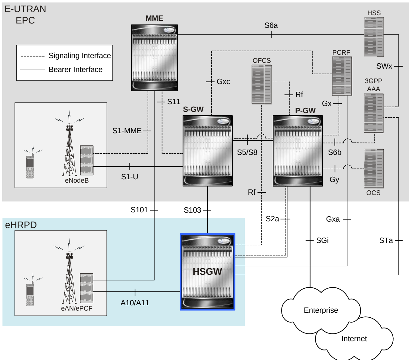
Figure 104. HSGW in an eHRPD Network Architecture
