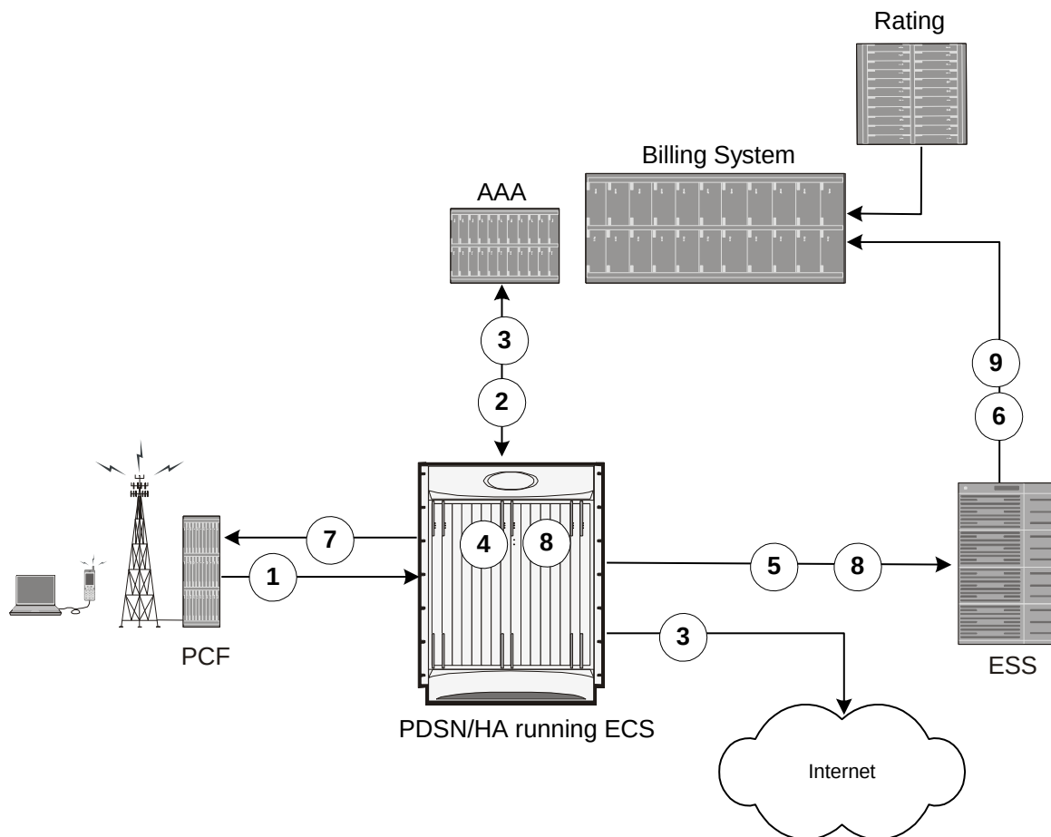
Figure 187. Postpaid Billing with ECS in CDMA-2000 Network
