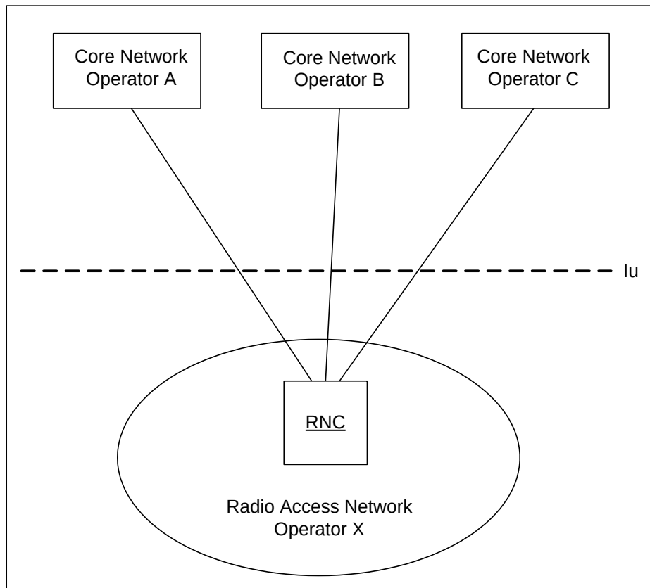
Figure 163. MOCN-type Network Sharing
