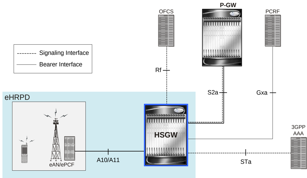
Figure 105. HSGW Supported Network Interfaces
