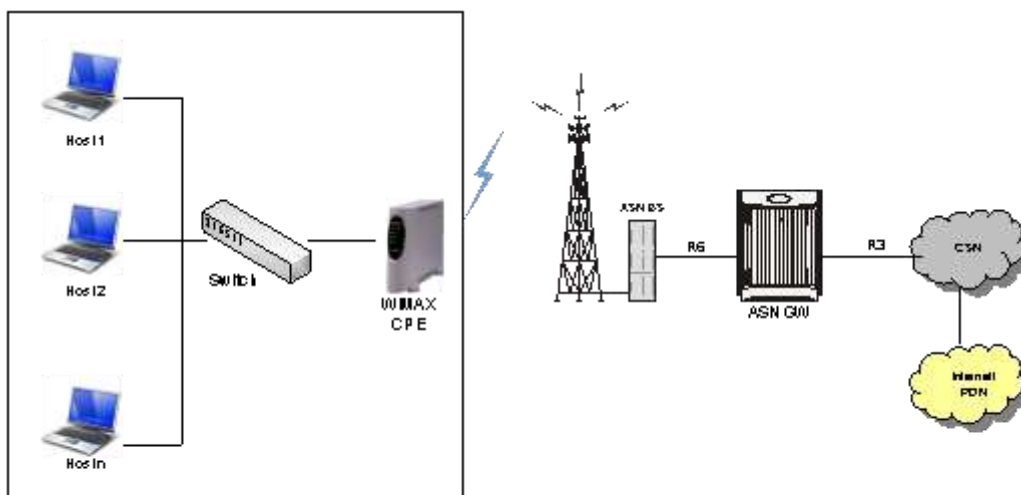
Figure 38. Multi Host Support in WiMAX Network
