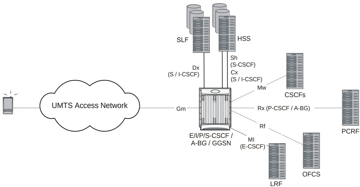
Figure 146. GSM/UMTS CSCF/A-BG/GGSN SCM Deployment Example
