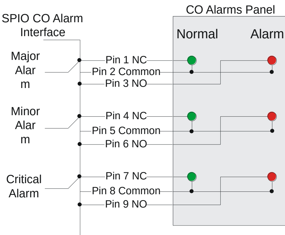
Figure 223. CO Alarm Wiring Example
