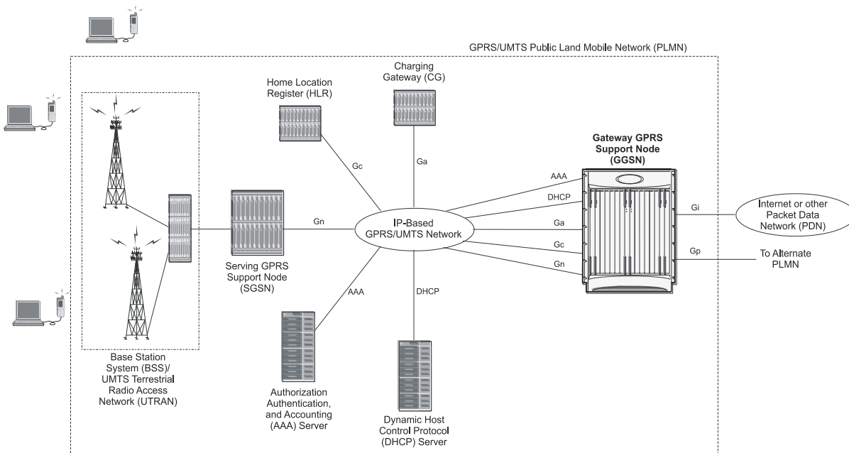
Figure 80. Basic GPRS/UMTS Network Topology
