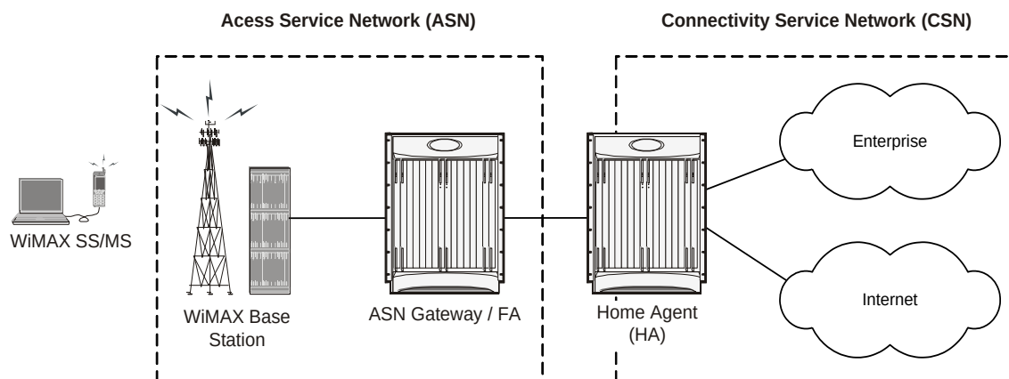
Figure 36. Basic ASN Gateway Mobile IP Network
