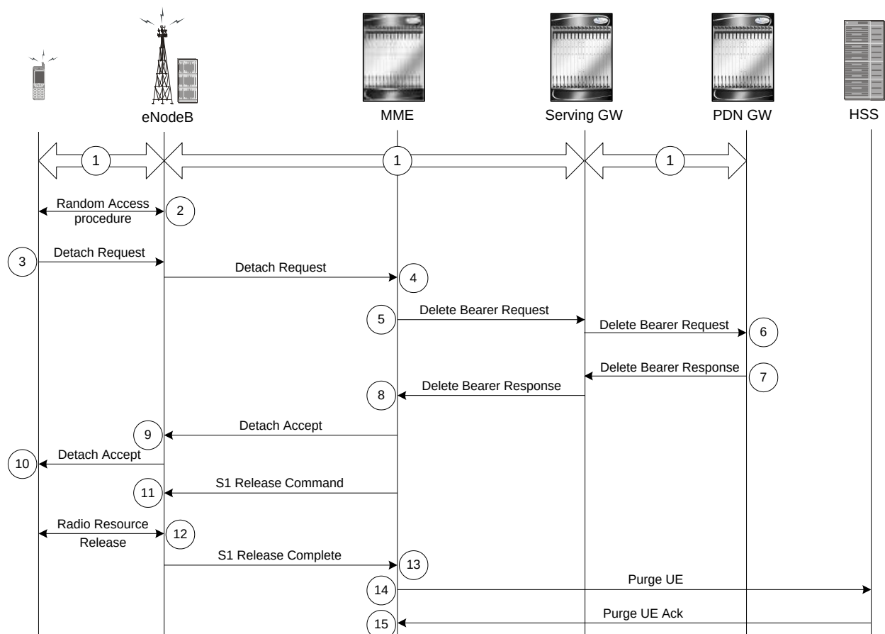
Figure 195. Subscriber De-registration Setup Message Flow
