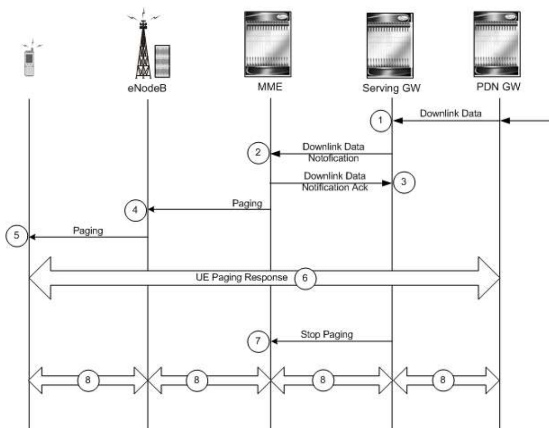
Figure 197. Network-initiated Service Request Message Flow
