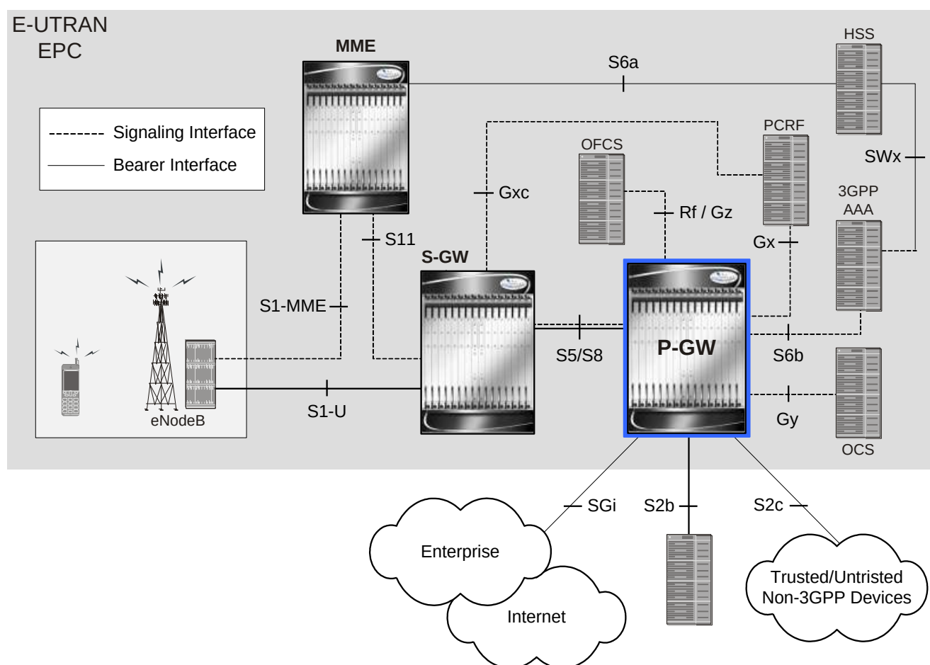
Figure 131. P-GW in the E-UTRAN/EPC Network
