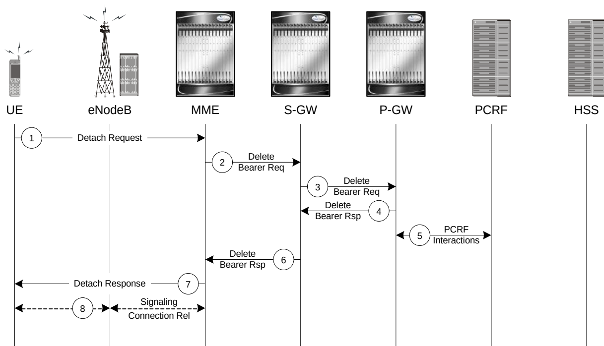
Figure 159. Subscriber-initiated Detach Call Flow
