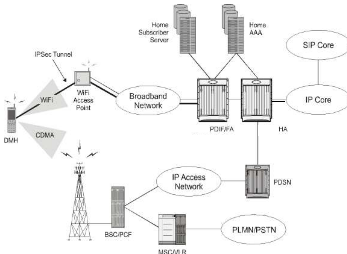
Figure 118. PDIF/FA Mobile IP Implementation
