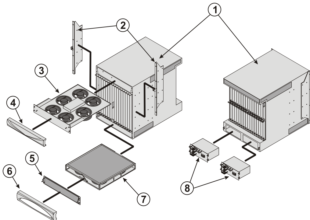
Figure 5. Chassis Components (front and rear views)
