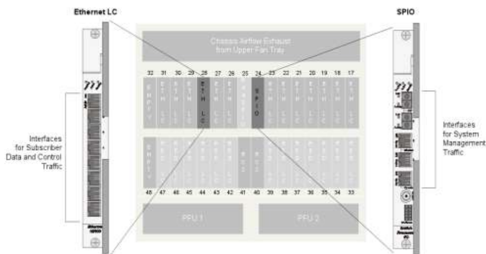
Figure 33. Separation of Management Data From User Data
