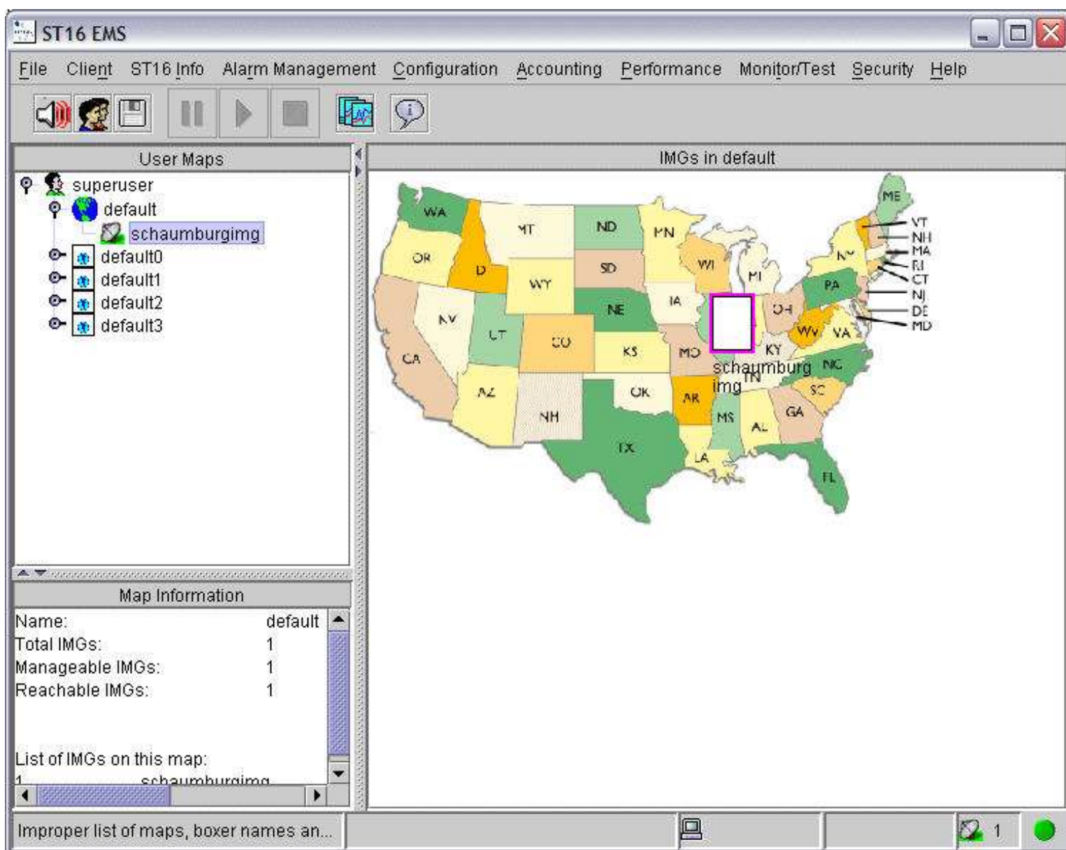
Figure 34. Web Element Manager Topology Window
