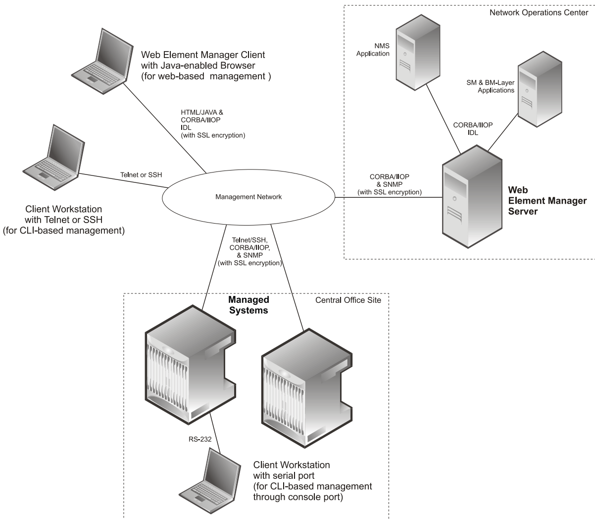
Figure 85. Element Management Methods
