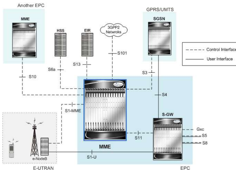
Figure 189. The MME in LTE/SAE Networks and Interfaces
