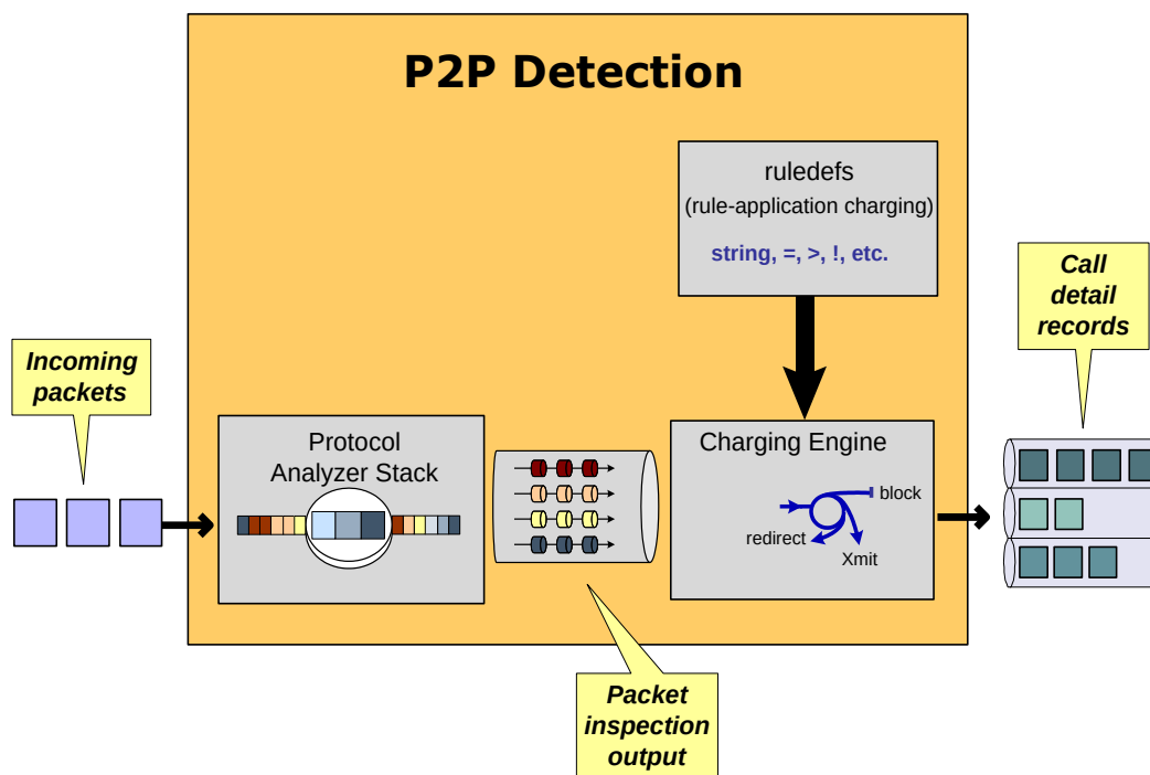
Figure 198. Overview of Packet Processing in ECSv2
