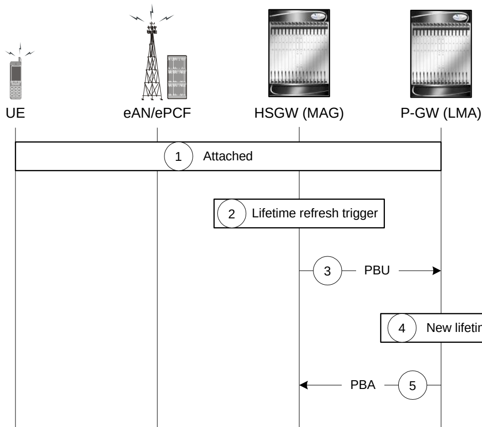
Figure 136. PMIPv6 Lifetime Extension (without handover) Call Flow
