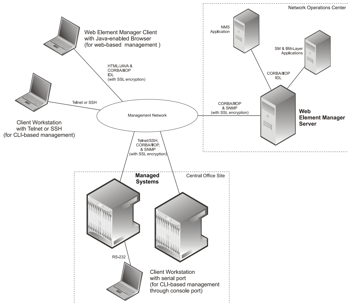
Figure 191. Element Management Methods
