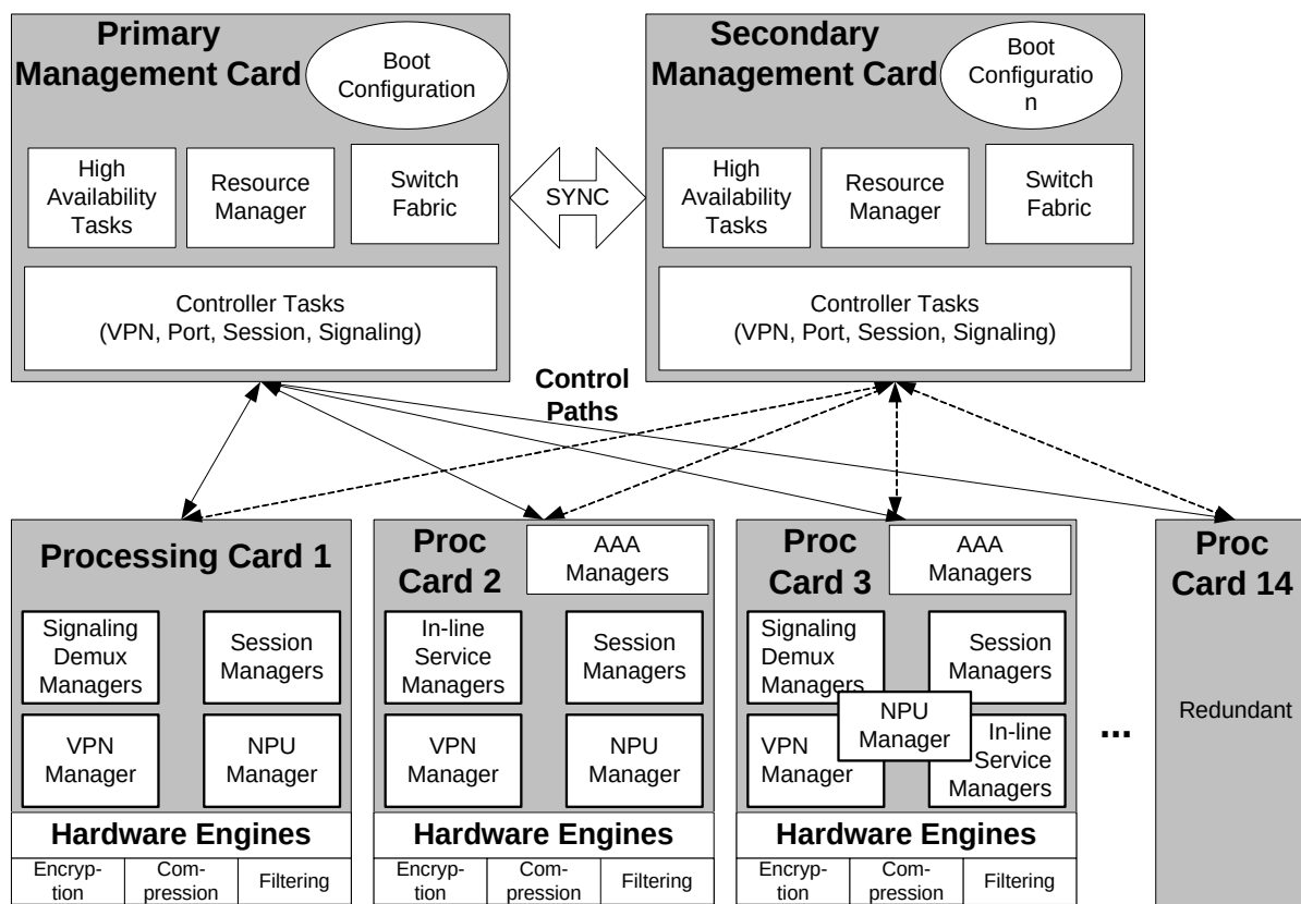
Figure 29. Software Architecture Block Diagram
