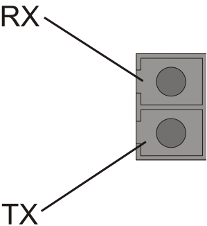
Figure 232. Optical ATM Line Card SM IR-1 SFP Pin-out
