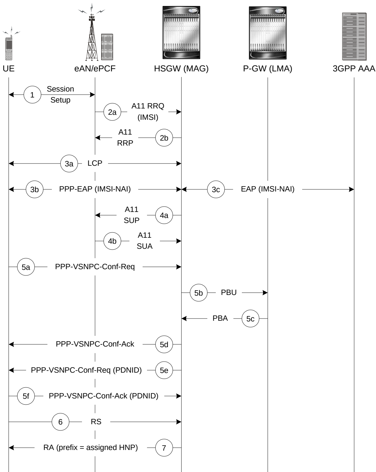
Figure 108. Initial Attach with IPv6/IPv4 Access Call Flow
