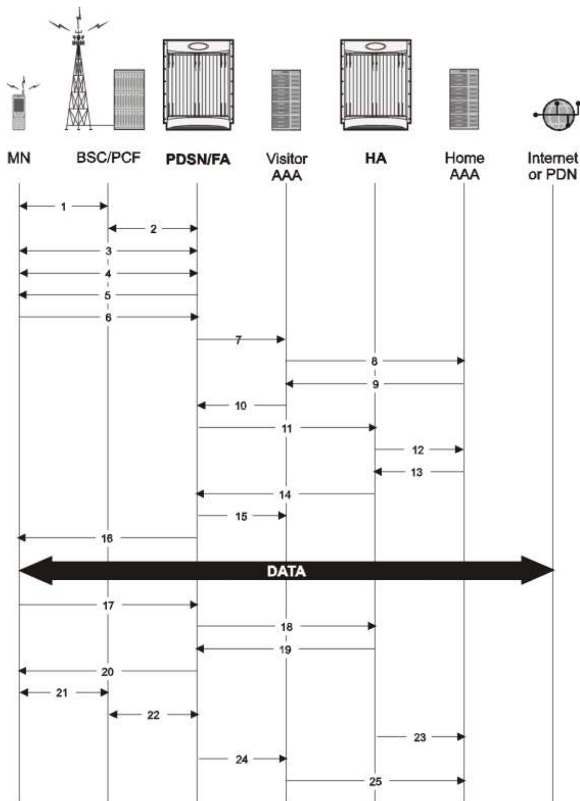
Figure 102. Mobile IP Call Flow
