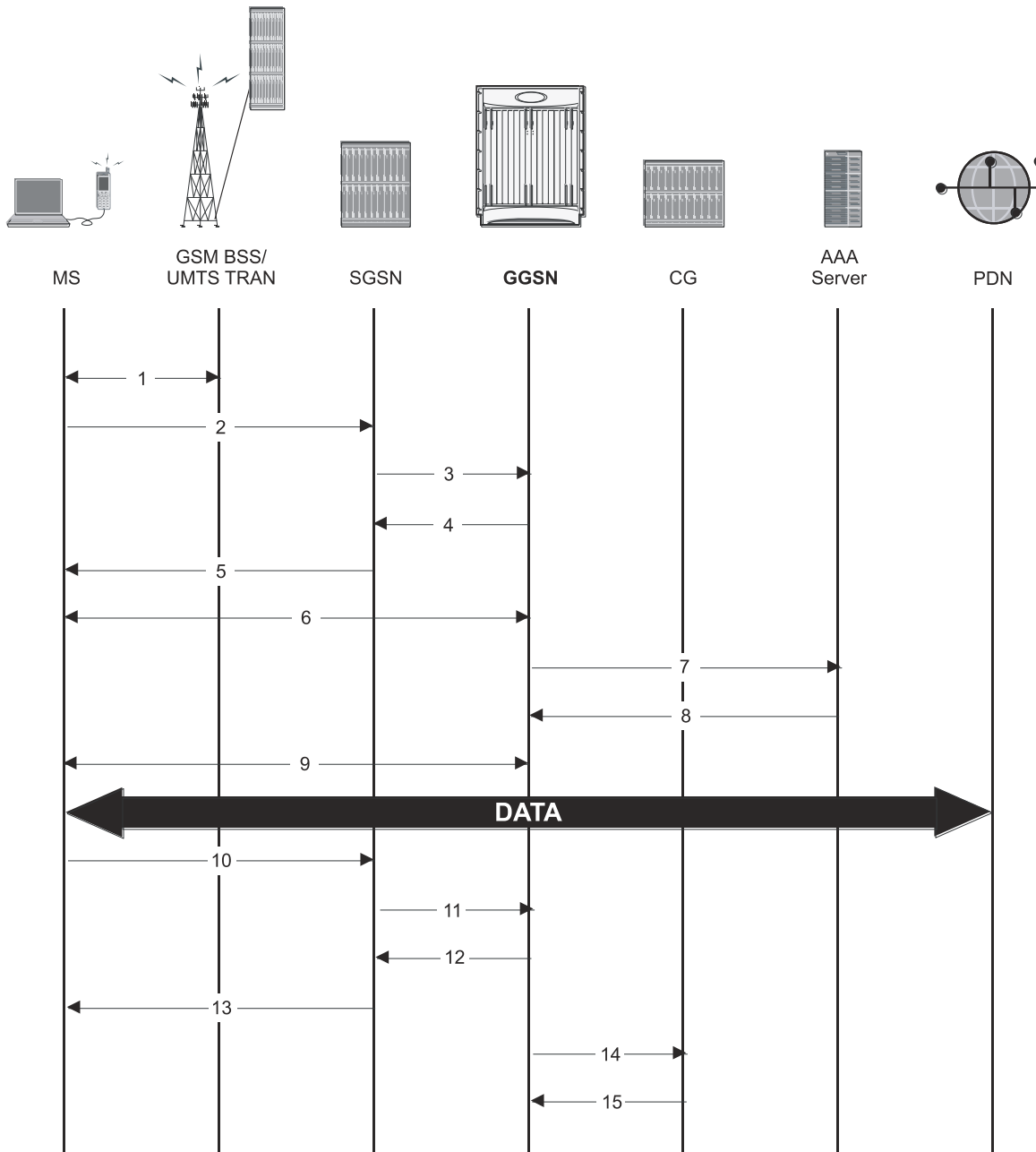
Figure 92. PPP Direct Access Call Flow
