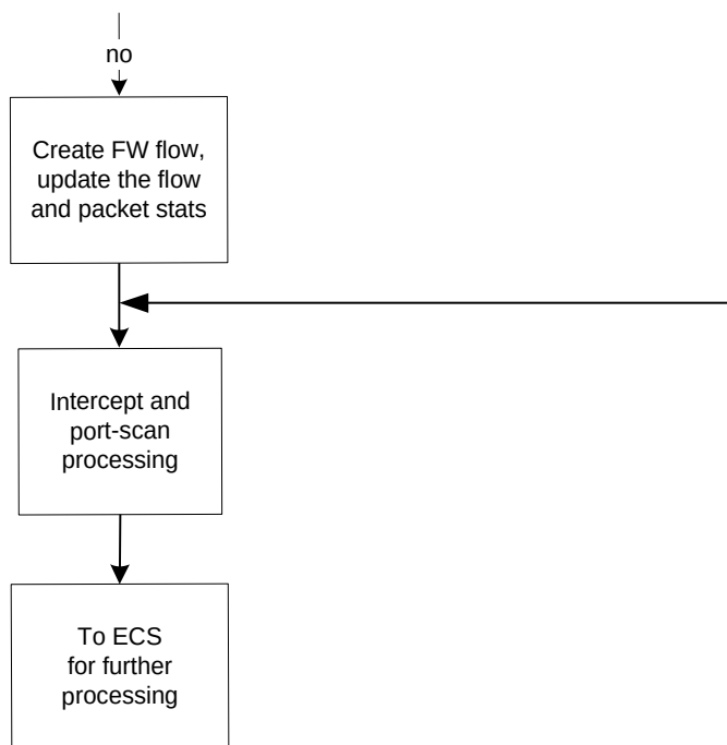
Figure 201. Continued... Stateful Firewall Processing
