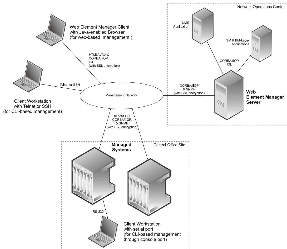
Figure 156. Element Management Methods
