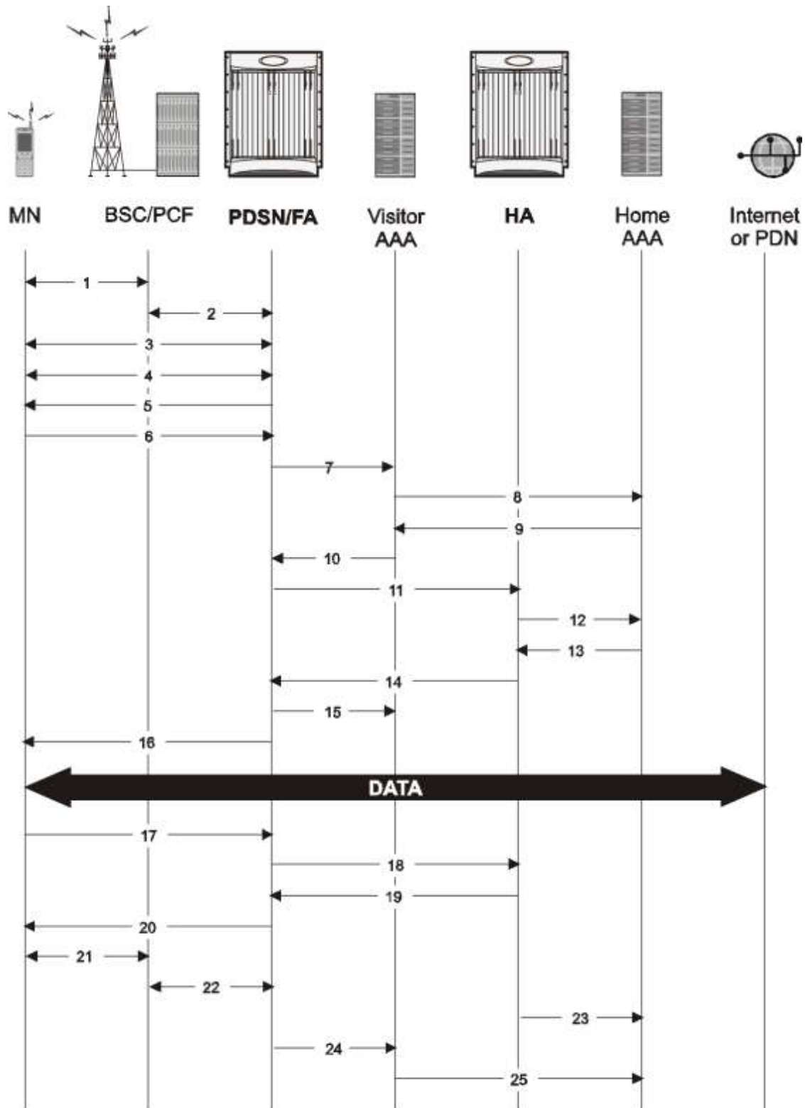
Figure 77. Mobile IP Call Flow
