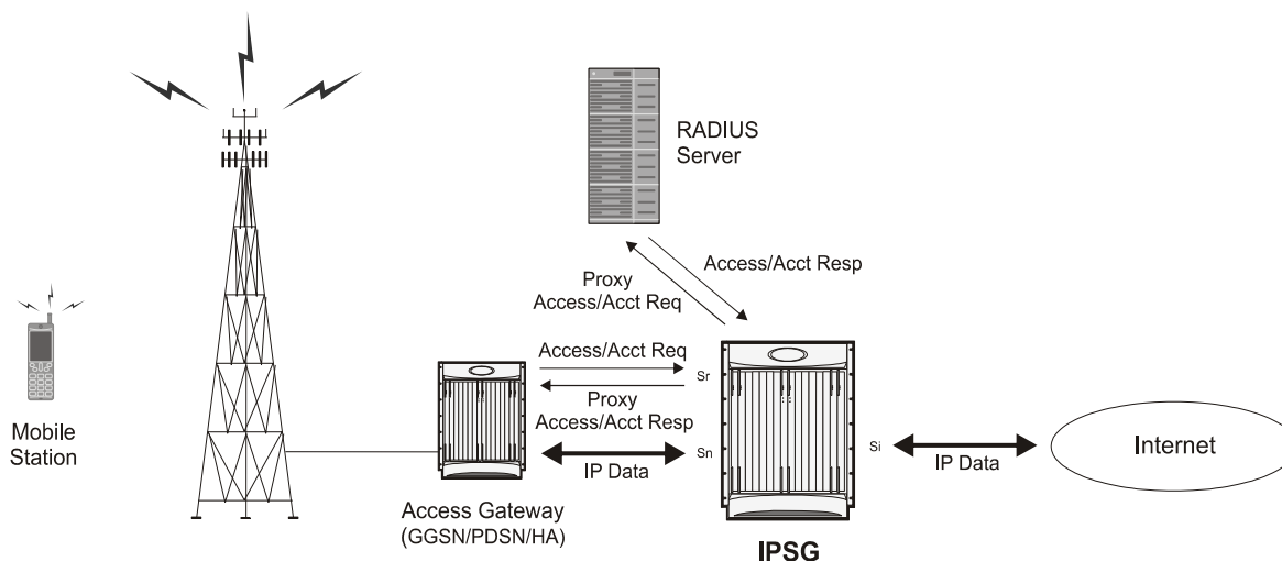
Figure 114. IPSG Message/Data Flow (RADIUS Server Mode - RADIUS Proxy)
