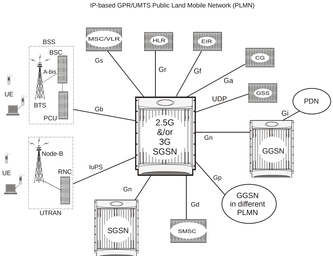
Figure 160. Dual Access 2.5G/3G SGSNs
