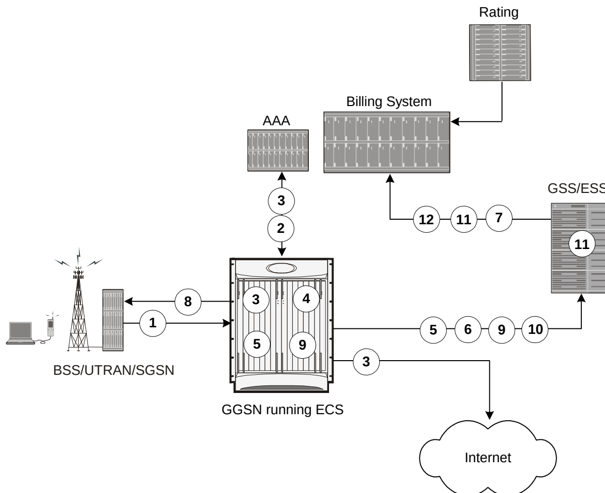
Figure 186. Postpaid Billing with ECS in GPRS/UMTS Network
