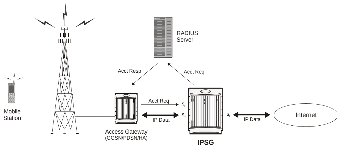
Figure 115. IPSG Message/Data Flow (RADIUS Snoop Mode)
