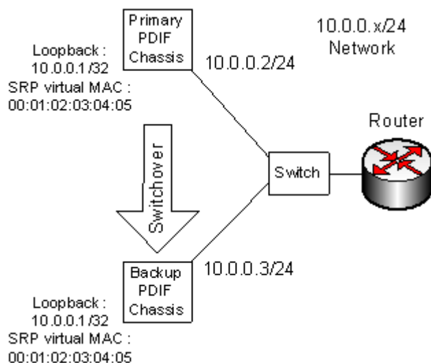
Figure 125. Switchover Example for Common IPv4 Subnet
