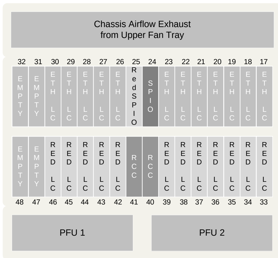
Figure 31. Recommended Redundant Configuration for Data Services - Rear View
