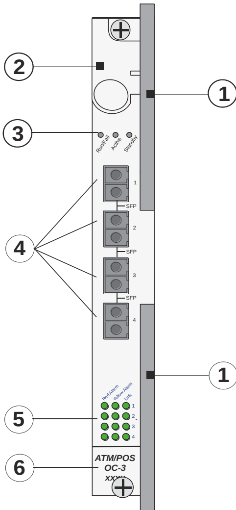
Figure 24. OLC Optical (ATM) Line Card
