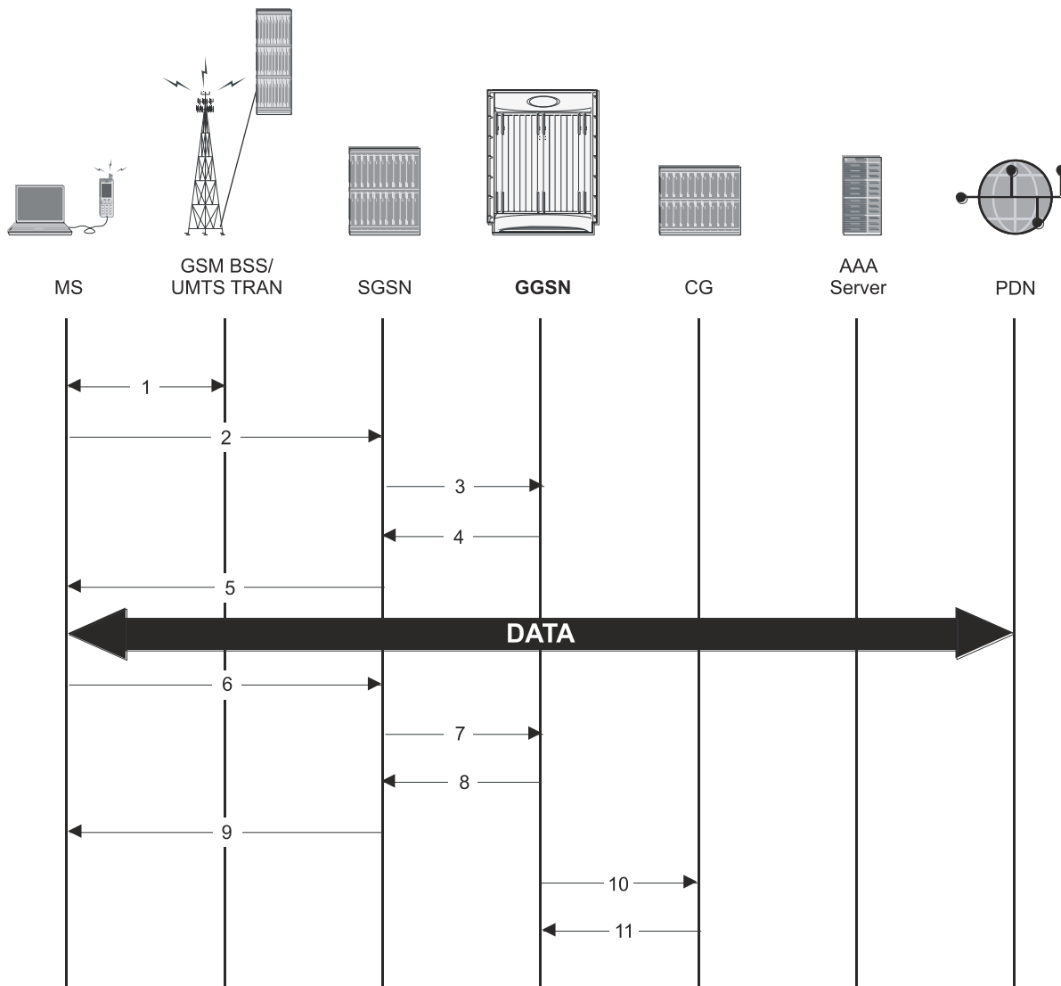
Figure 89. Transparent IP Session Call Flow
