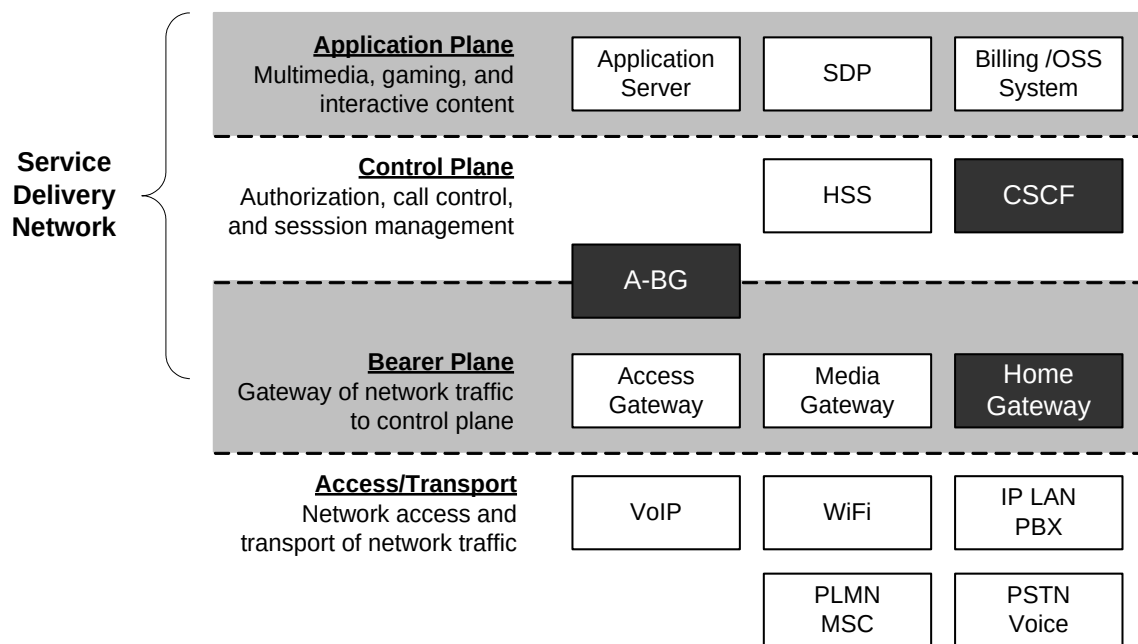
Figure 142. IMS Service Delivery Networks Components
