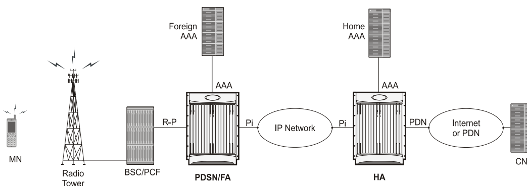
Figure 71. PDSN/FA and HA Network Deployment Configuration Example
