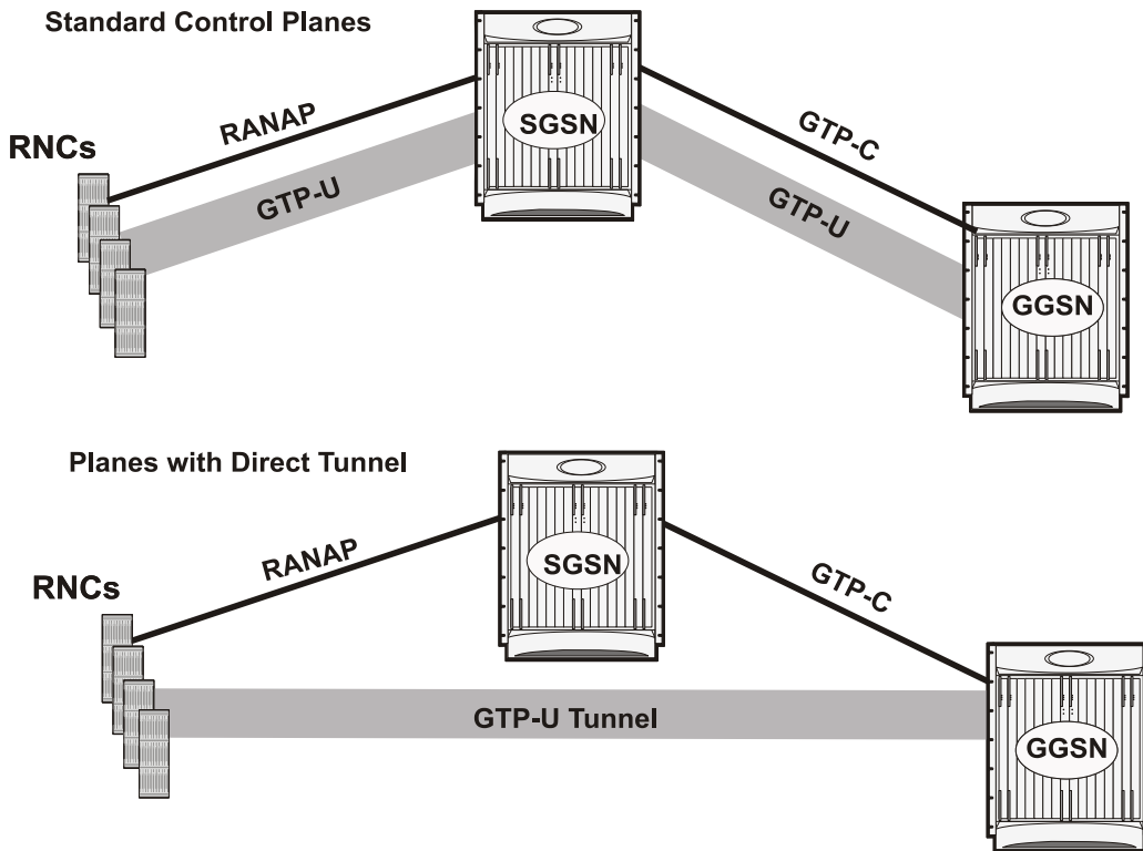
Figure 84. Direct Tunnel Support in GGSN
