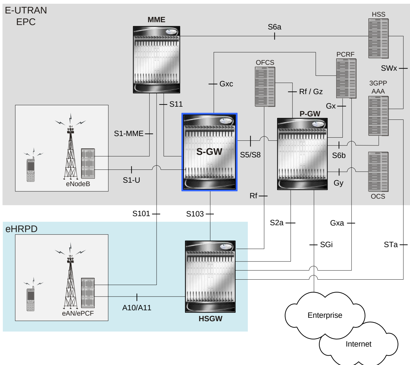
Figure 153. Basic E-UTRAN/EPC and eHRPD Network Topology
