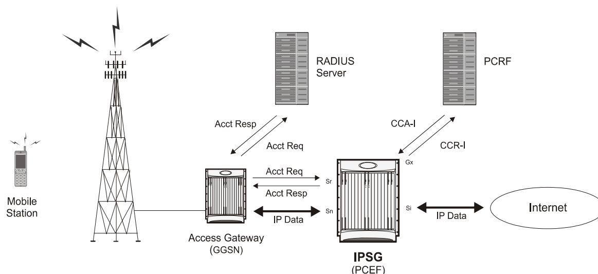
Figure 116. PSG Message/Data Flow (RADIUS Server Mode - IMS Auth Service)
