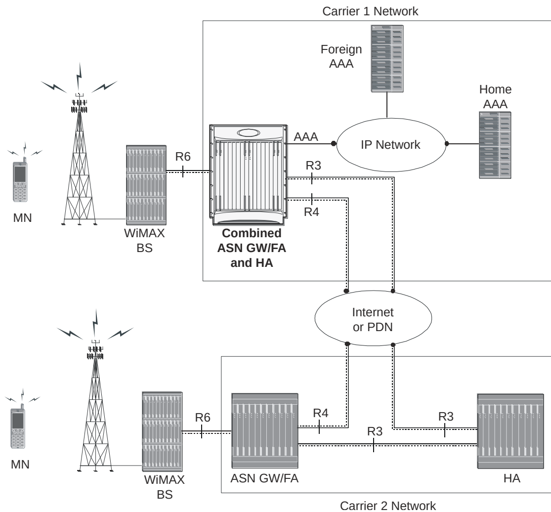
Figure 43. Co-located ASN Gateway/FA and HA Network Deployment Configuration Example
