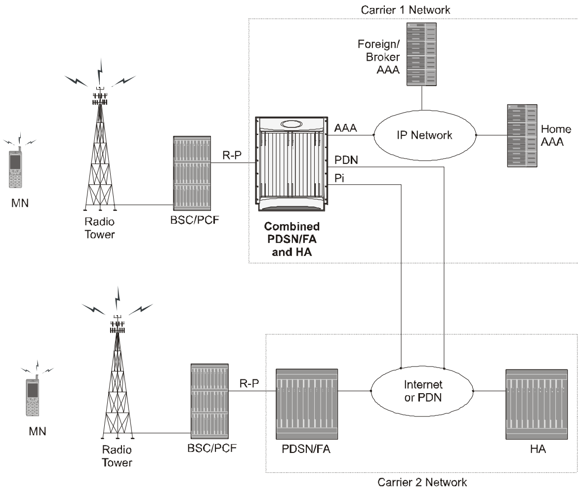
Figure 72. Co-located PDSN/FA and HA Configuration Example
