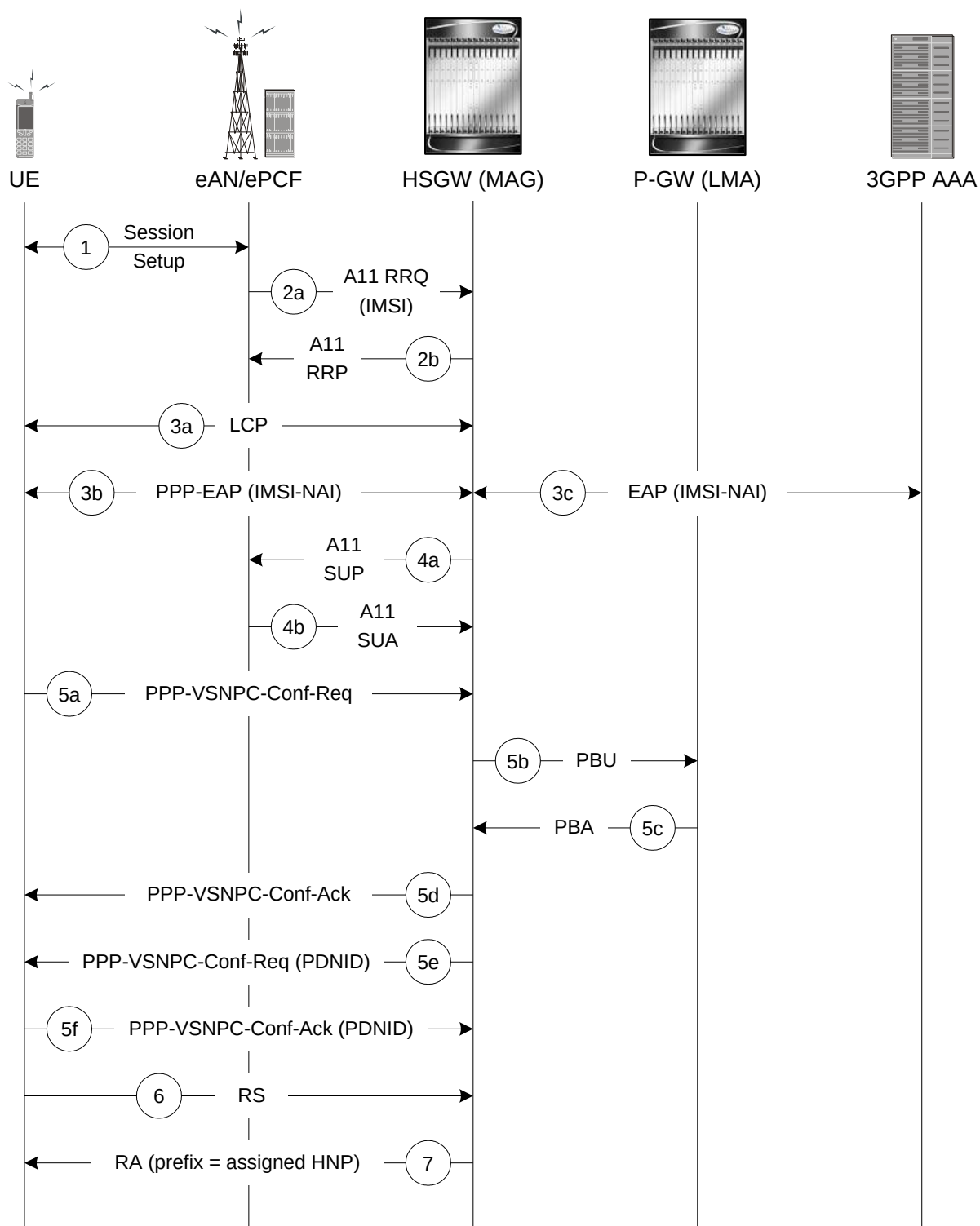
Figure 135. Initial Attach with IPv6/IPv4 Access Call Flow
