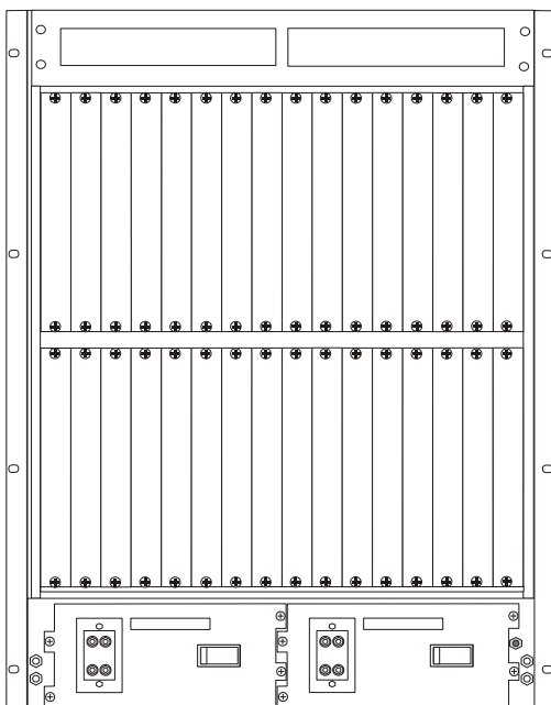
Figure 7. Rear Slot Numbering Scheme for Line Cards
