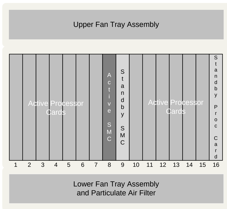
Figure 30. Recommended Redundant Configuration for Data Services - Front View
