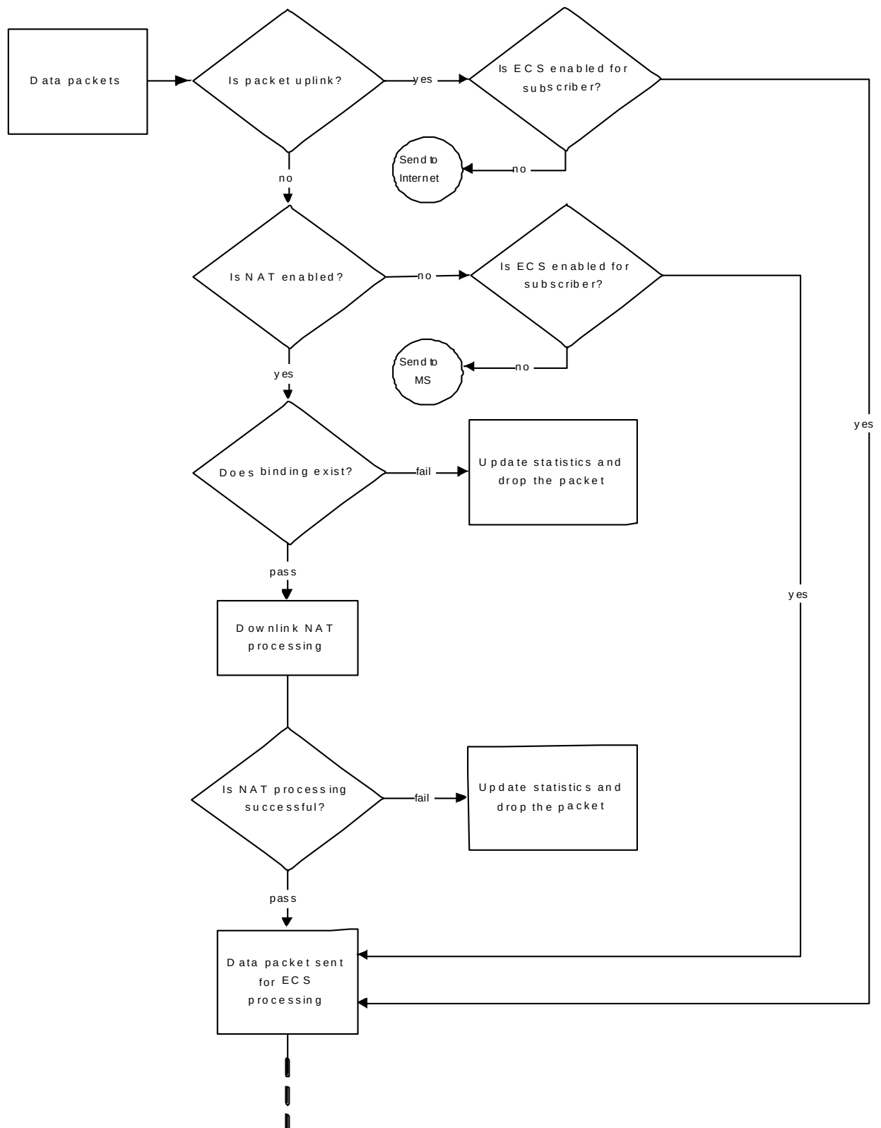
Figure 211. NAT Processing Flow
