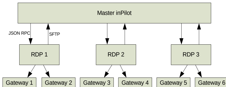
Figure 209. inPilot with RDPs in Distributed Model
