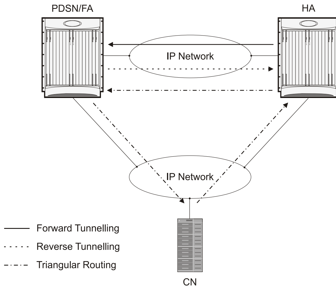
Figure 75. Mobile IP, FA and HA Tunneling/Transport Methods
