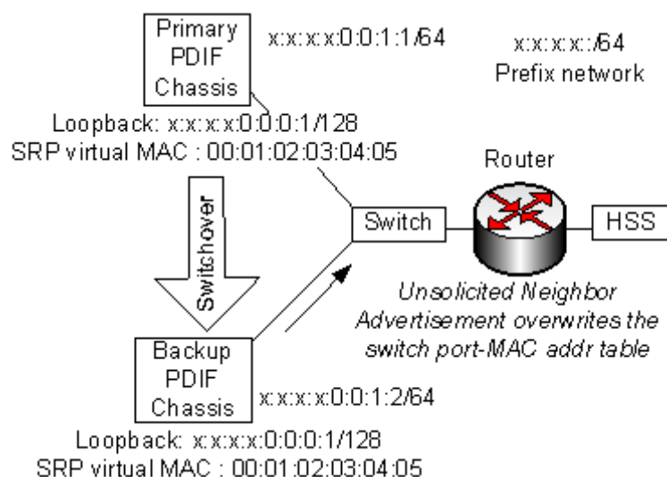
Figure 126. Switchover Example for a Common IPv6 Subnet
