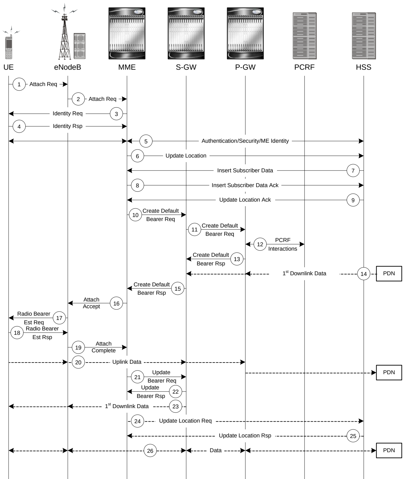
Figure 140. Subscriber-initiated Attach (initial) Call Flow
