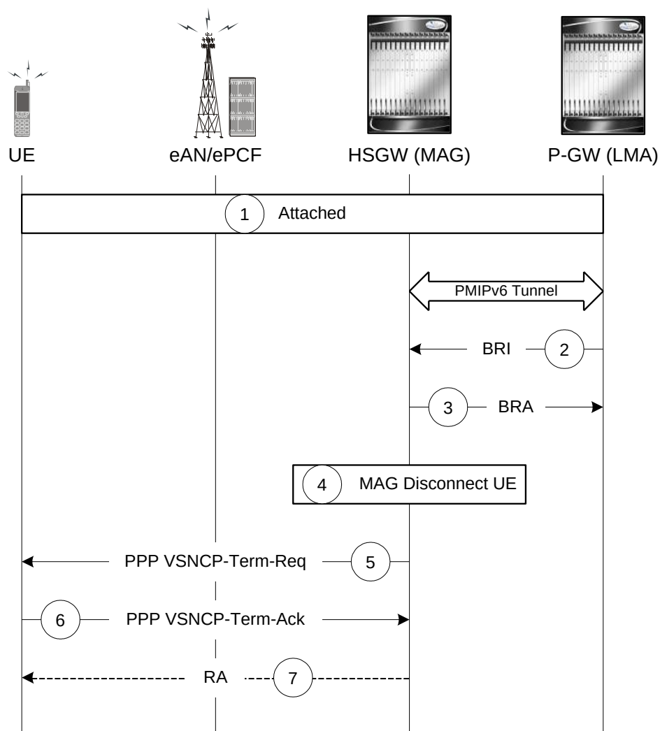
Figure 139. PDN Connection Release by the HSGW Call Flow
