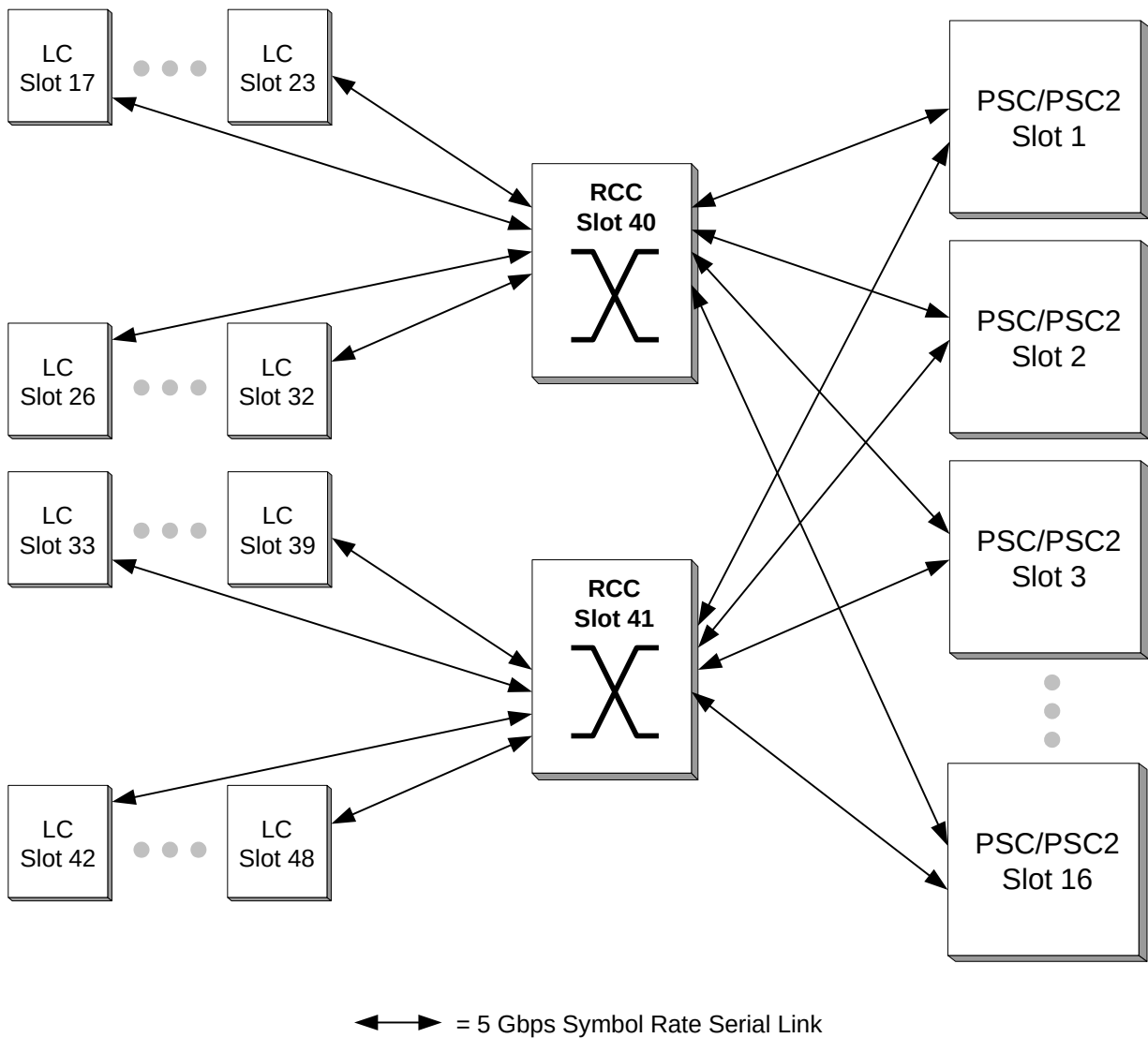
Figure 9. Logical View of RCC Links for Failover
