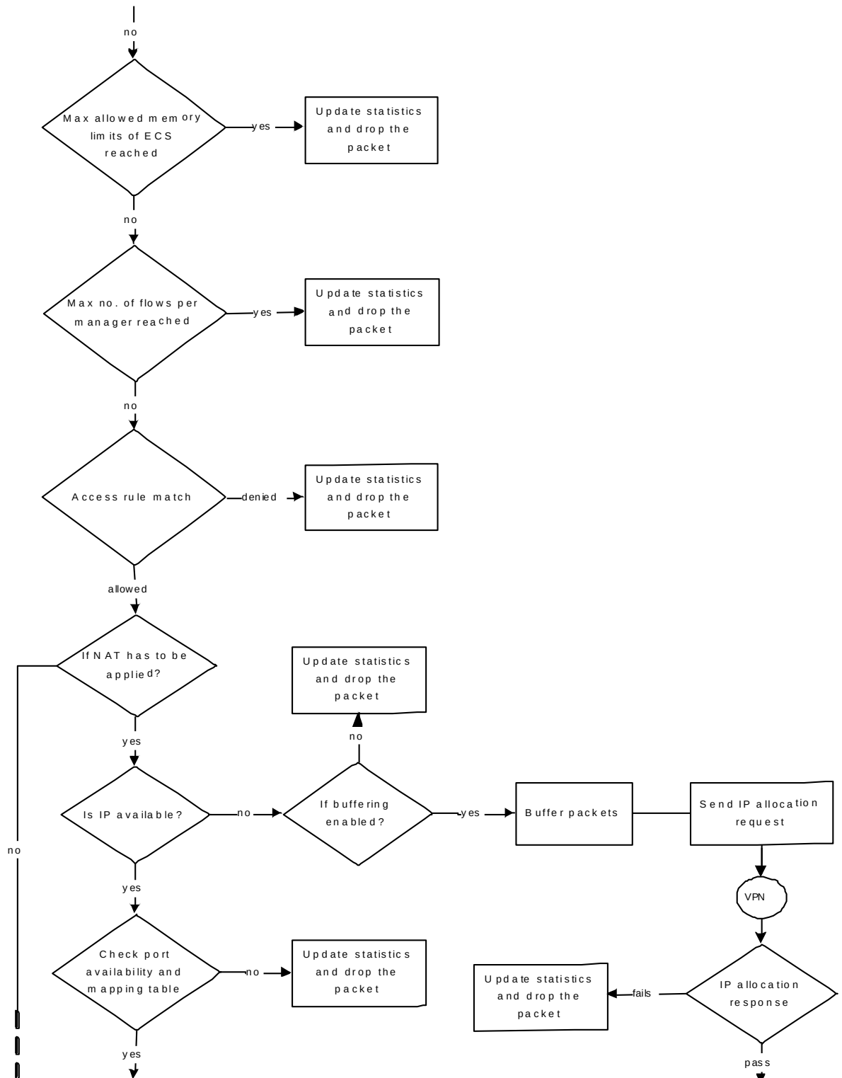
Figure 213. ... NAT Processing Flow
