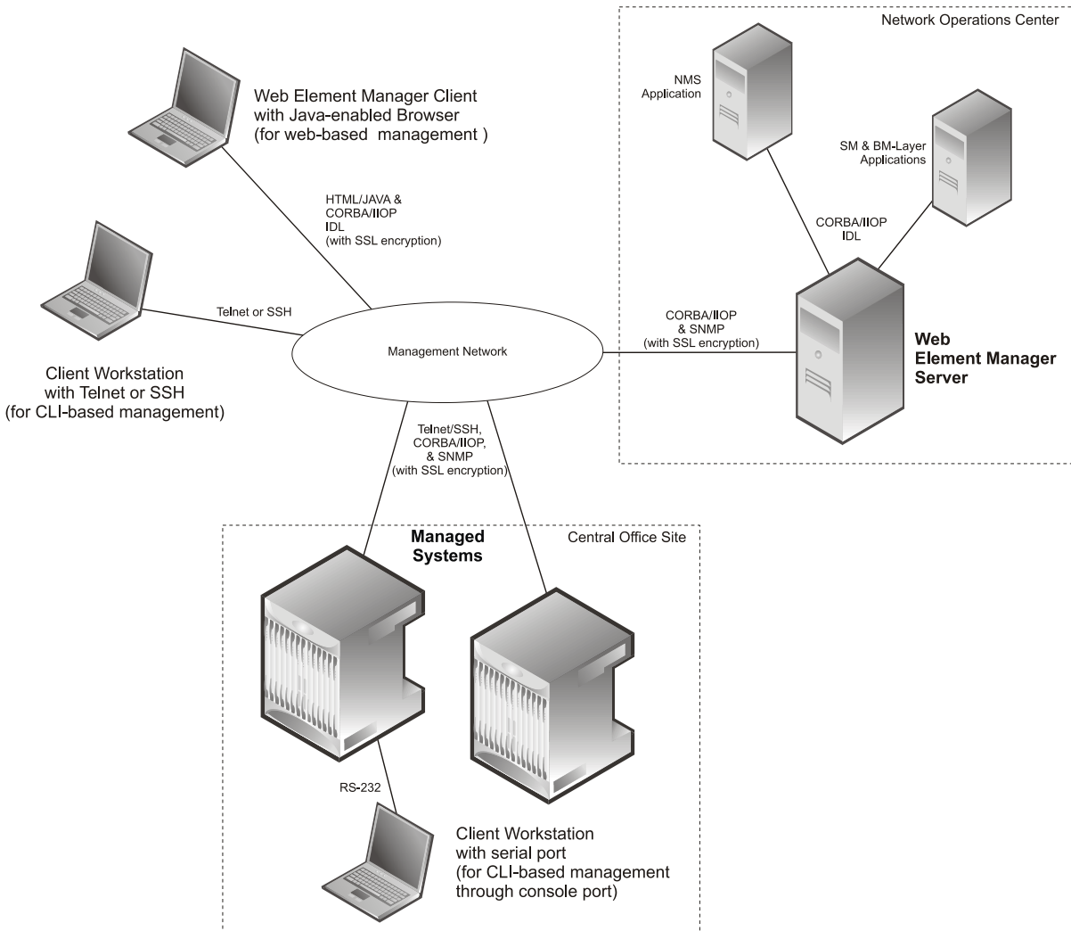
Figure 106. Element Management Methods
