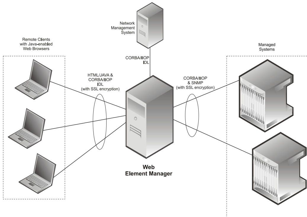
Figure 134. Web Element Manager Network Interfaces
