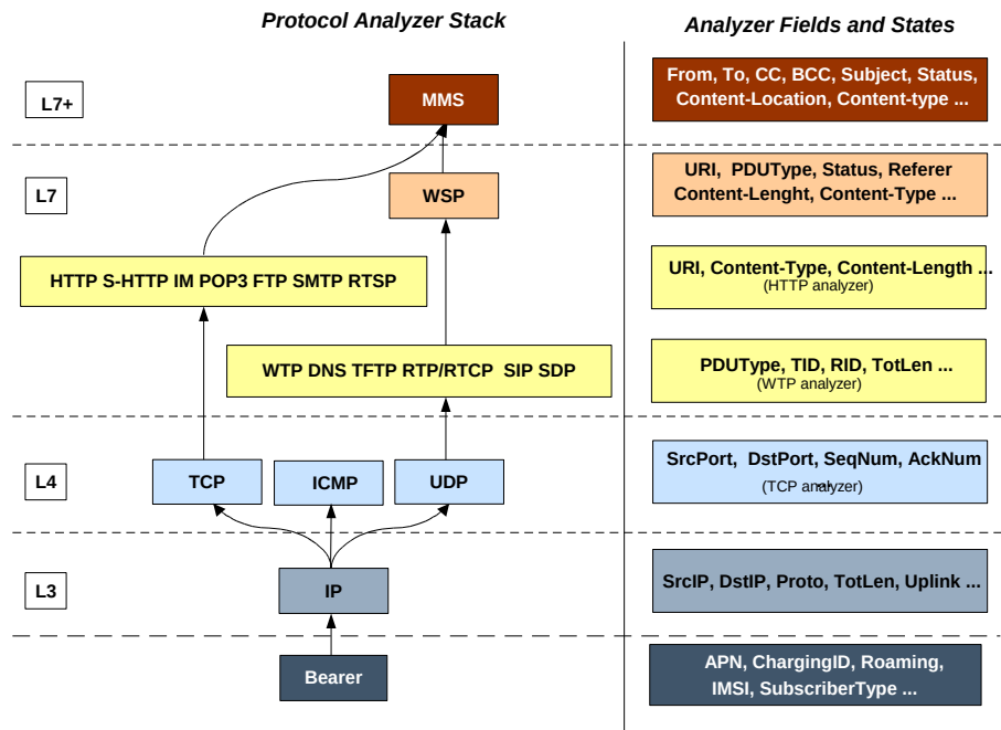
Figure 177. ECS Protocol Analyzer Stack
