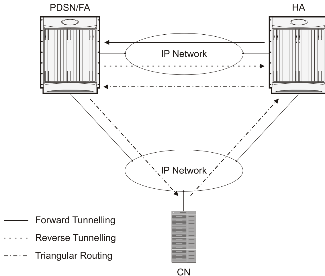
Figure 100. Mobile IP, FA and HA Tunneling/Transport Methods.
