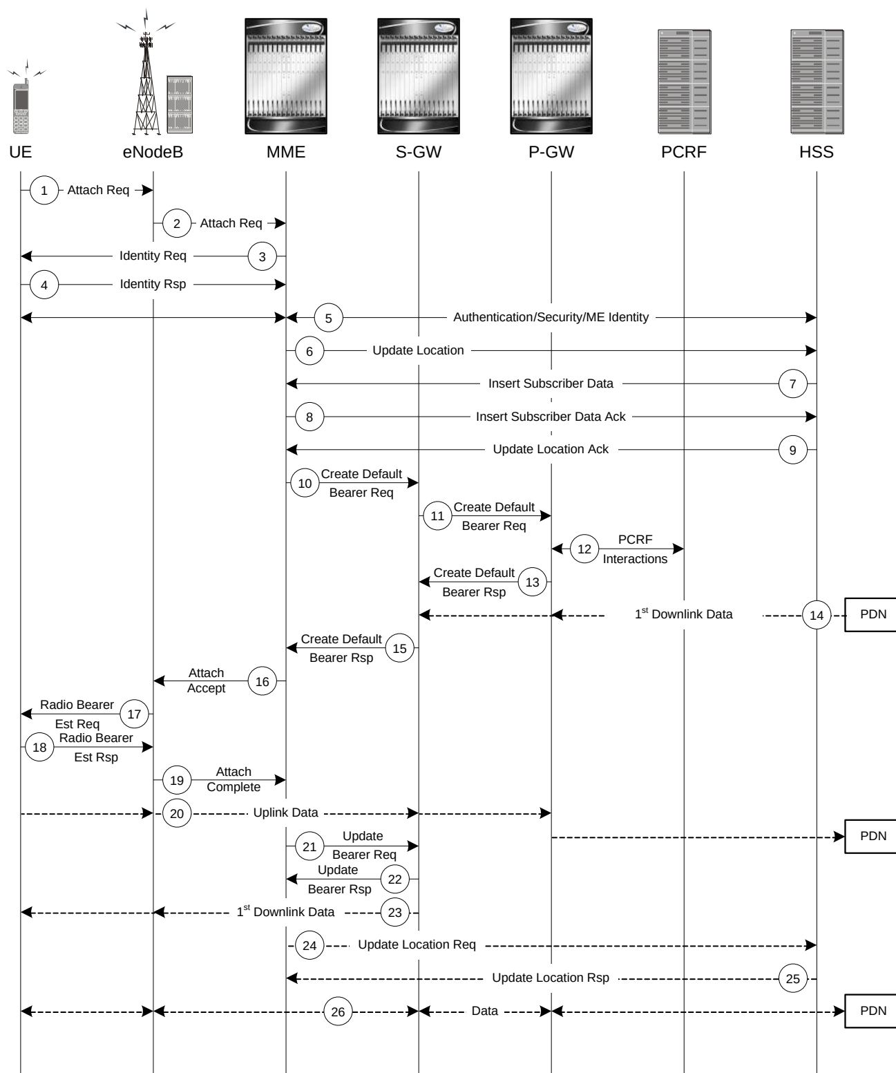
Figure 158. Subscriber-initiated Attach (initial) Call Flow
