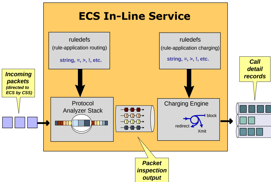
Figure 178. ECS In-line Service Processing
