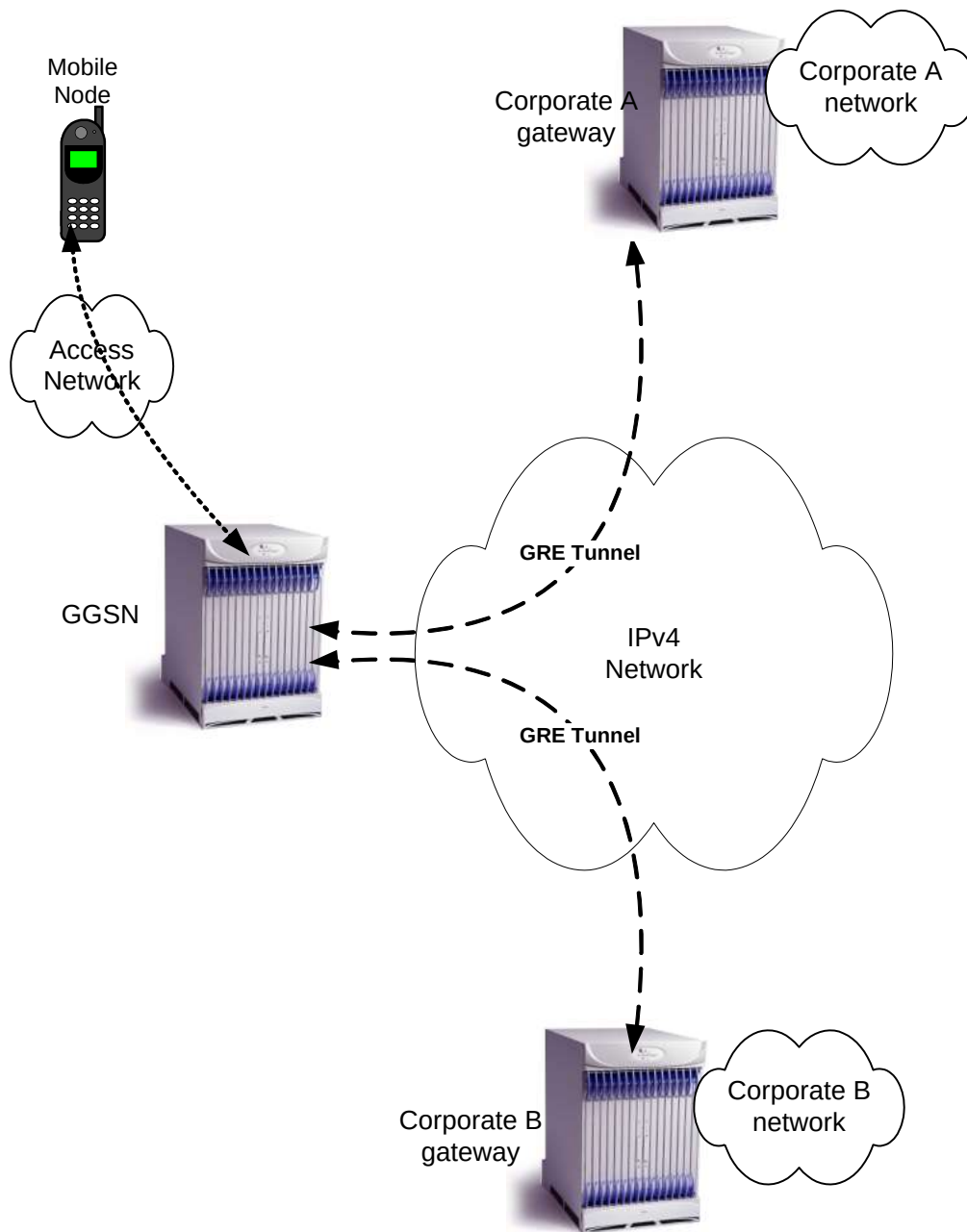
Figure 86. GRE Deployment Scenario
