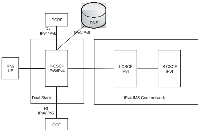
Figure 148. Interworking Between IPv6 UE and IPv4 IMS Core Network
