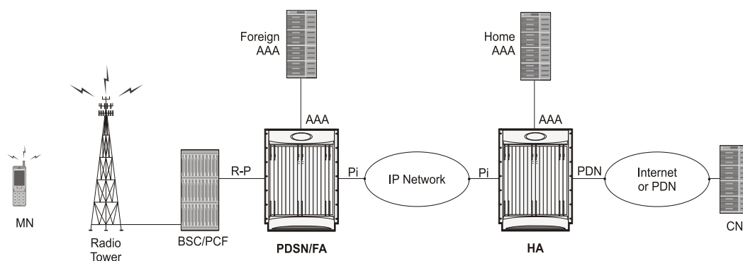
Figure 98. PDSN/FA and HA Network Deployment Configuration Example
