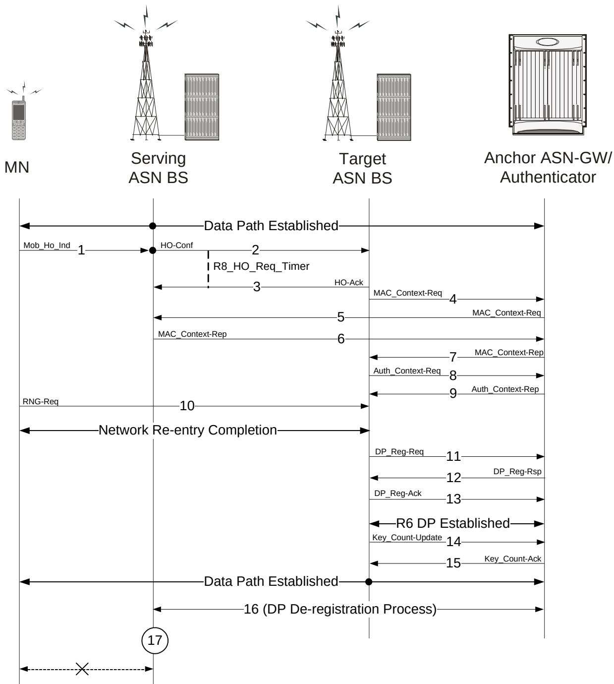
Figure 50. MS initiated Uncontrolled Intra-ASN Gateway Handover Action Phase
