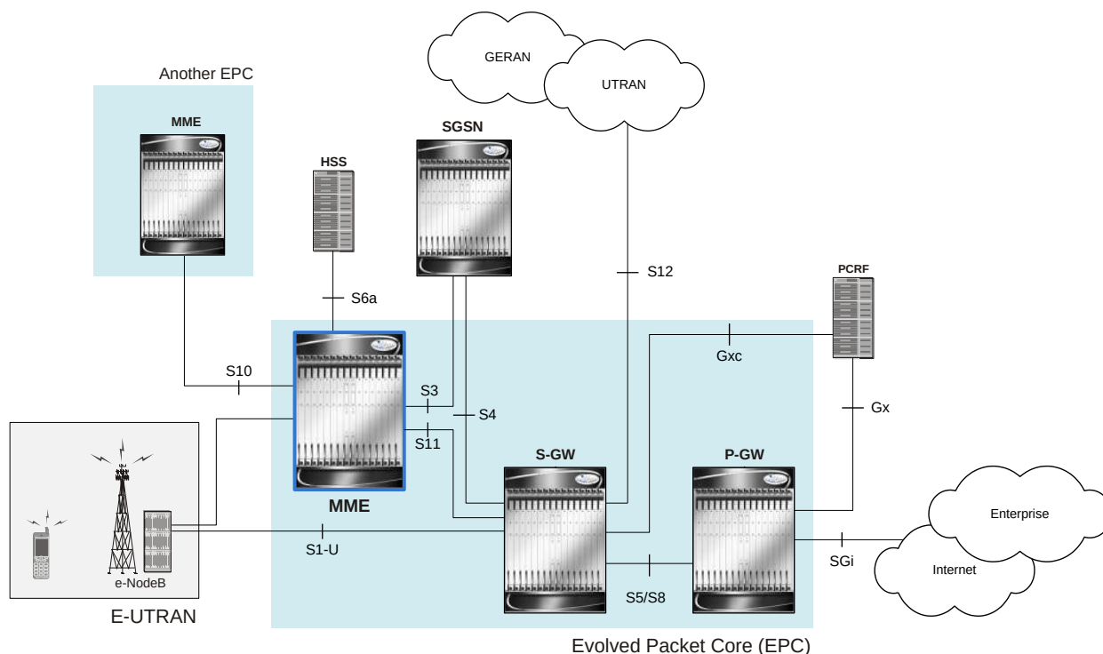
Figure 188. Architecture of LTE/SAE Network
