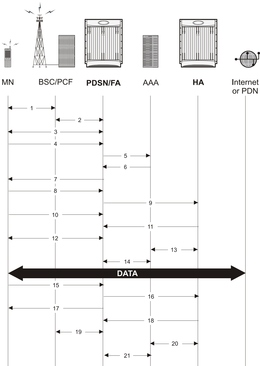
Figure 78. AAA/PDSN Assigned IP Address Proxy Mobile IP Call Flow
