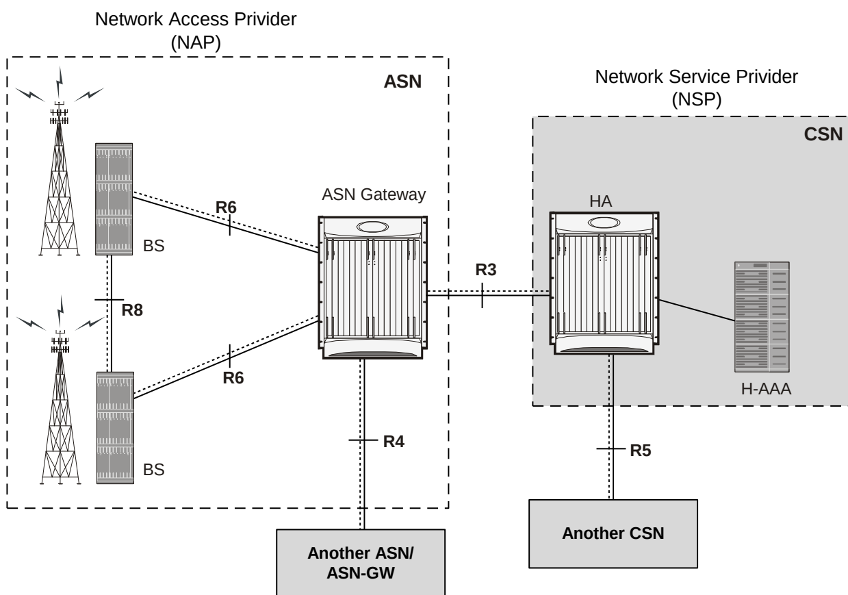
Figure 40. ASN Network Reference Model with ASN Gateway
