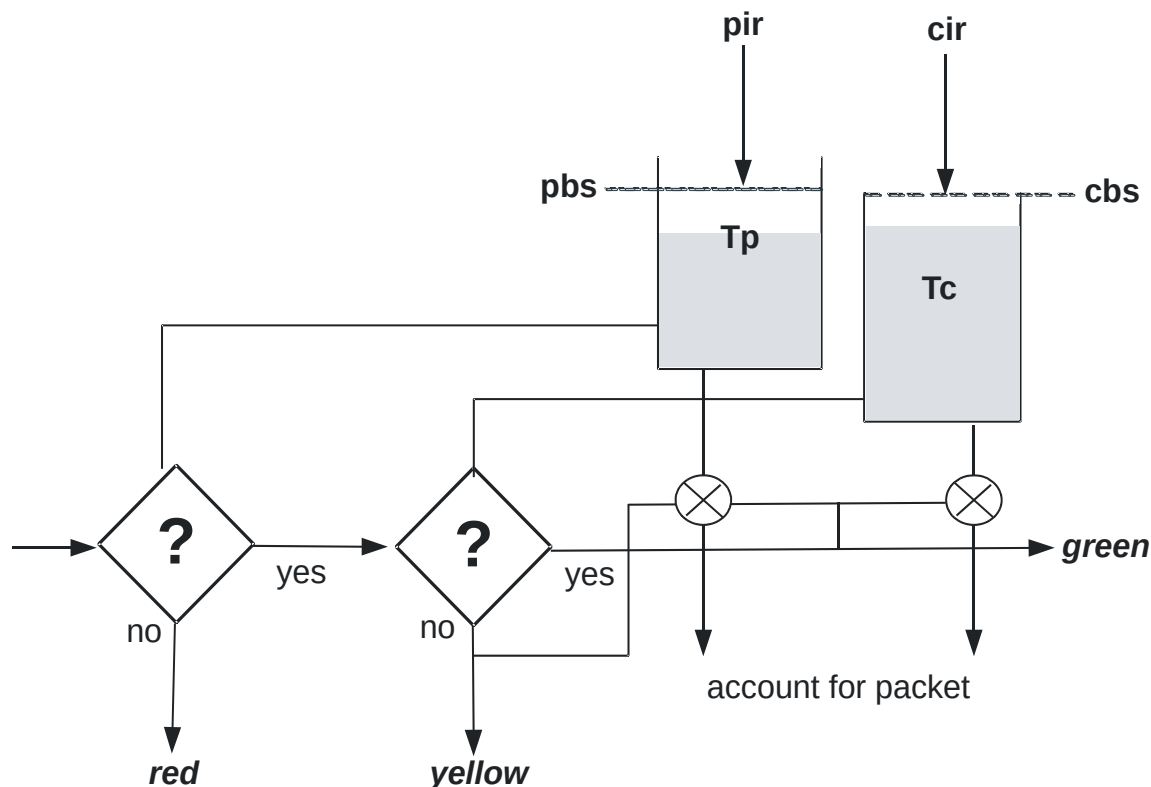
Figure 167. trTCM Algorithm Logic for Traffic Policing
