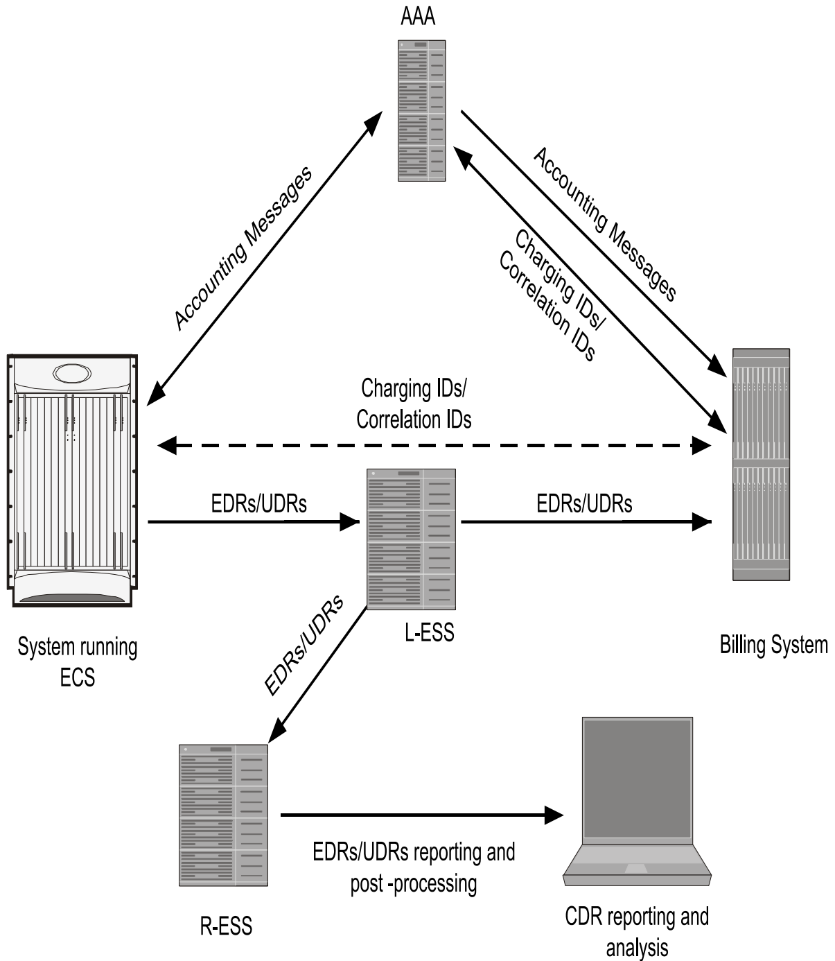
Figure 206. ESS architecture with ECS
