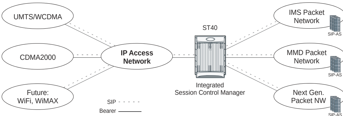
Figure 147. Cisco Integrated Session Control Manager
