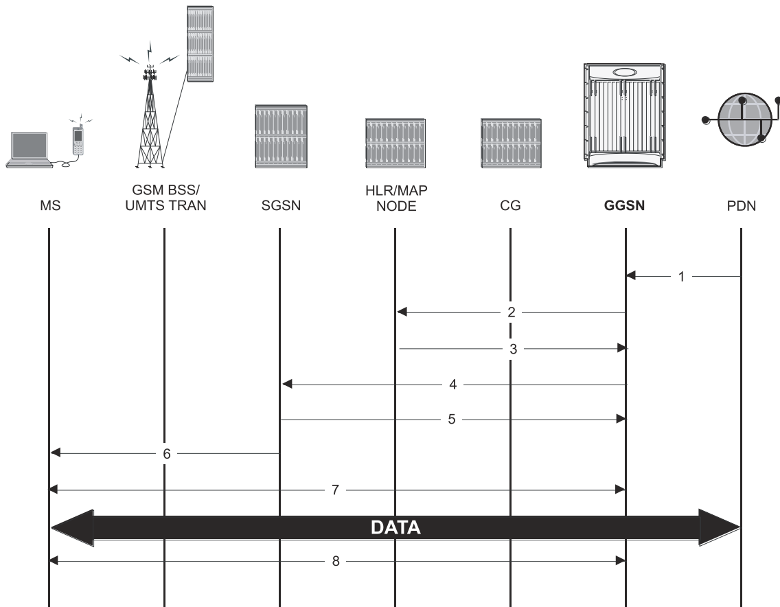
Figure 91. Network-initiated Session Call Flow
