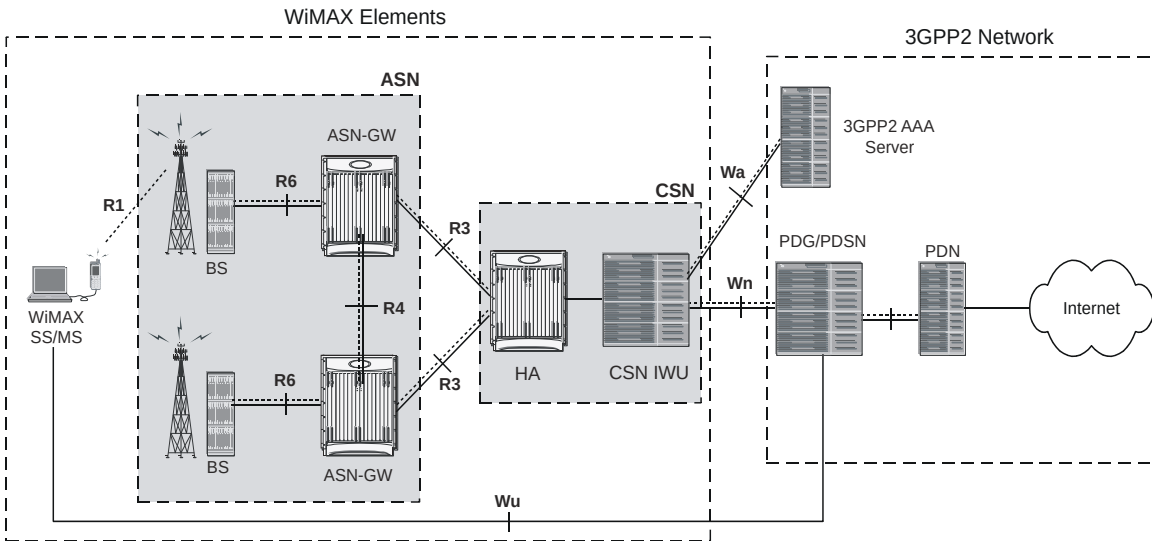
Figure 64. ASN Gateway with 3GPP2 Overlay
