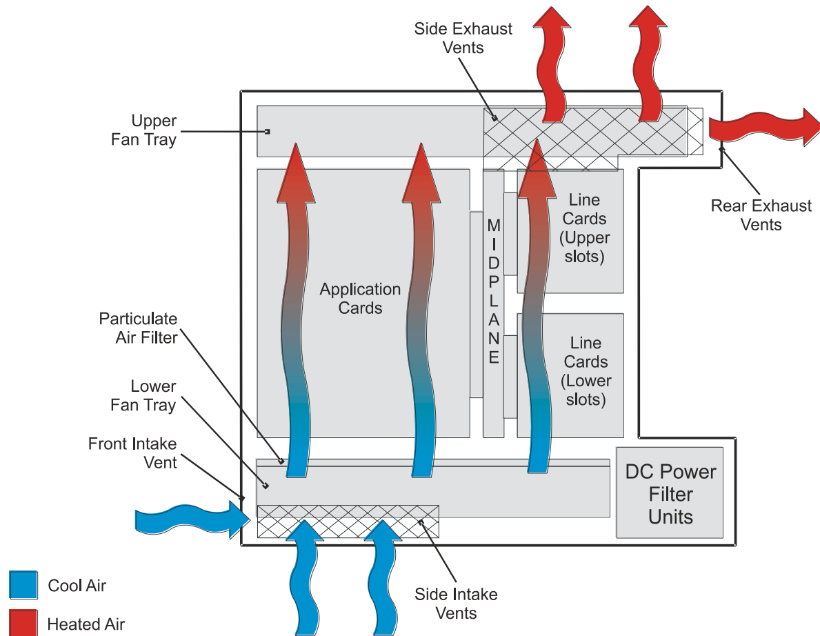
Figure 236. System Airflow and Ventilation
