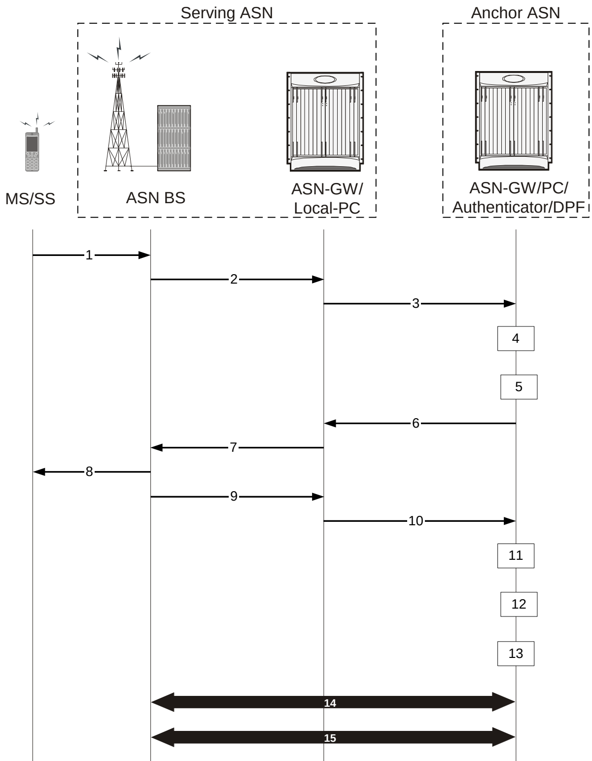
Figure 68. MS Initiated Idle Mode Entry Procedure Flow
