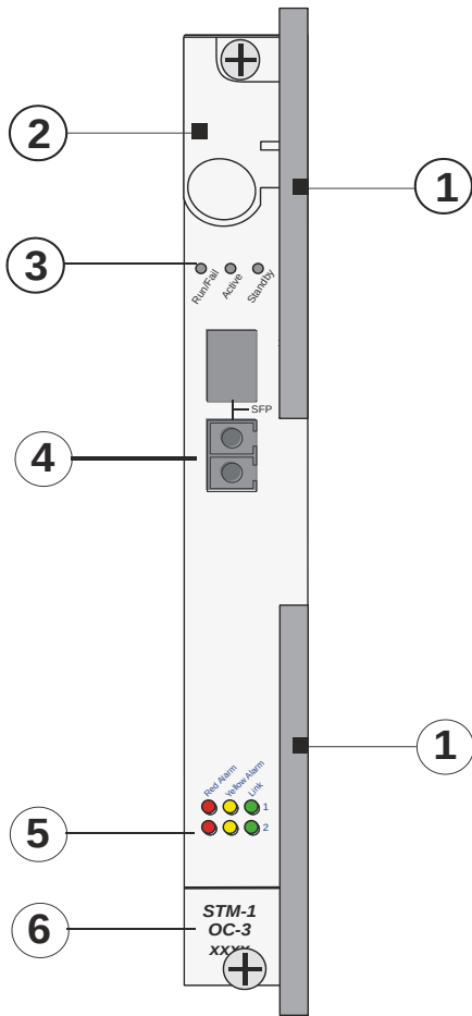
Figure 26. CLC Channelized Line Card
