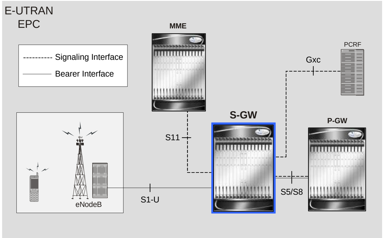
Figure 155. S-GW Interfaces in the E-UTRAN/EPC Network
