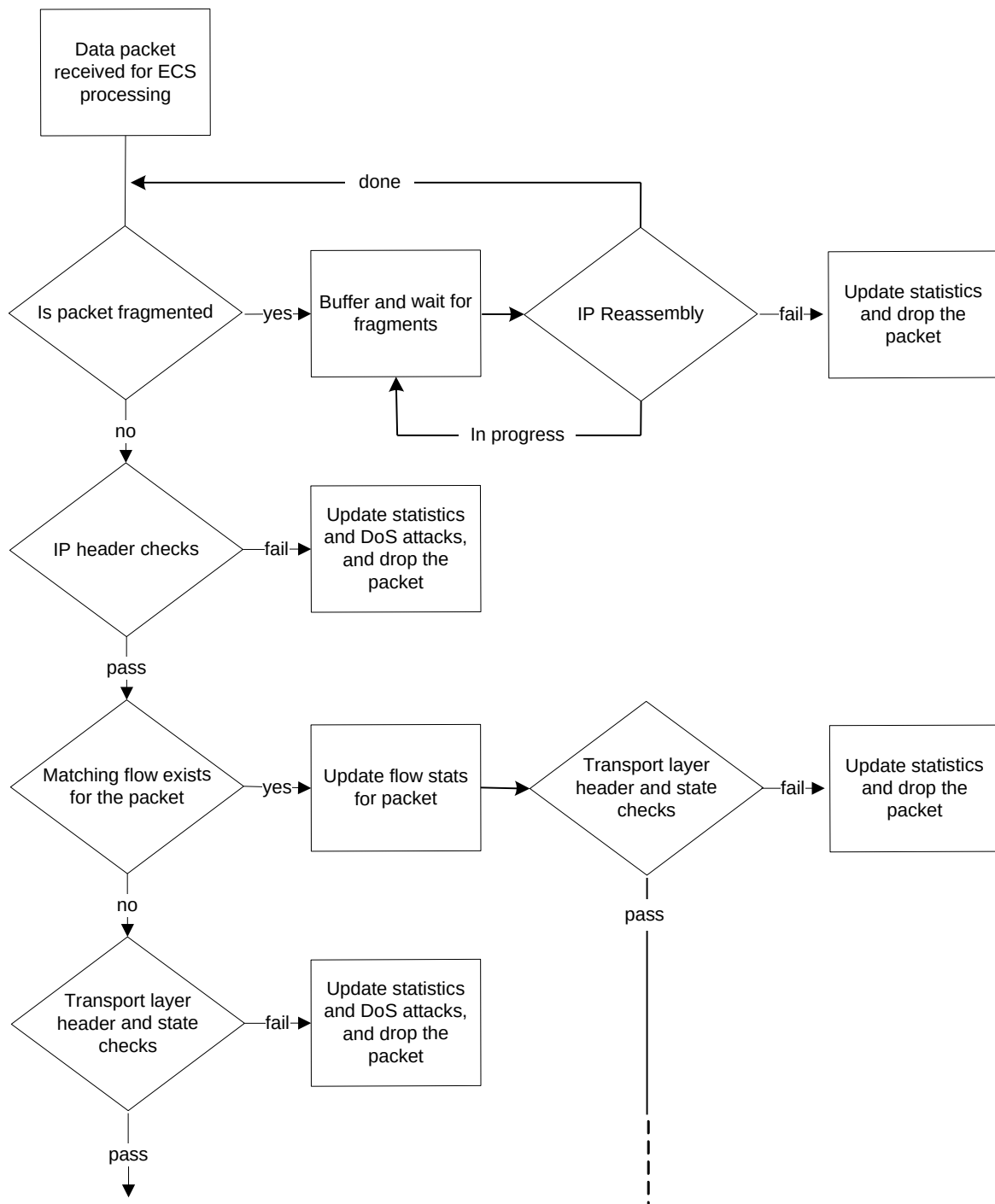
Figure 199. Stateful Firewall Processing
