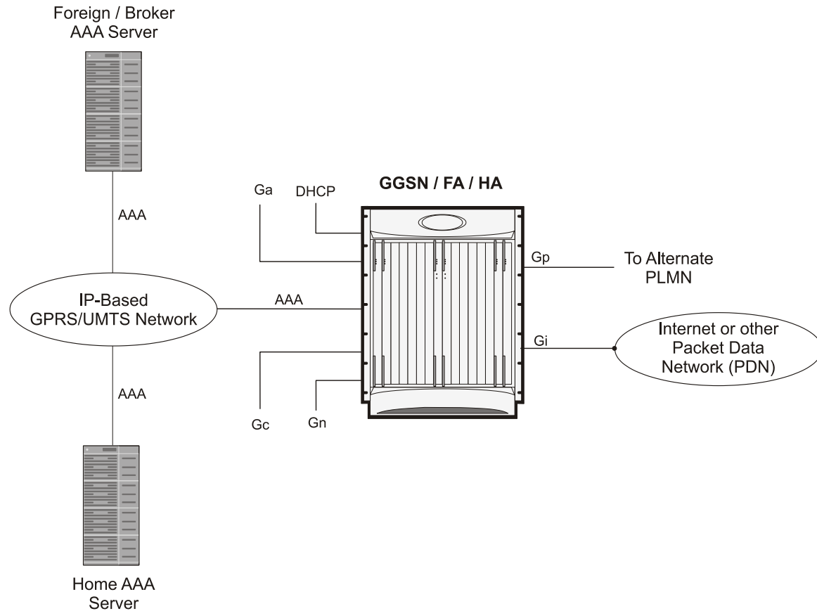
Figure 83. Combined GGSN/FA/HA Deployment for Mobile IP and/or Proxy Mobile IP Support
