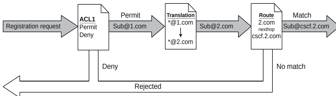
Figure 152. Admission and Routing Method
