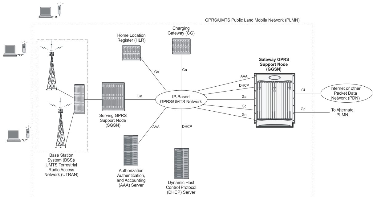
Figure 81. Basic GPRS/UMTS Network Topology
