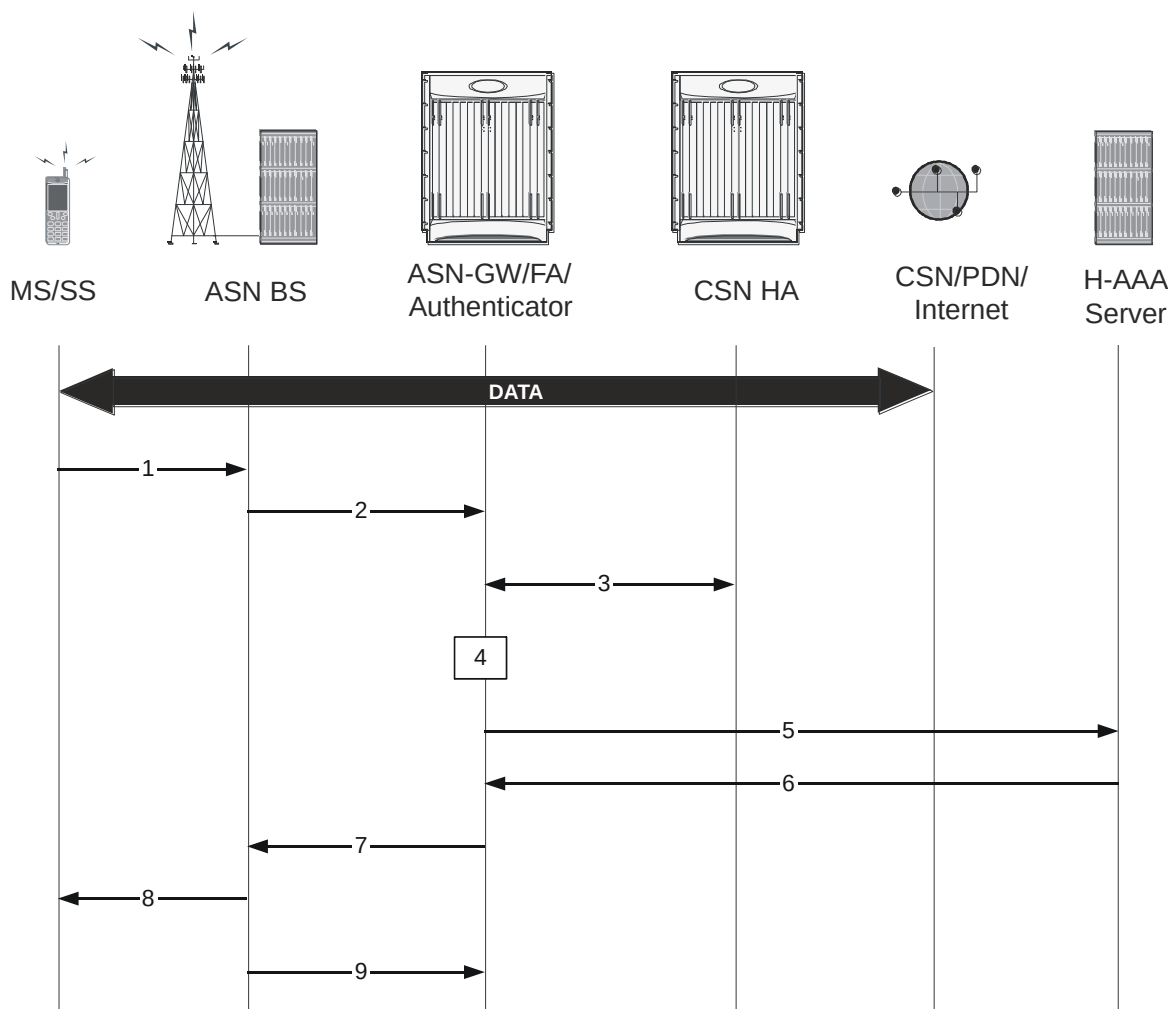
Figure 46. MS Triggered Network Exit Call Flow
