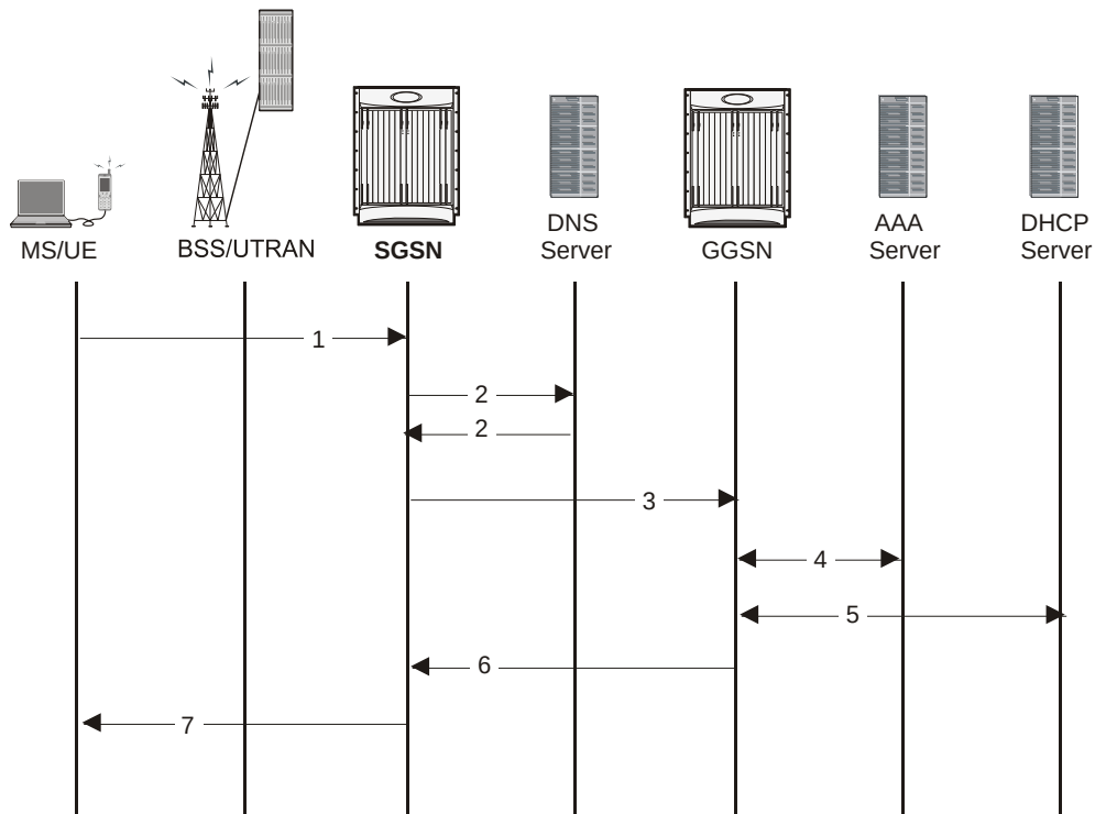
Figure 169. Call Flow for PDP Context Activation
