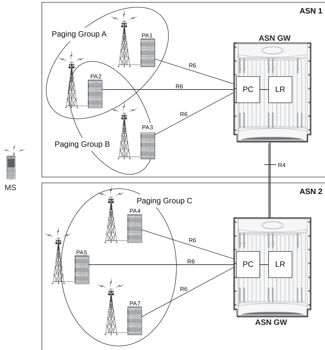
Figure 65. ASN Paging Controller and Location Registry in WiMAX Networks
