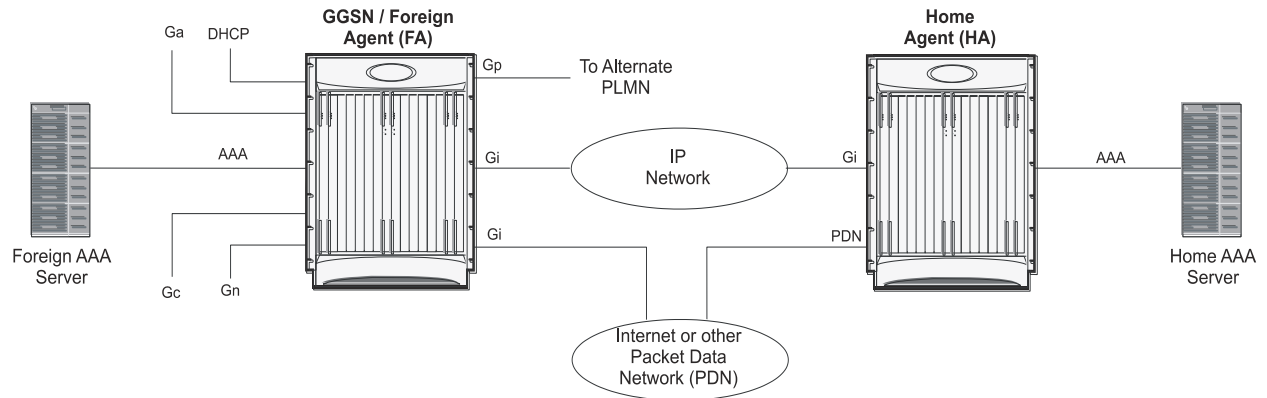
Figure 83. Combined GGSN/FA/HA Deployment for Mobile IP and/or Proxy Mobile IP Support
