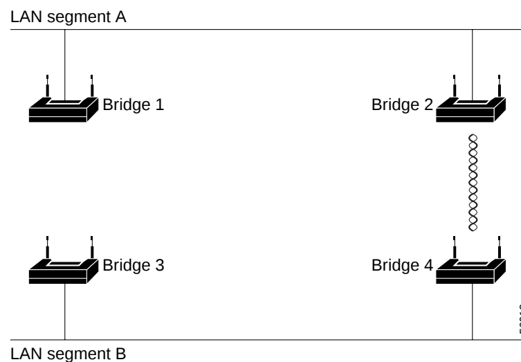
Figure 8-1 Spanning-Tree Topology
