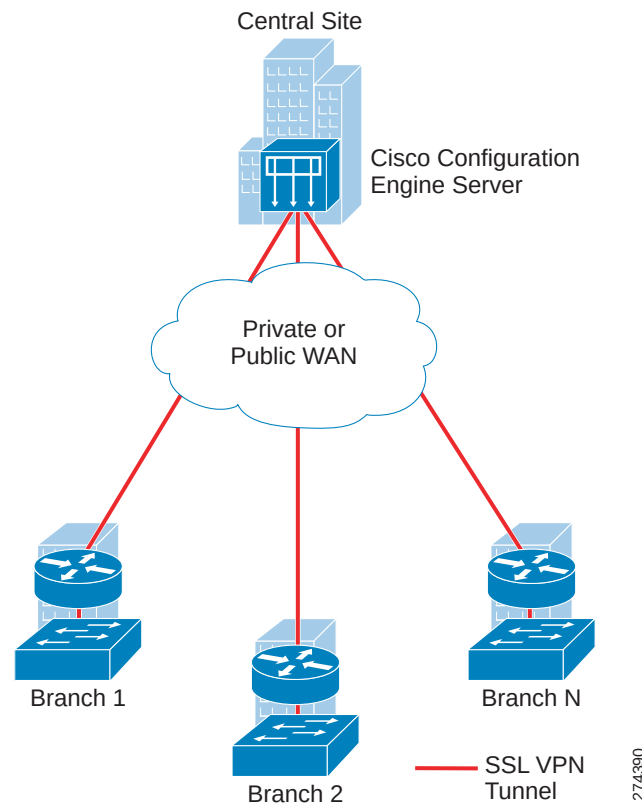
Figure 42 Deployment of CCE in the Streamlined Small Branch Network.
