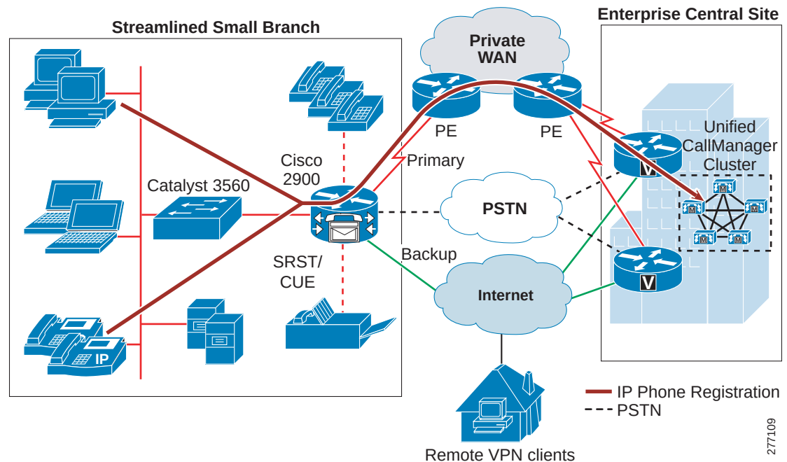
Figure 46 Centralized Call Control Model
