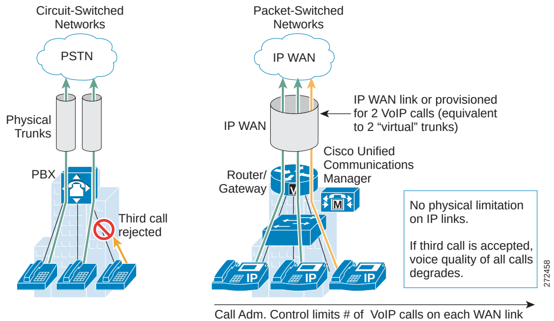
Figure 52 Traditional Versus VoIP Call Admission Control
