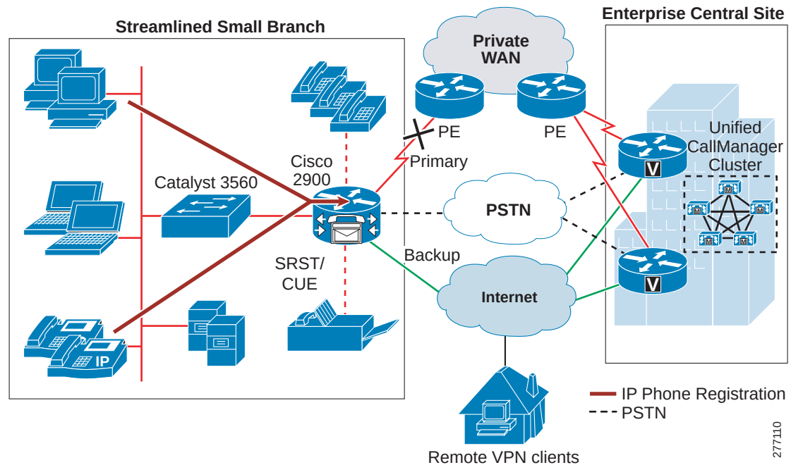
Figure 47 Cisco Unified SRST Mode for Centralized Call Control Model
