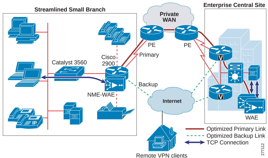
Figure 58 Cisco WAAS Optimization Path
