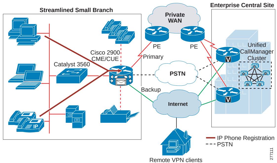
Figure 48 Distributed Call Control Model
