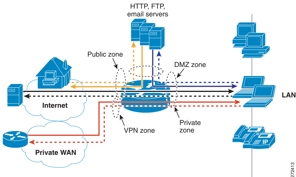
Figure 37 Security Zones
