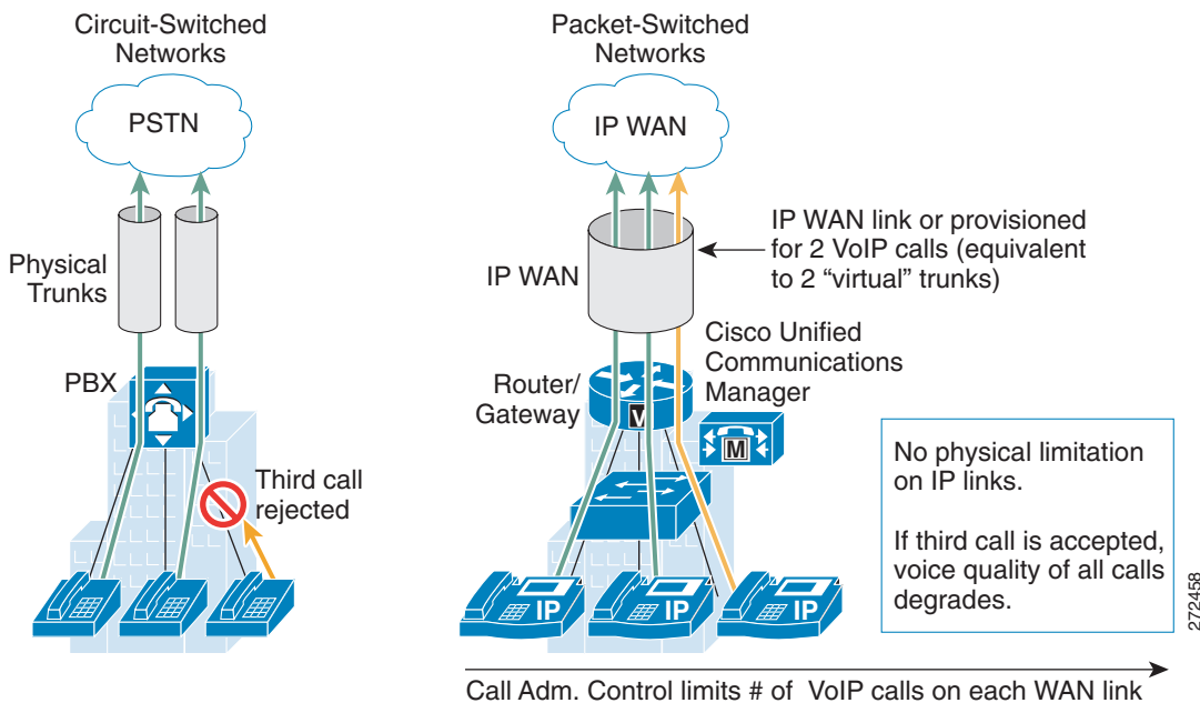
Figure 51 Traditional Versus VoIP Call Admission Control
