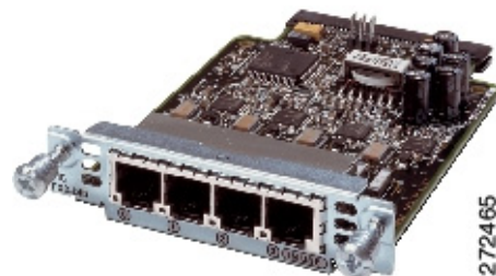
Figure 54 Four Port FXS/DID Voice Interface Card
