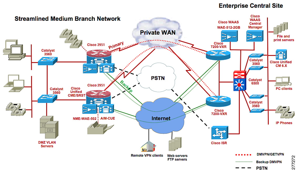
Figure 1 Streamlined Medium Branch Network Test Bed
