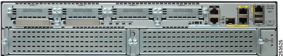
Figure 4 Interface Card and Service Module Configuration On a Cisco 2921
