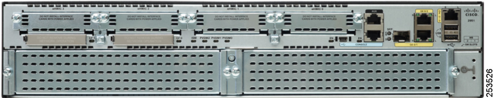
Figure 3 Interface Card and Service Module Configuration on a Cisco 2951 Router
