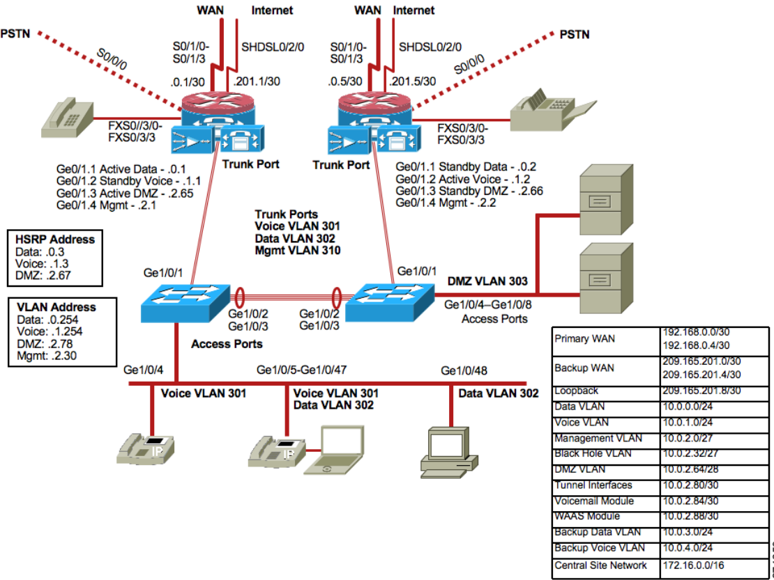
Figure 2 Streamlined Medium Branch Network Topology
