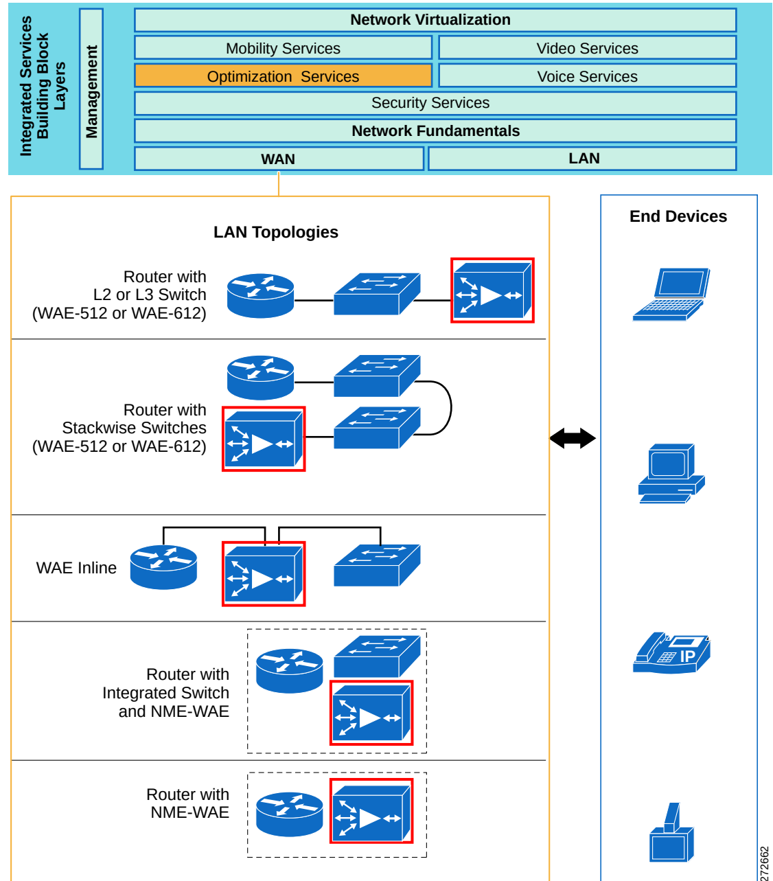
Figure 57 Cisco WAAS Deployment Options
