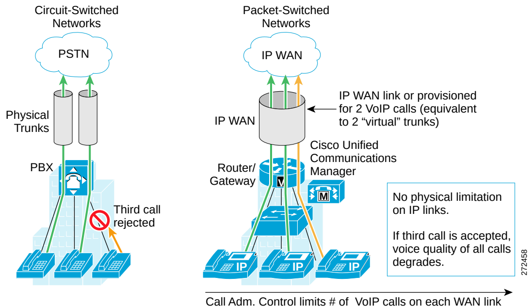
Figure 53 Traditional Versus VoIP Call Admission Control
