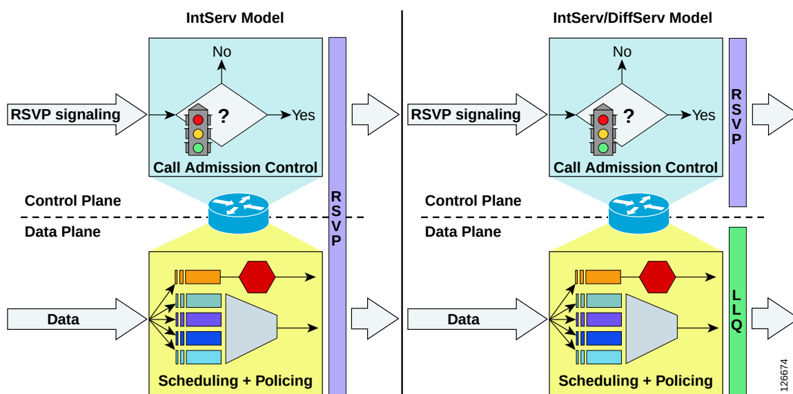
Figure 54 RSVP Operational Models: IntServ and IntServ/DiffServ
