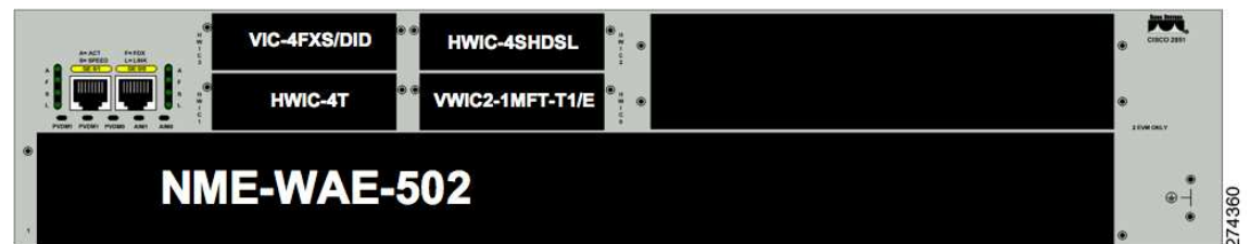
Figure 3 Interface Card and Service Module Configuration on a Cisco 2951 Router
