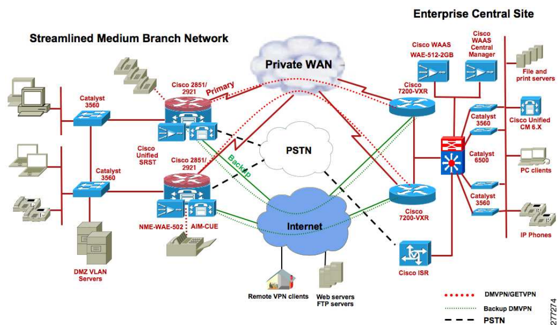
Figure 2 Private WAN, Cisco Unified SRST Mode
