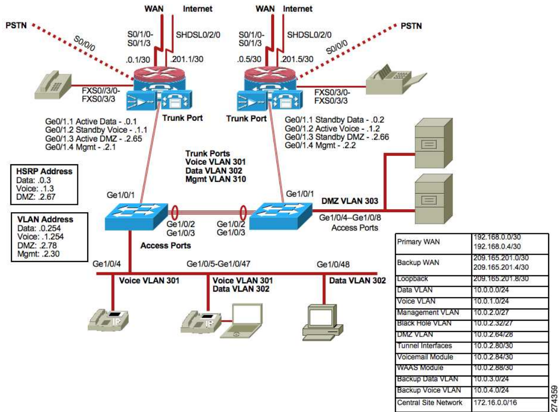
Figure 2 Streamlined Medium Branch Network Topology
