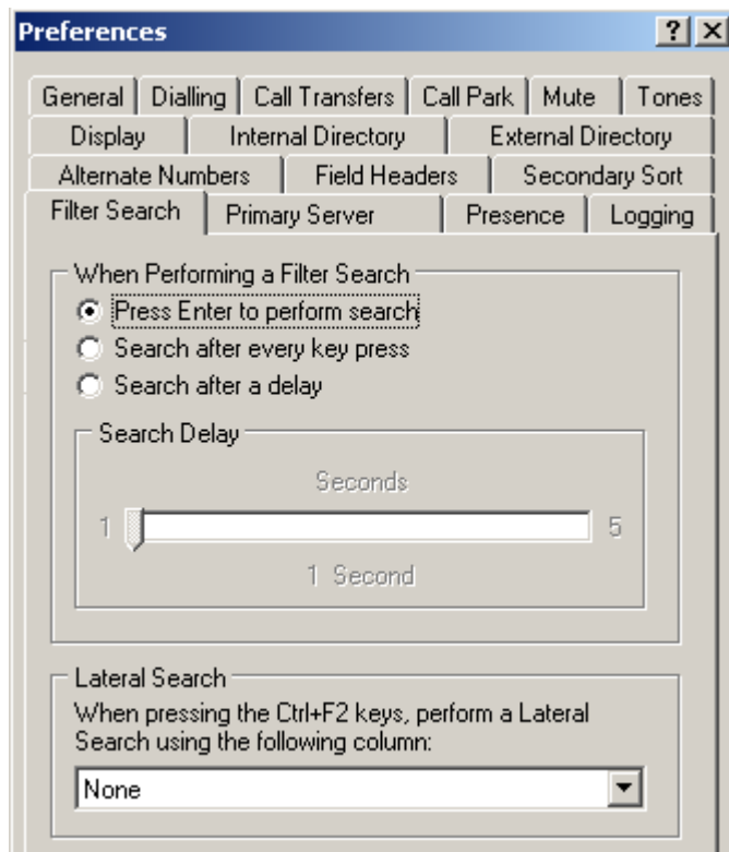
Figure 2-13 Displays the Filter Search Tab in the Preferences Section
