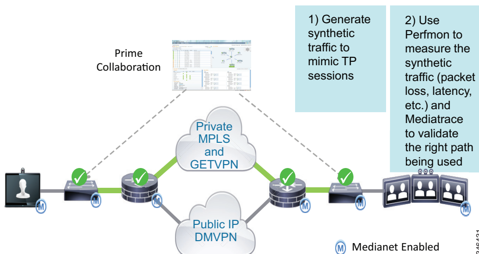
Figure 3-28 Pre-Deployment Assessment Procedure
