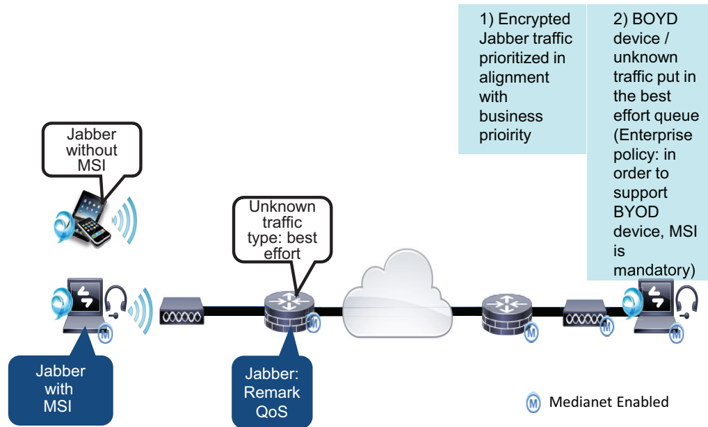
Figure 3-33 Recommended QoS Policy for Jabber
