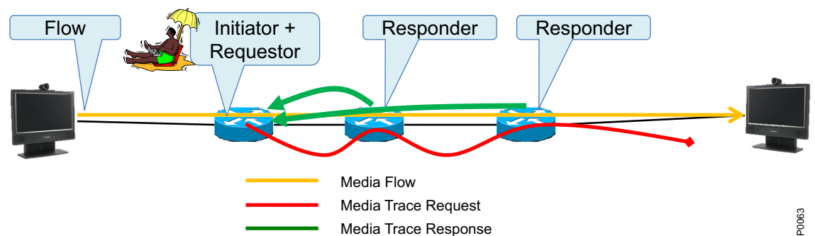
Figure 3-25 Mediatrace Initiated from a Local Router Using the CLI
