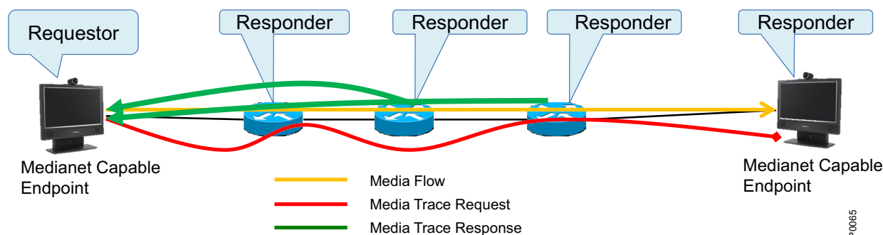
Figure 3-27 Mediatrace Initiated from an Endpoint
