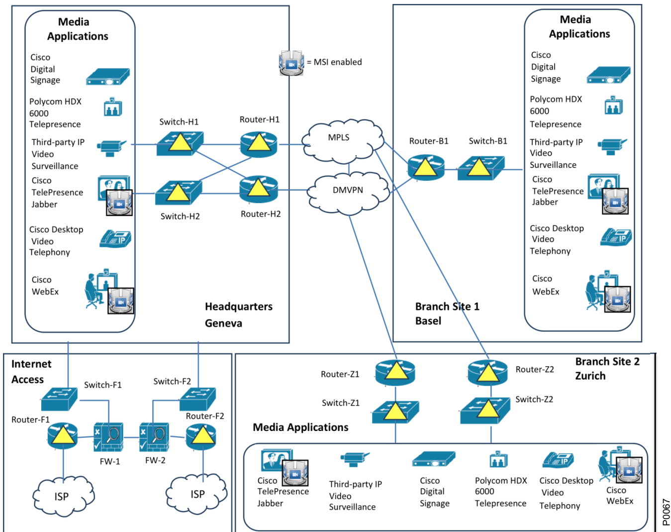
Figure 3-31 Deploying Flow Metadata on Campus and Branch
