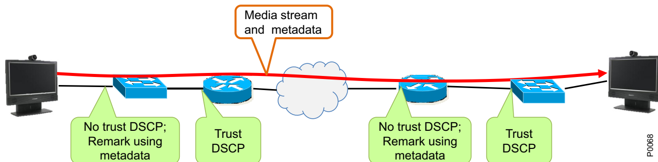
Figure 3-32 DSCP Re-Making of Traffic Using Metadata
