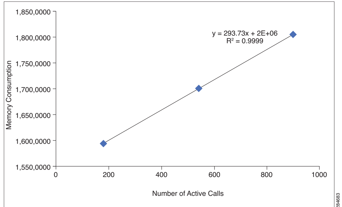
Figure 29-4 Memory Consumption Per Active Call
