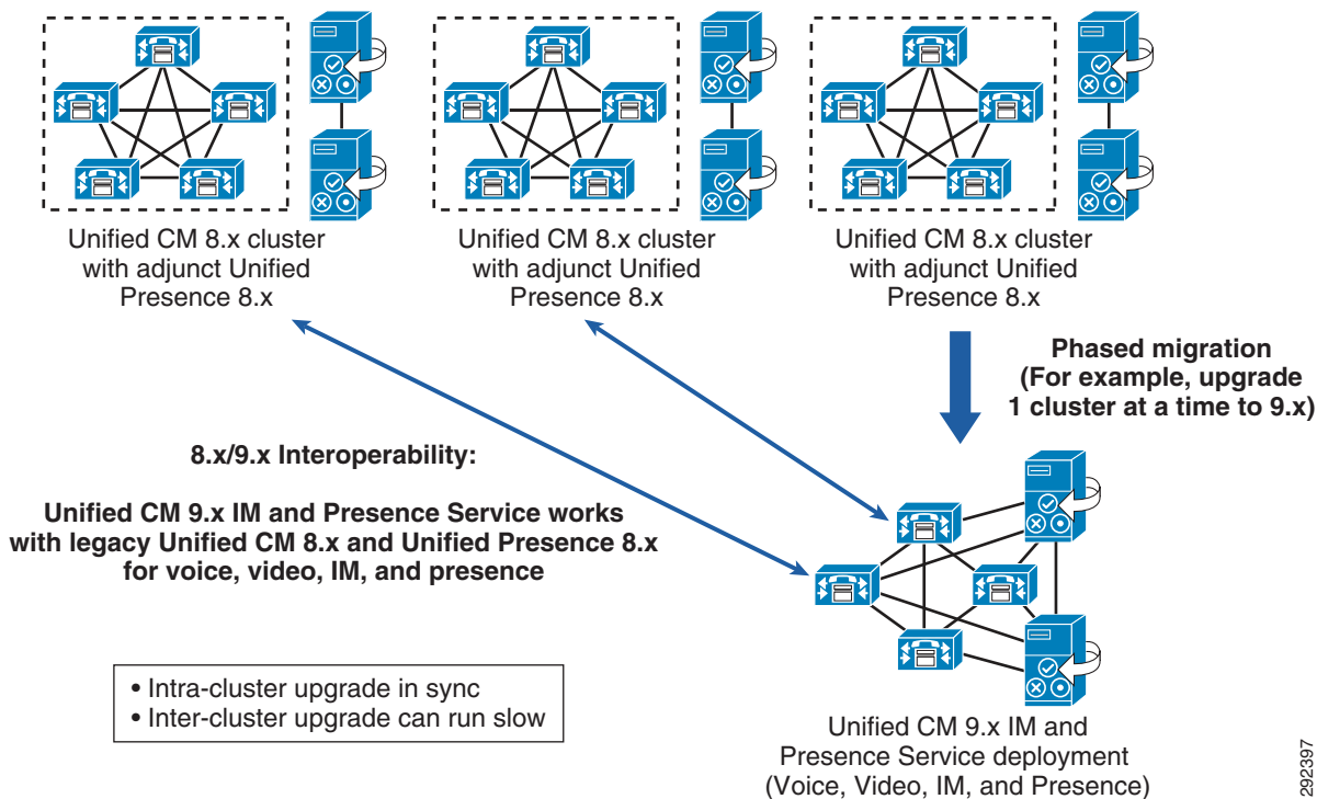
Figure 23-14 Large Enterprise Migration with Backward Compatibility
