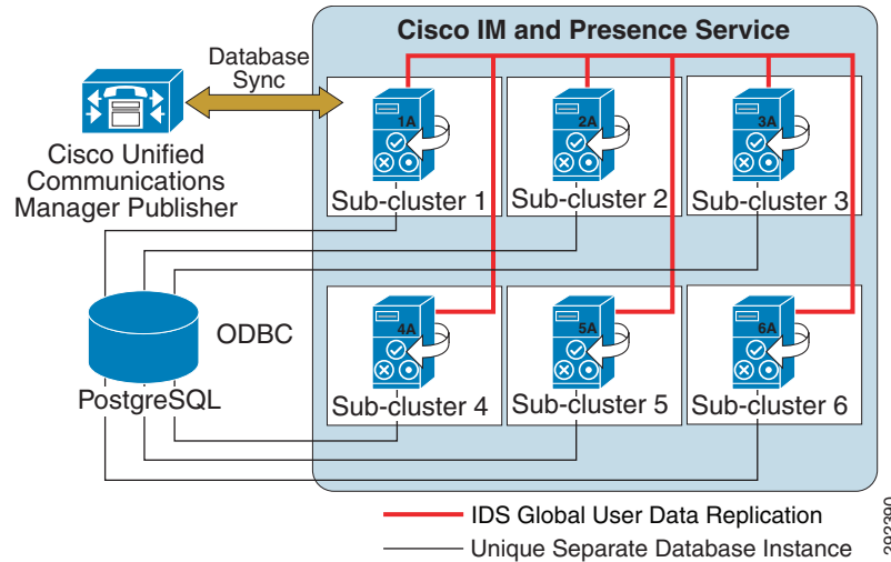
Figure 23-15 Cisco IM and Presence Persistent Chat
