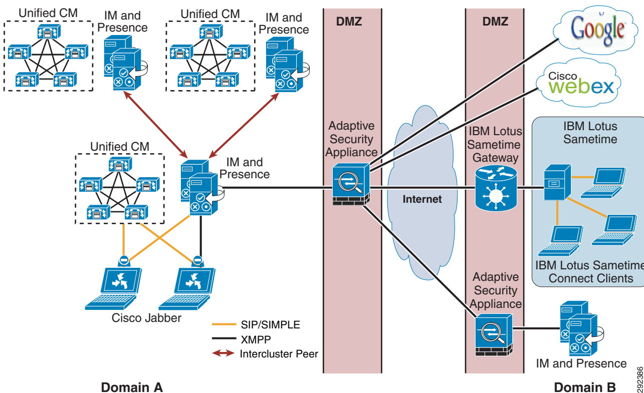
Figure 23-10 Cisco IM and Presence XMPP Federation (Inter-Domain)
