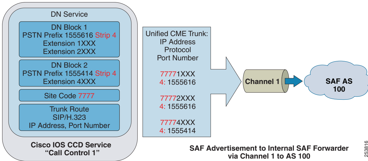
Figure 5-32 Cisco IOS CCD Service Call Control 1 Advertising Through Channel 1 to SAF AS 100
