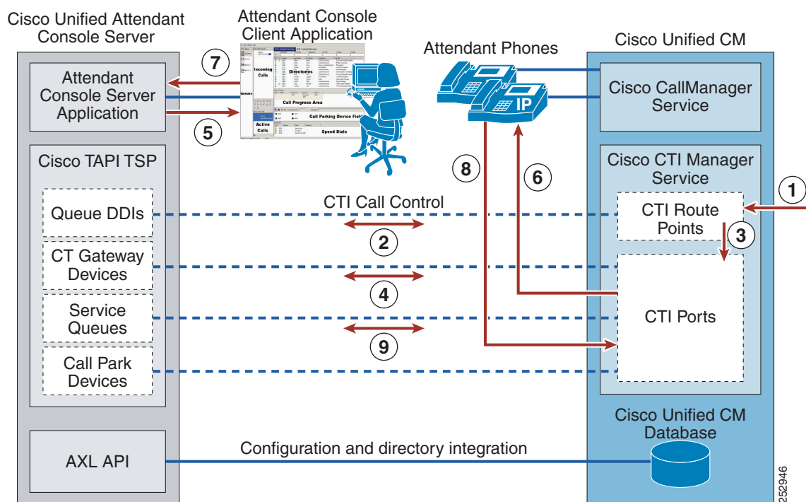
Figure 19-18 Architecture for Cisco Unified Department, Business, and Enterprise Attendant Consoles
