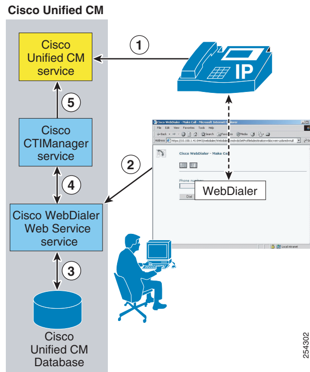
Figure 19-16 WebDialer Architecture
