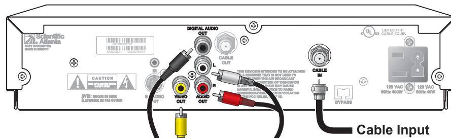
Explorer 3250 DHCT
