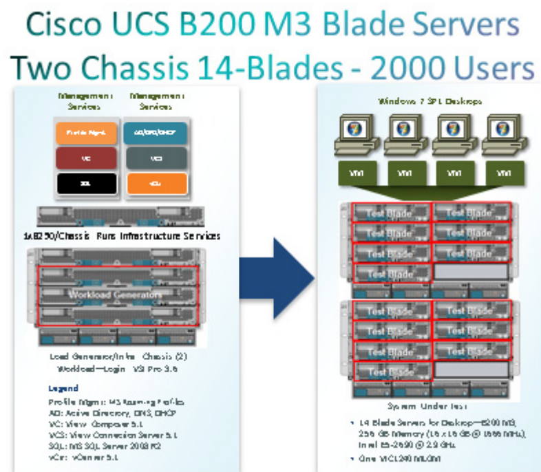
Figure 20 Two Chassis Test Configuration-14 x B200 M3 Blade Servers
