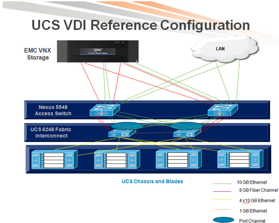
Figure 9 Architecture Block Diagram
