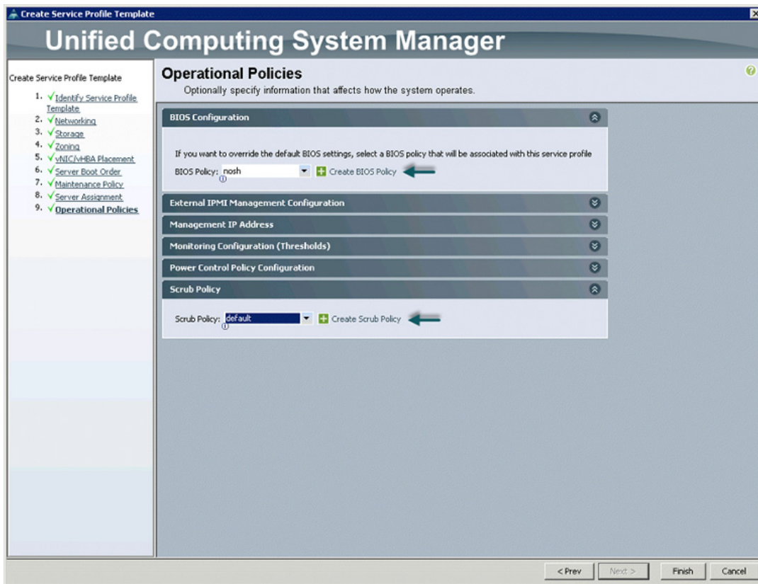
Figure 41 Creating Operational Policies
