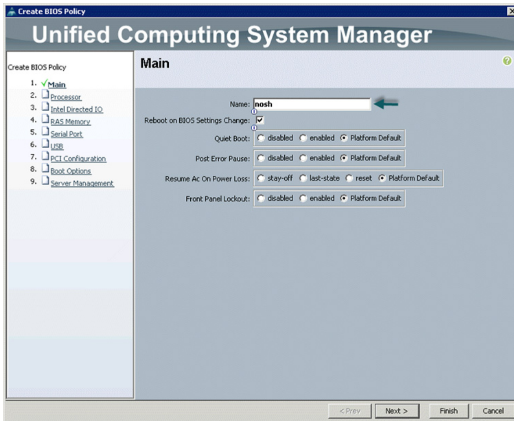
Figure 25 Creating BIOS Policy
