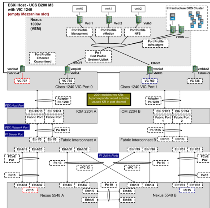
Figure 11 FlexPod Distinct Uplink Design: Cisco UCS B-Series and Cisco Nexus 5500 Focus
