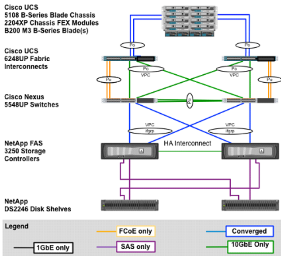
Figure 3 FlexPod: Distinct Uplink Design with Data ONTAP in 7-Mode
