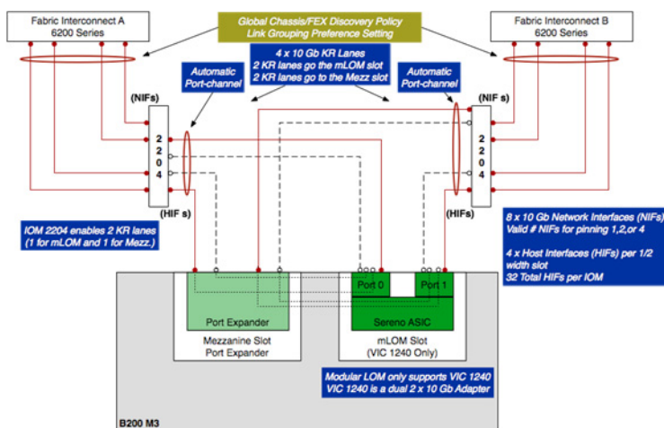
Figure 15 Validated Cisco UCS Backplane Configuration - VIC 1240 with Port Extender
