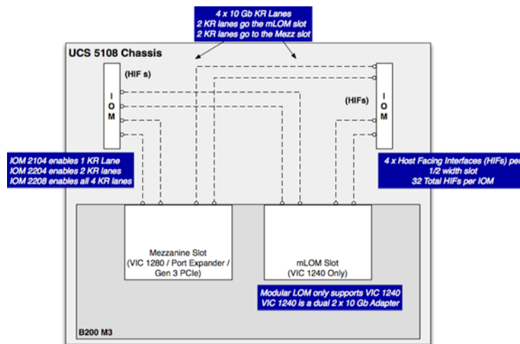
Figure 24 Generic Cisco UCS B-Series M3 Backplane
