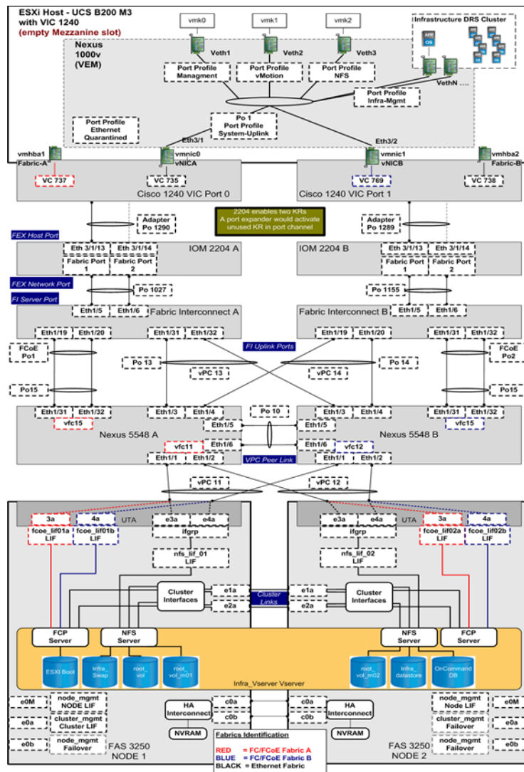
FlexPod Distinct Uplink Design with Clustered Data ONTAP (Switchless Cluster)
