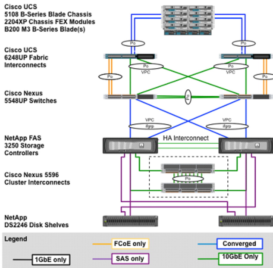
Figure 2 FlexPod: Distinct Uplink Design with Clustered Data ONTAP
