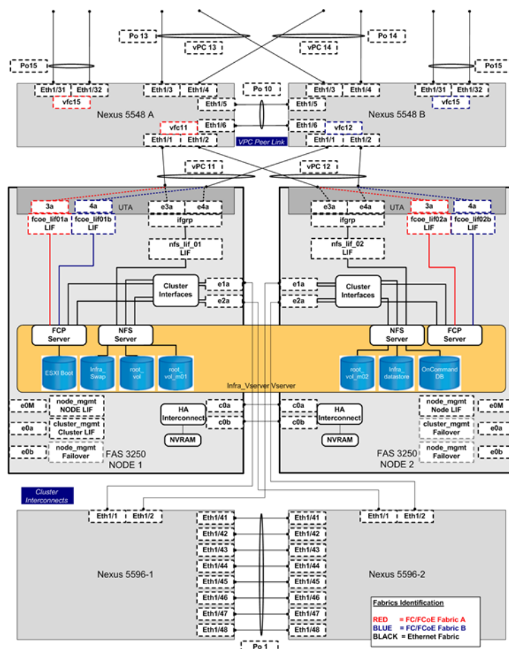
Figure 17 FlexPod
