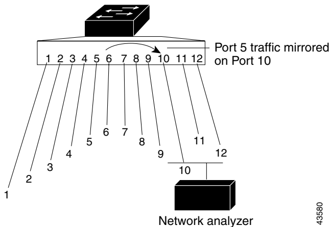
Figure 21-1 Example of Local SPAN Configuration on a Switch
