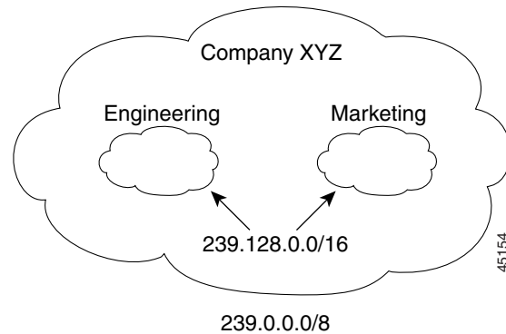
Figure 31-5 Administratively-Scoped Boundaries
