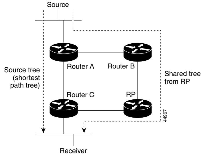
Figure 31-4 Shared Tree and Source Tree (Shortest-Path Tree)
