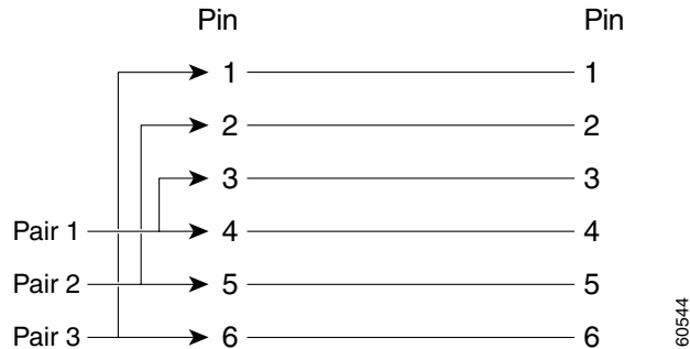
Figure B-6 Telephone Straight-Through Cable Schematic
