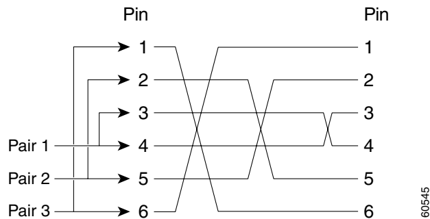
Figure B-7 Telephone Rollover Cable Schematic
