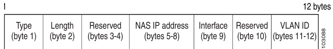
Figure 14-2 Format of the Agent Remote ID Suboption
