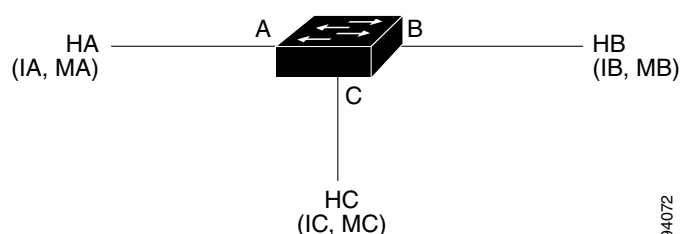
Figure 46-1 ARP Cache Poisoning
